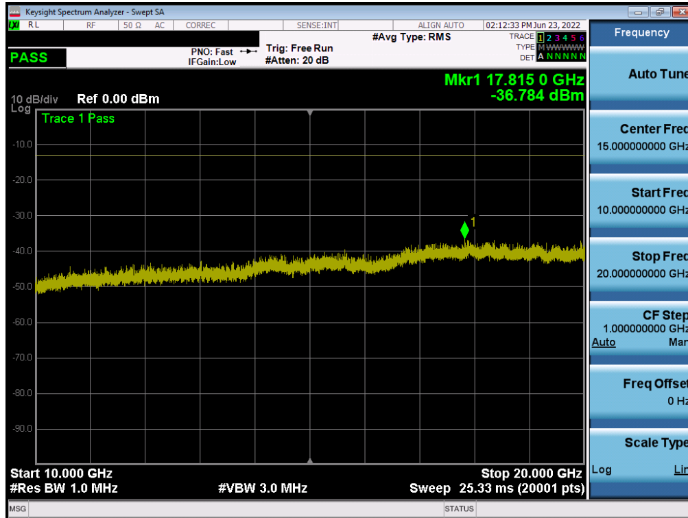
Plot 7-5. Conducted Spurious Plot (GPRS Ch. 128)
