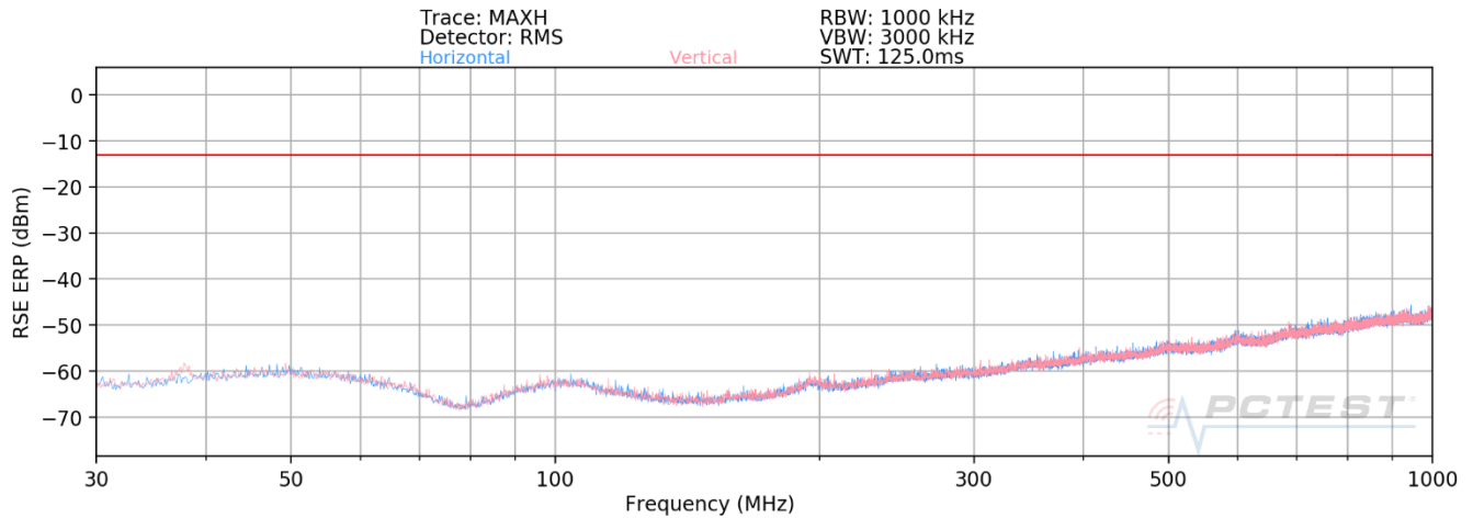
Plot 7-16. Radiated Spurious Plot Below 1GHz (GPRS Cell) – OPEN
