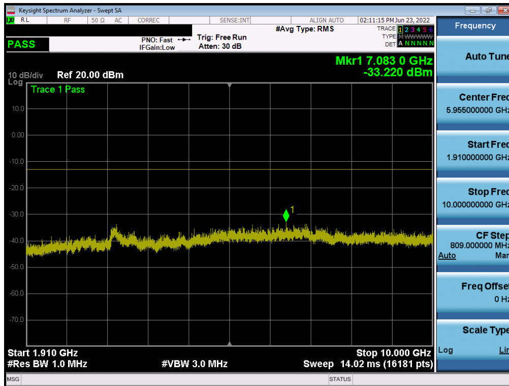
Plot 7-7. Conducted Spurious Plot (GPRS Ch. 190)
