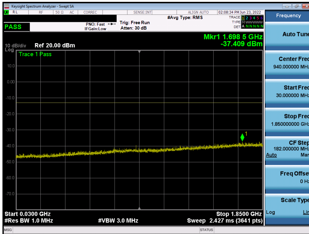
Plot 7-9. Conducted Spurious Plot (GPRS Ch. 251)
