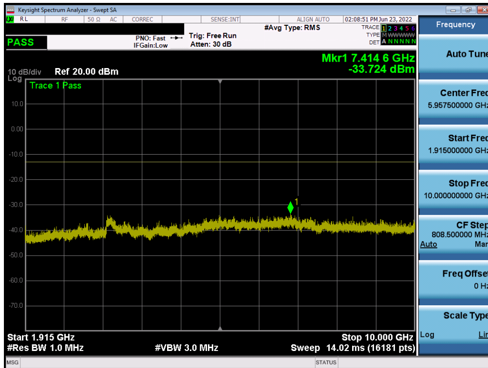
Plot 7-10. Conducted Spurious Plot (GPRS Ch. 251)
