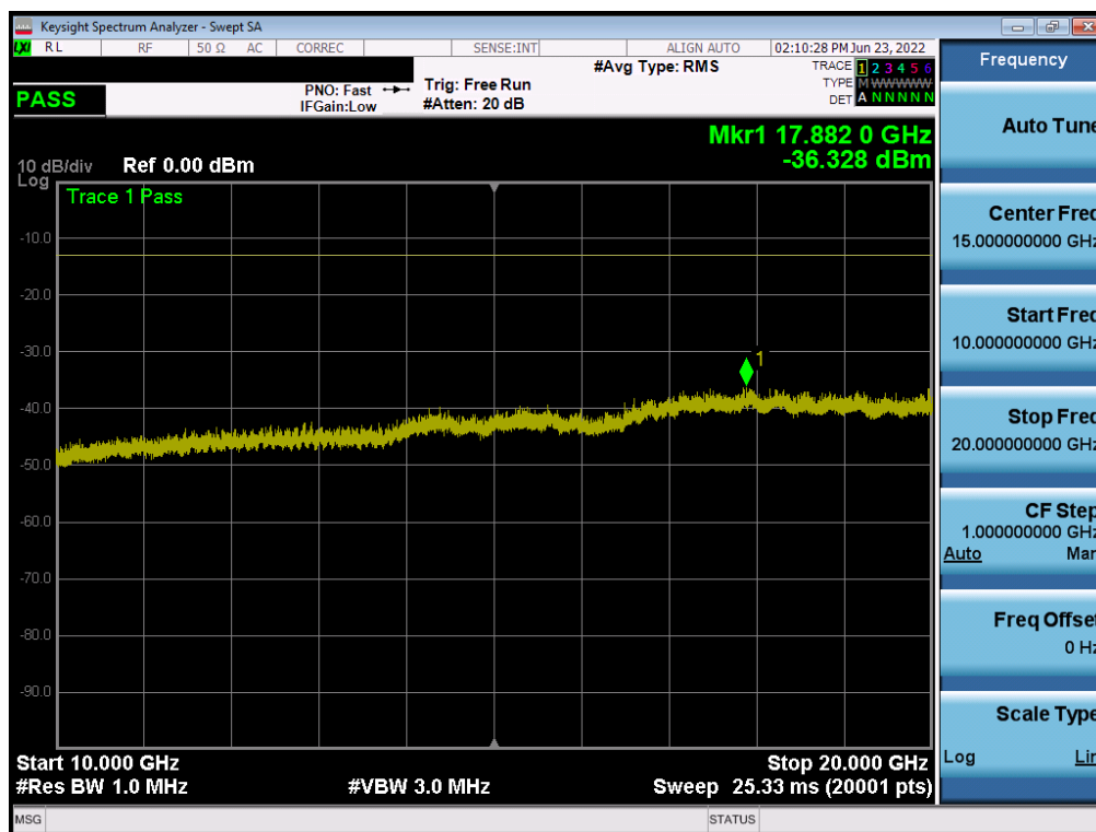
Plot 7-11. Conducted Spurious Plot (GPRS Ch. 251)
