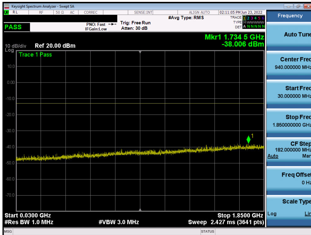
Plot 7-6. Conducted Spurious Plot (GPRS Ch. 190)
