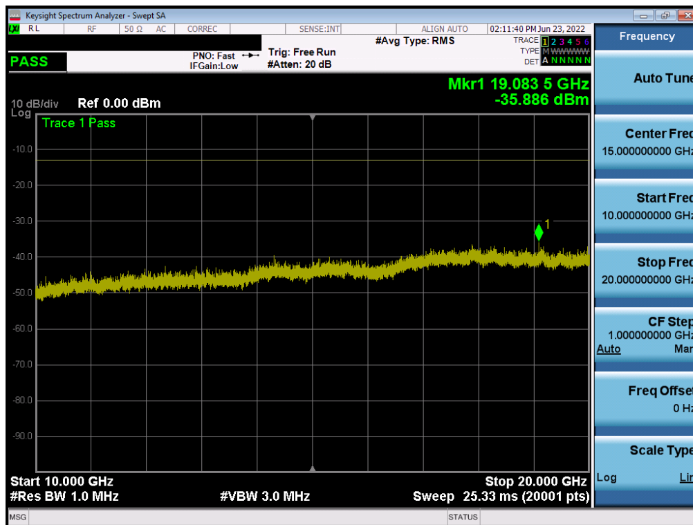
Plot 7-8. Conducted Spurious Plot (GPRS Ch. 190)
