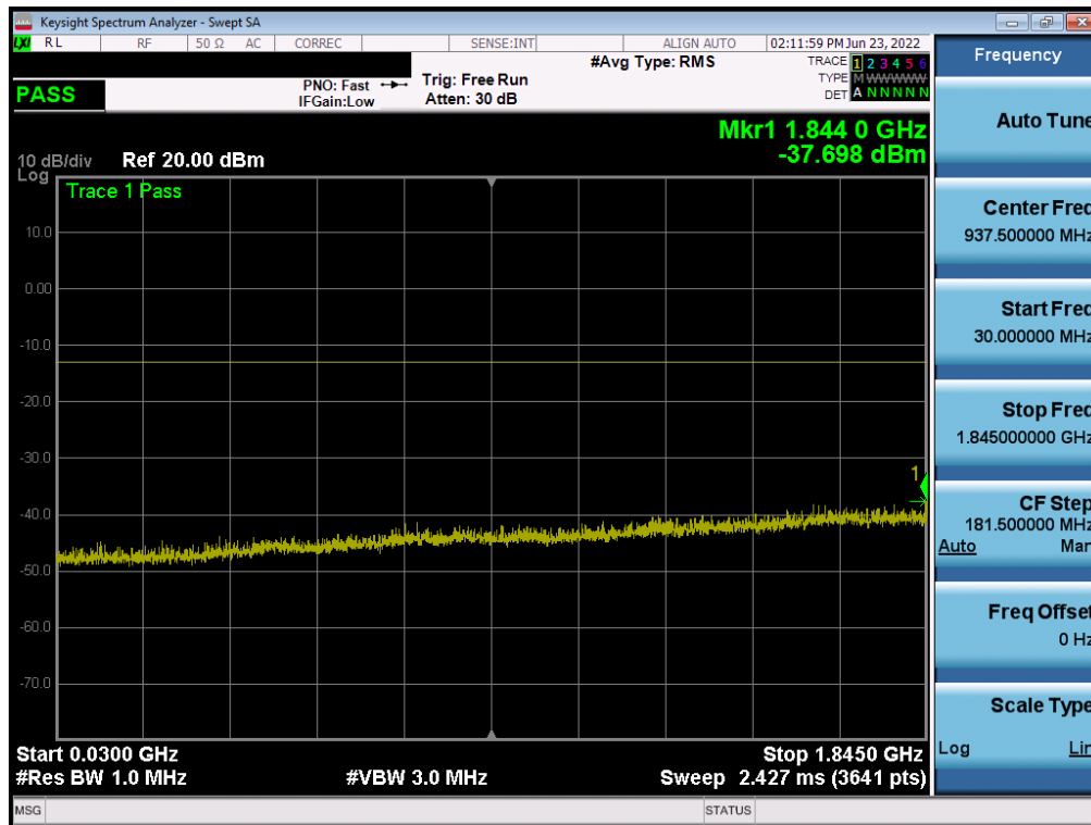
Plot 7-3. Conducted Spurious Plot (GPRS Ch. 128)
