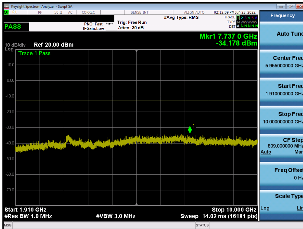
Plot 7-4. Conducted Spurious Plot (GPRS Ch. 128)
