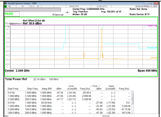
BPSK Low channel 1RB_Offset High
