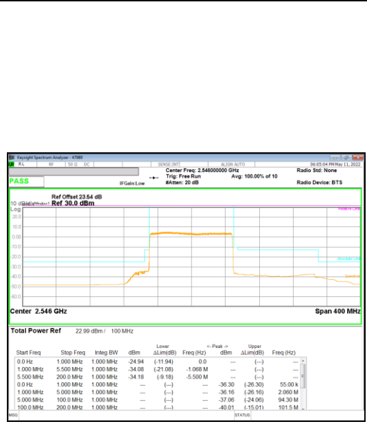
BPSK Low channel FRB
