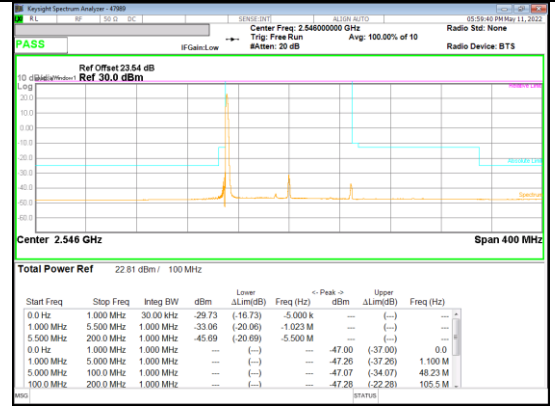
BPSK Low channel 1RB_Offset Low
