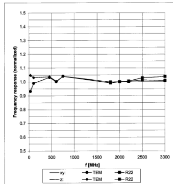
Figure 4-2 E-Field Probe Frequency Response
