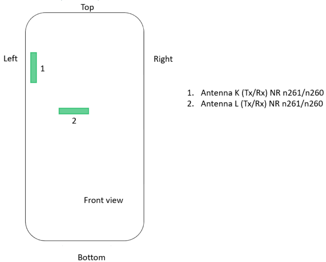
Figure 2: Location of mmW antenna modules looking from front of the DUT - Open
