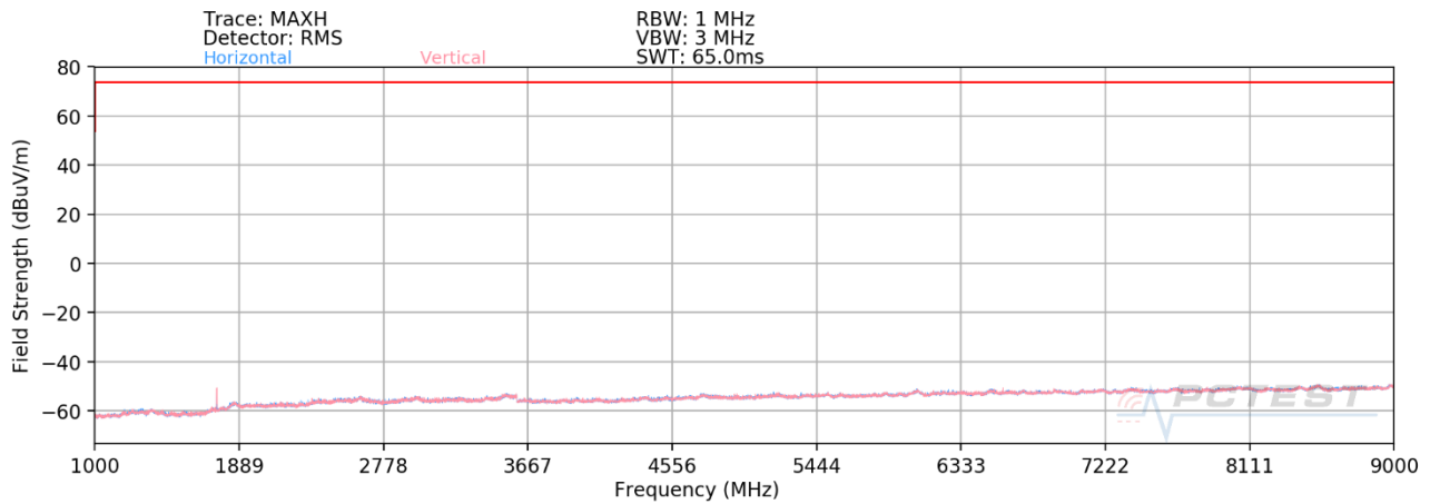
Plot 7-2. Radiated Spurious Plot above 1GHz – Open
