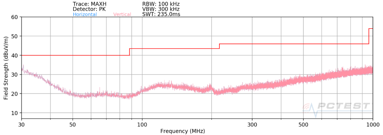
Plot 7-1. Radiated Spurious Plot below 1GHz – Open
