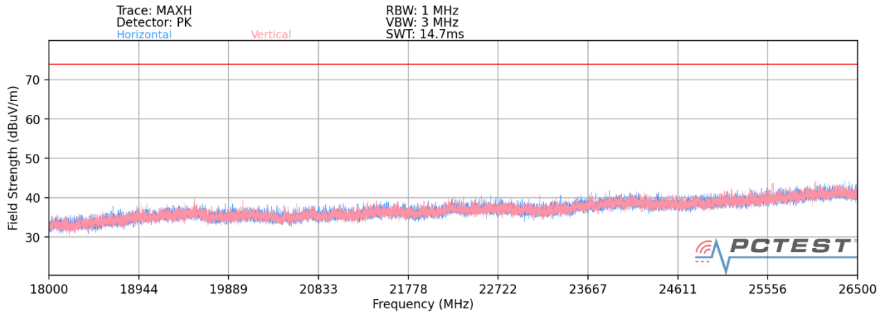
Plot 7-78. Radiated Spurious Plot above 18GHz CDD – CLOSED
