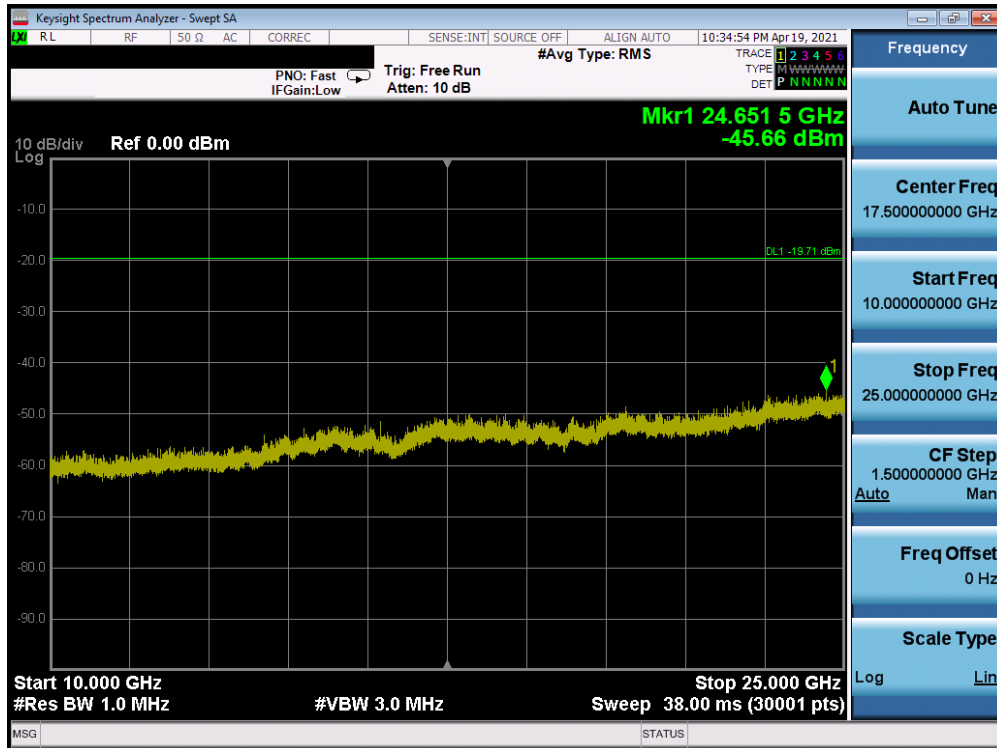
Plot 7-58. Conducted Spurious Plot SISO ANT2 (802.11b – Ch. 1)
