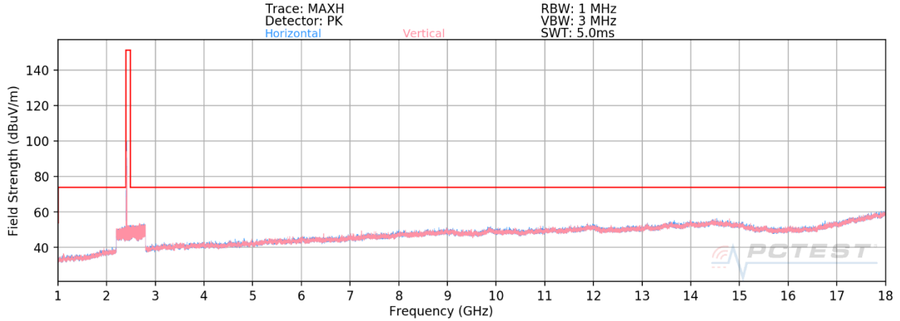
Plot 7-66. Radiated Spurious Plot above 1GHz SISO ANT2 (802.11b – Ch. 1) – CLOSED
