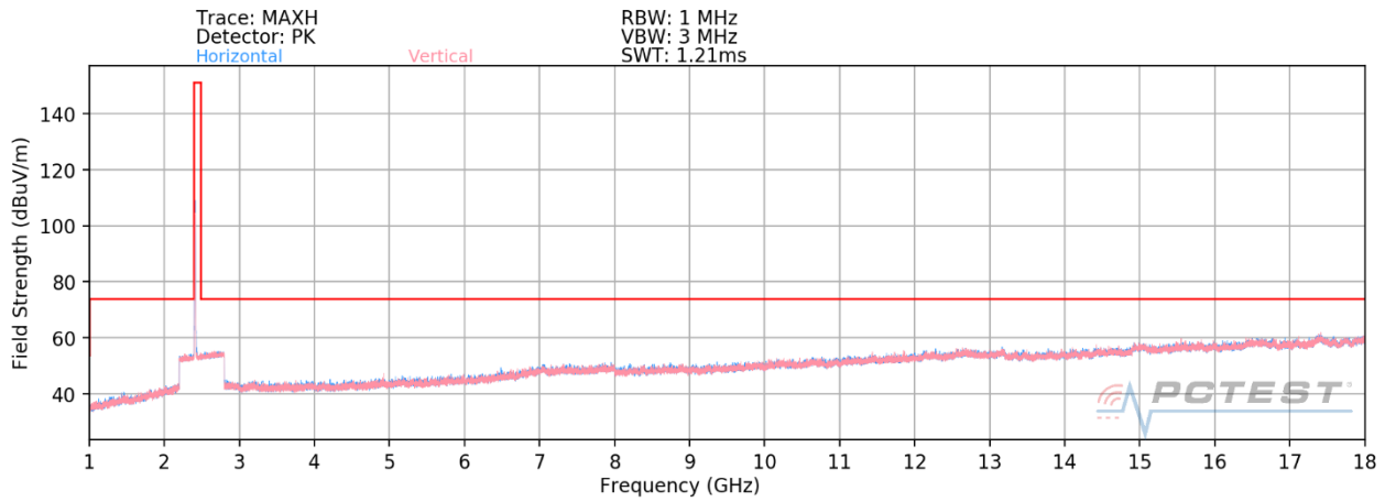
Plot 7-71. Radiated Spurious Plot above 1GHz CDD (802.11b – Ch. 1) – OPEN
