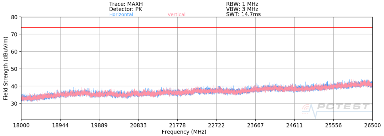
Plot 7-77. Radiated Spurious Plot above 18GHz CDD – OPEN
