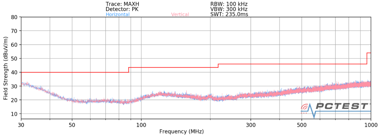
Plot 7-89. Radiated Spurious Plot below 1GHz MIMO – OPEN
