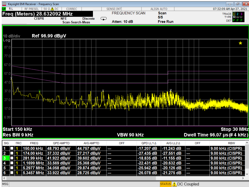
Plot 7-94. Line Conducted Plot with 802.11b (N) – CLOSED
