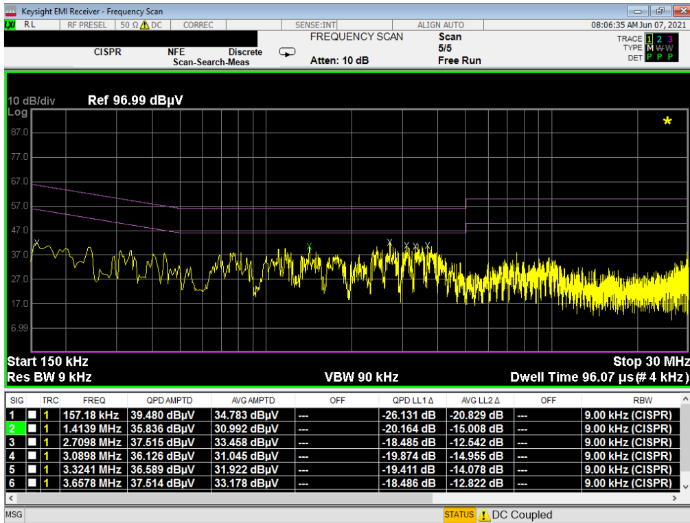
Plot 7-96. Line Conducted Plot with 802.11b (N) with WCP
