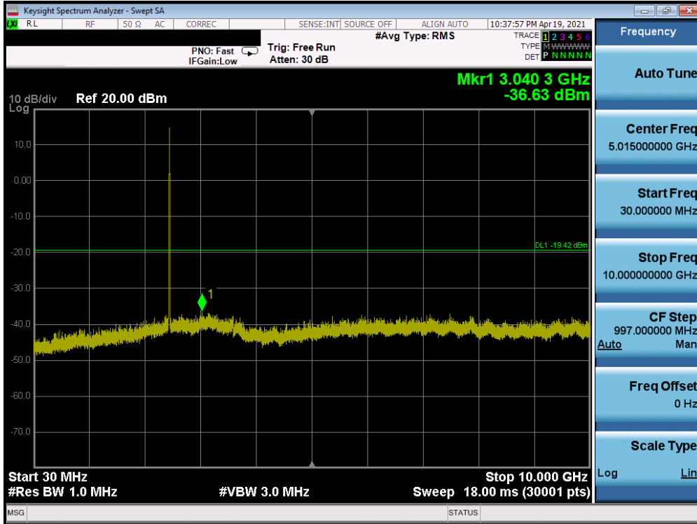
Plot 7-61. Conducted Spurious Plot SISO ANT2 (802.11b – Ch. 11)
