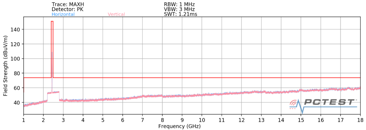
Plot 7-75. Radiated Spurious Plot above 1GHz CDD (802.11b – Ch. 6) – CLOSED
