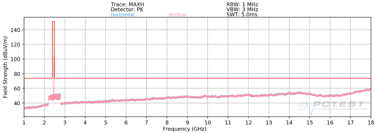
Plot 7-64. Radiated Spurious Plot above 1GHz SISO ANT2 (802.11b – Ch. 6) – OPEN
