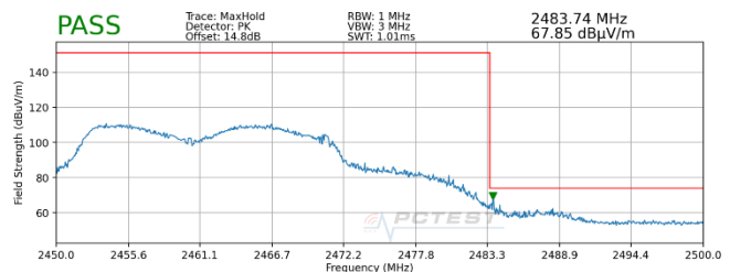
Plot 7-86. Radiated Restricted Upper Band Edge Measurement MIMO (Peak)
