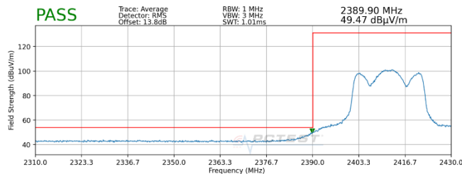
Plot 7-83. Radiated Restricted Lower Band Edge Measurement MIMO (Average)
