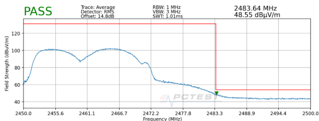
Plot 7-85. Radiated Restricted Upper Band Edge Measurement MIMO (Average)
