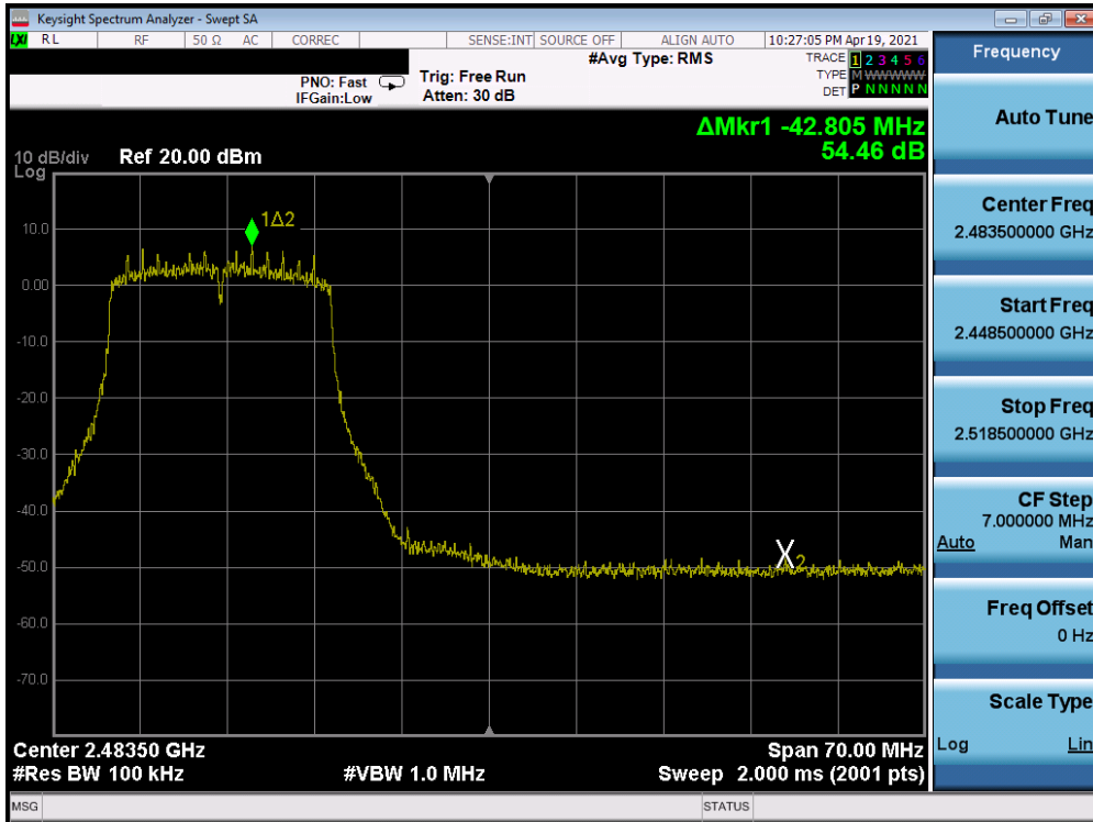
Plot 7-54. Band Edge Plot SISO ANT2 (802.11n (2.4GHz) – Ch. 11)
