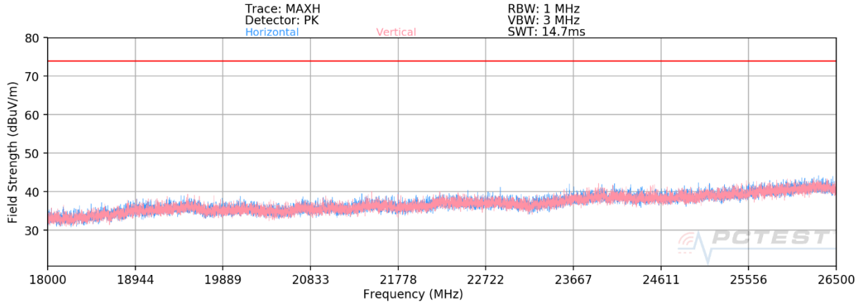
Plot 7-69. Radiated Spurious Plot above 18GHz SISO ANT2 – OPEN
