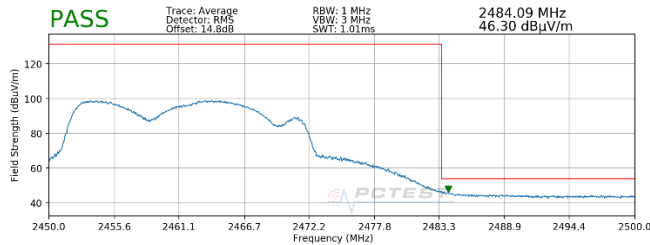
Plot 7-87. Radiated Restricted Band Edge Measurement MIMO with WCP (Average)
