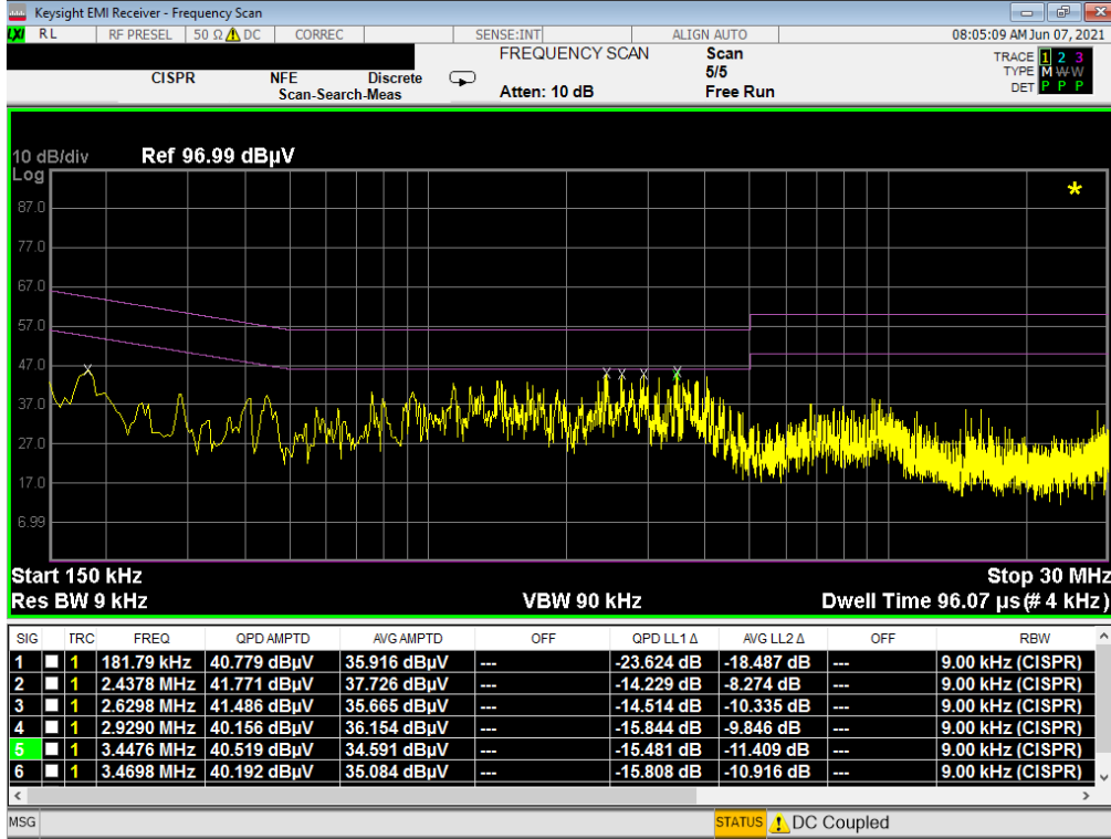
Plot 7-95. Line Conducted Plot with 802.11b (L1) with WCP
