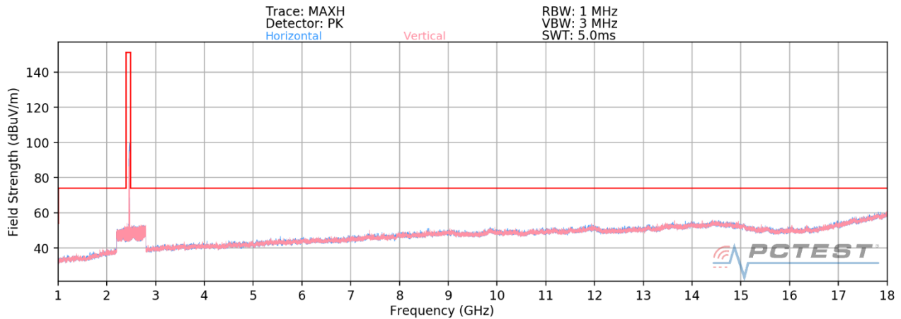
Plot 7-68. Radiated Spurious Plot above 1GHz SISO ANT2 (802.11b – Ch. 11) – CLOSED
