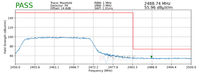
Plot 7-82. Radiated Restricted Upper Band Edge Measurement SISO ANT2 (Peak)
