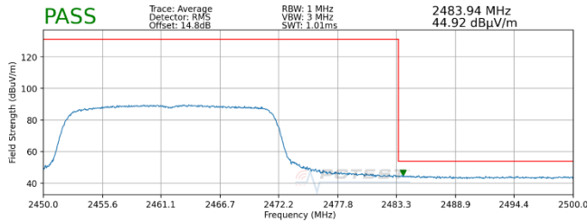
Plot 7-81. Radiated Restricted Upper Band Edge Measurement SISO ANT2 (Average)
