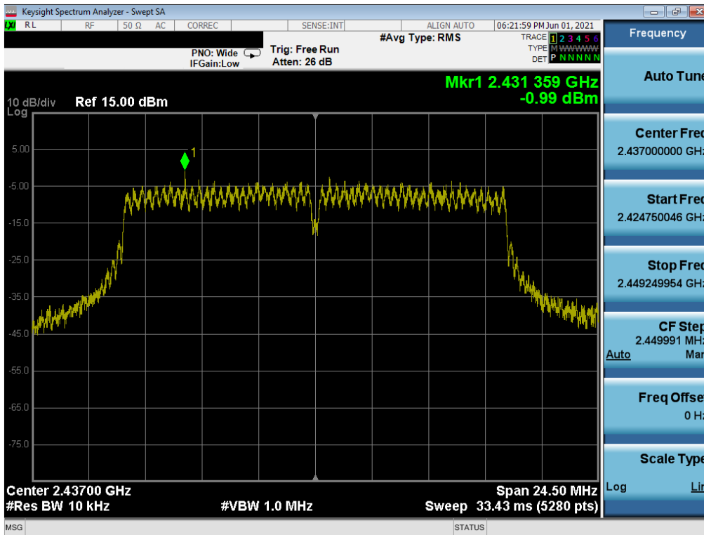
Plot 7-41. Power Spectral Density Plot MIMO ANT2 (802.11g – Ch. 6)
