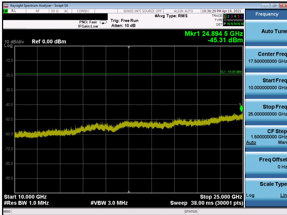
Plot 7-60. Conducted Spurious Plot SISO ANT2 (802.11b – Ch. 6)
