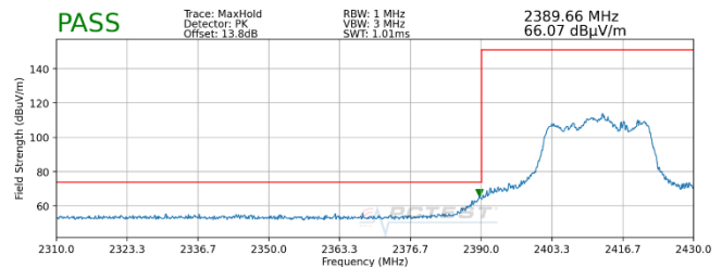
Plot 7-84. Radiated Restricted Lower Band Edge Measurement MIMO (Peak)
