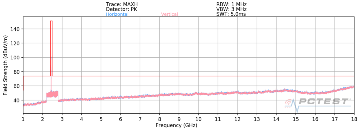
Plot 7-67. Radiated Spurious Plot above 1GHz SISO ANT2 (802.11b – Ch. 6) – CLOSED
