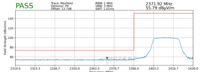
Plot 7-80. Radiated Restricted Lower Band Edge Measurement SISO ANT2 (Peak)
