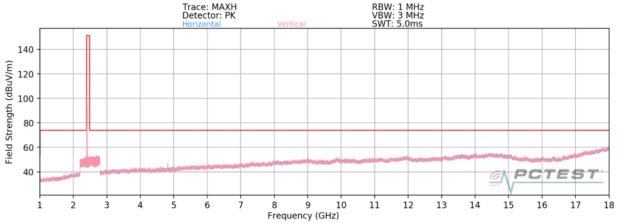
Plot 7-63. Radiated Spurious Plot above 1GHz SISO ANT2 (802.11b – Ch. 1) – OPEN
