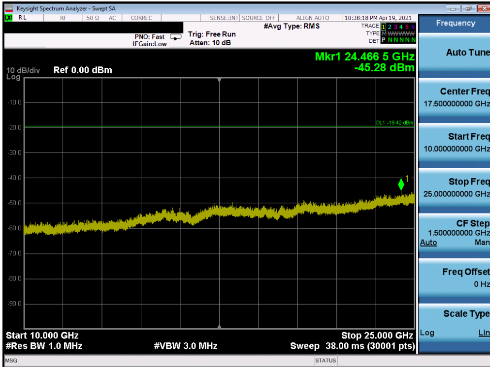
Plot 7-62. Conducted Spurious Plot SISO ANT2 (802.11b – Ch. 11)
