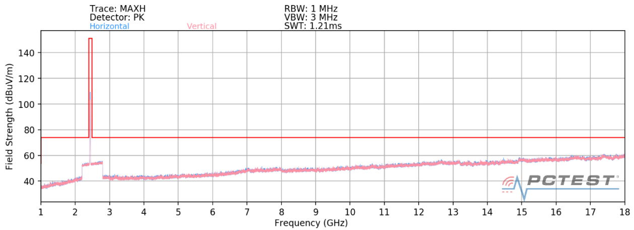
Plot 7-72. Radiated Spurious Plot above 1GHz CDD (802.11b – Ch. 6) – OPEN
