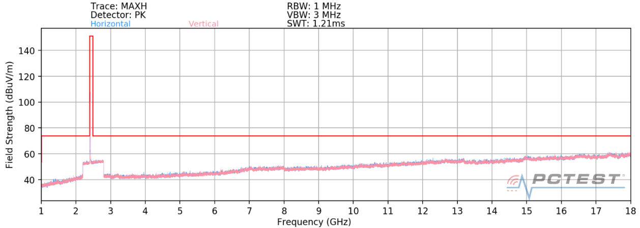
Plot 7-74. Radiated Spurious Plot above 1GHz CDD (802.11b – Ch. 1) – CLOSED
