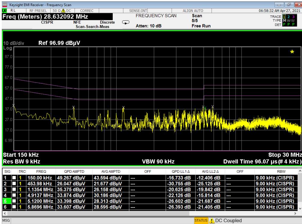
Plot 7-92. Line Conducted Plot with 802.11b (N) – OPEN
