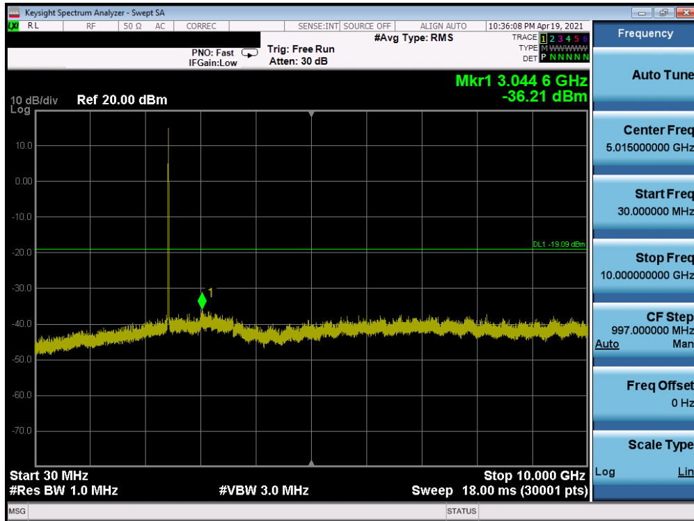
Plot 7-59. Conducted Spurious Plot SISO ANT2 (802.11b – Ch. 6)
