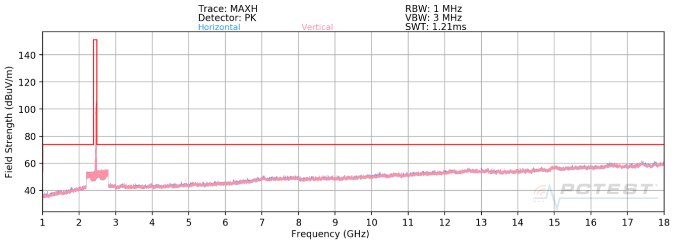
Plot 7-65. Radiated Spurious Plot above 1GHz SISO ANT2 (802.11b – Ch. 11) – OPEN
