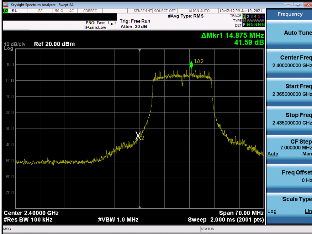
Plot 7-51. Band Edge Plot SISO ANT2 (802.11g- Ch. 1)
