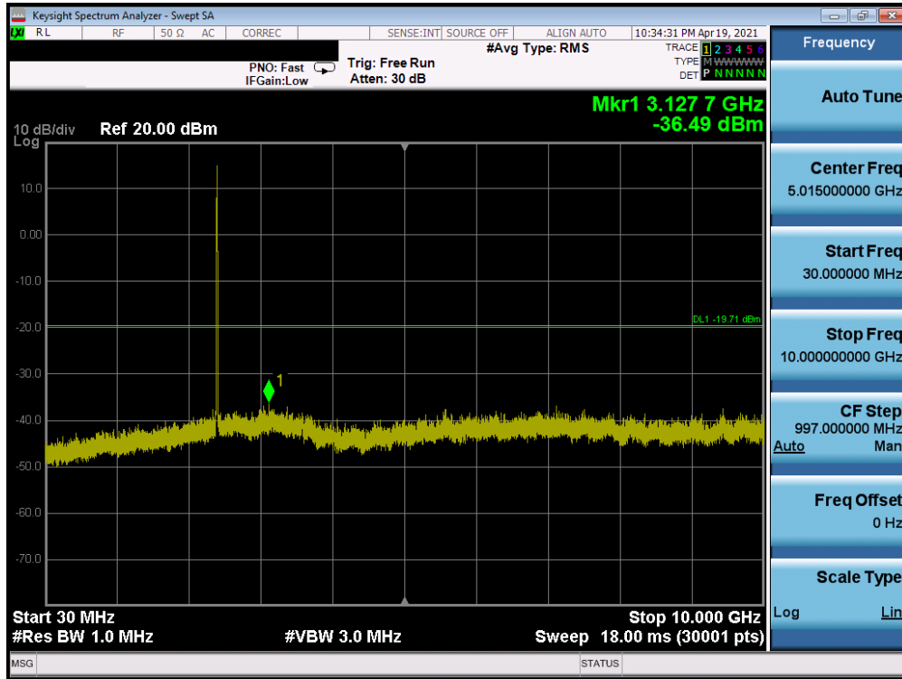
Plot 7-57. Conducted Spurious Plot SISO ANT2 (802.11b – Ch. 1)
