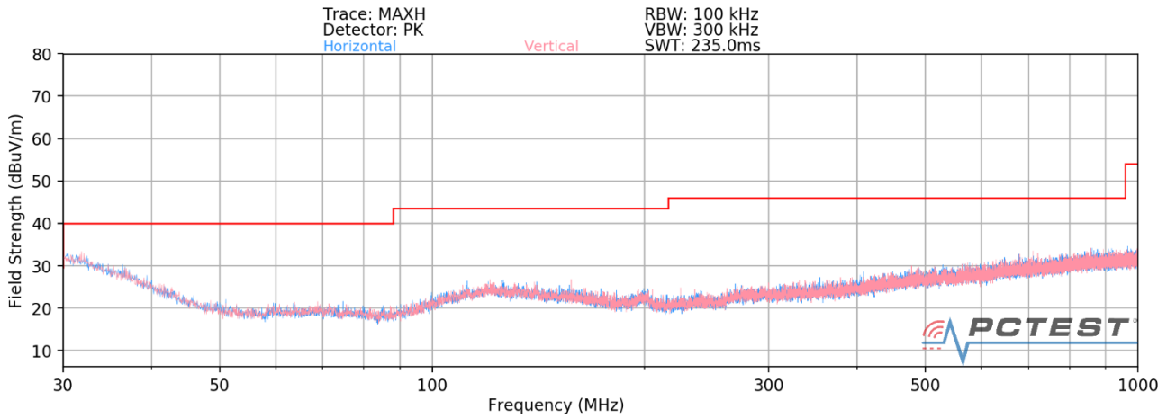
Plot 7-90. Radiated Spurious Plot below 1GHz MIMO – CLOSED
