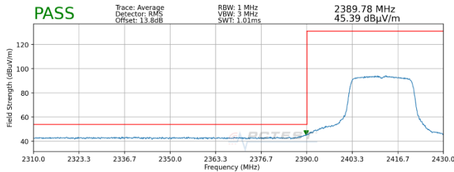
Plot 7-79. Radiated Restricted Lower Band Edge Measurement SISO ANT2 (Average)
