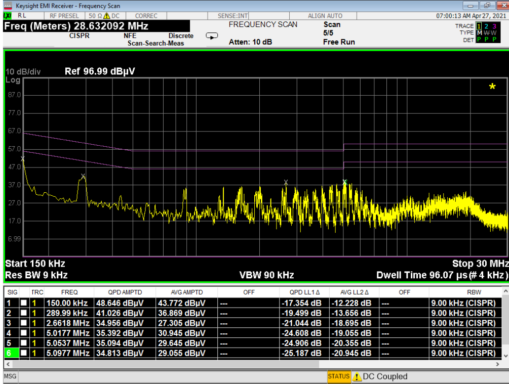
Plot 7-91. Line Conducted Plot with 802.11b (L1) – OPEN
