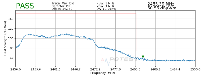
Plot 7-88. Radiated Restricted Band Edge Measurement MIMO with WCP (Peak)
