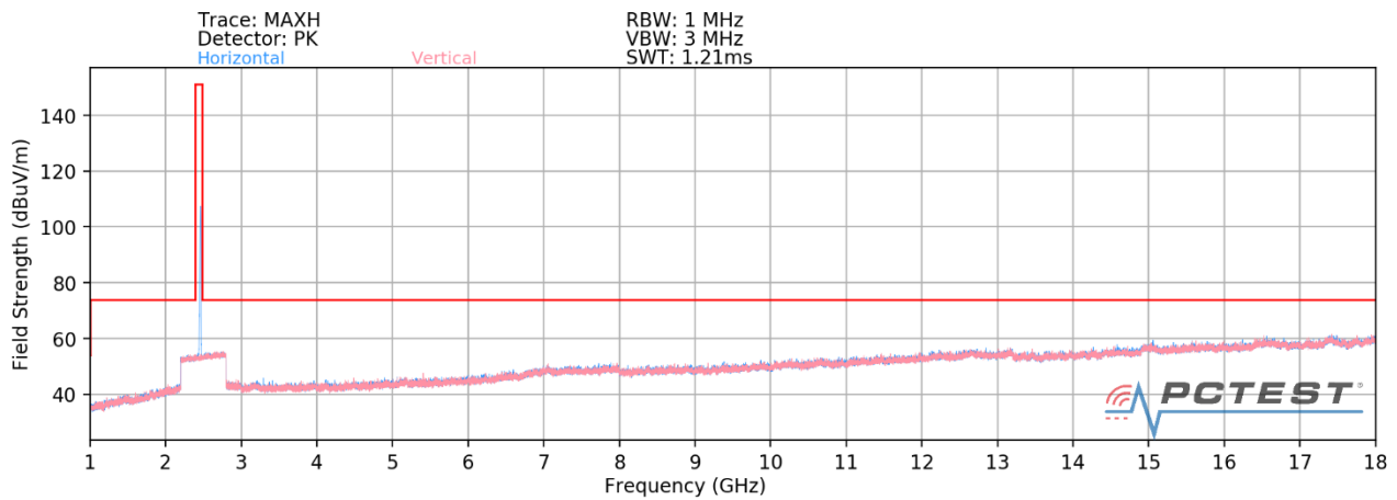
Plot 7-73. Radiated Spurious Plot above 1GHz CDD (802.11b – Ch. 11) – OPEN
