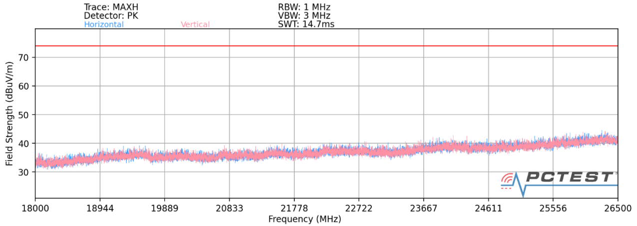
Plot 7-70. Radiated Spurious Plot above 18GHz SISO ANT2- CLOSED
