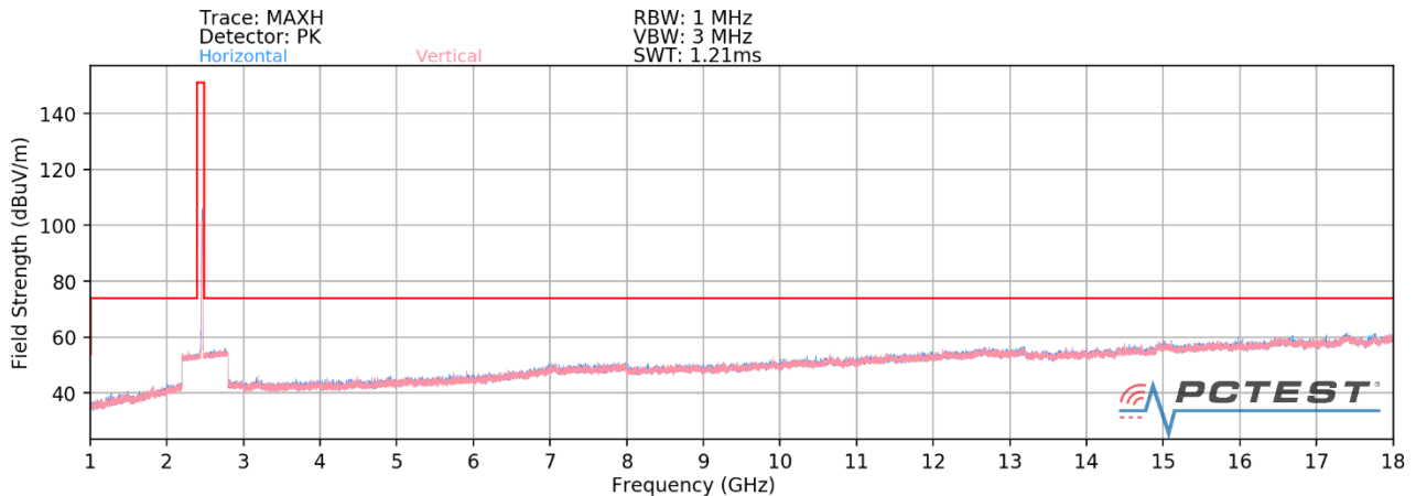
Plot 7-76. Radiated Spurious Plot above 1GHz CDD (802.11b – Ch. 11) – CLOSED
