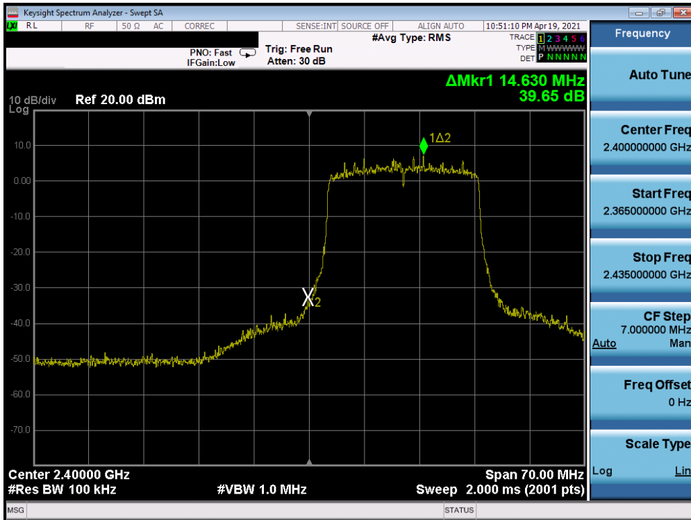
Plot 7-55. Band Edge Plot SISO ANT2 (802.11ax (2.4GHz) – Ch. 1)
