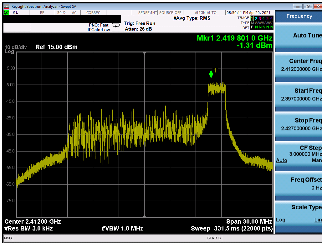
Plot 7-7. Power Spectral Density Plot SISO ANT2 (802.11ax OFDMA – 26 Tones – Ch. 1)
