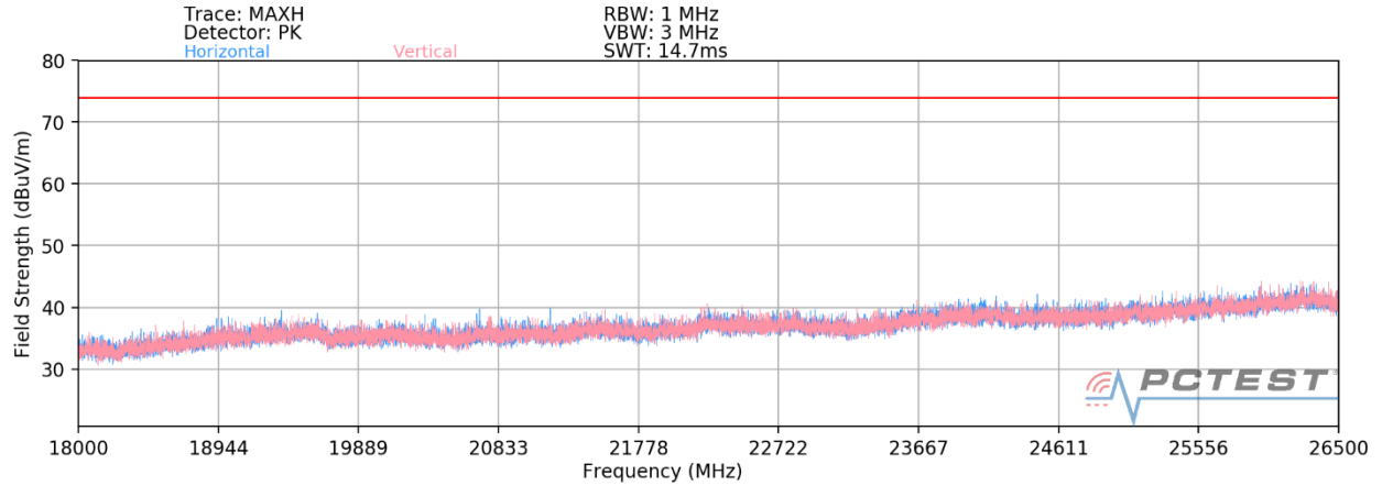
Plot 7-72. Radiated Spurious Plot above 18GHz MIMO (802.11ax OFDMA – 242 Tones) – CLOSED
