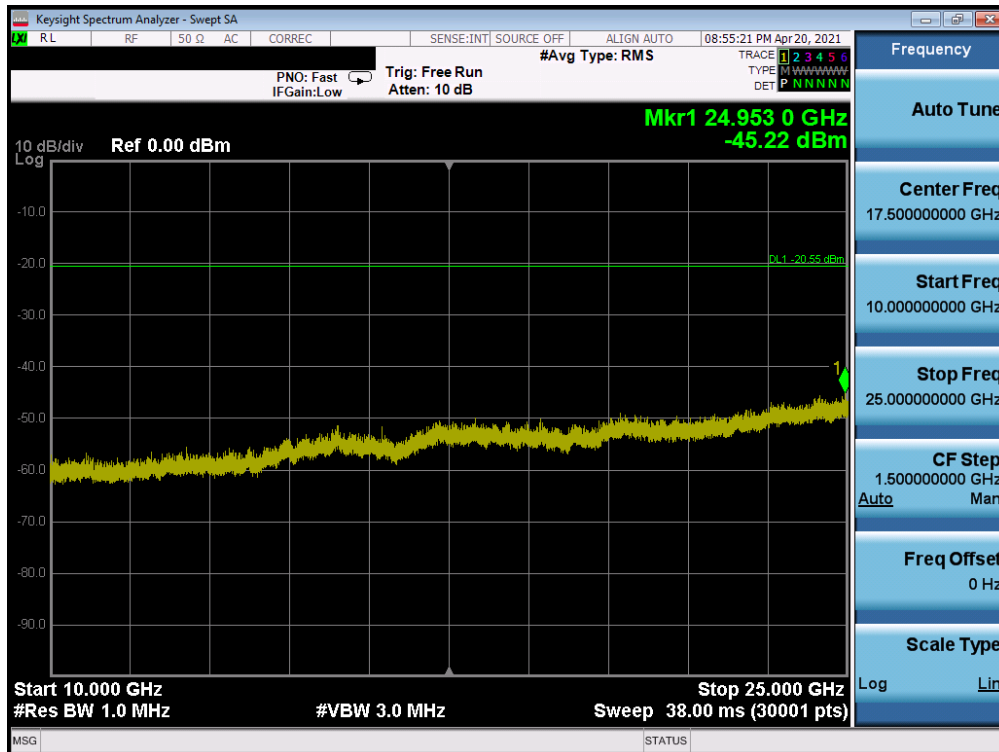
Plot 7-34. Conducted Spurious Plot SISO ANT2 (802.11ax OFDMA – 26 Tones – Ch. 11)
