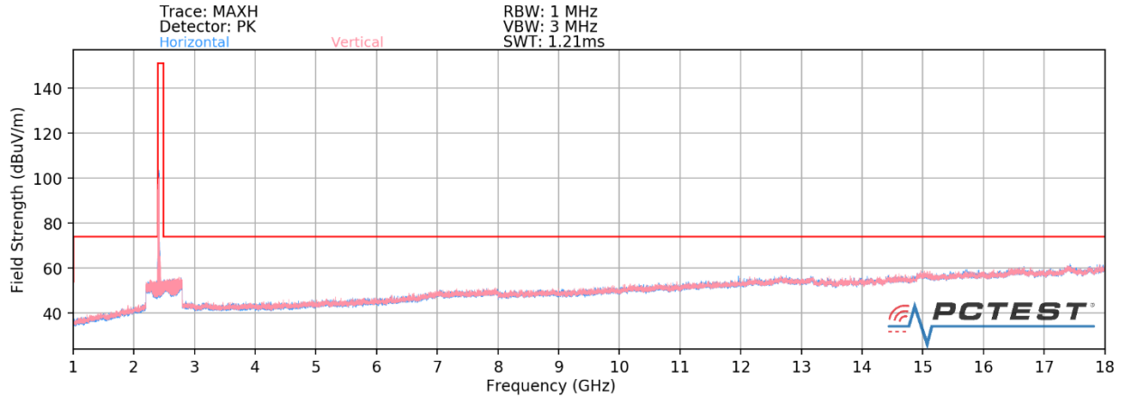
Plot 7-50. Radiated Spurious Plot above 1GHz SISO ANT2 (802.11ax OFDMA – 242 Tones – Ch. 1) – CLOSED
