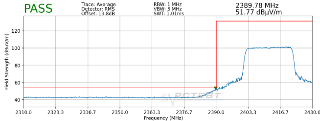
Plot 7-85. Radiated Restricted Lower Band Edge Measurement MIMO (Average – 242 Tones)
