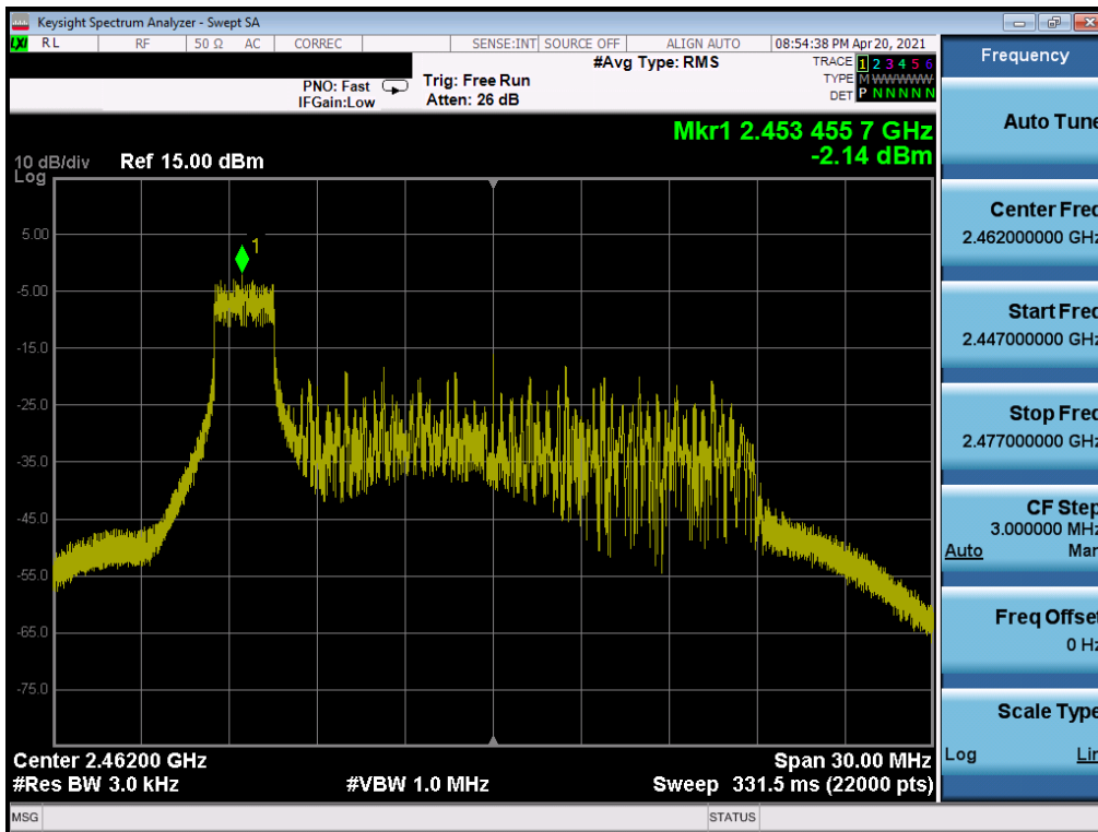
Plot 7-9. Power Spectral Density Plot SISO ANT2 (802.11ax OFDMA – 26 Tones – Ch. 11)
