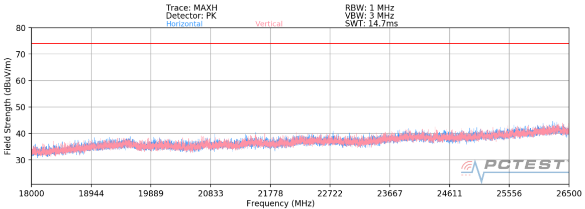
Plot 7-55. Radiated Spurious Plot above 18GHz SISO ANT2 (802.11ax OFDMA – 242 Tones) – OPEN
