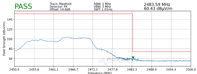
Plot 7-76. Radiated Restricted Upper Band Edge Measurement SISO ANT2 (Peak – 106 Tones)
