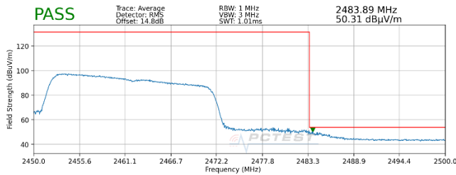
Plot 7-87. Radiated Restricted Upper Band Edge Measurement MIMO (Average – 242 Tones)
