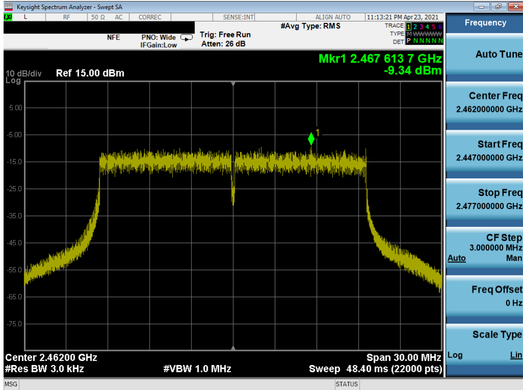
Plot 7-24. Power Spectral Density Plot MIMO ANT2 (802.11ax OFDMA – 242 Tones – Ch. 11) – Q
