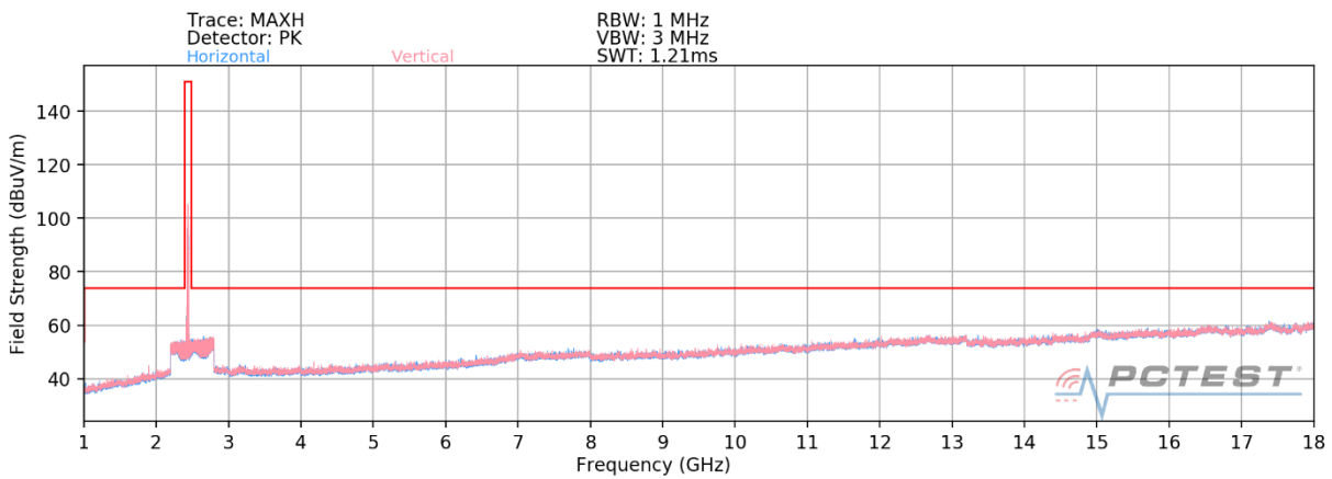
Plot 7-61. Radiated Spurious Plot above 1GHz MIMO (802.11ax OFDMA – 26 Tones – Ch. 6) – CLOSED
