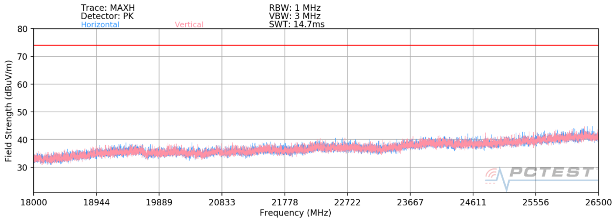
Plot 7-71. Radiated Spurious Plot above 18GHz MIMO (802.11ax OFDMA – 26 Tones) – CLOSED
