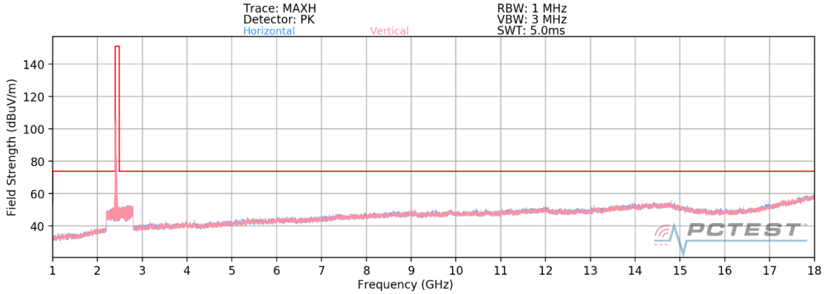
Plot 7-63. Radiated Spurious Plot above 1GHz MIMO (802.11ax OFDMA – 242 Tones – Ch. 1) – OPEN
