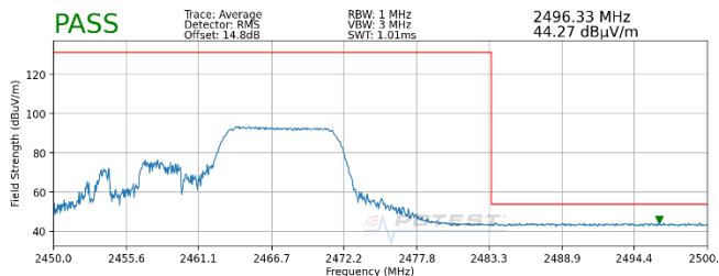
Plot 7-75. Radiated Restricted Upper Band Edge Measurement SISO ANT2 (Average – 106 Tones)
