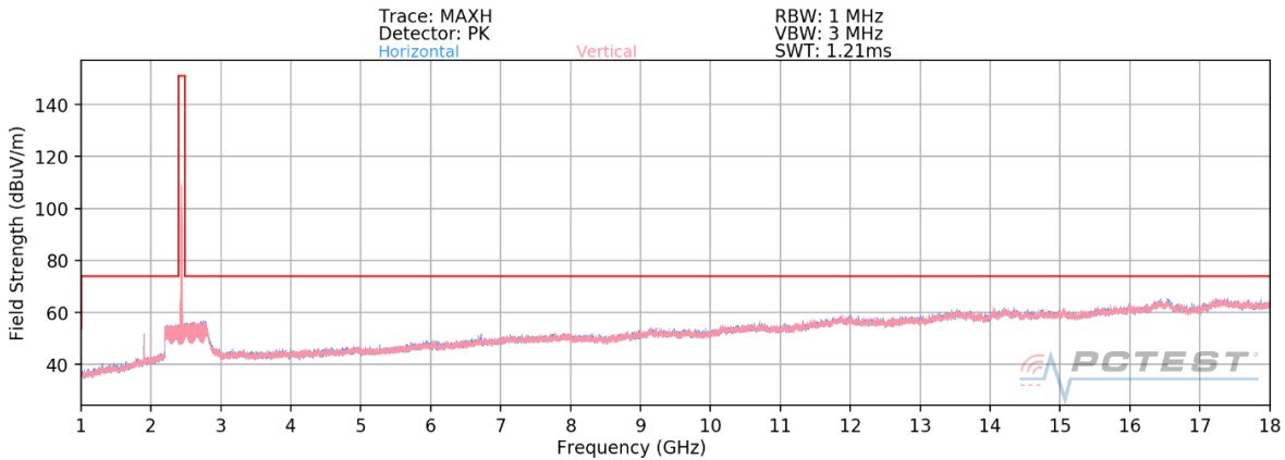
Plot 7-42. Radiated Spurious Plot above 1GHz SISO ANT2 (802.11ax OFDMA – 26 Tones – Ch. 6) – OPEN
