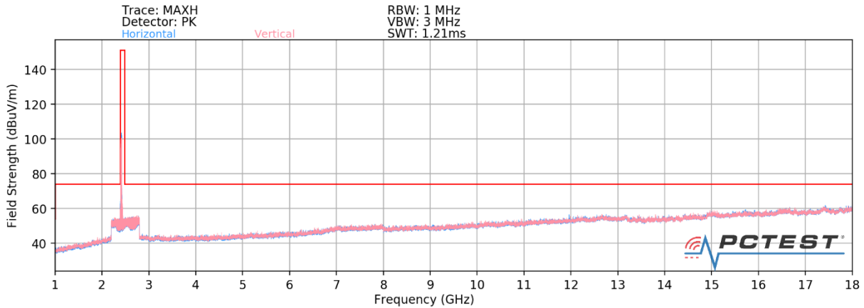
Plot 7-66. Radiated Spurious Plot above 1GHz MIMO (802.11ax OFDMA – 242 Tones – Ch. 1) – CLOSED
