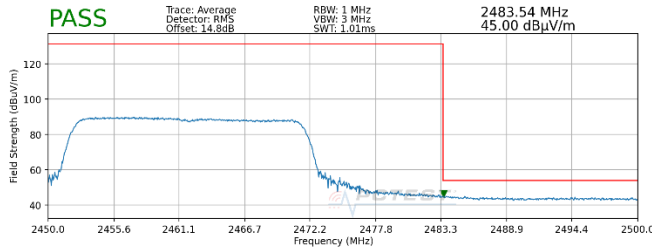
Plot 7-79. Radiated Restricted Upper Band Edge Measurement SISO ANT2 (Average – 242 Tones)
