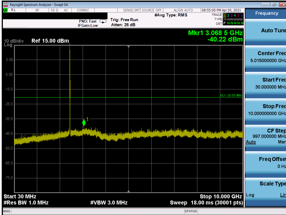
Plot 7-33. Conducted Spurious Plot SISO ANT2 (802.11ax OFDMA – 26 Tones – Ch. 11)
