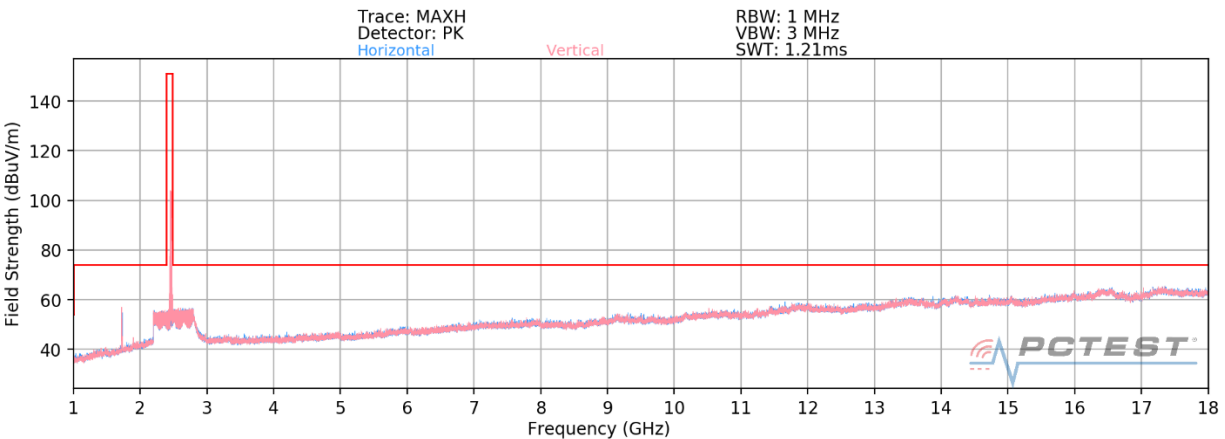
Plot 7-49. Radiated Spurious Plot above 1GHz SISO ANT2 (802.11ax OFDMA – 242 Tones – Ch. 11) – OPEN
