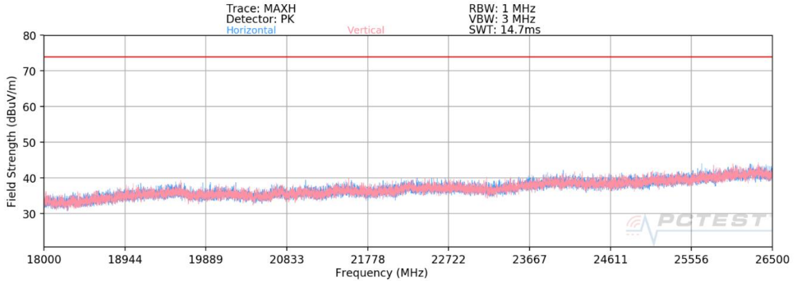
Plot 7-53. Radiated Spurious Plot above 18GHz SISO ANT2 (802.11ax OFDMA – 26 Tones) – OPEN
