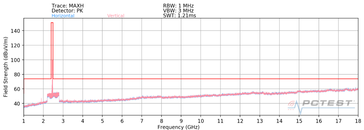
Plot 7-52. Radiated Spurious Plot above 1GHz SISO ANT2 (802.11ax OFDMA – 242 Tones – Ch. 11) – CLOSED
