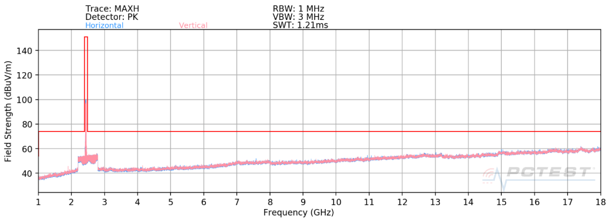
Plot 7-67. Radiated Spurious Plot above 1GHz MIMO (802.11ax OFDMA – 242 Tones – Ch. 6) – CLOSED
