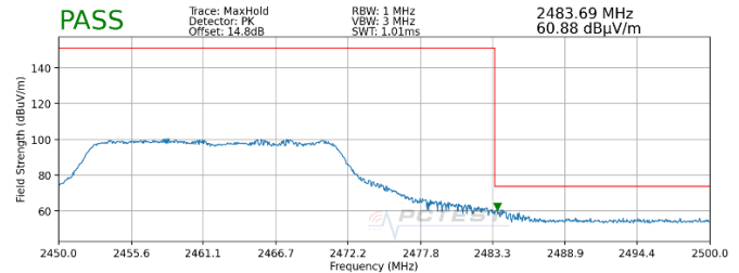
Plot 7-80. Radiated Restricted Upper Band Edge Measurement SISO ANT2 (Peak – 242 Tones)
