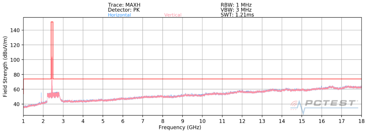
Plot 7-48. Radiated Spurious Plot above 1GHz SISO ANT2 (802.11ax OFDMA – 242 Tones – Ch. 6) – OPEN
