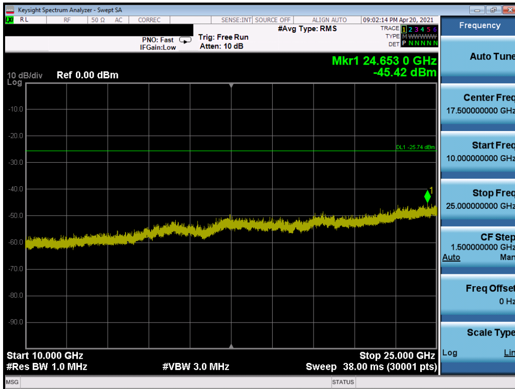
Plot 7-38. Conducted Spurious Plot SISO ANT2 (802.11ax OFDMA – 242 Tones – Ch. 6)
