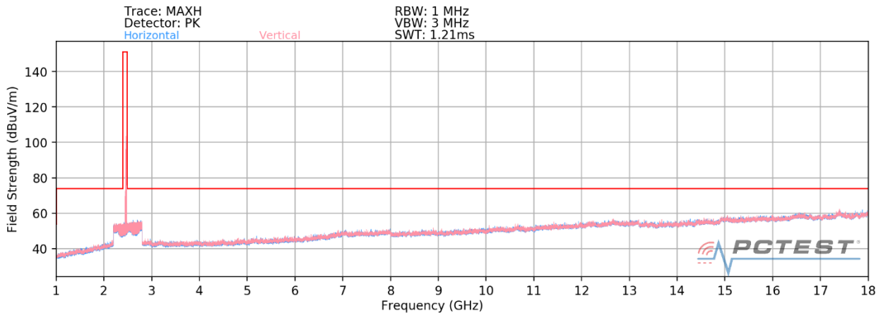
Plot 7-46. Radiated Spurious Plot above 1GHz SISO ANT2 (802.11ax OFDMA – 26 Tones – Ch. 11) – CLOSED
