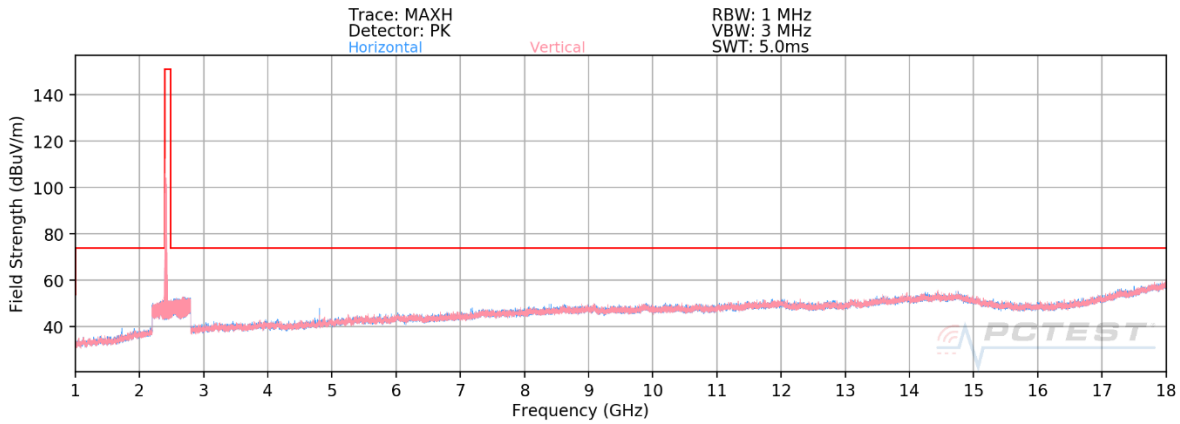
Plot 7-57. Radiated Spurious Plot above 1GHz MIMO (802.11ax OFDMA – 26 Tones – Ch. 1) – OPEN
