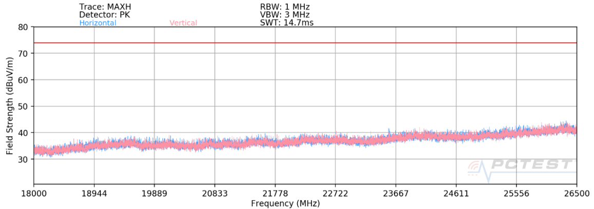
Plot 7-54. Radiated Spurious Plot above 18GHz SISO ANT2 (802.11ax OFDMA – 26 Tones) – CLOSED
