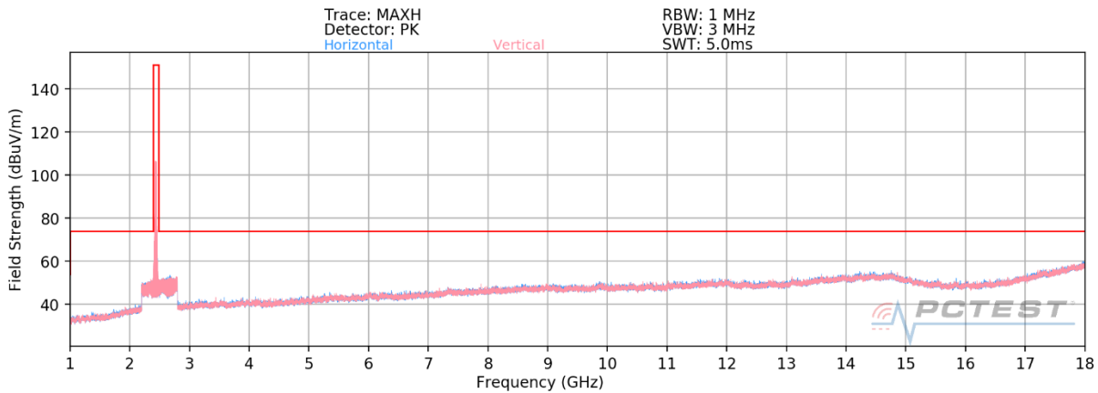
Plot 7-64. Radiated Spurious Plot above 1GHz MIMO (802.11ax OFDMA – 242 Tones – Ch. 6) – OPEN
