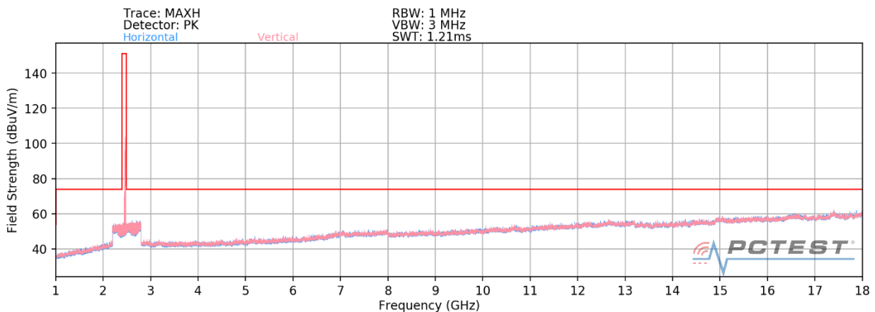
Plot 7-62. Radiated Spurious Plot above 1GHz MIMO (802.11ax OFDMA – 26 Tones – Ch. 11) – CLOSED
