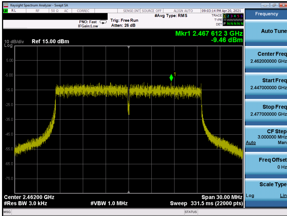
Plot 7-12. Power Spectral Density Plot SISO ANT2 (802.11ax OFDMA – 242 Tones – Ch. 11)
