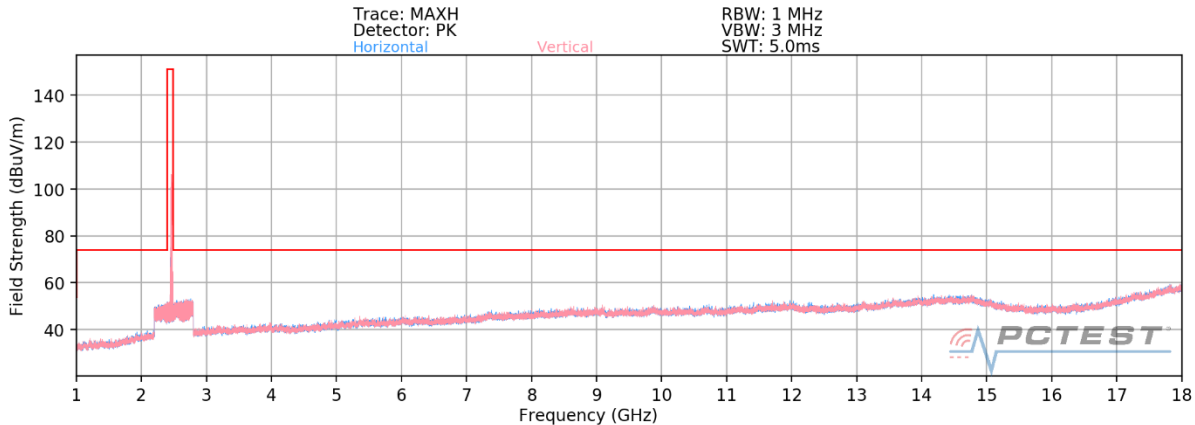
Plot 7-59. Radiated Spurious Plot above 1GHz MIMO (802.11ax OFDMA – 26 Tones – Ch. 11) – OPEN
