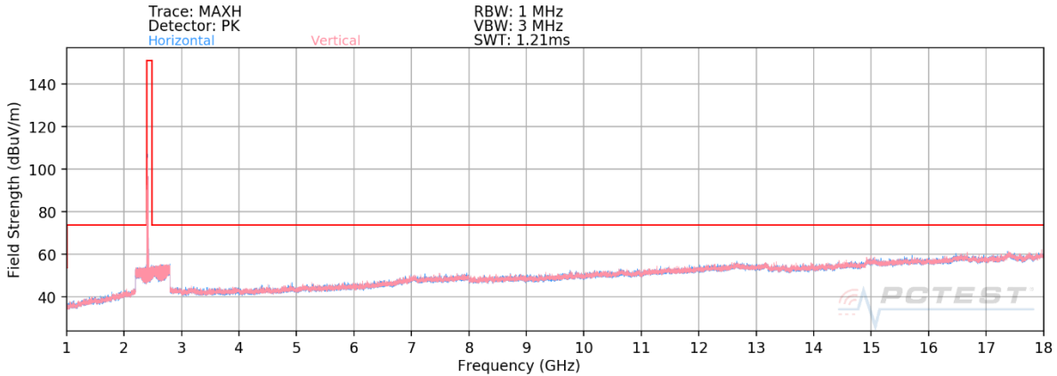
Plot 7-60. Radiated Spurious Plot above 1GHz MIMO (802.11ax OFDMA – 26 Tones – Ch. 1) – CLOSED
