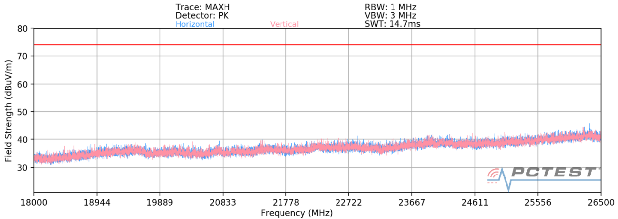
Plot 7-70. Radiated Spurious Plot above 18GHz MIMO (802.11ax OFDMA – 242 Tones) – OPEN
