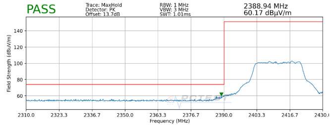
Plot 7-78. Radiated Restricted Lower Band Edge Measurement SISO ANT2 (Peak – 242 Tones)
