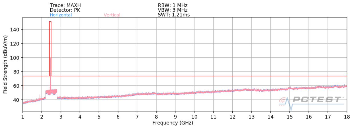
Plot 7-68. Radiated Spurious Plot above 1GHz MIMO (802.11ax OFDMA – 242 Tones – Ch. 11) – CLOSED
