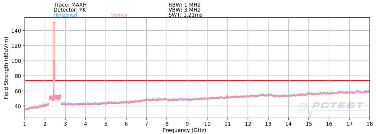
Plot 7-51. Radiated Spurious Plot above 1GHz SISO ANT2 (802.11ax OFDMA – 242 Tones – Ch. 6) – CLOSED
