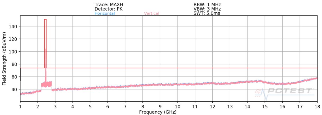
Plot 7-65. Radiated Spurious Plot above 1GHz MIMO (802.11ax OFDMA – 242 Tones – Ch. 11) – OPEN
