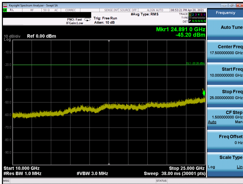
Plot 7-32. Conducted Spurious Plot SISO ANT2 (802.11ax OFDMA – 26 Tones – Ch. 6)
