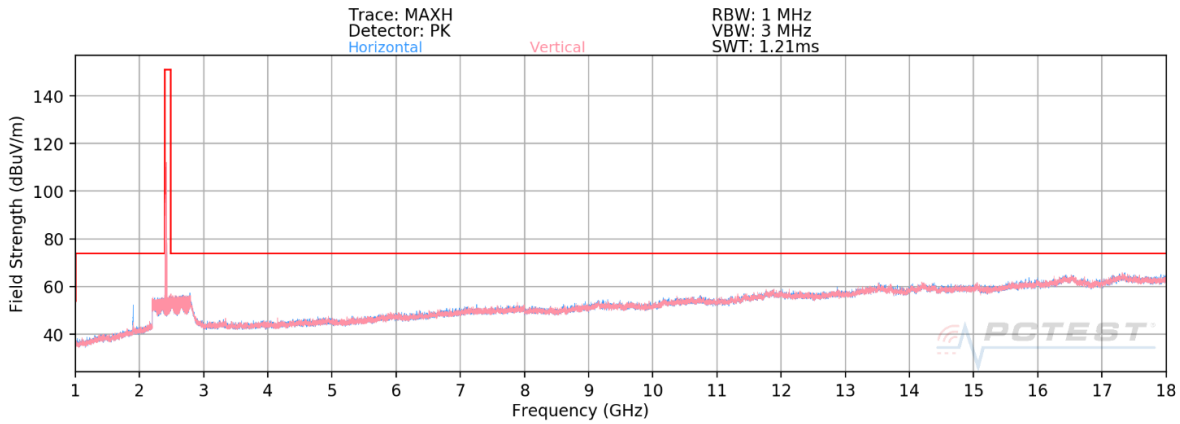
Plot 7-41. Radiated Spurious Plot above 1GHz SISO ANT2 (802.11ax OFDMA – 26 Tones – Ch. 1) – OPEN
