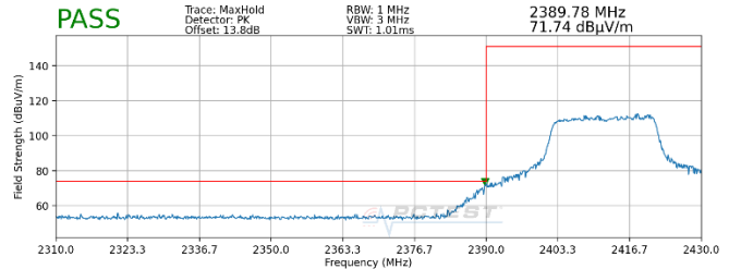
Plot 7-86. Radiated Restricted Lower Band Edge Measurement MIMO (Peak – 242 Tones)
