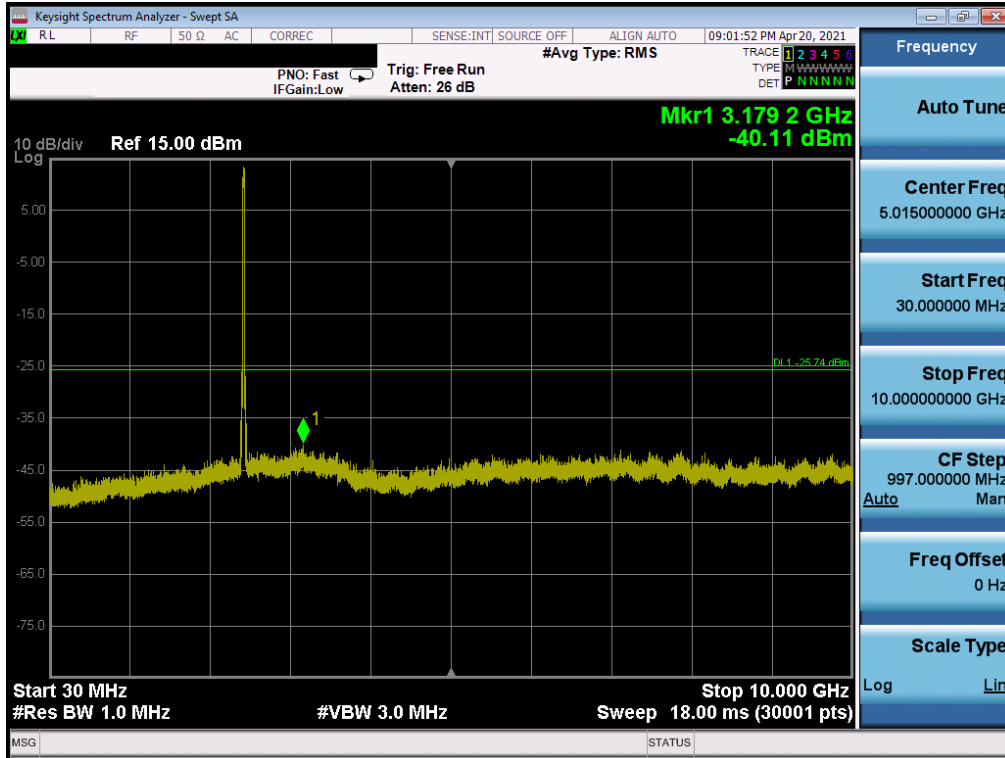
Plot 7-37. Conducted Spurious Plot SISO ANT2 (802.11ax OFDMA – 242 Tones – Ch. 6)
