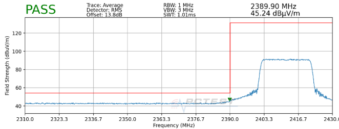
Plot 7-77. Radiated Restricted Lower Band Edge Measurement SISO ANT2 (Average – 242 Tones)
