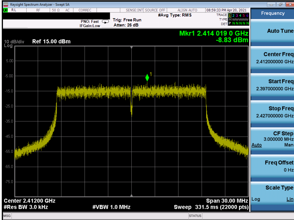
Plot 7-10. Power Spectral Density Plot SISO ANT2 (802.11ax OFDMA – 242 Tones – Ch. 1)
