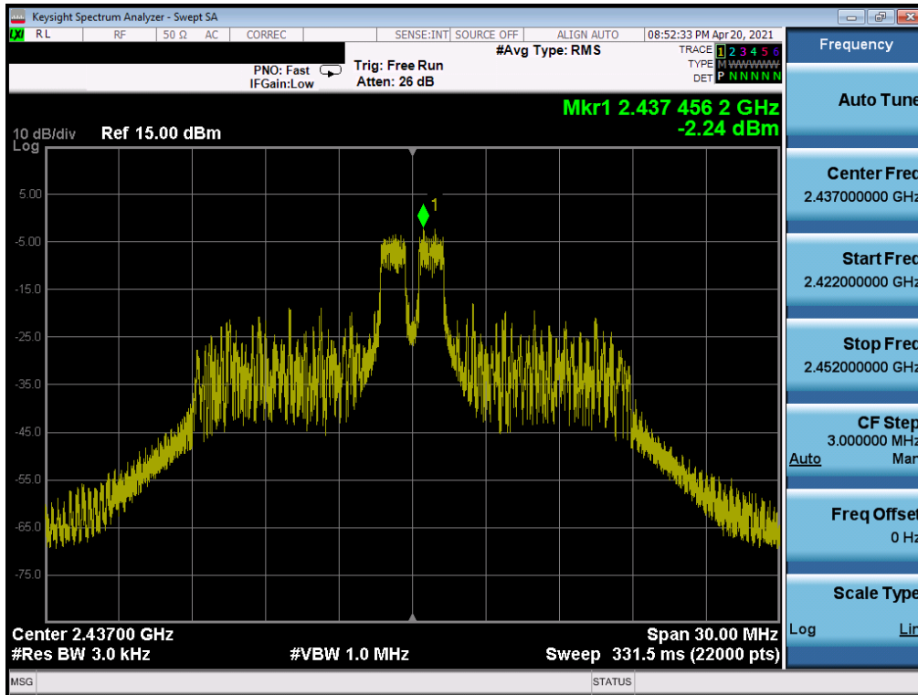
Plot 7-8. Power Spectral Density Plot SISO ANT2 (802.11ax OFDMA – 26 Tones – Ch. 6)
