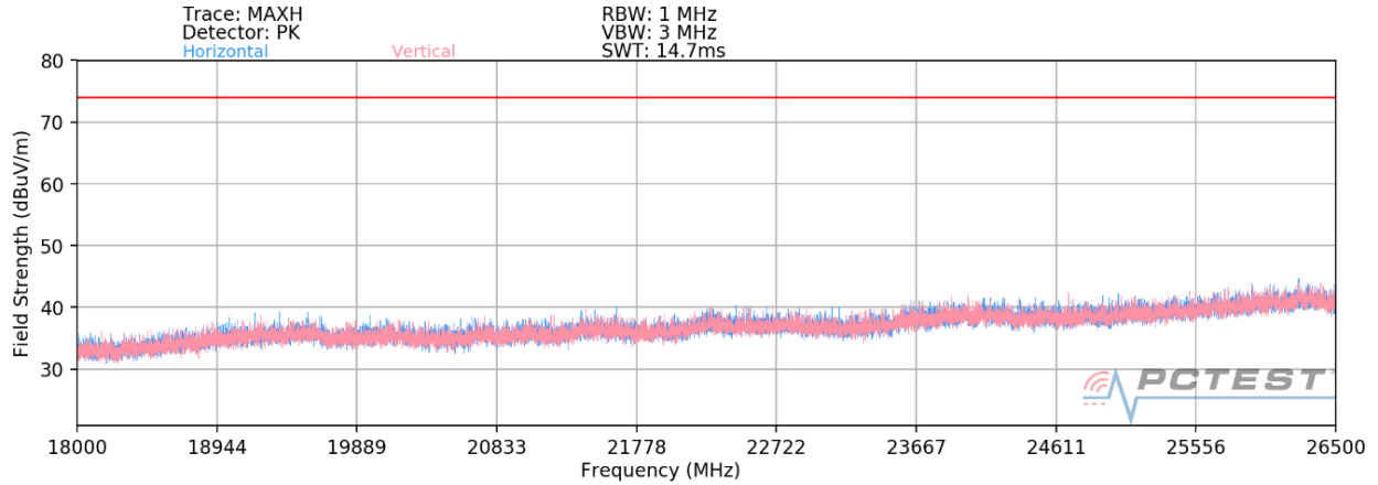
Plot 7-56. Radiated Spurious Plot above 18GHz SISO ANT2 (802.11ax OFDMA – 242 Tones) – CLOSED
