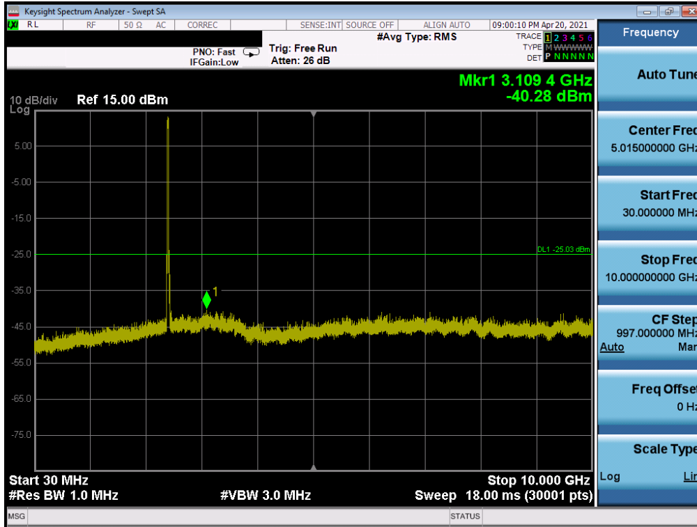
Plot 7-35. Conducted Spurious Plot SISO ANT2 (802.11ax OFDMA – 242 Tones – Ch. 1)
