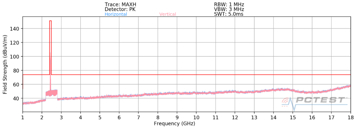
Plot 7-58. Radiated Spurious Plot above 1GHz MIMO (802.11ax OFDMA – 26 Tones – Ch. 6) – OPEN
