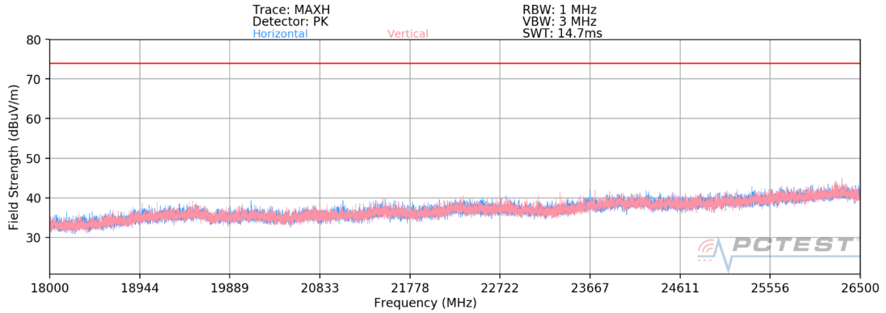
Plot 7-69. Radiated Spurious Plot above 18GHz MIMO (802.11ax OFDMA – 26 Tones) – OPEN
