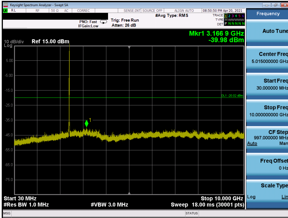
Plot 7-29. Conducted Spurious Plot SISO ANT2 (802.11ax OFDMA – 26 Tones – Ch. 1)
