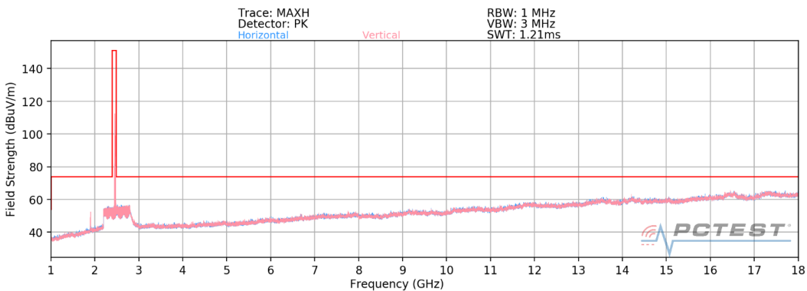
Plot 7-43. Radiated Spurious Plot above 1GHz SISO ANT2 (802.11ax OFDMA – 26 Tones – Ch. 11) – OPEN
