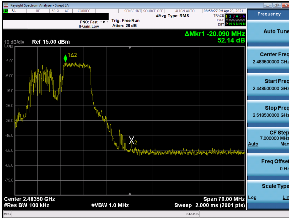
Plot 7-26. Band Edge Plot SISO ANT2 (802.11ax OFDMA – 106 Tones – Ch. 11)
