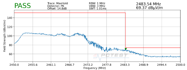
Plot 7-88. Radiated Restricted Upper Band Edge Measurement MIMO (Peak – 242 Tones)
