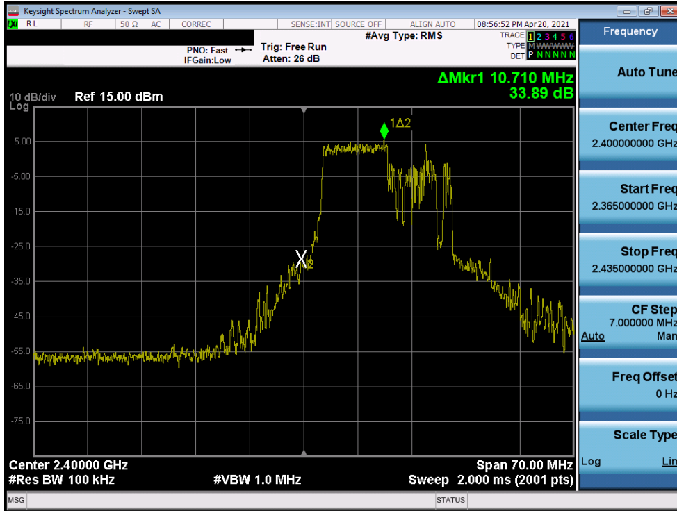
Plot 7-25. Band Edge Plot SISO ANT2 (802.11ax OFDMA – 106 Tones – Ch. 1)
