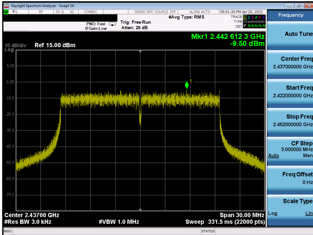
Plot 7-11. Power Spectral Density Plot SISO ANT2 (802.11ax OFDMA – 242 Tones – Ch. 6)
