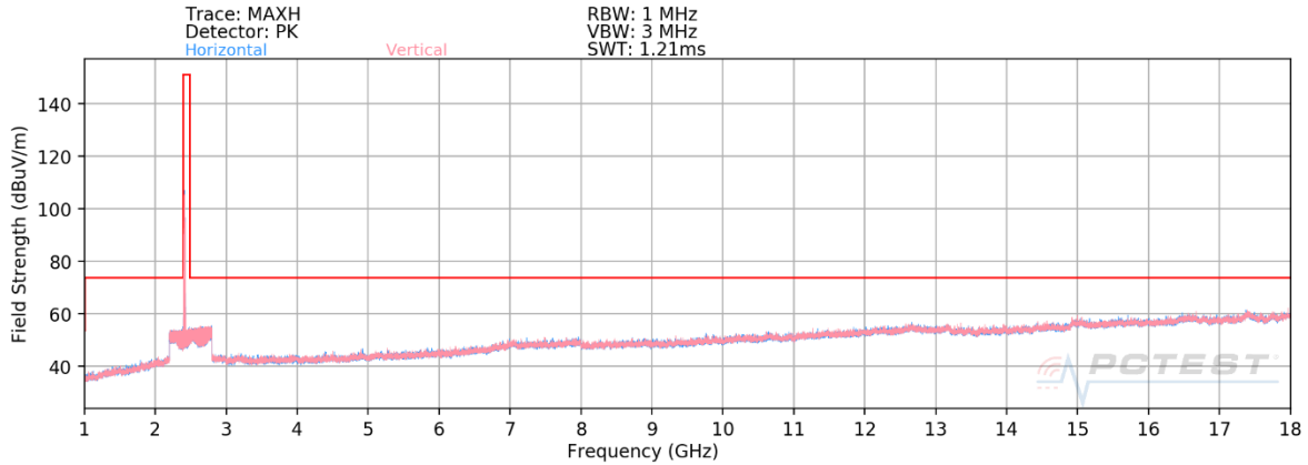
Plot 7-44. Radiated Spurious Plot above 1GHz SISO ANT2 (802.11ax OFDMA – 26 Tones – Ch. 1) – CLOSED
