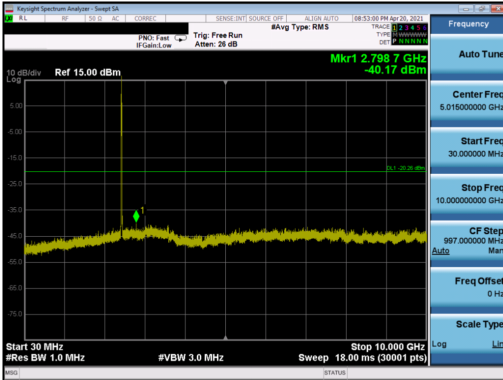
Plot 7-31. Conducted Spurious Plot SISO ANT2 (802.11ax OFDMA – 26 Tones – Ch. 6)
