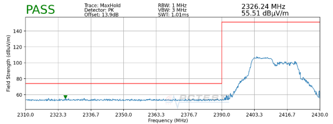
Plot 7-74. Radiated Restricted Lower Band Edge Measurement SISO ANT2 (Peak – 106 Tones)
