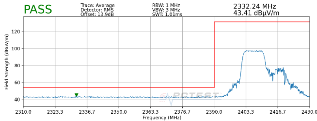
Plot 7-73. Radiated Restricted Lower Band Edge Measurement SISO ANT2 (Average – 106 Tones)
