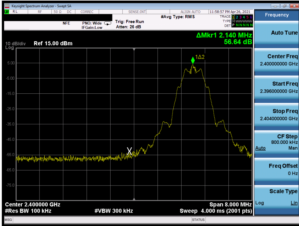
Plot 7-81. Band Edge Plot (Bluetooth (LE), 125kbps – Ch. 0)
