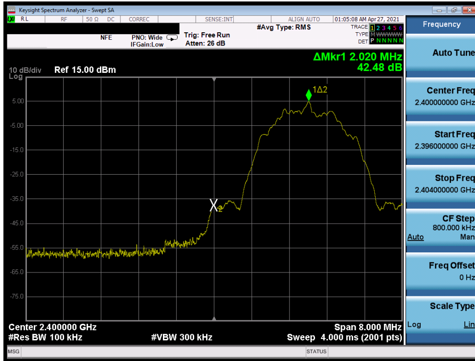
Plot 7-87. Band Edge Plot (Bluetooth (LE), 2Mbps – Ch. 0)
