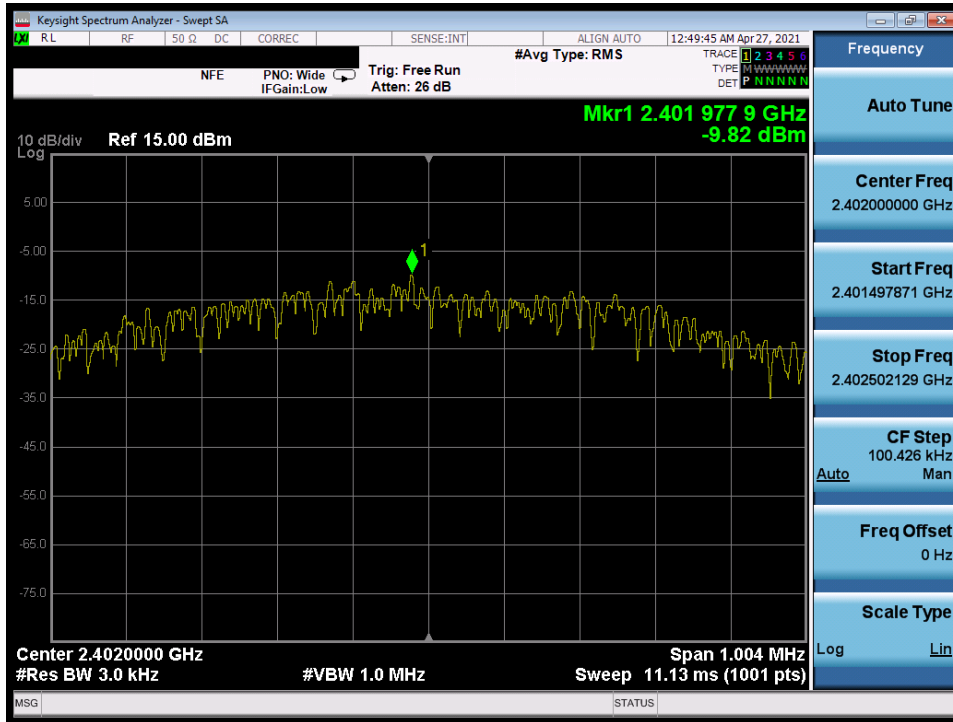
Plot 7-67. Power Spectral Density Plot (Bluetooth (LE), 1Mbps – Ch. 0)
