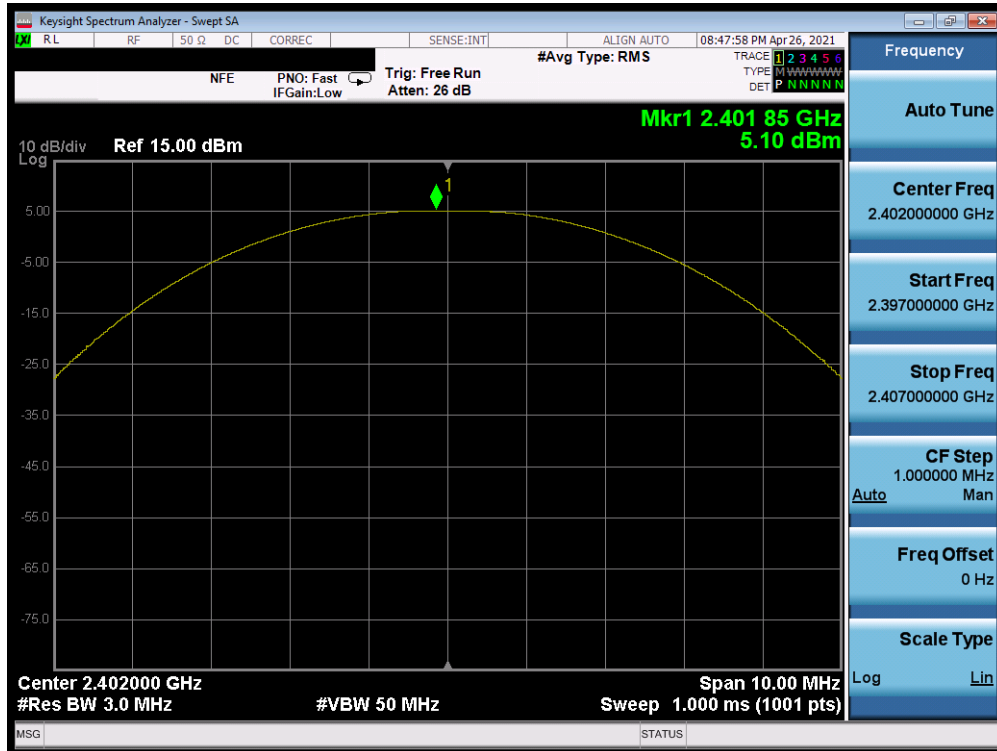
Plot 7-40. Peak Power Plot (Bluetooth (LE), 500kbps – Ch. 0)
