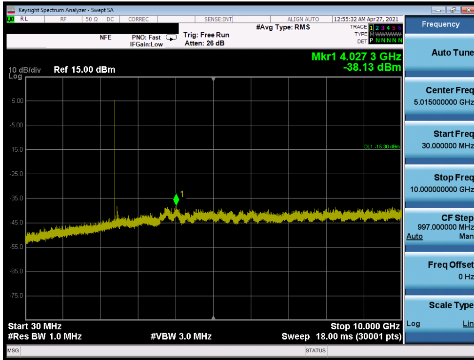
Plot 7-95. Conducted Spurious Plot (Bluetooth (LE), 1Mbps – Ch. 0)
