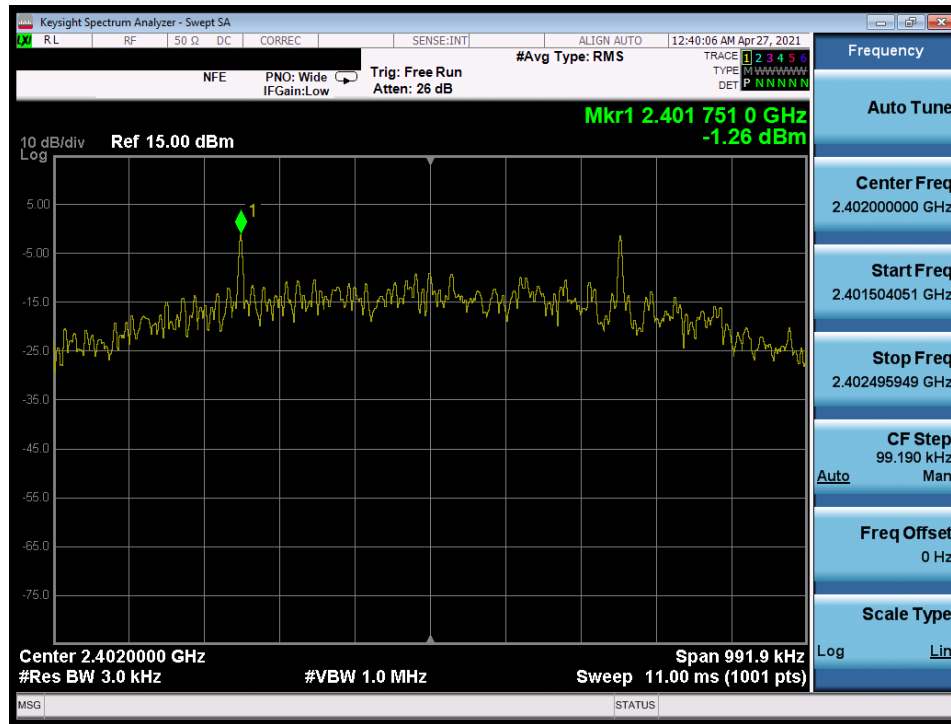
Plot 7-64. Power Spectral Density Plot (Bluetooth (LE), 500kbps – Ch. 0)
