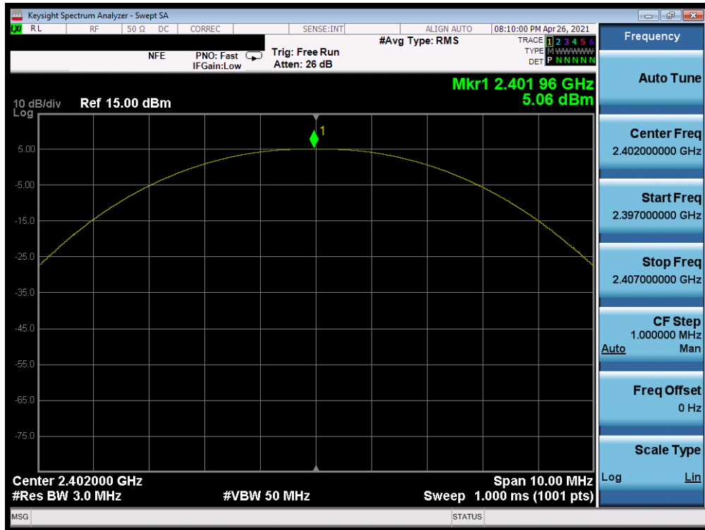
Plot 7-37. Peak Power Plot (Bluetooth (LE), 125kbps – Ch. 0)
