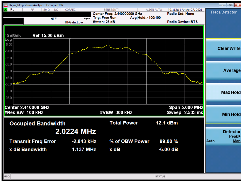
Plot 7-23. 6dB Bandwidth Plot (Bluetooth (LE), 2Mbps – Ch. 19)
