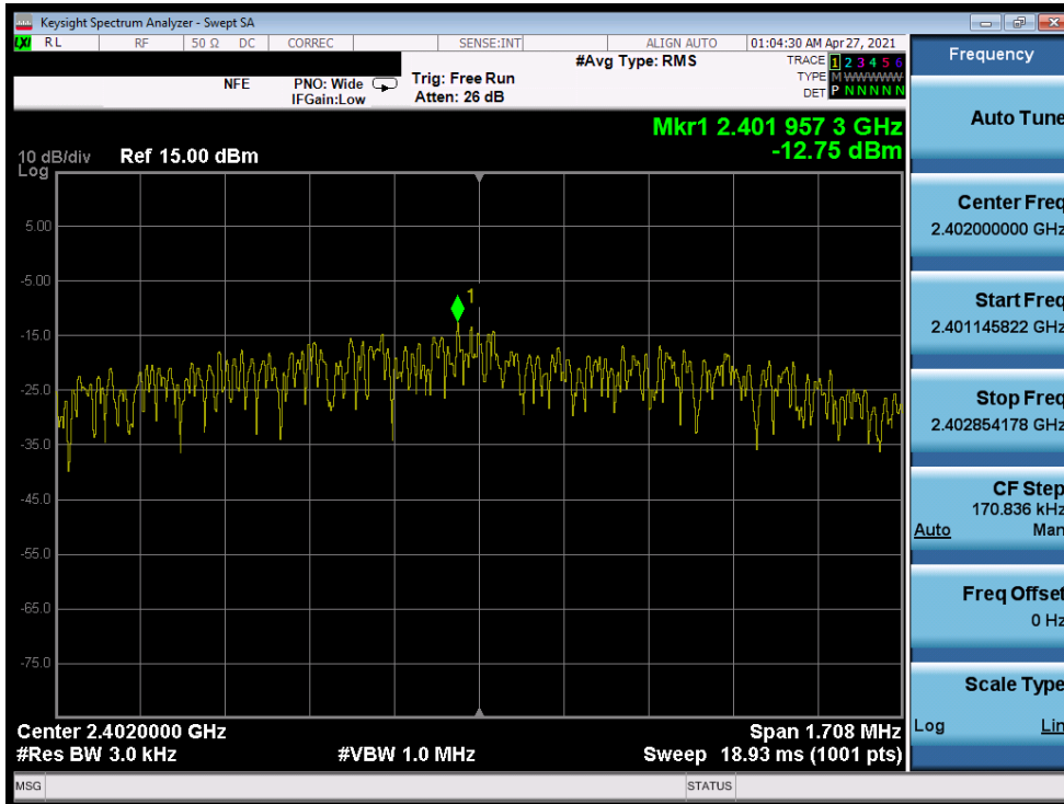
Plot 7-70. Power Spectral Density Plot (Bluetooth (LE), 2Mbps – Ch. 0)
