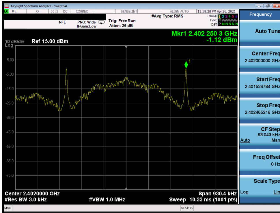
Plot 7-61. Power Spectral Density Plot (Bluetooth (LE), 125kbps – Ch. 0)
