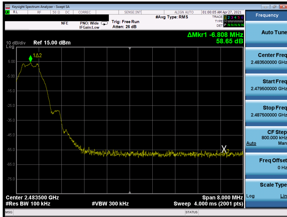
Plot 7-86. Band Edge Plot (Bluetooth (LE), 1Mbps – Ch. 39)
