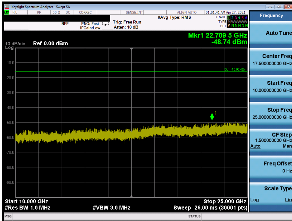
Plot 7-100. Conducted Spurious Plot (Bluetooth (LE), 1Mbps – Ch. 39)
