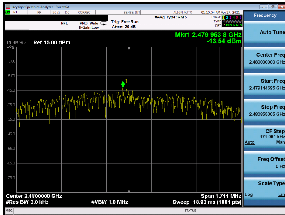
Plot 7-72. Power Spectral Density Plot (Bluetooth (LE), 2Mbps – Ch. 39)
