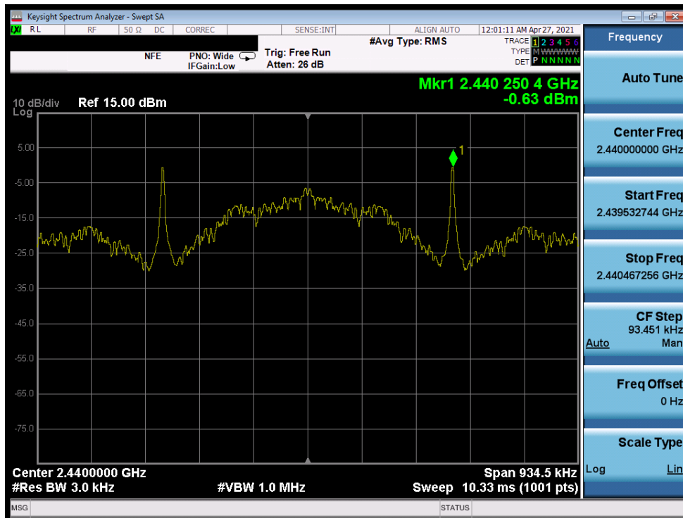
Plot 7-62. Power Spectral Density Plot (Bluetooth (LE), 125kbps – Ch. 19)
