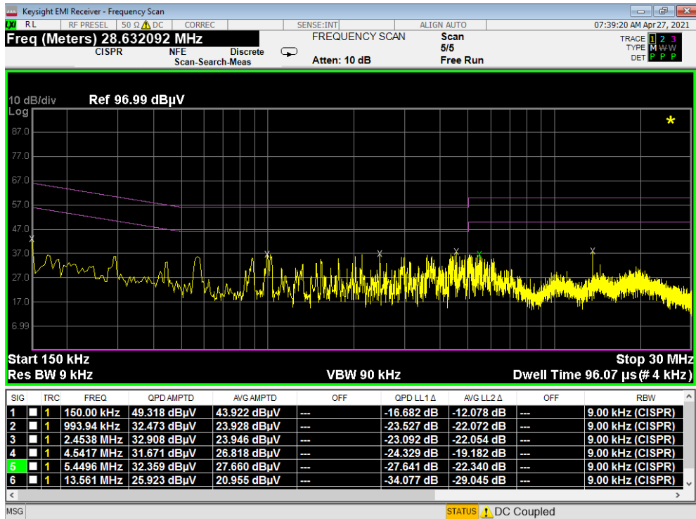
Plot 7-108. Line Conducted Plot with Bluetooth LE (N) - OPEN
