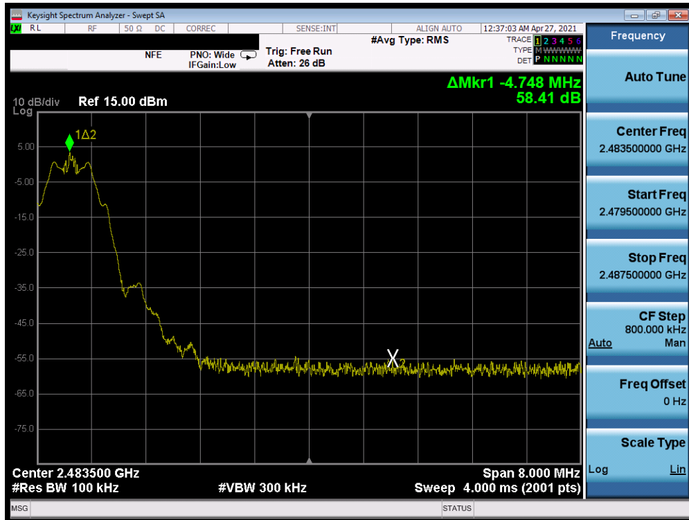
Plot 7-82. Band Edge Plot (Bluetooth (LE), 125kbps – Ch. 39)
