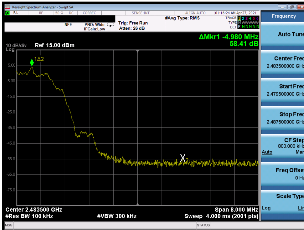
Plot 7-88. Band Edge Plot (Bluetooth (LE), 2Mbps – Ch. 39)
