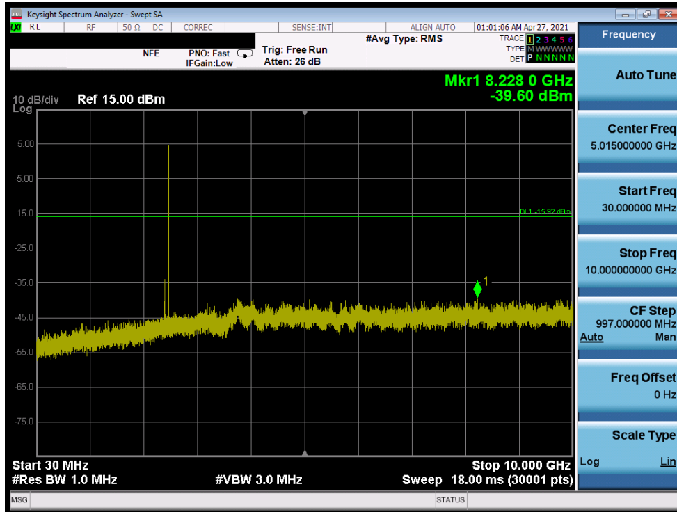
Plot 7-99. Conducted Spurious Plot (Bluetooth (LE), 1Mbps – Ch. 39)
