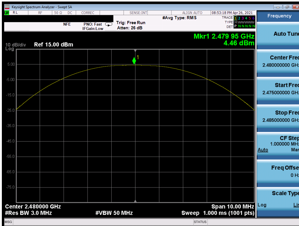
Plot 7-48. Peak Power Plot (Bluetooth (LE), 2Mbps – Ch. 39)
