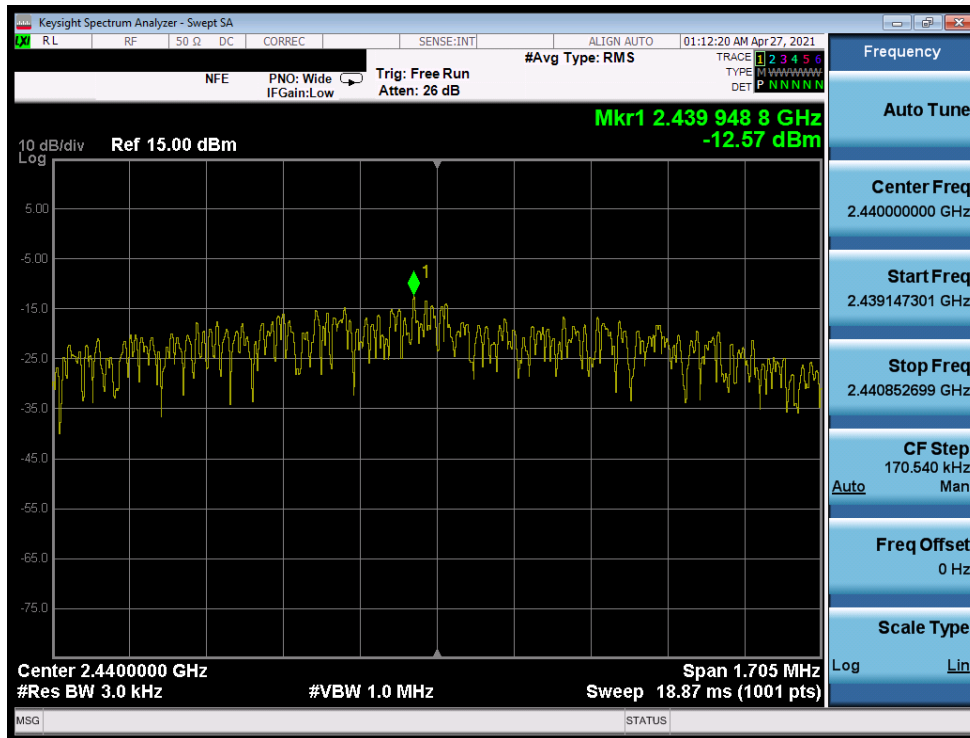
Plot 7-71. Power Spectral Density Plot (Bluetooth (LE), 2Mbps – Ch. 19)
