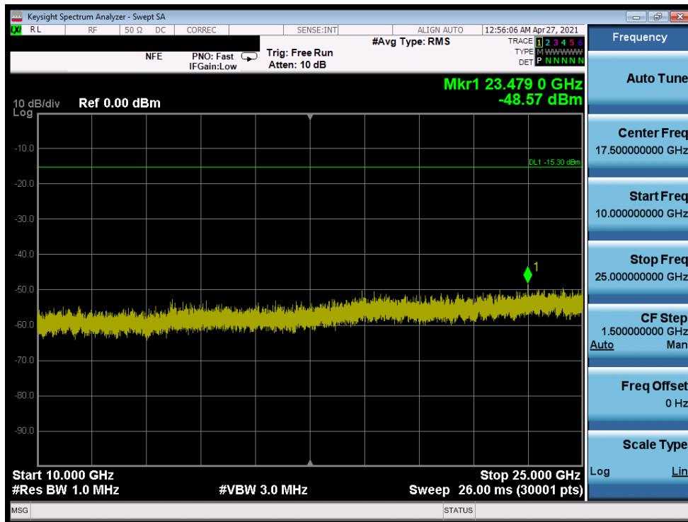
Plot 7-96. Conducted Spurious Plot (Bluetooth (LE), 1Mbps – Ch. 0)
