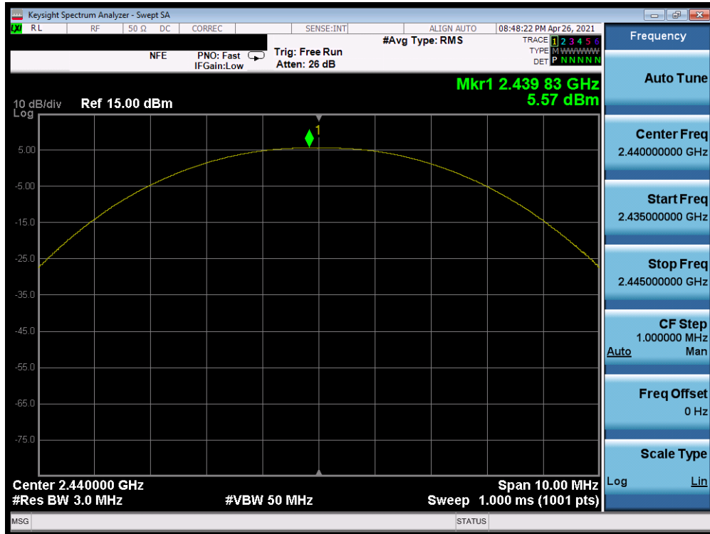
Plot 7-41. Peak Power Plot (Bluetooth (LE), 500kbps – Ch. 19)
