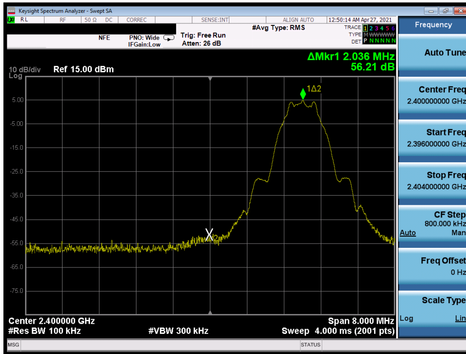
Plot 7-85. Band Edge Plot (Bluetooth (LE), 1Mbps – Ch. 0)
