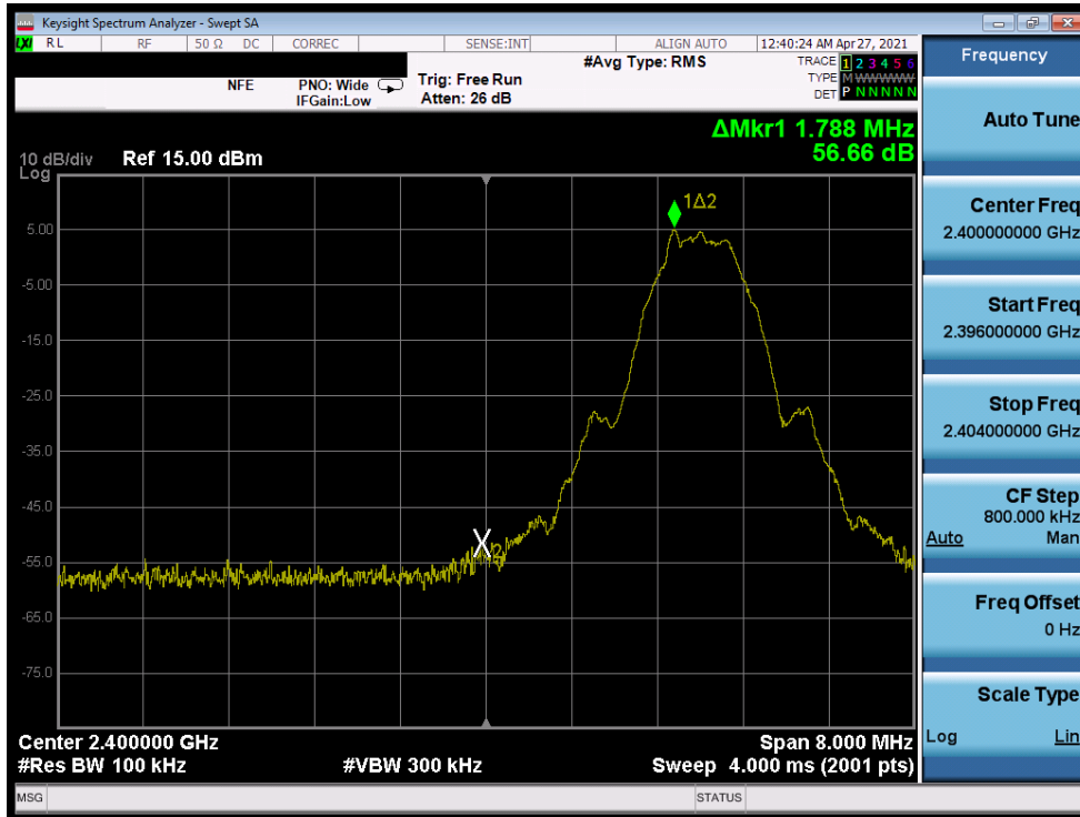
Plot 7-83. Band Edge Plot (Bluetooth (LE), 500kbps – Ch. 0)
