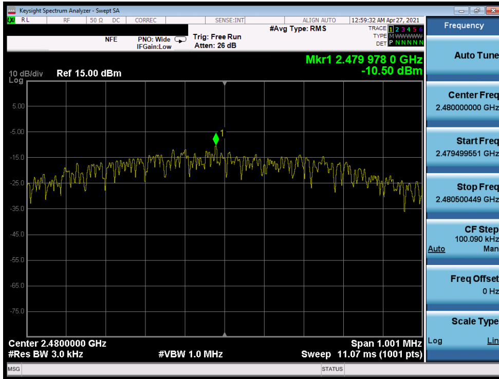
Plot 7-69. Power Spectral Density Plot (Bluetooth (LE), 1Mbps – Ch. 39)
