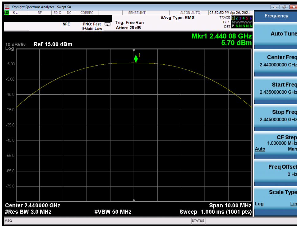
Plot 7-47. Peak Power Plot (Bluetooth (LE), 2Mbps – Ch. 19)
