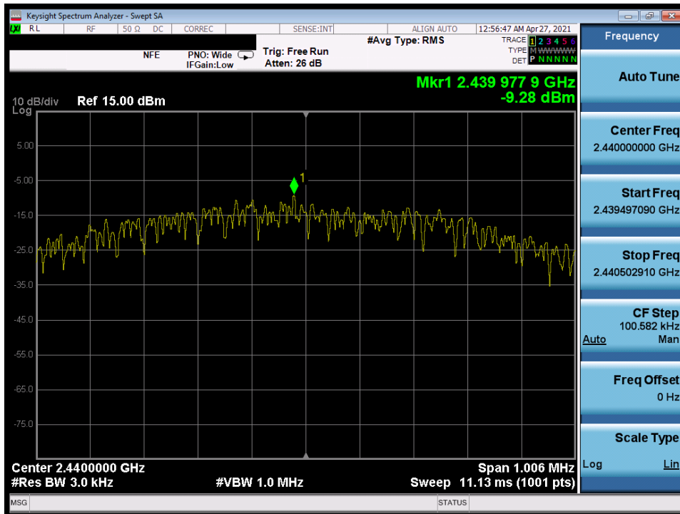
Plot 7-68. Power Spectral Density Plot (Bluetooth (LE), 1Mbps – Ch. 19)
