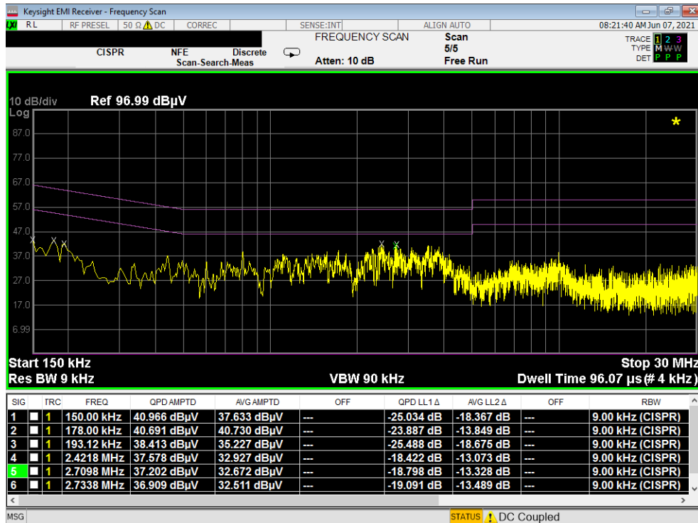
Plot 7-112. Line Conducted Plot with Bluetooth LE (N) with WCP
