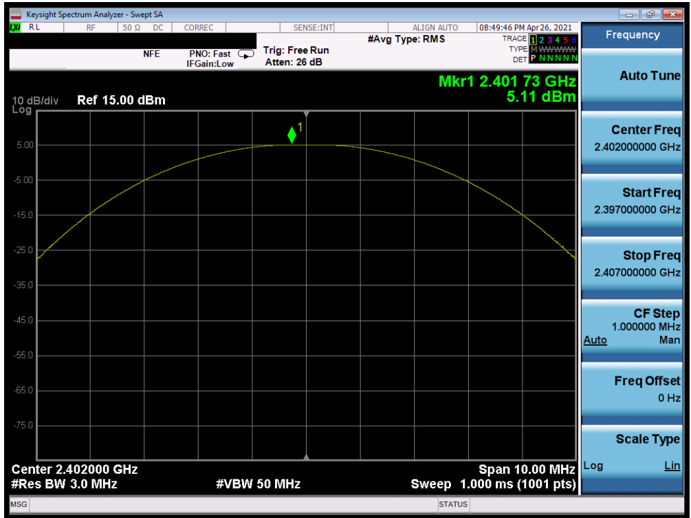
Plot 7-43. Peak Power Plot (Bluetooth (LE), 1Mbps – Ch. 0)
