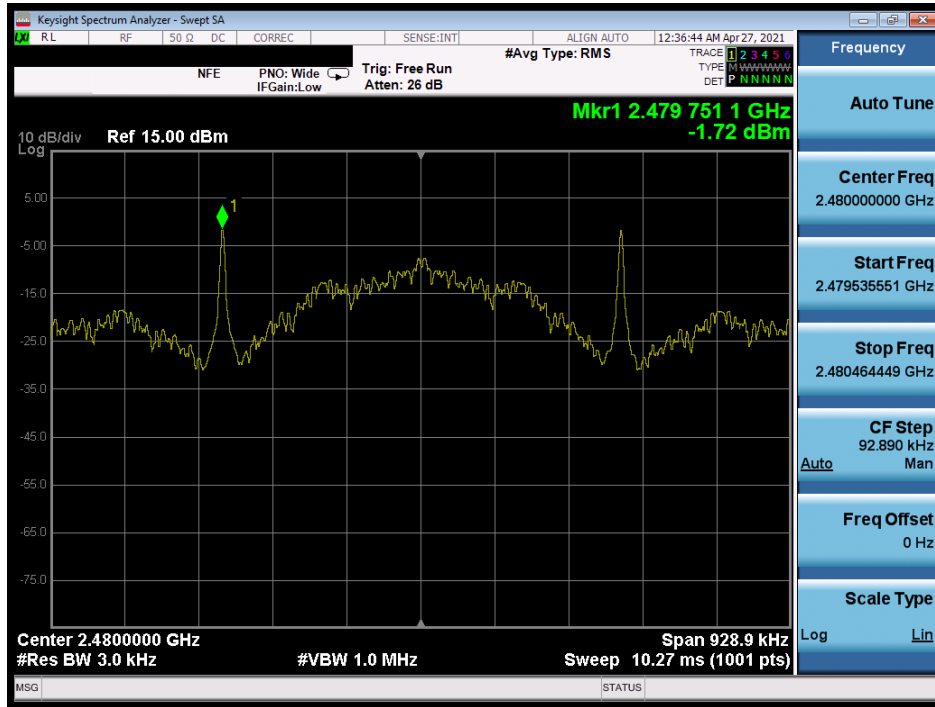
Plot 7-63. Power Spectral Density Plot (Bluetooth (LE), 125kbps – Ch. 39)
