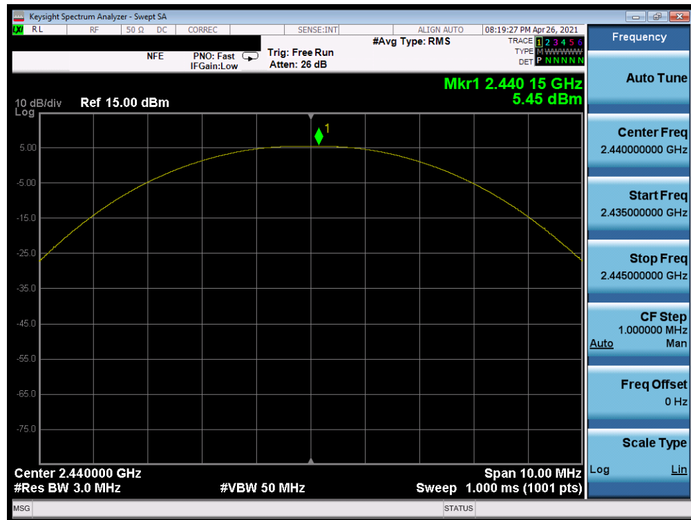
Plot 7-38. Peak Power Plot (Bluetooth (LE), 125kbps – Ch. 19)
