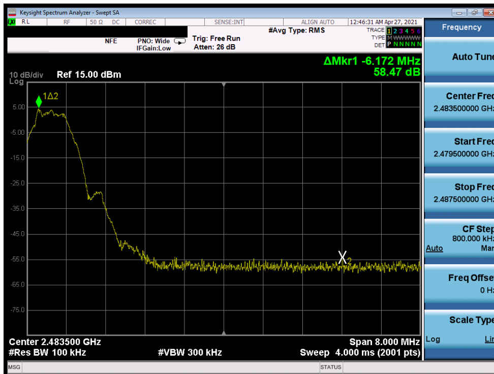
Plot 7-84. Band Edge Plot (Bluetooth (LE), 500kbps – Ch. 39)
