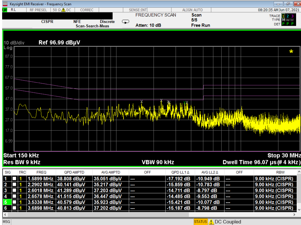
Plot 7-111. Line Conducted Plot with Bluetooth LE (L1) with WCP
