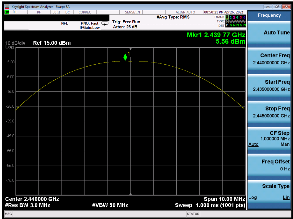
Plot 7-44. Peak Power Plot (Bluetooth (LE), 1Mbps – Ch. 19)
