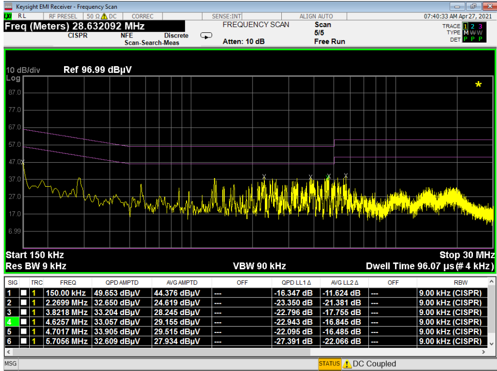
Plot 7-107. Line Conducted Plot with Bluetooth LE (L1) - OPEN
