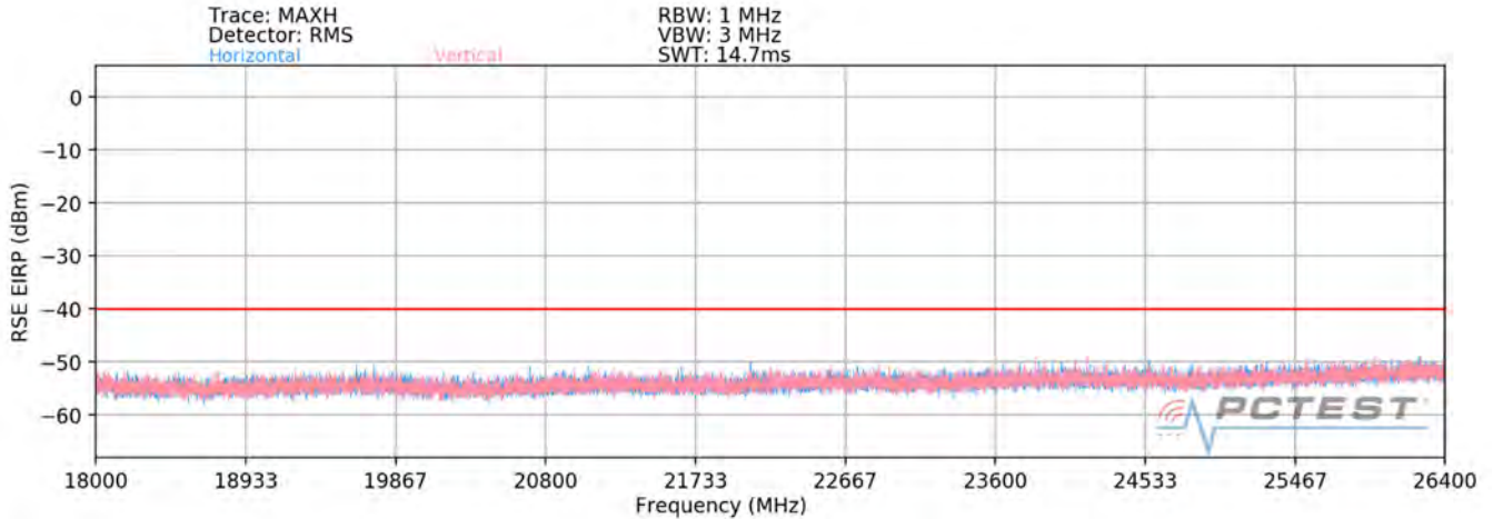
Plot 7-34. Radiated Spurious Plot - 18-26.5 GHz (NR Band n48) – Open
