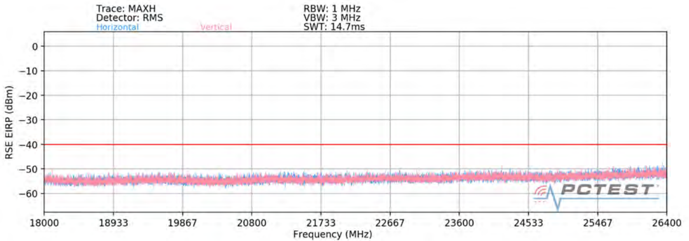
Plot 7-35. Radiated Spurious Plot - 18-26.5 GHz (NR Band n48) – Closed
