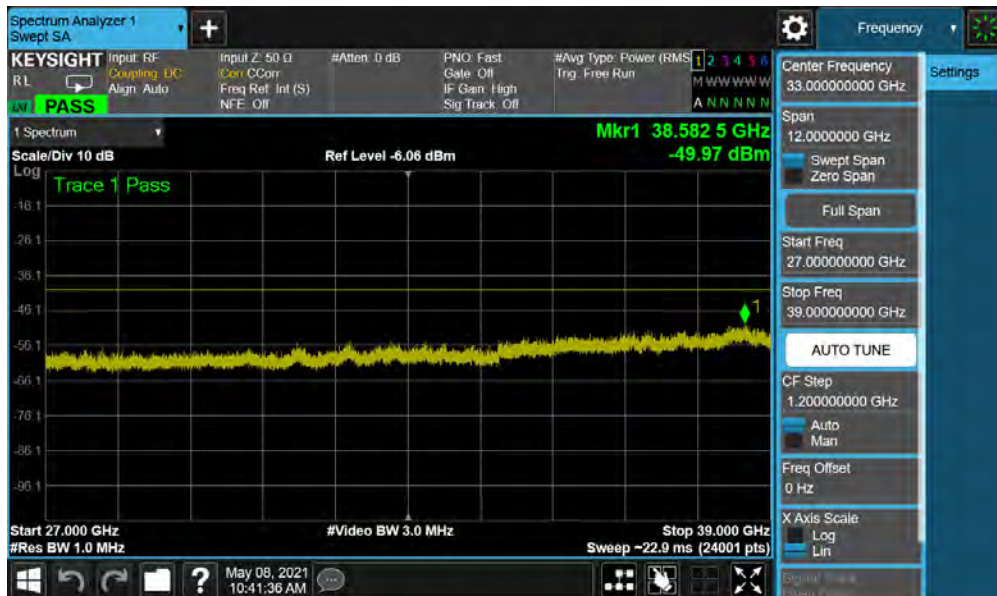
Plot 7-17. Conducted Spurious Plot (NR Band n48 - 40MHz QPSK - Mid Channel)
