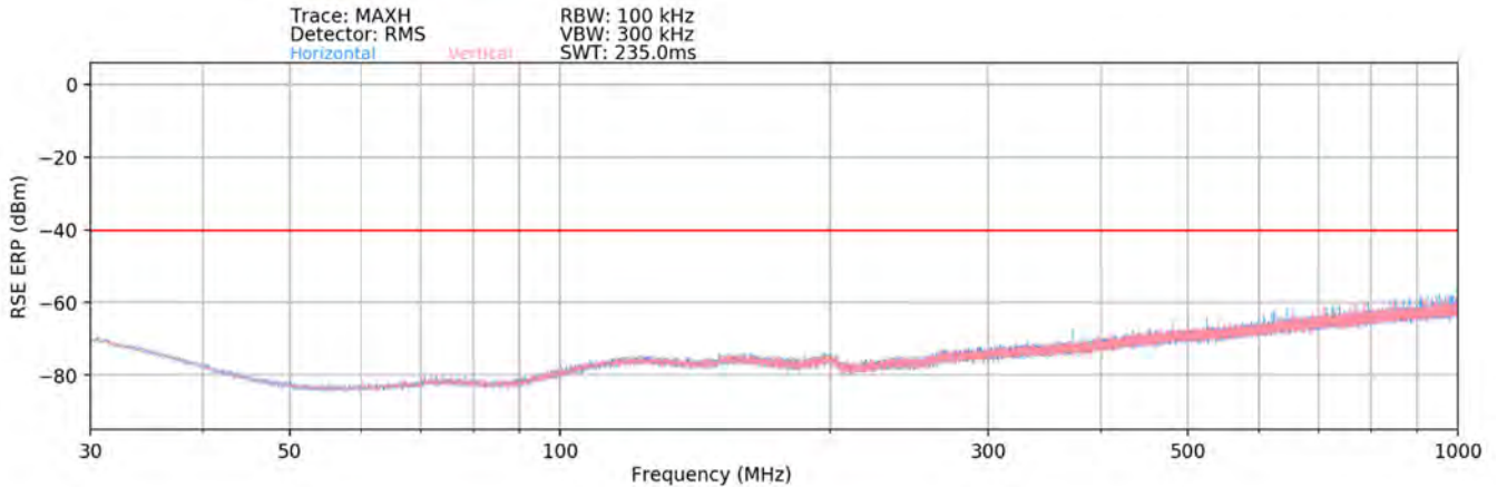
Plot 7-31. Radiated Spurious Plot – 30MHz -1 GHz (NR Band n48) – Open
