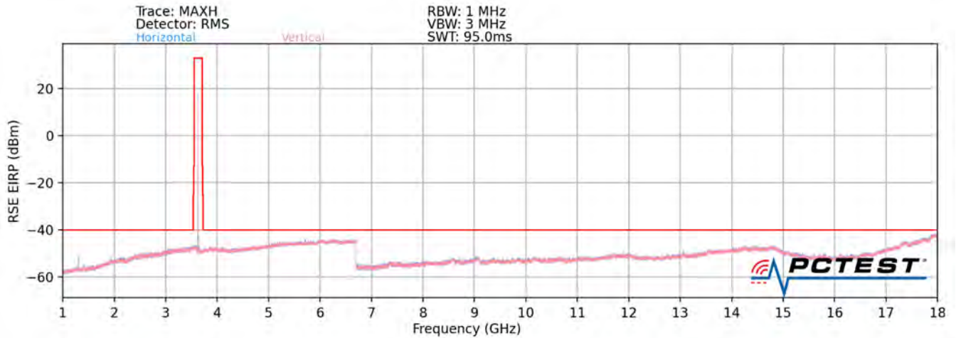
Plot 7-32. Radiated Spurious Plot - 1-18 GHz (NR Band n48) – Open
