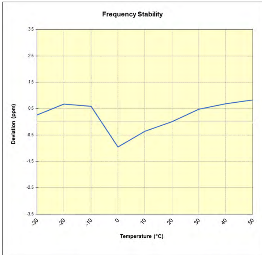
Plot 7-40. NR Band n48 Frequency Stability Chart
