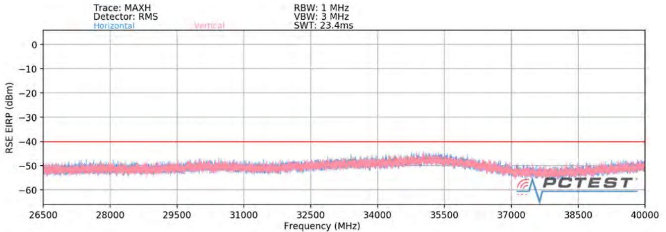
Plot 7-37. Radiated Spurious Plot - 26.5-40 GHz (NR Band n48) – Closed
