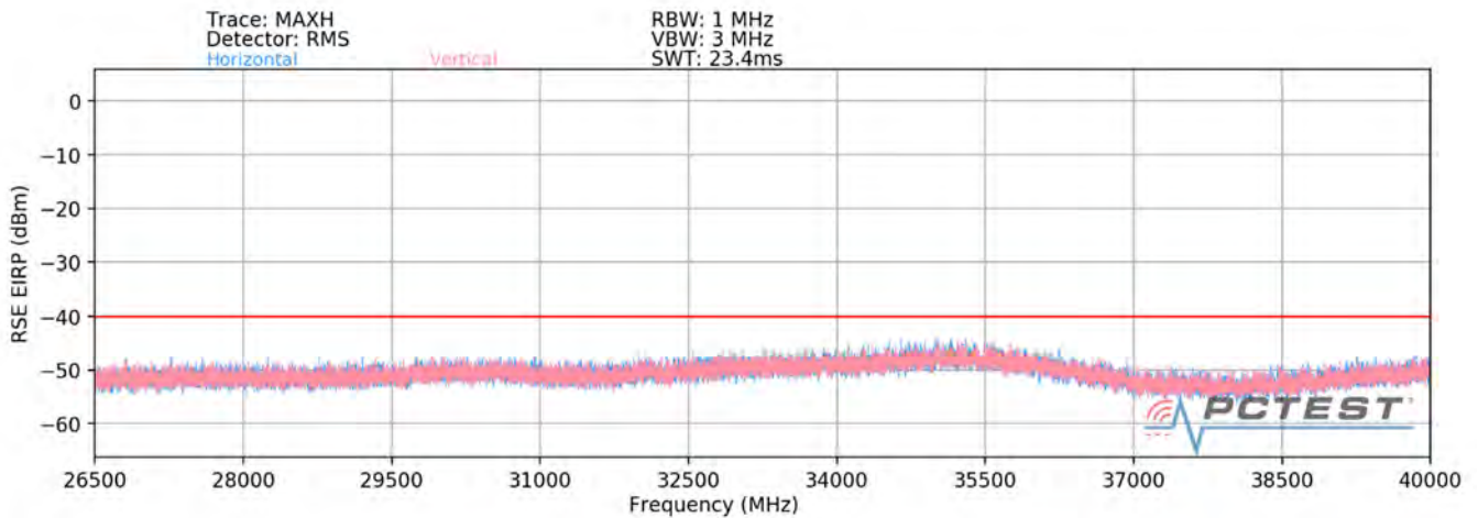
Plot 7-36. Radiated Spurious Plot - 26.5-40 GHz (NR Band n48) – Open
