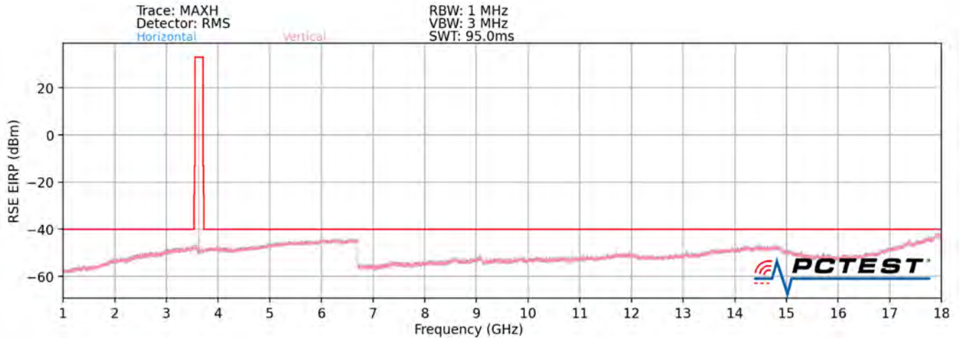
Plot 7-33. Radiated Spurious Plot - 1-18 GHz (NR Band n48) – Closed
