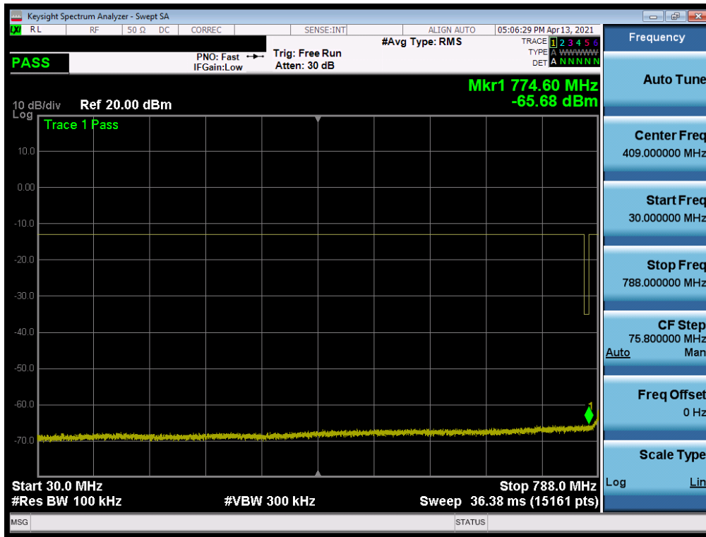
Plot 7-15. Conducted Spurious Plot (LTE Band 14 - 10MHz QPSK - RB Size 1, RB Offset 0)
