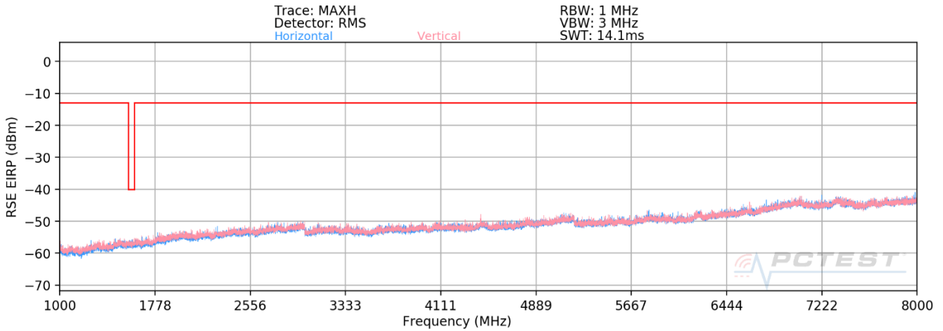
Plot 7-37. Radiated Spurious Plot (LTE Band 14 – Open)
