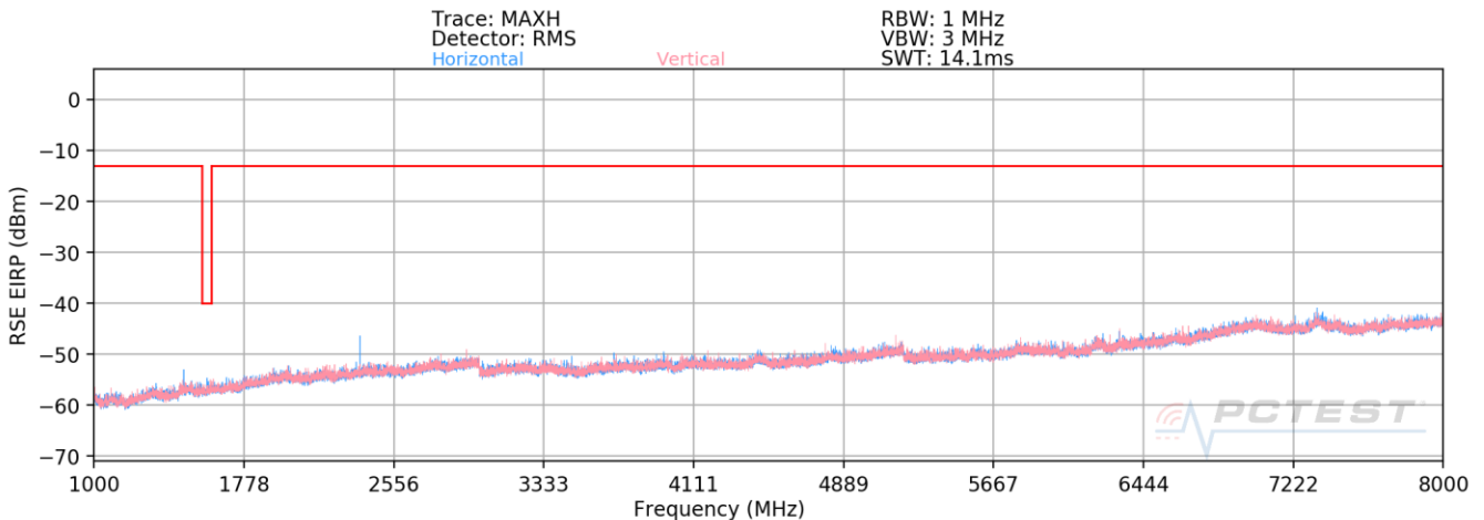
Plot 7-38. Radiated Spurious Plot (LTE Band 14 – Closed)
