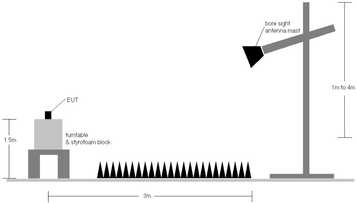
Figure 7-5. Test Instrument & Measurement Setup
