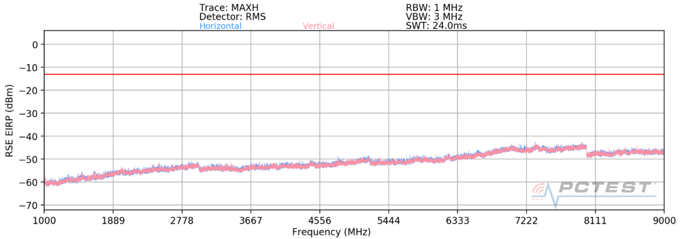
Plot 7-39. Radiated Spurious Plot (LTE Band 26 – Open)
