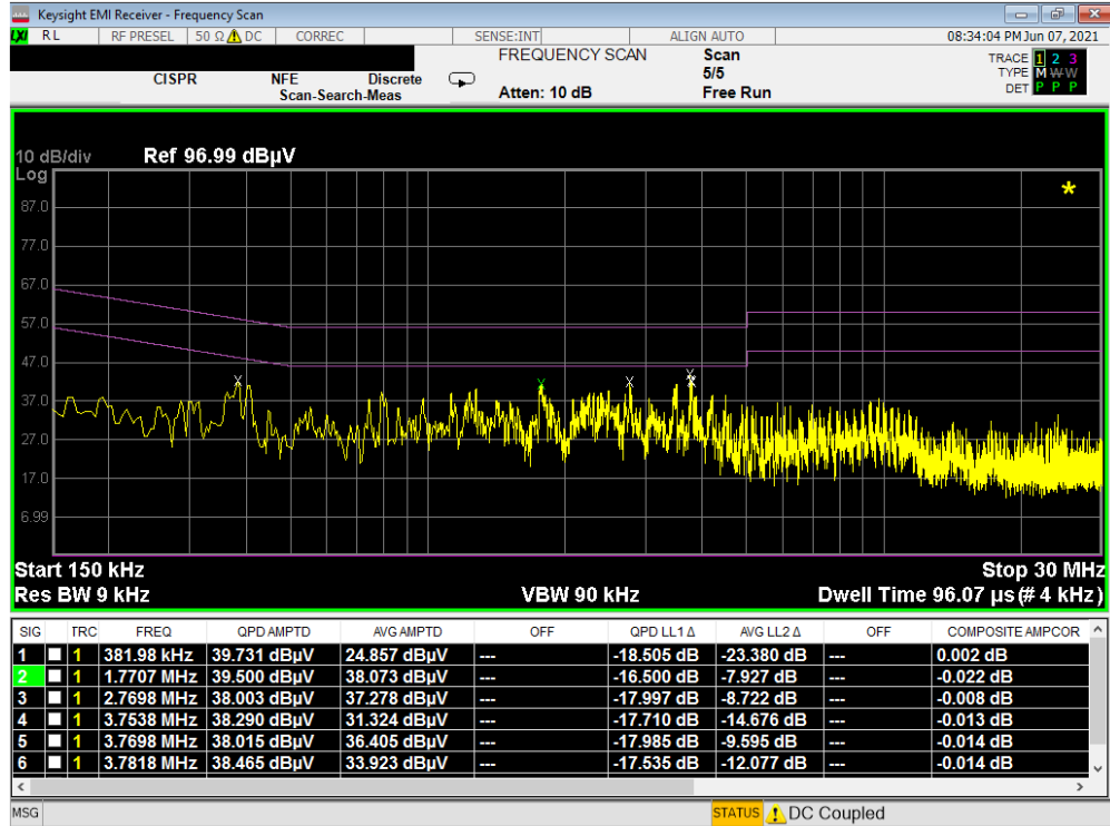
Plot 7-11. Line-Conducted Test Plot (L1) with WCP
