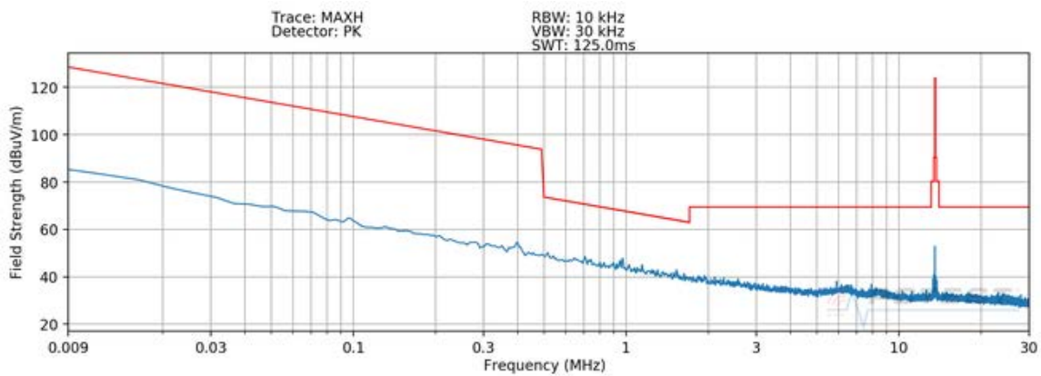
Plot 7-5. Radiated Spurious Plot 9kHz – 30MHz (Pol. Y) _CLOSED
