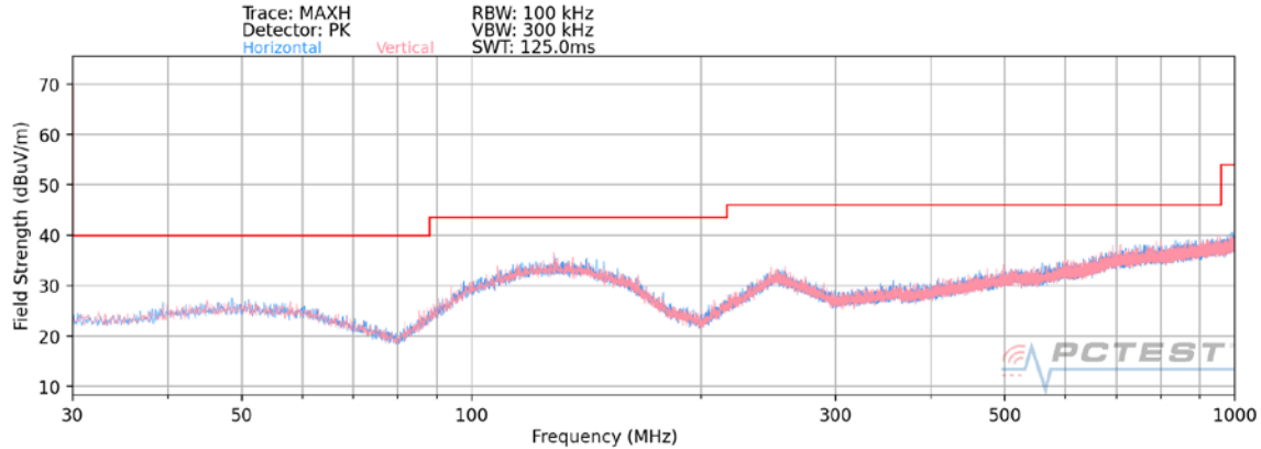
Plot 7-7. Radiated Spurious Plot 30MHz – 1GHz _OPEN
