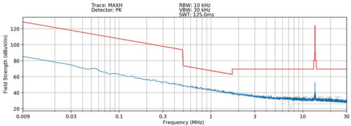
Plot 7-2. Radiated Spurious Plot 9kHz – 30MHz (Pol. Y) _OPEN
