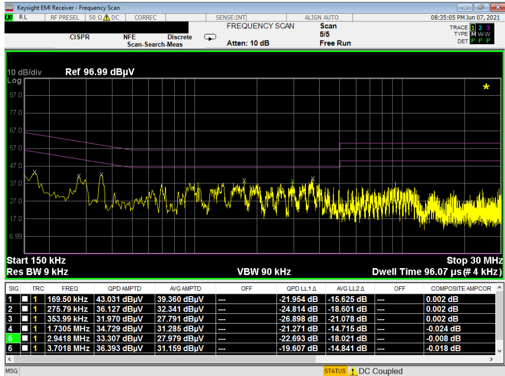
Plot 7-12. Line-Conducted Test Plot (N) with WCP
