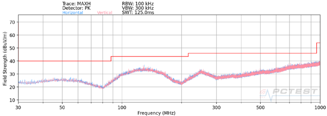
Plot 7-8. Radiated Spurious Plot 30MHz – 1GHz _CLOSED
