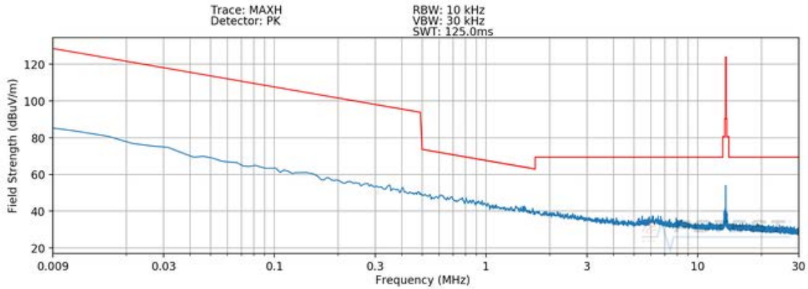
Plot 7-4. Radiated Spurious Plot 9kHz – 30MHz (Pol. X) _CLOSED
