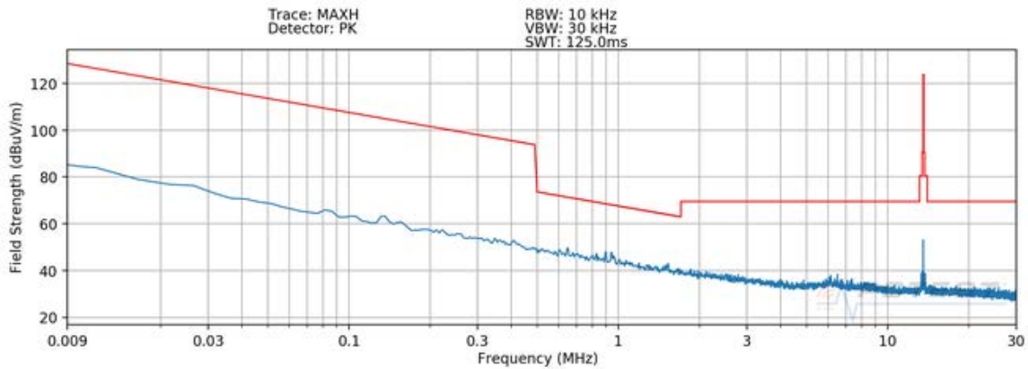
Plot 7-6. Radiated Spurious Plot 9kHz – 30MHz (Pol. Z) _CLOSED
