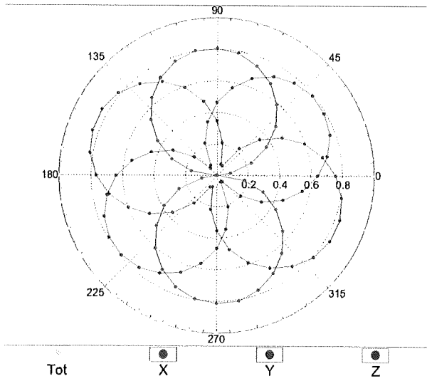
f=600 MHz,TEM
