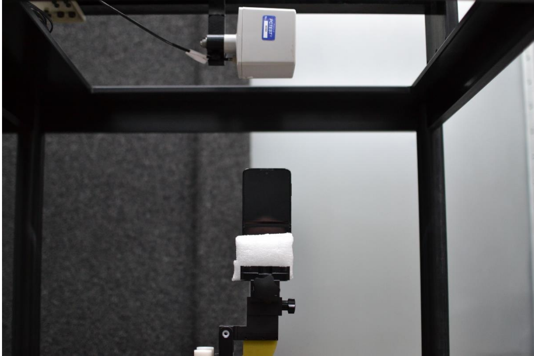
Plot 29. E-field – 15cm
