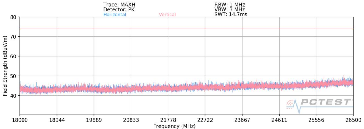
Plot 7-155. Radiated Spurious Plot above 18GHz CDD – OPEN (N)
