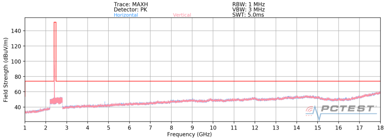
Plot 7-125. Radiated Spurious Plot above 1GHz SISO ANT2 (802.11b – Ch. 1) – OPEN (Q)
