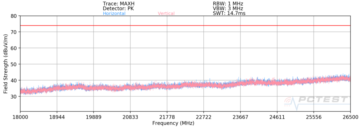
Plot 7-137. Radiated Spurious Plot above 18GHz SISO ANT2 – OPEN (Q)
