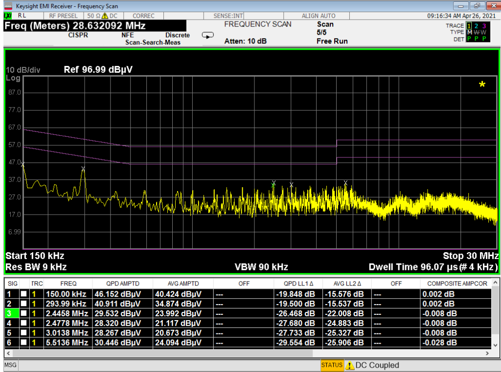
Plot 7-187. Line Conducted Plot with 802.11b (L1) – CLOSED (N)
