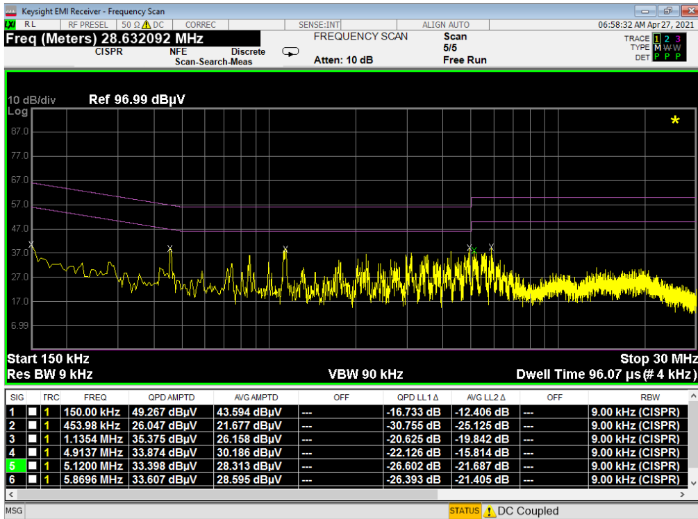
Plot 7-182. Line Conducted Plot with 802.11b (N) – OPEN (Q)
