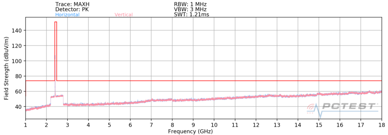
Plot 7-150. Radiated Spurious Plot above 1GHz CDD (802.11b – Ch. 1) – CLOSED (N)
