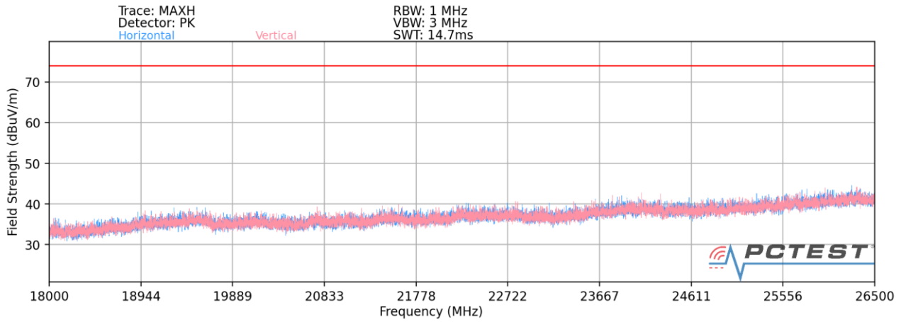
Plot 7-138. Radiated Spurious Plot above 18GHz SISO ANT2– CLOSED (Q)
