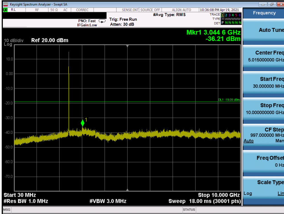
Plot 7-115. Conducted Spurious Plot SISO ANT2 (802.11b – Ch. 6) – Q
