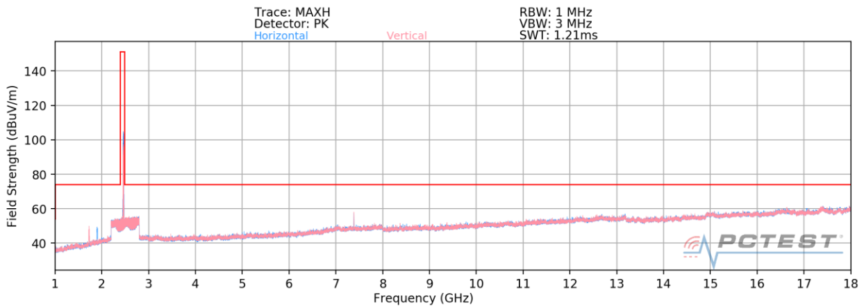
Plot 7-136. Radiated Spurious Plot above 1GHz SISO ANT2 (802.11b – Ch. 11) – CLOSED (N)
