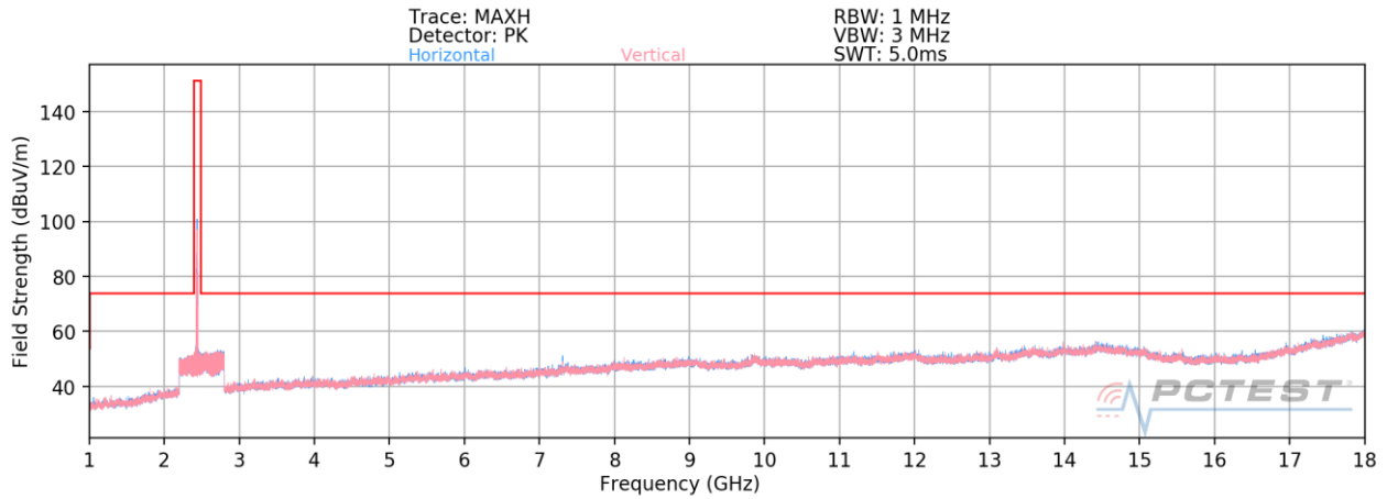
Plot 7-129. Radiated Spurious Plot above 1GHz SISO ANT2 (802.11b – Ch. 6) – CLOSED (Q)
