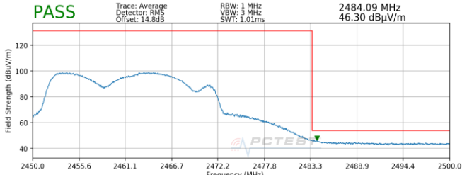
Plot 7-173. Radiated Restricted Band Edge Measurement MIMO with WCP (Average) – Q
