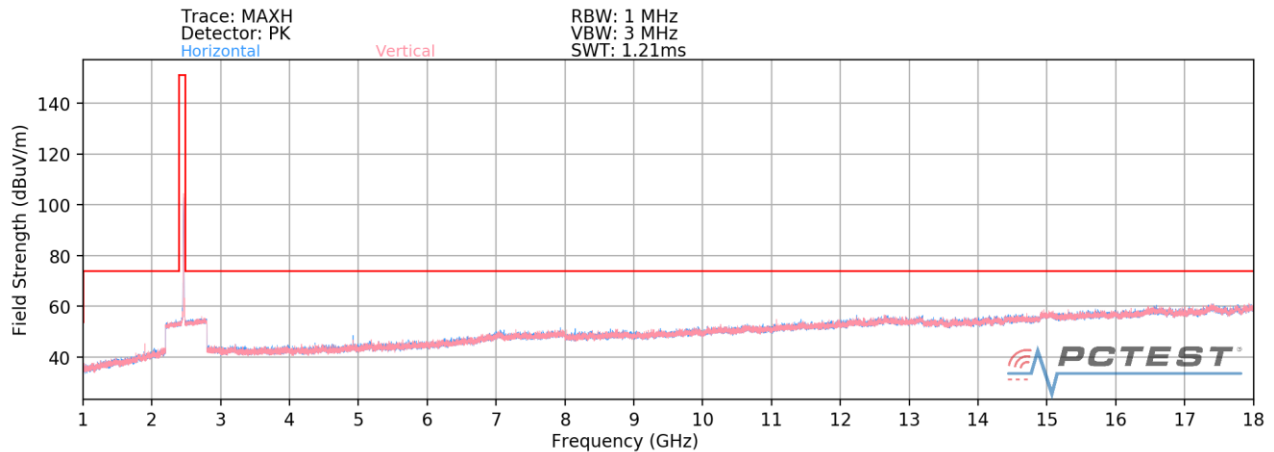
Plot 7-149. Radiated Spurious Plot above 1GHz CDD (802.11b – Ch. 11) – OPEN (N)
