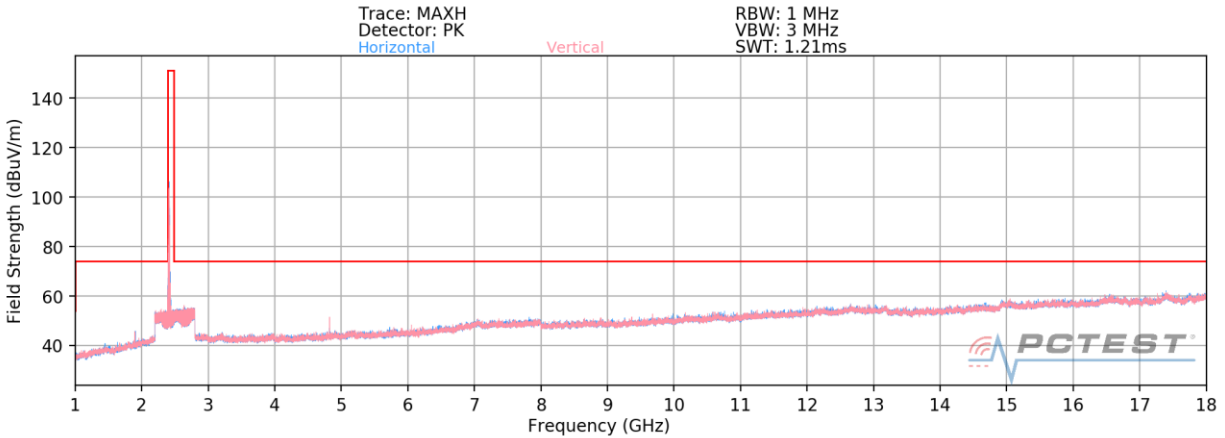
Plot 7-131. Radiated Spurious Plot above 1GHz SISO ANT2 (802.11b – Ch. 1) – OPEN (N)
