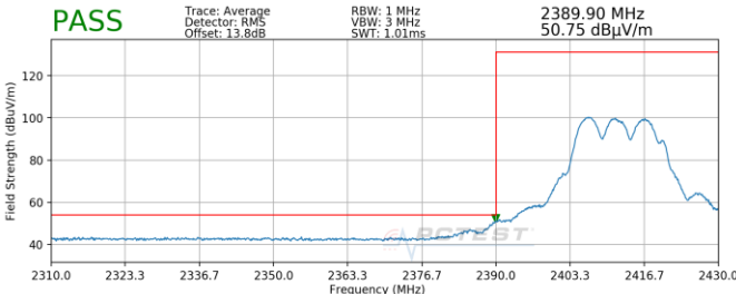
Plot 7-175. Radiated Restricted Band Edge Measurement MIMO with WCP (Average) – N
