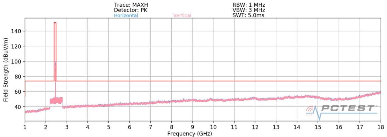
Plot 7-130. Radiated Spurious Plot above 1GHz SISO ANT2 (802.11b – Ch. 11) – CLOSED (Q)
