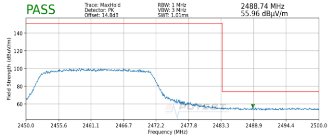
Plot 7-162. Radiated Restricted Upper Band Edge Measurement SISO ANT2 (Peak) - Q
