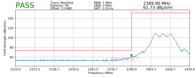
Plot 7-176. Radiated Restricted Band Edge Measurement MIMO with WCP (Peak) – N
