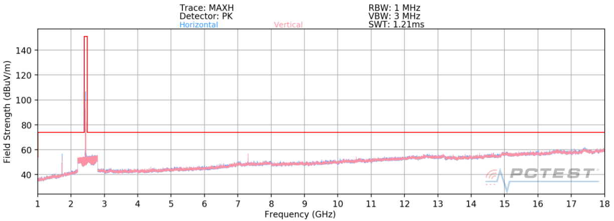
Plot 7-135. Radiated Spurious Plot above 1GHz SISO ANT2 (802.11b – Ch. 6) – CLOSED (N)
