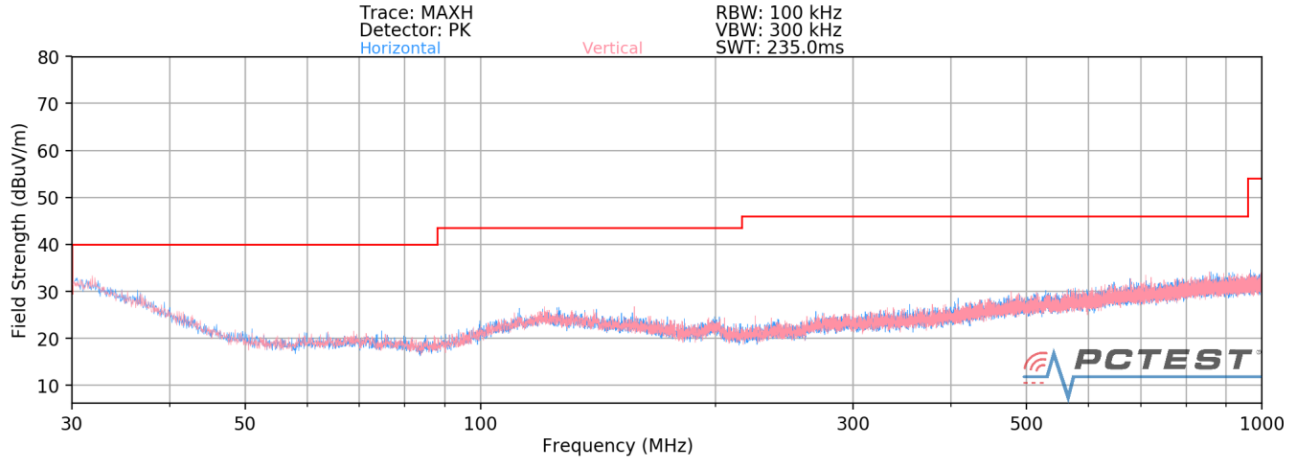
Plot 7-177. Radiated Spurious Plot below 1GHz MIMO – OPEN (Q)
