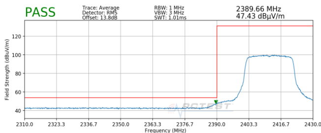
Plot 7-159. Radiated Restricted Lower Band Edge Measurement SISO ANT2 (Average) - N
