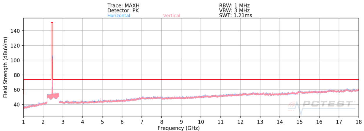
Plot 7-127. Radiated Spurious Plot above 1GHz SISO ANT2 (802.11b – Ch. 11) – OPEN (Q)
