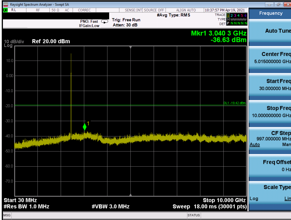
Plot 7-117. Conducted Spurious Plot SISO ANT2 (802.11b – Ch. 11) – Q
