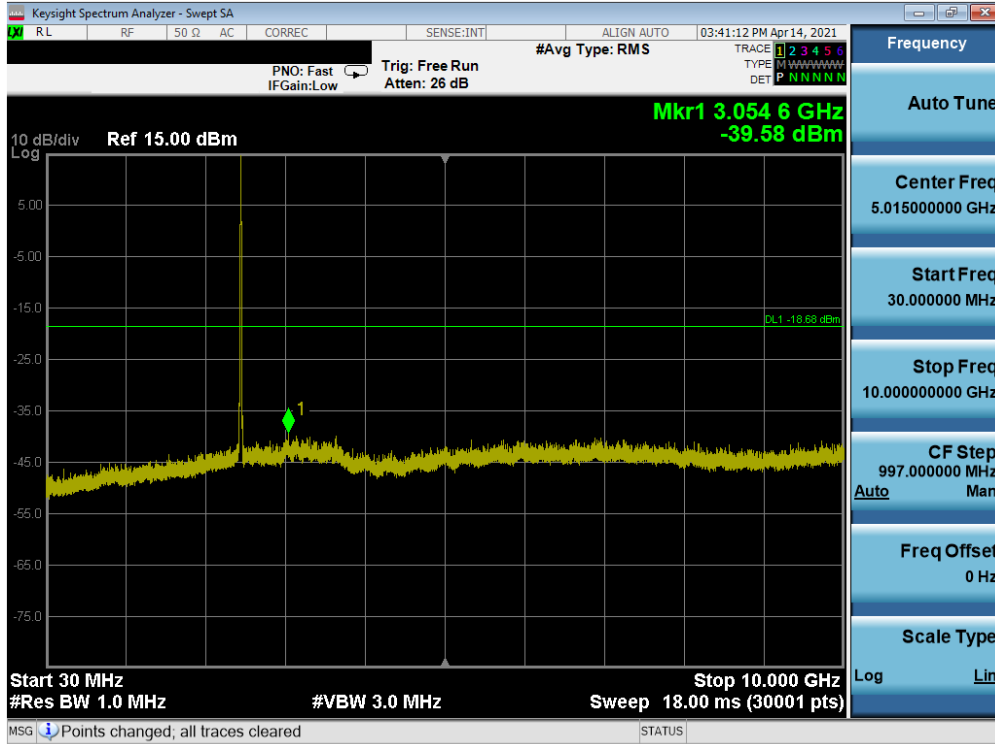
Plot 7-123. Conducted Spurious Plot SISO ANT2 (802.11b – Ch. 11) – N
