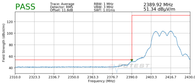
Plot 7-167. Radiated Restricted Lower Band Edge Measurement MIMO (Average) – N
