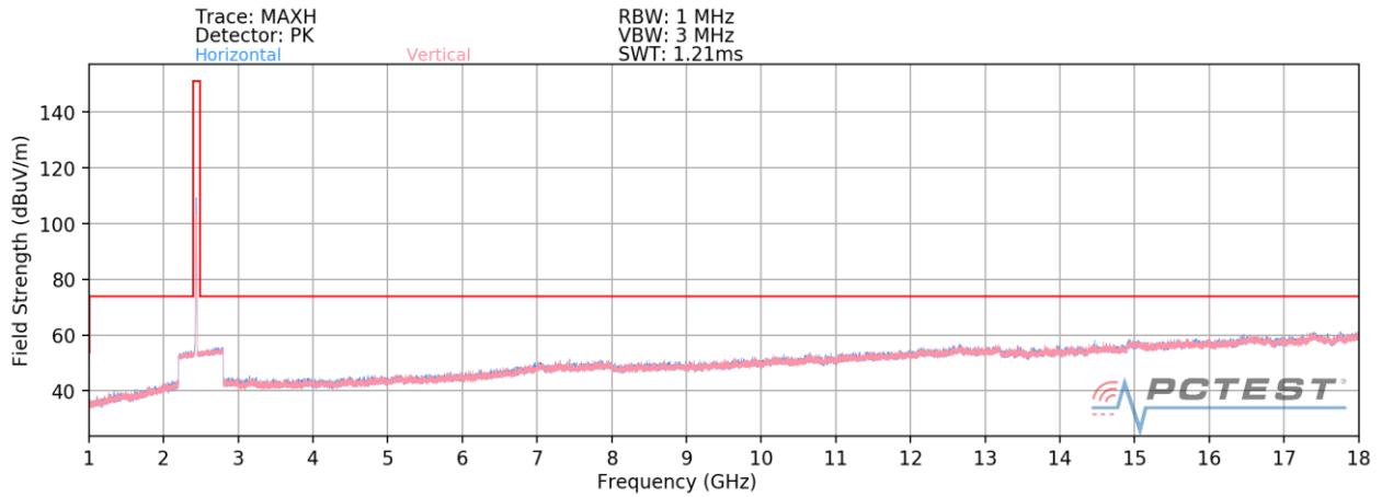
Plot 7-142. Radiated Spurious Plot above 1GHz CDD (802.11b – Ch. 6) – OPEN (Q)
