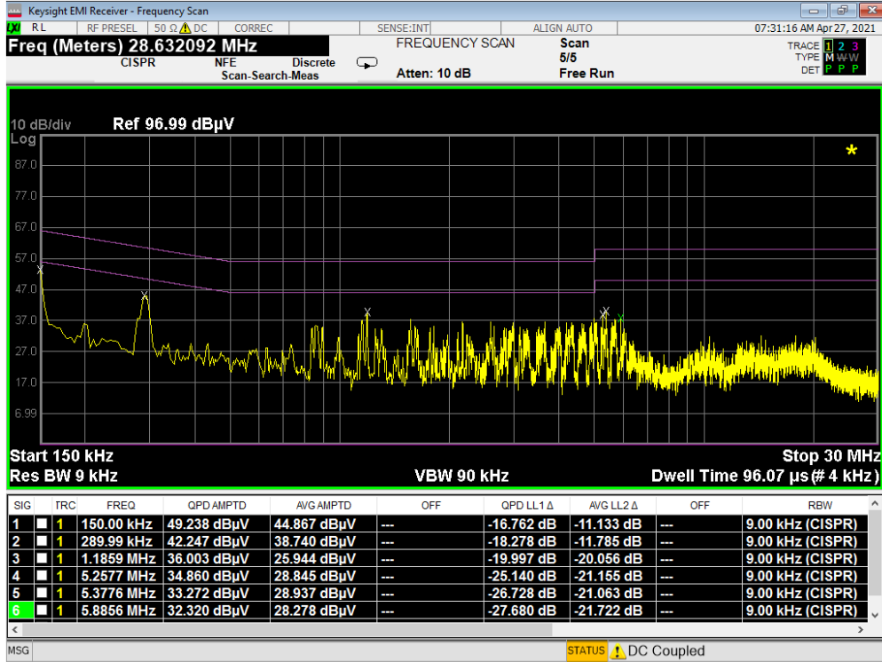
Plot 7-183. Line Conducted Plot with 802.11b (L1) – CLOSED (Q)
