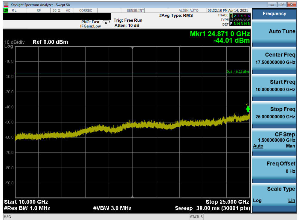
Plot 7-122. Conducted Spurious Plot SISO ANT2 (802.11b – Ch. 6) – N
