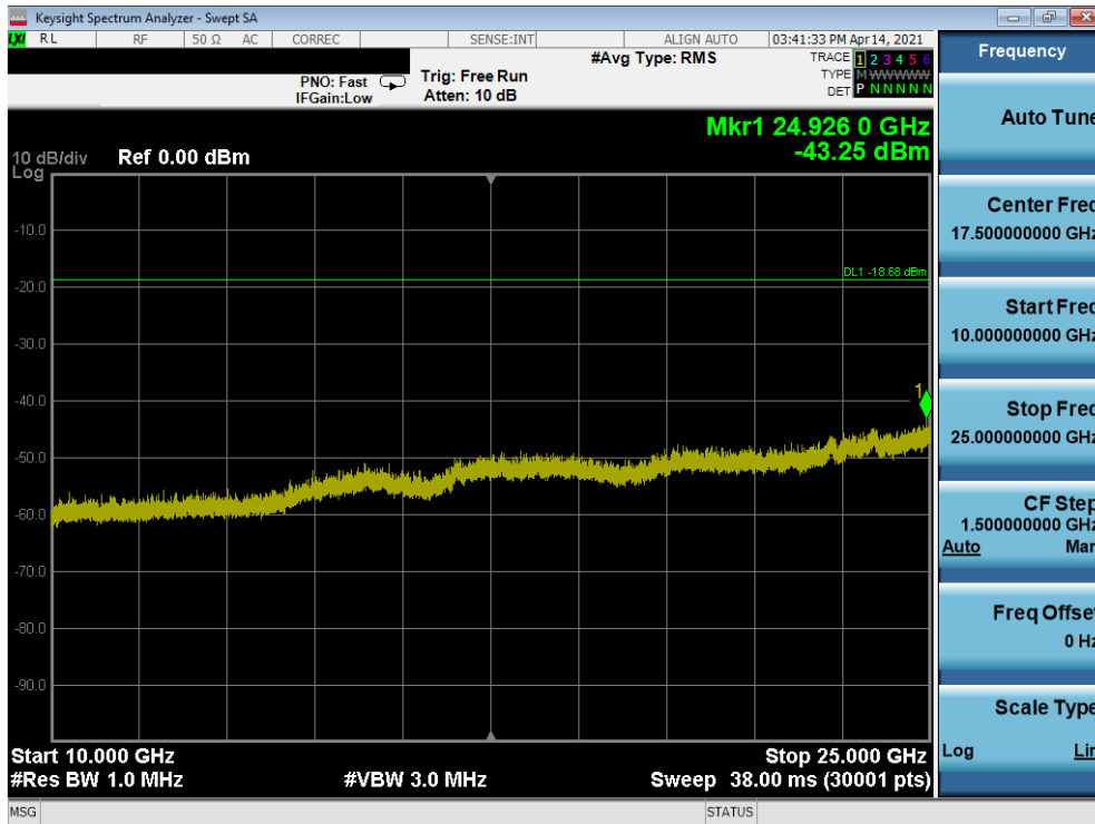
Plot 7-124. Conducted Spurious Plot SISO ANT2 (802.11b – Ch. 11) – N
