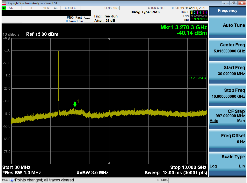
Plot 7-121. Conducted Spurious Plot SISO ANT2 (802.11b – Ch. 6) – N
