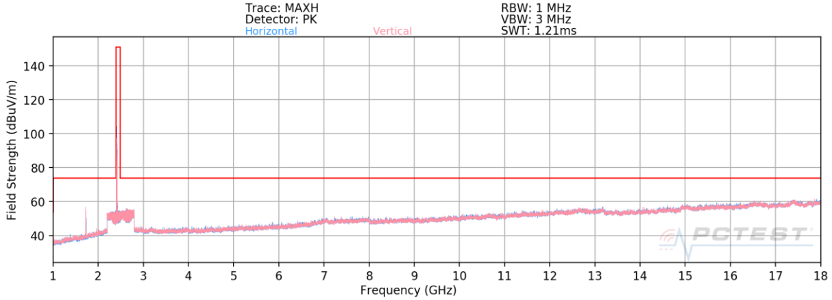
Plot 7-134. Radiated Spurious Plot above 1GHz SISO ANT2 (802.11b – Ch. 1) – CLOSED (N)
