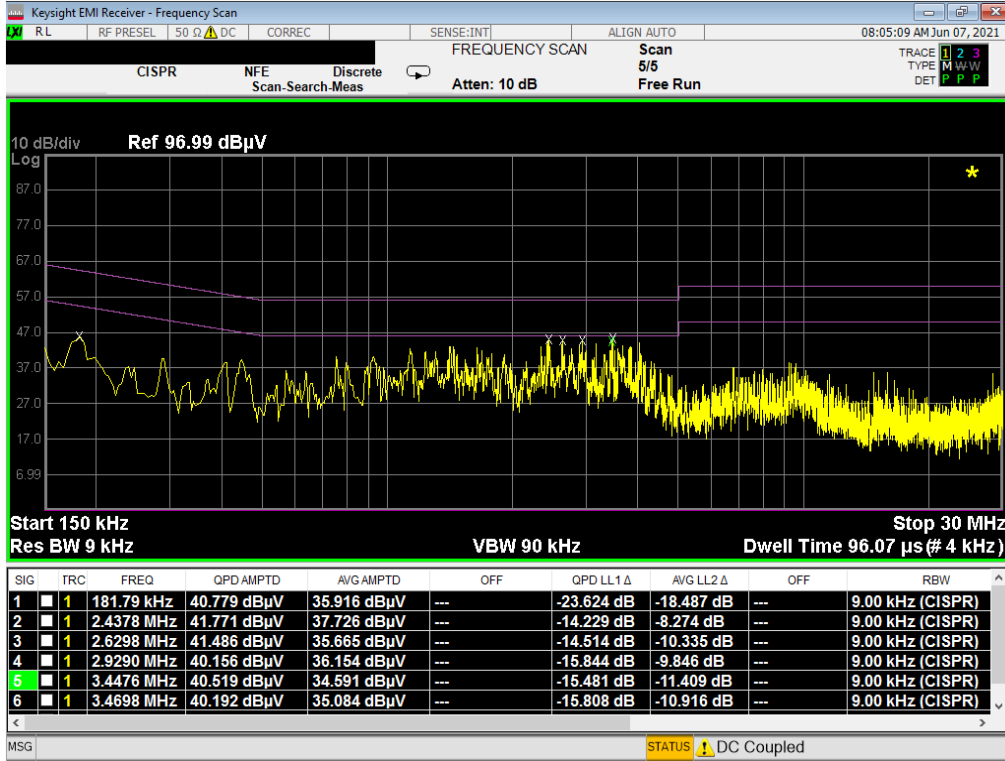
Plot 7-189. Line Conducted Plot with 802.11b (L1) with WCP – Q
