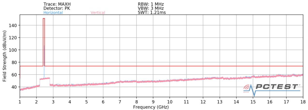
Plot 7-143. Radiated Spurious Plot above 1GHz CDD (802.11b – Ch. 11) – OPEN (Q)
