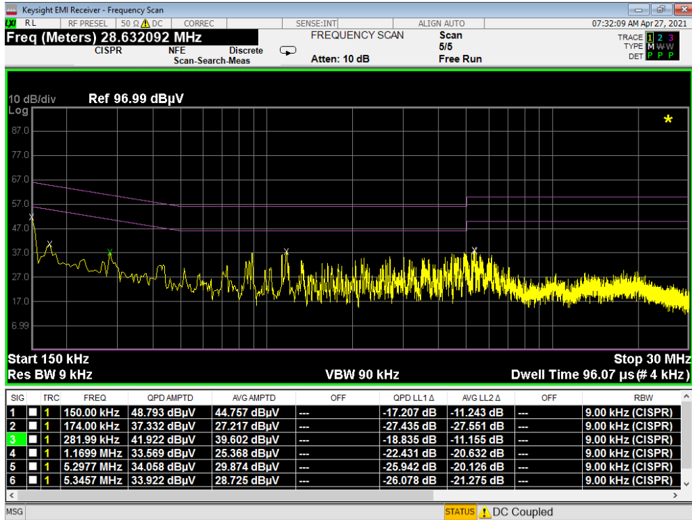
Plot 7-184. Line Conducted Plot with 802.11b (N) – CLOSED (Q)
