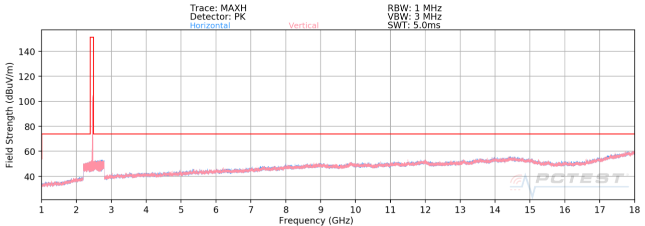
Plot 7-126. Radiated Spurious Plot above 1GHz SISO ANT2 (802.11b – Ch. 6) – OPEN (Q)
