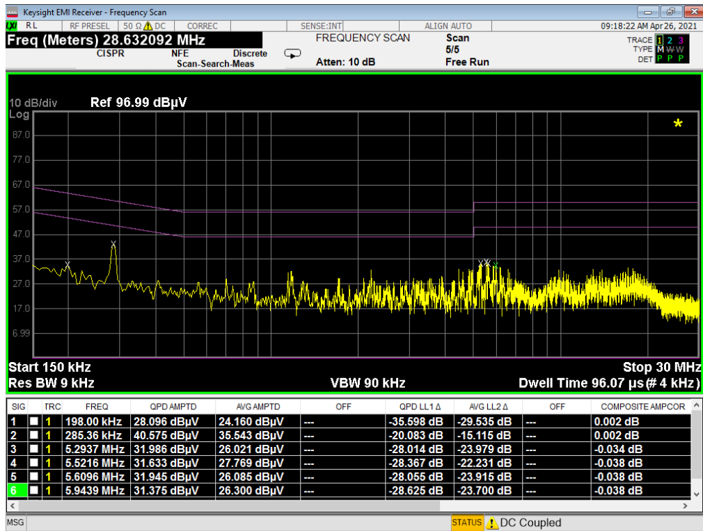
Plot 7-188. Line Conducted Plot with 802.11b (N) – CLOSED (N)
