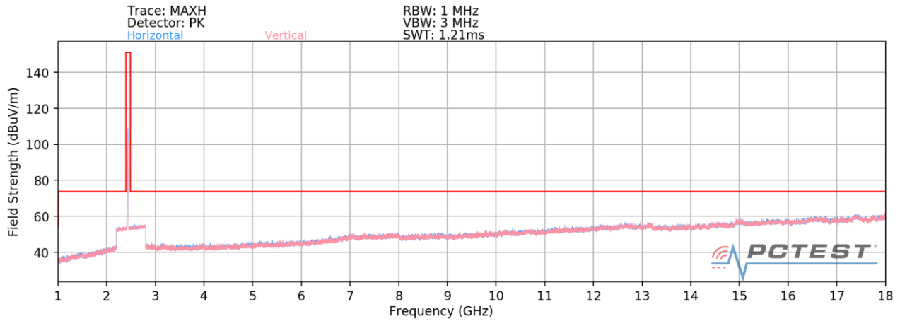
Plot 7-145. Radiated Spurious Plot above 1GHz CDD (802.11b – Ch. 6) – CLOSED (Q)
