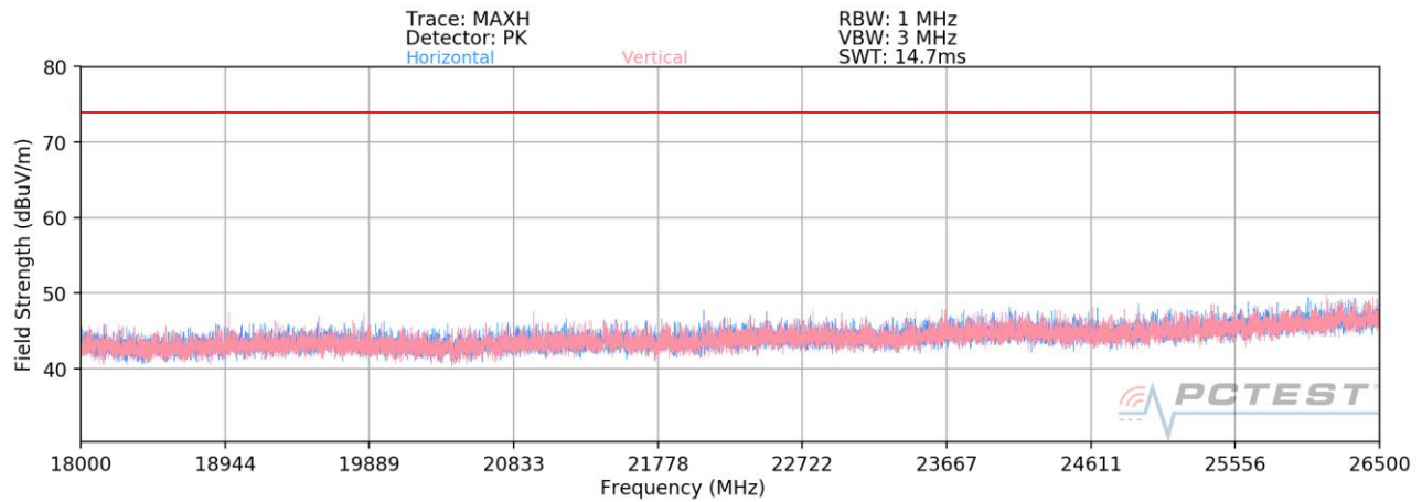
Plot 7-156. Radiated Spurious Plot above 18GHz CDD – CLOSED (N)
