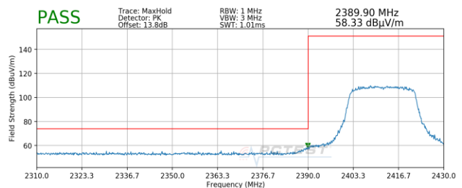
Plot 7-160. Radiated Restricted Lower Band Edge Measurement SISO ANT2 (Peak) - N
