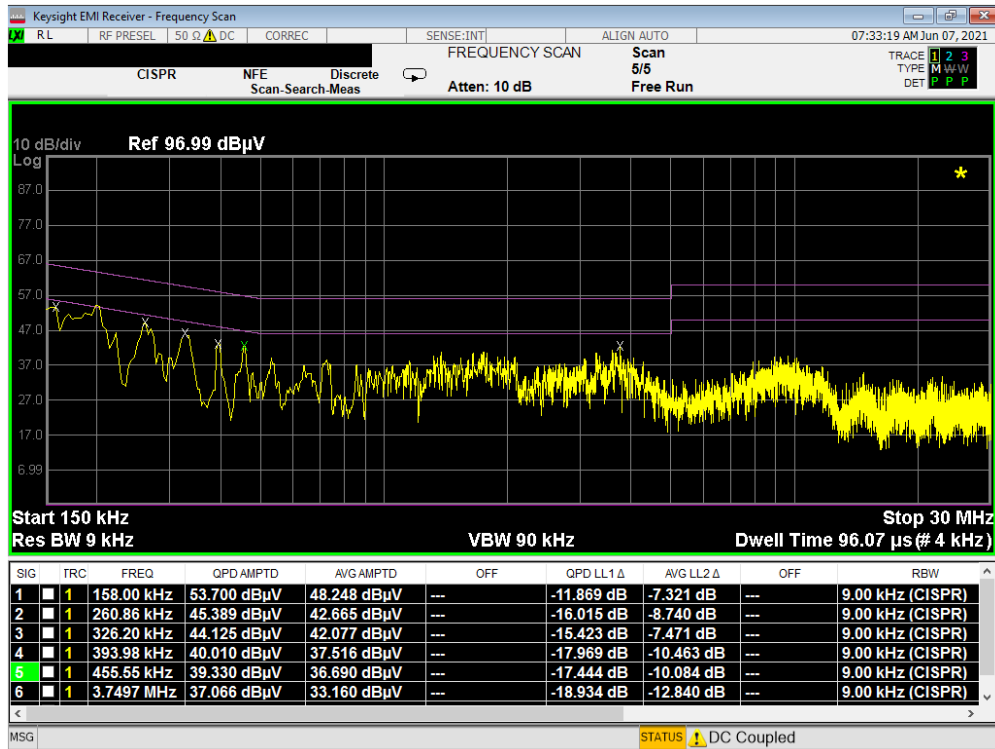
Plot 7-192. Line Conducted Plot with 802.11b (N) with WCP - N
