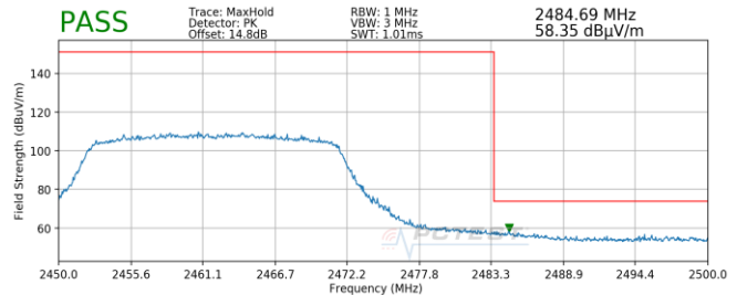
Plot 7-164. Radiated Restricted Upper Band Edge Measurement SISO ANT2 (Peak) - N
