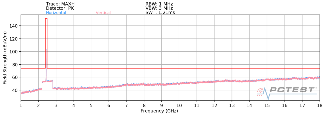
Plot 7-148. Radiated Spurious Plot above 1GHz CDD (802.11b – Ch. 6) – OPEN (N)
