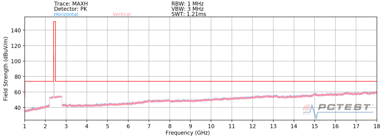
Plot 7-144. Radiated Spurious Plot above 1GHz CDD (802.11b – Ch. 1) – CLOSED (Q)
