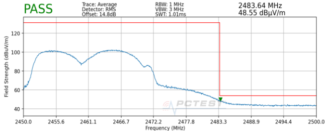
Plot 7-169. Radiated Restricted Upper Band Edge Measurement MIMO (Average) – Q
