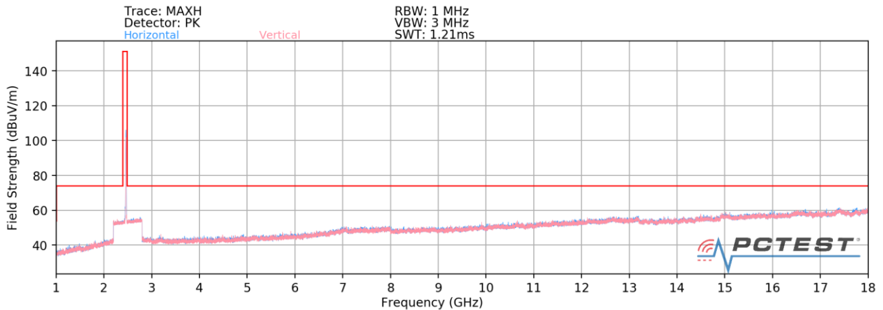
Plot 7-146. Radiated Spurious Plot above 1GHz CDD (802.11b – Ch. 11) – CLOSED (Q)
