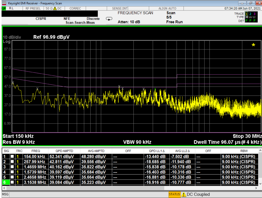
Plot 7-191. Line Conducted Plot with 802.11b (L1) with WCP - N
