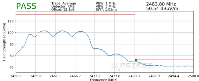
Plot 7-171. Radiated Restricted Upper Band Edge Measurement MIMO (Average) – N
