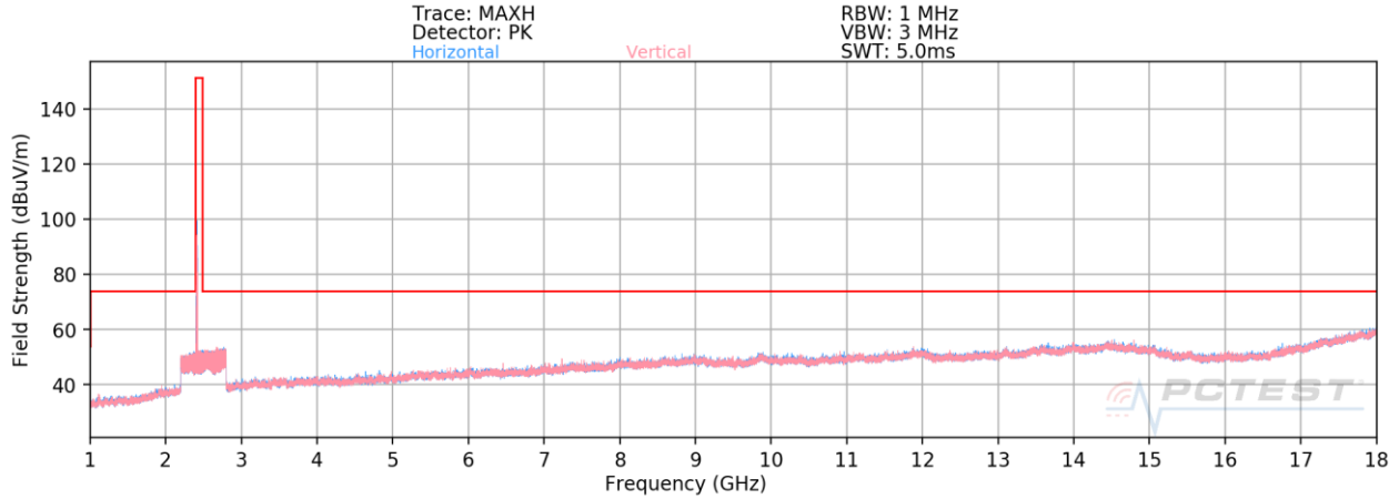
Plot 7-128. Radiated Spurious Plot above 1GHz SISO ANT2 (802.11b – Ch. 1) – CLOSED (Q)
