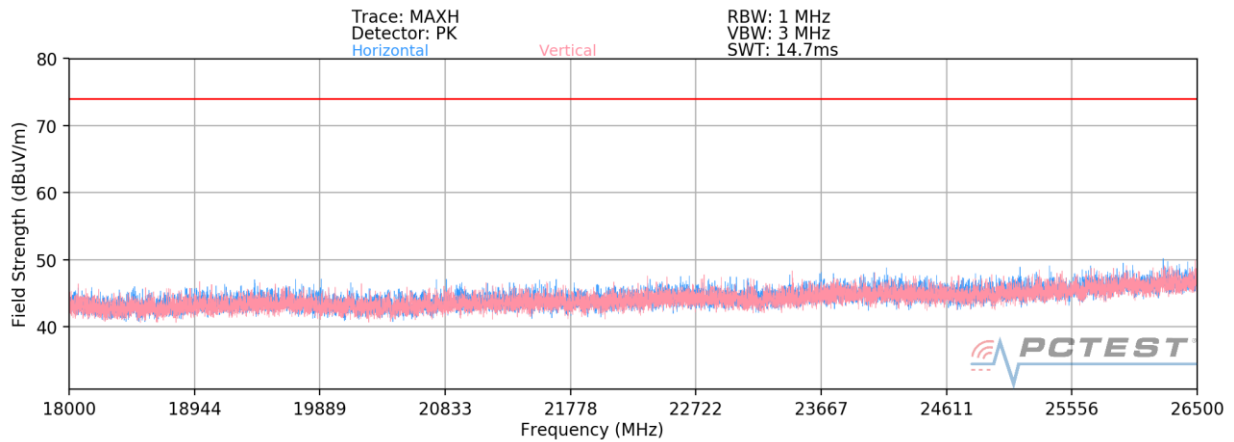
Plot 7-140. Radiated Spurious Plot above 18GHz SISO ANT2- CLOSED (N)
