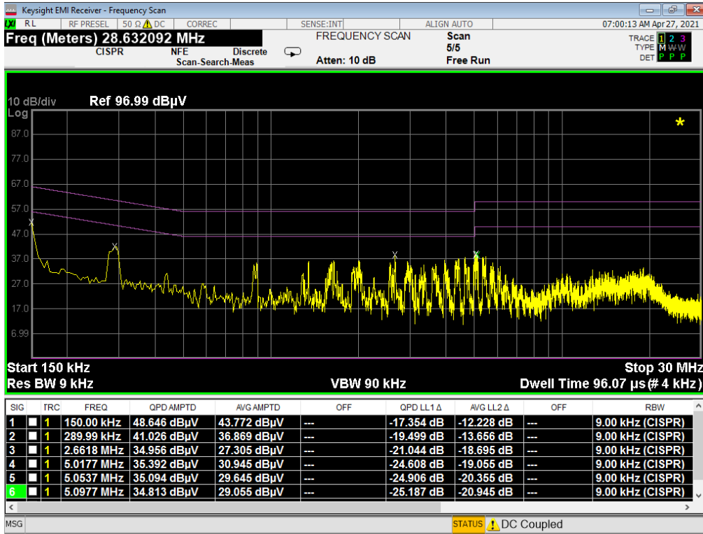
Plot 7-181. Line Conducted Plot with 802.11b (L1) – OPEN (Q)
