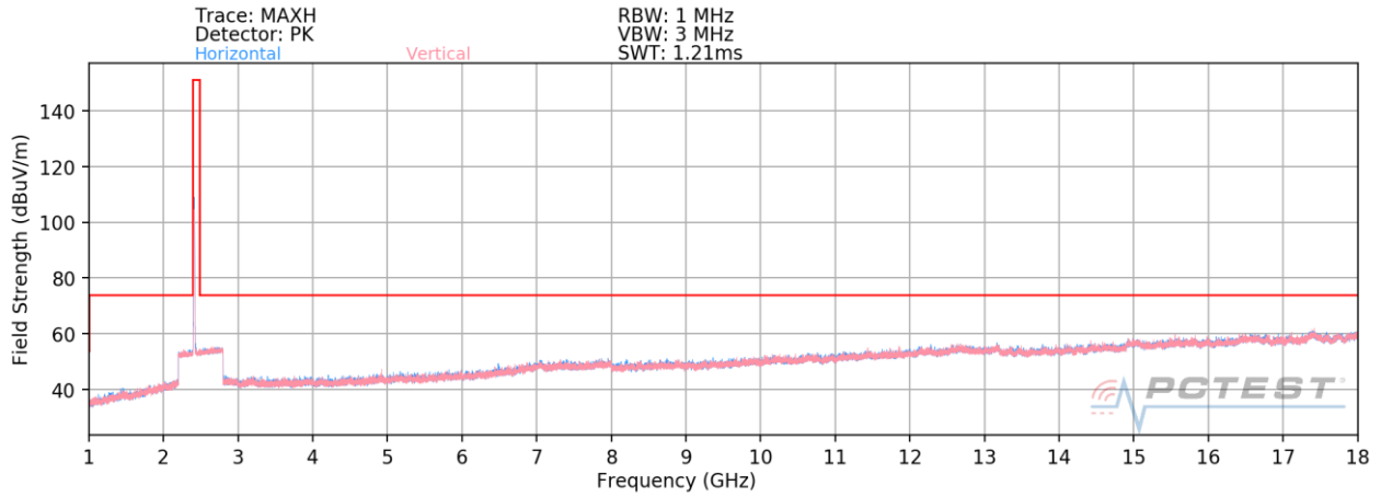
Plot 7-141. Radiated Spurious Plot above 1GHz CDD (802.11b – Ch. 1) – OPEN (Q)
