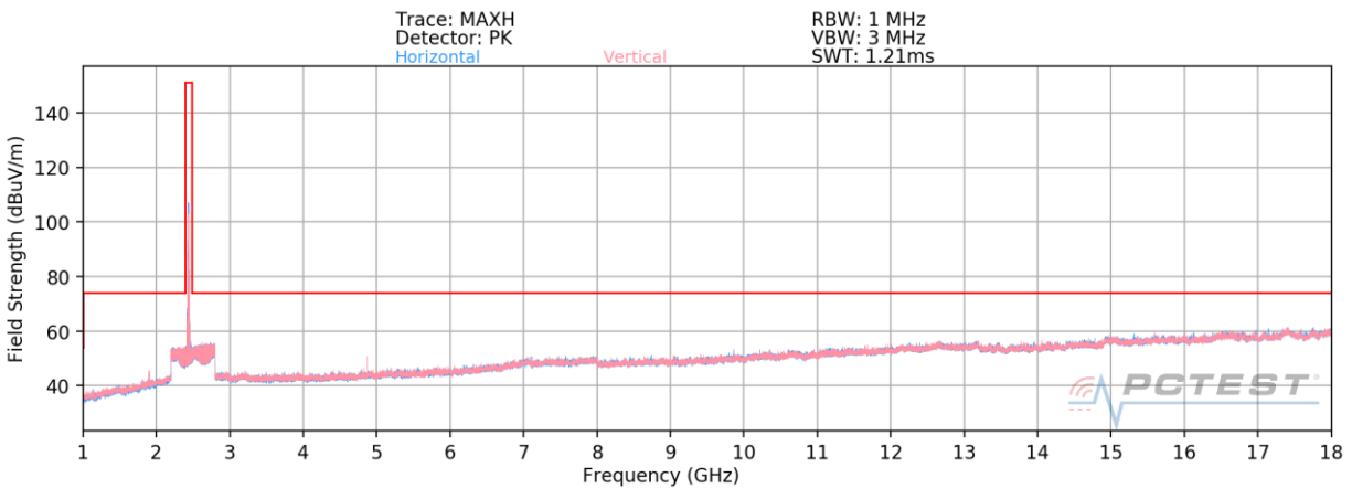
Plot 7-132. Radiated Spurious Plot above 1GHz SISO ANT2 (802.11b – Ch. 6) – OPEN (N)
