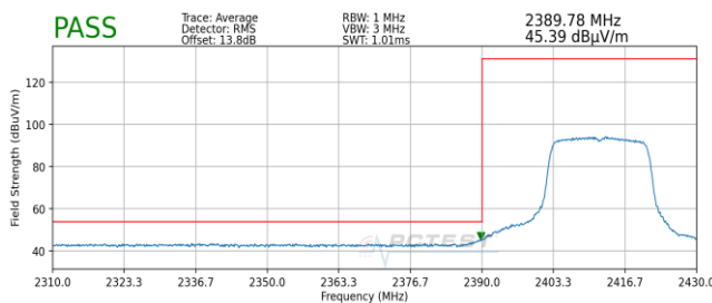
Plot 7-157. Radiated Restricted Lower Band Edge Measurement SISO ANT2 (Average) - Q
