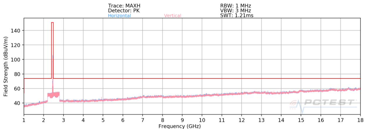
Plot 7-133. Radiated Spurious Plot above 1GHz SISO ANT2 (802.11b – Ch. 11) – OPEN (N)
