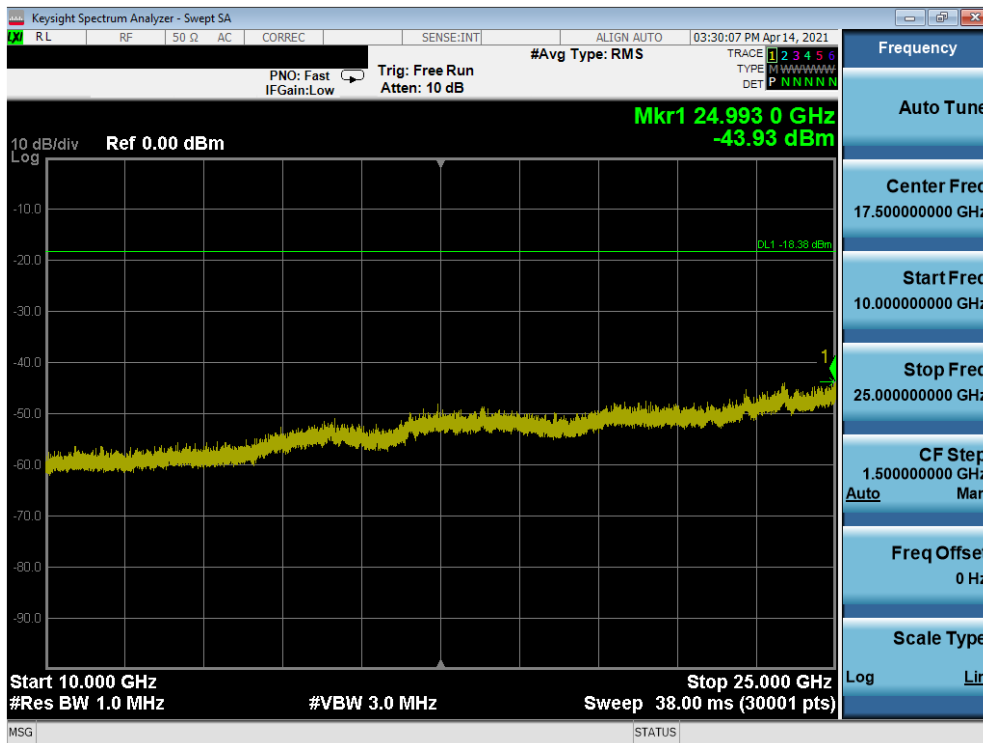
Plot 7-120. Conducted Spurious Plot SISO ANT2 (802.11b – Ch. 1) – N
