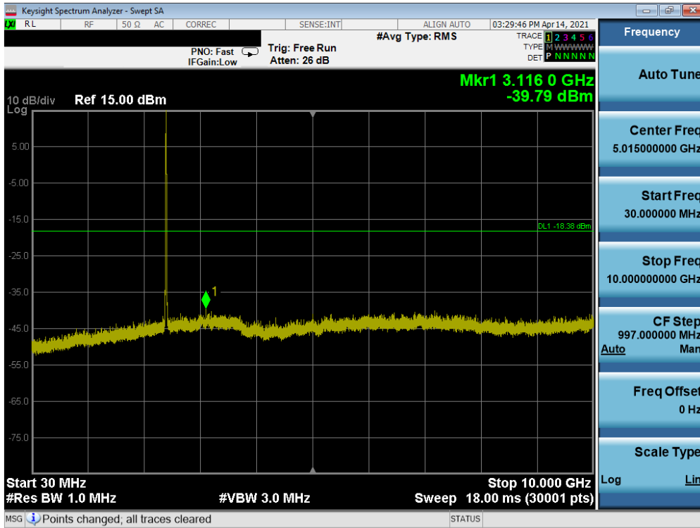
Plot 7-119. Conducted Spurious Plot SISO ANT2 (802.11b – Ch. 1) – N
