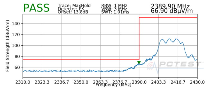
Plot 7-168. Radiated Restricted Lower Band Edge Measurement MIMO (Peak) – N
