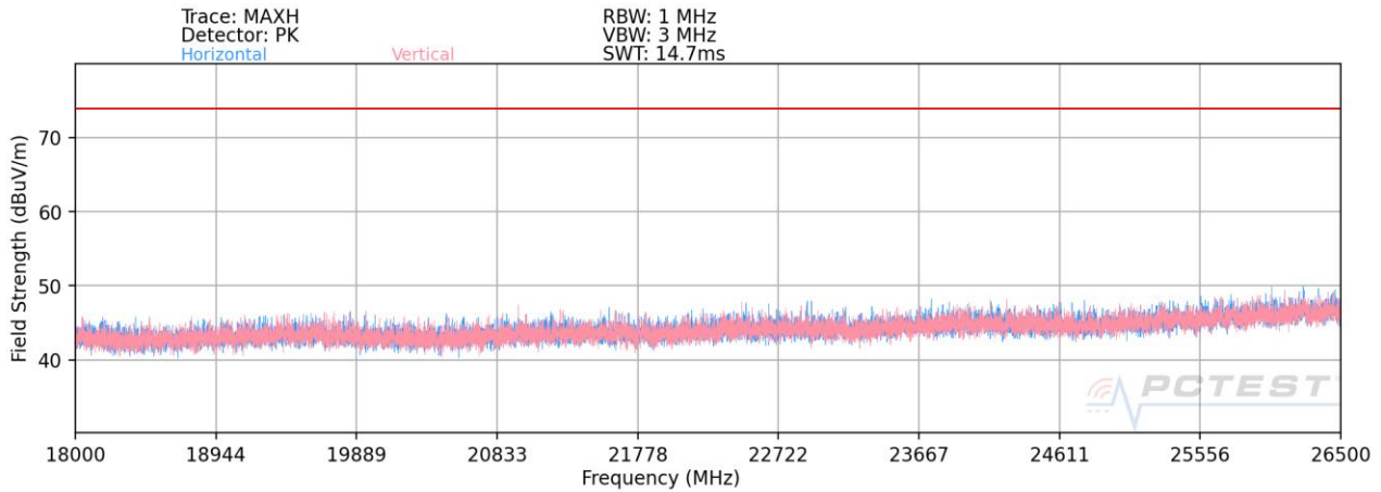
Plot 7-139. Radiated Spurious Plot above 18GHz SISO ANT2– OPEN (N)
