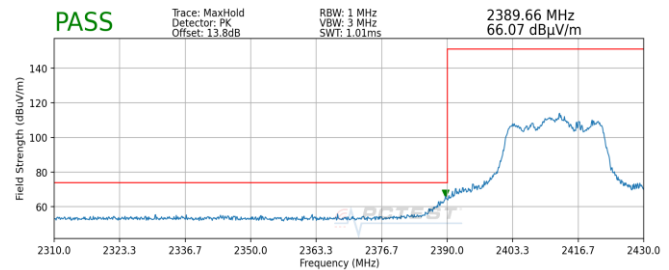
Plot 7-166. Radiated Restricted Lower Band Edge Measurement MIMO (Peak) – Q
