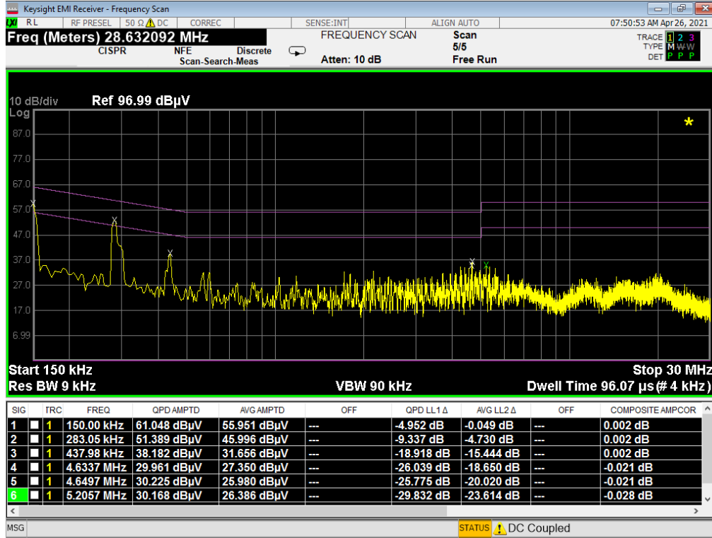
Plot 7-185. Line Conducted Plot with 802.11b (L1) – OPEN (N)
