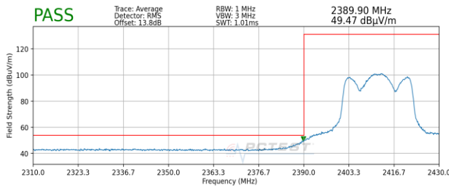
Plot 7-165. Radiated Restricted Lower Band Edge Measurement MIMO (Average) – Q
