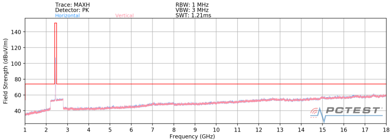
Plot 7-151. Radiated Spurious Plot above 1GHz CDD (802.11b – Ch. 6) – CLOSED (N)
