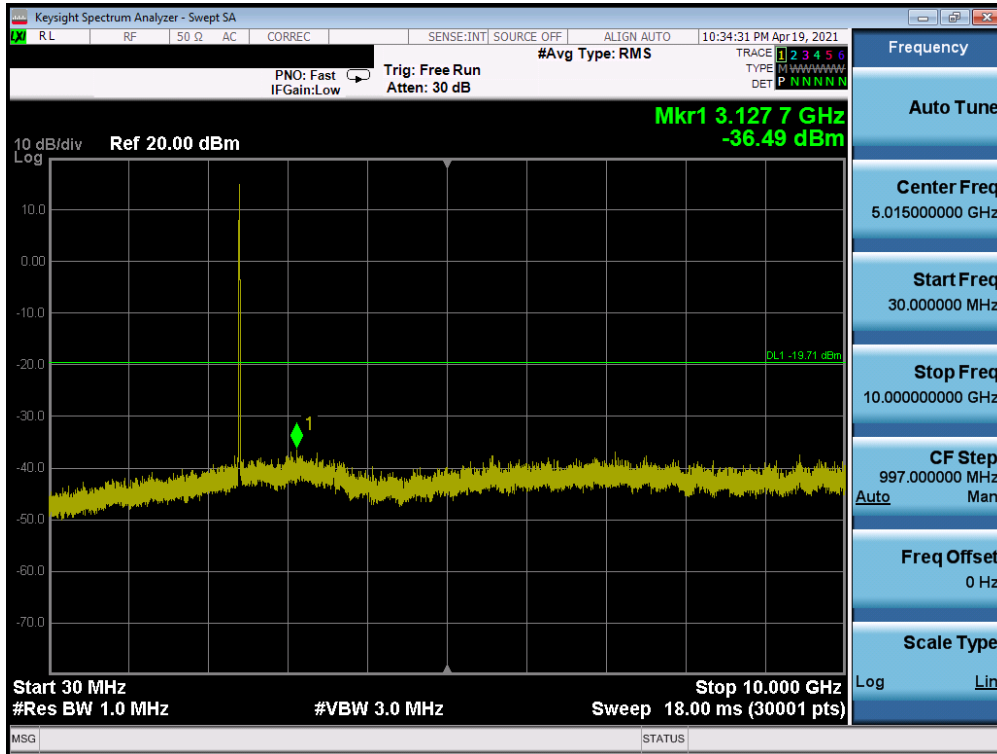
Plot 7-113. Conducted Spurious Plot SISO ANT2 (802.11b – Ch. 1) – Q
