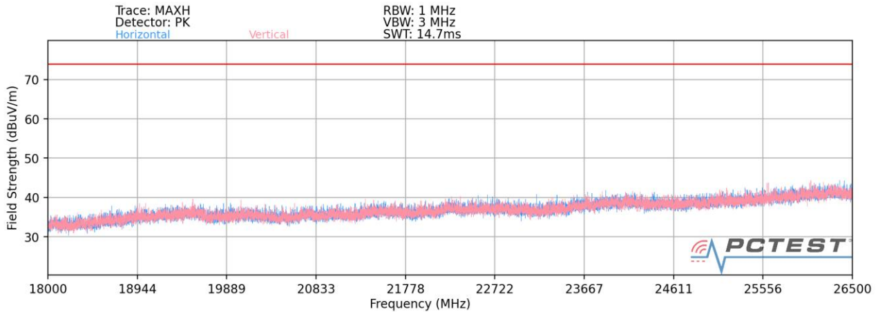
Plot 7-154. Radiated Spurious Plot above 18GHz CDD – CLOSED (Q)
