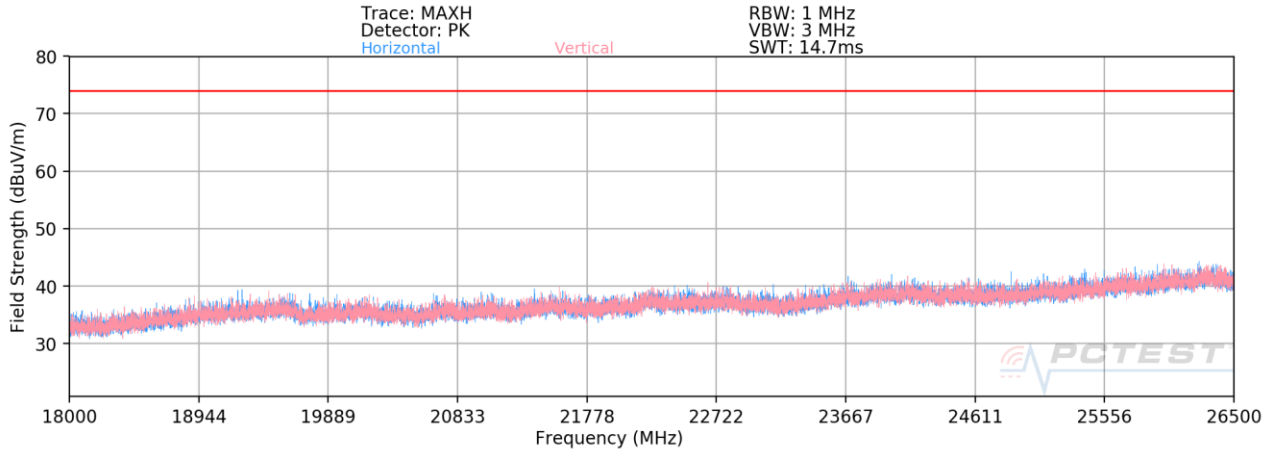
Plot 7-153. Radiated Spurious Plot above 18GHz CDD – OPEN (Q)
