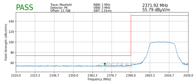
Plot 7-158. Radiated Restricted Lower Band Edge Measurement SISO ANT2 (Peak) - Q
