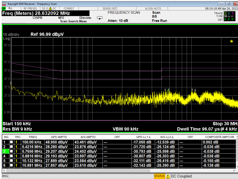
Plot 7-186. Line Conducted Plot with 802.11b (N) – OPEN (N)
