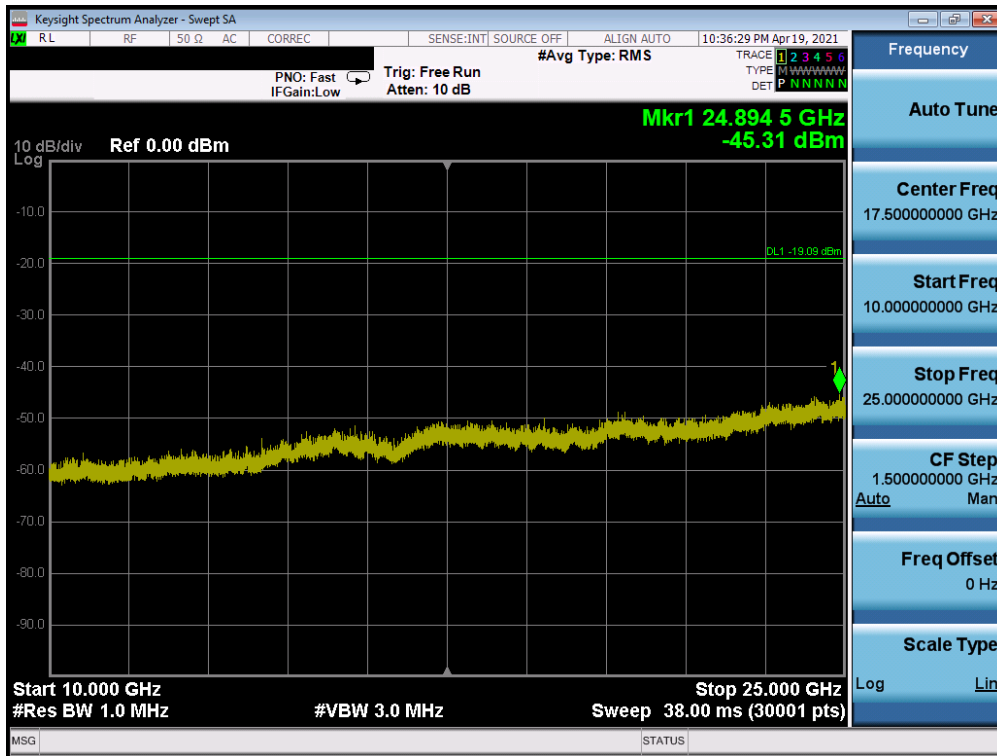
Plot 7-116. Conducted Spurious Plot SISO ANT2 (802.11b – Ch. 6) – Q
