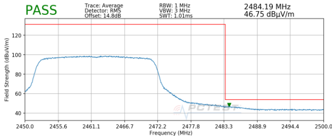
Plot 7-163. Radiated Restricted Upper Band Edge Measurement SISO ANT2 (Average) - N
