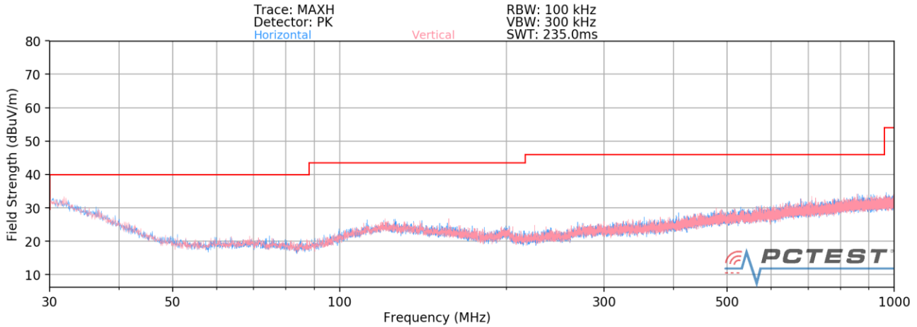
Plot 7-178. Radiated Spurious Plot below 1GHz MIMO – CLOSED (Q)
