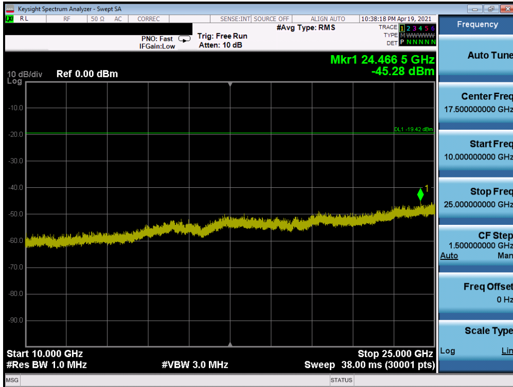
Plot 7-118. Conducted Spurious Plot SISO ANT2 (802.11b – Ch. 11) – Q
