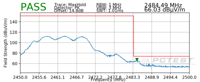
Plot 7-172. Radiated Restricted Upper Band Edge Measurement MIMO (Peak) – N
