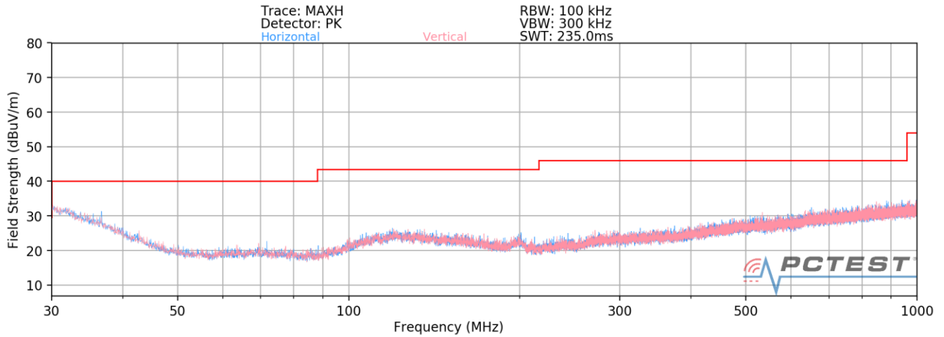
Plot 7-180. Radiated Spurious Plot below 1GHz MIMO – CLOSED (N)
