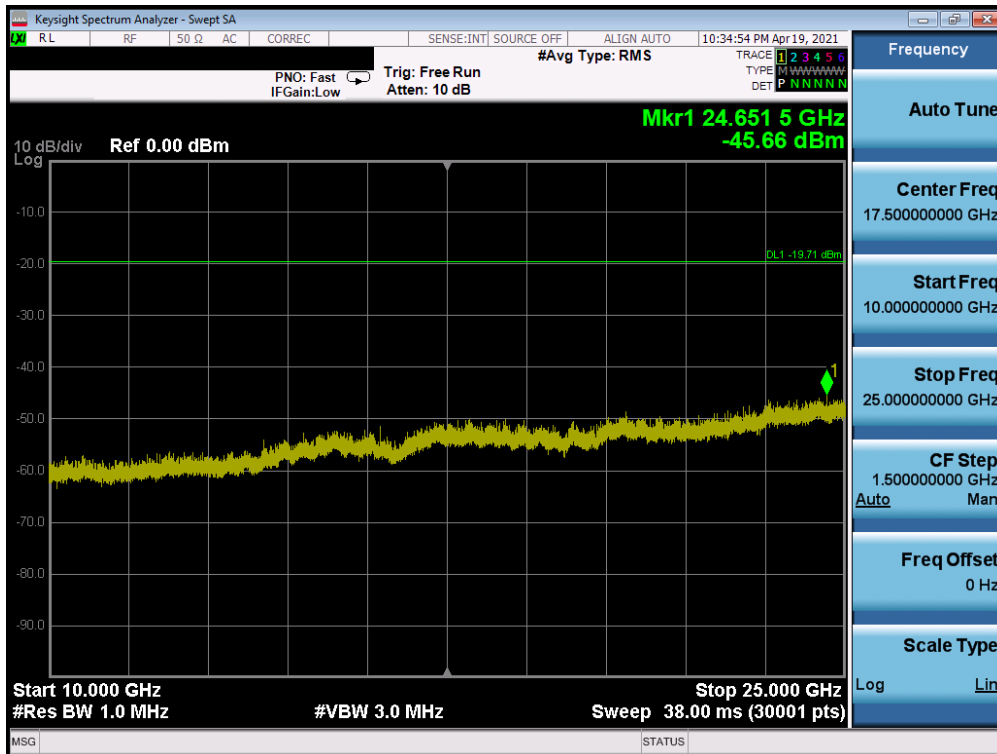
Plot 7-114. Conducted Spurious Plot SISO ANT2 (802.11b – Ch. 1) – Q
