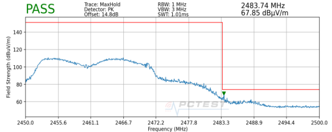
Plot 7-170. Radiated Restricted Upper Band Edge Measurement MIMO (Peak) – Q
