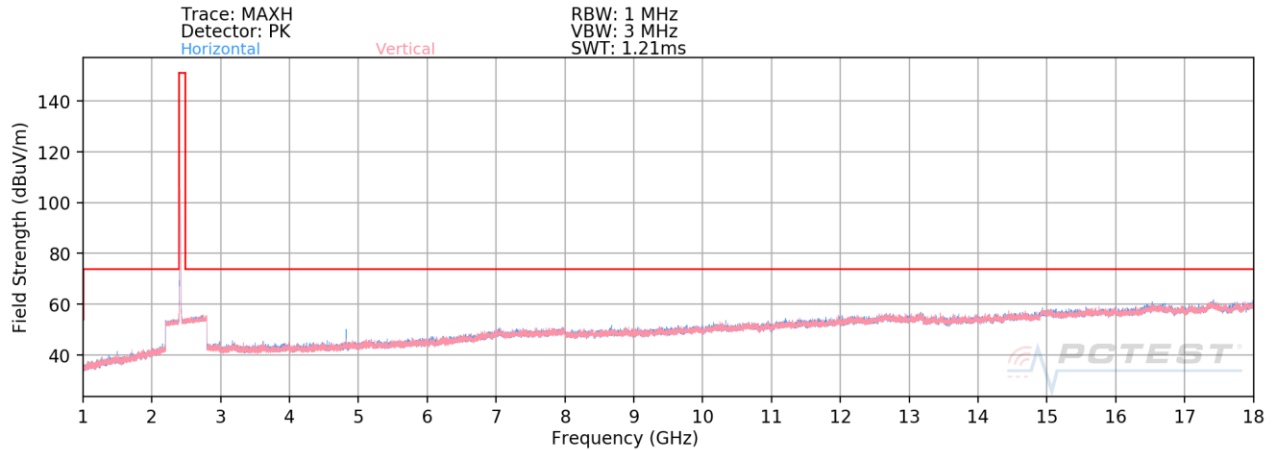
Plot 7-147. Radiated Spurious Plot above 1GHz CDD (802.11b – Ch. 1) – OPEN (N)
