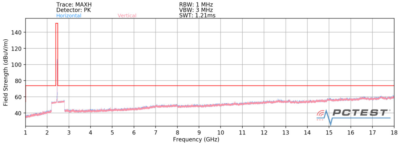
Plot 7-152. Radiated Spurious Plot above 1GHz CDD (802.11b – Ch. 11) – CLOSED (N)
