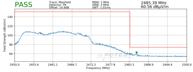
Plot 7-174. Radiated Restricted Band Edge Measurement MIMO with WCP (Peak) – Q
