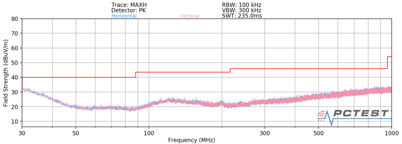
Plot 7-179. Radiated Spurious Plot below 1GHz MIMO – OPEN (N)
