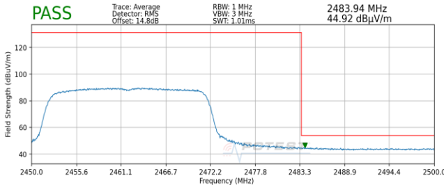
Plot 7-161. Radiated Restricted Upper Band Edge Measurement SISO ANT2 (Average) - Q
