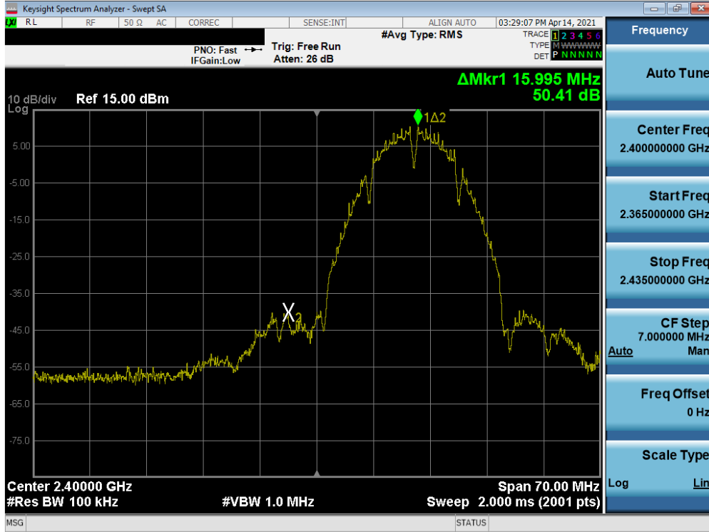
Plot 7-105. Band Edge Plot SISO ANT2 (802.11b – Ch. 1) – N
