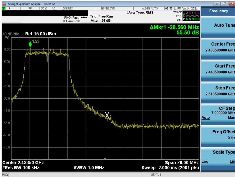
Plot 7-108. Band Edge Plot SISO ANT2 (802.11g - Ch. 11) – N
