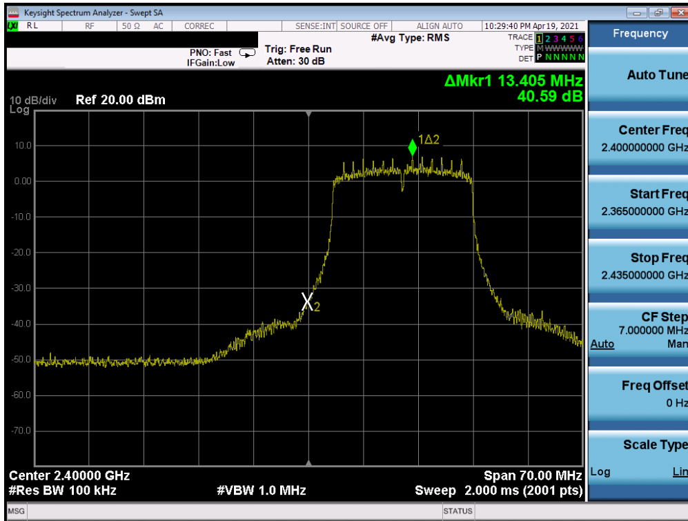
Plot 7-101. Band Edge Plot SISO ANT2 (802.11n (2.4GHz) – Ch. 1) – Q
