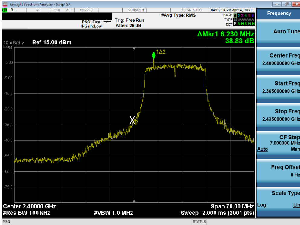
Plot 7-109. Band Edge Plot SISO ANT2 (802.11n (2.4GHz) – Ch. 1) – N
