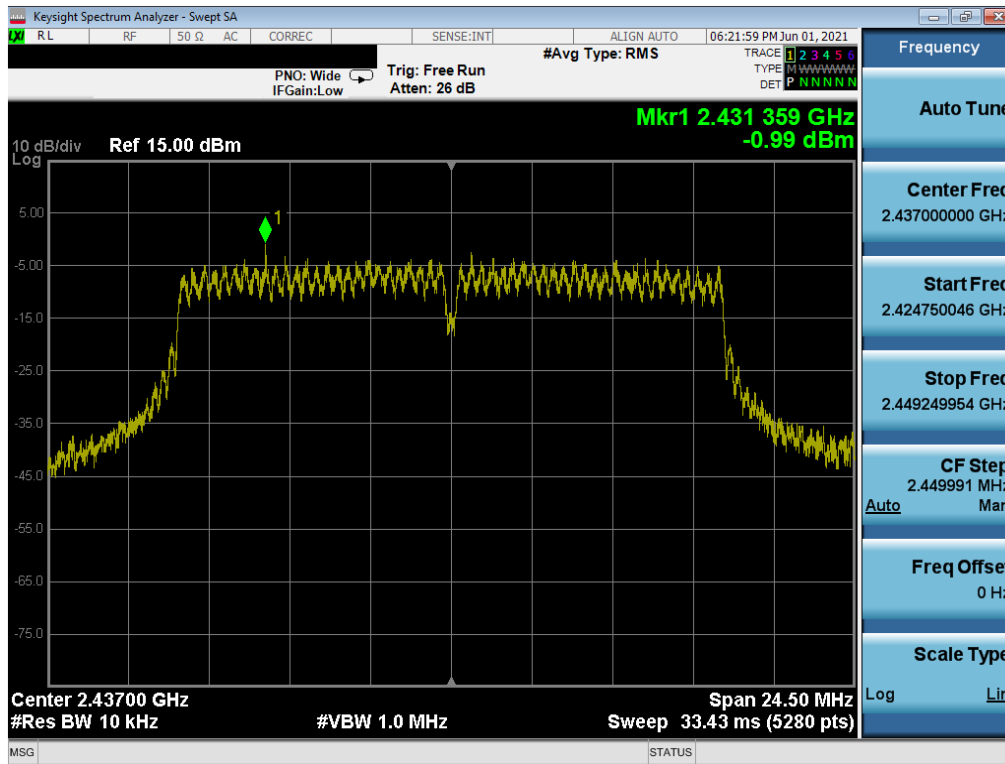
Plot 7-65. Power Spectral Density Plot MIMO ANT2 (802.11g – Ch. 6) – Q
