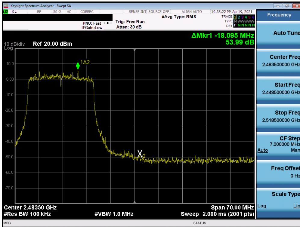
Plot 7-104. Band Edge Plot SISO ANT2 (802.11ax (2.4GHz) – Ch. 11) – Q
