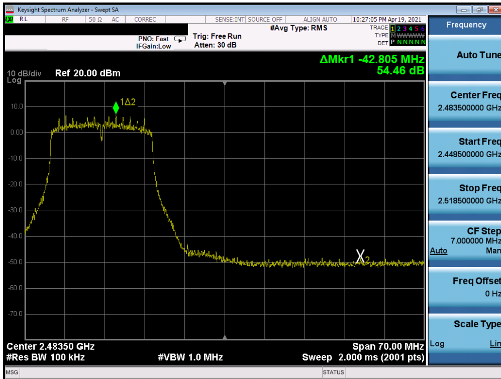
Plot 7-102. Band Edge Plot SISO ANT2 (802.11n (2.4GHz) – Ch. 11) – Q
