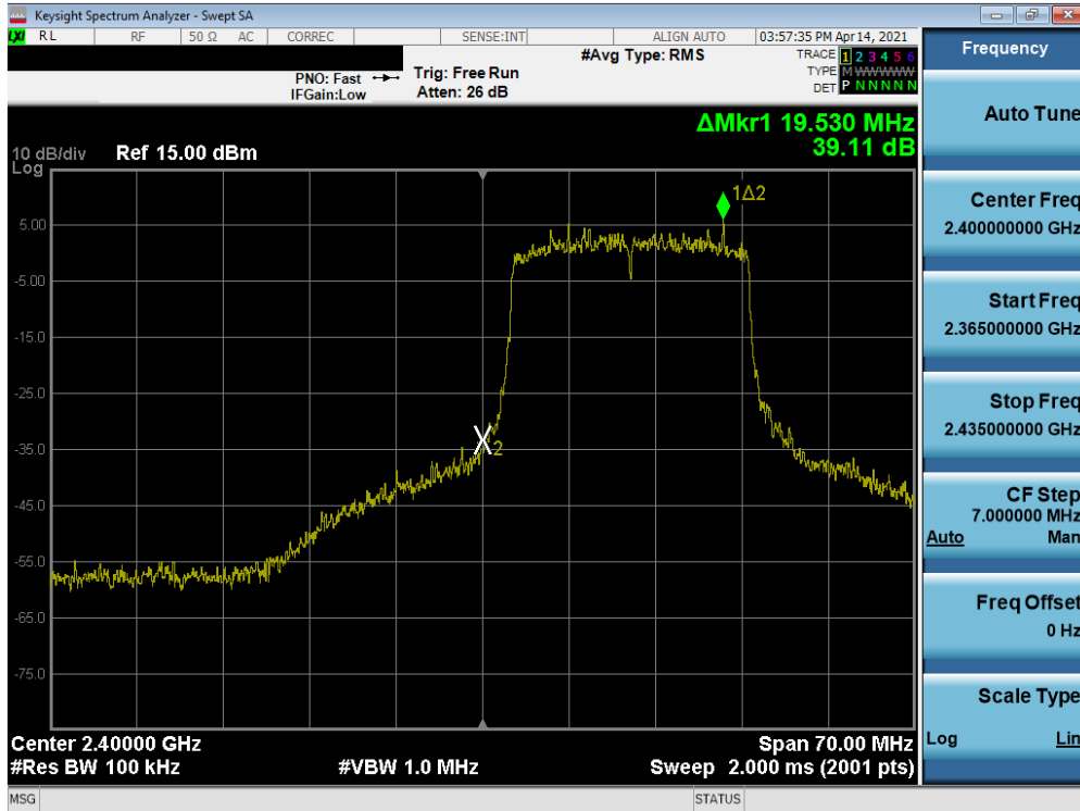
Plot 7-111. Band Edge Plot SISO ANT2 (802.11ax (2.4GHz) – Ch. 1) – N
