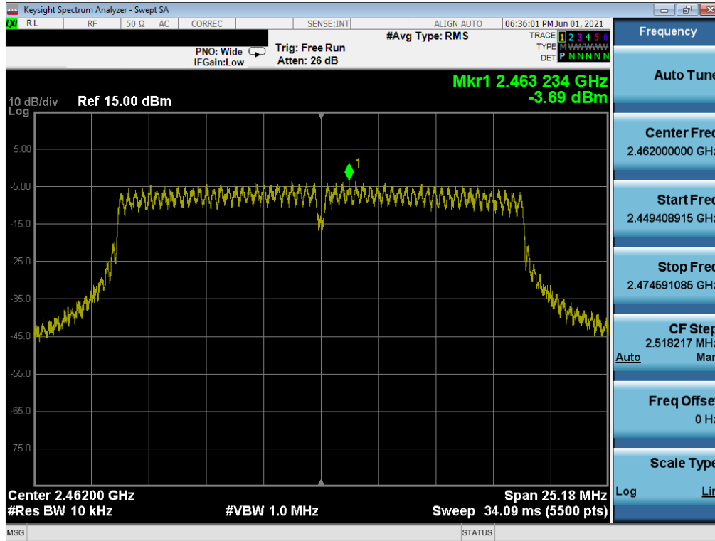
Plot 7-54. Power Spectral Density Plot MIMO ANT1 (802.11g – Ch. 11) – Q
