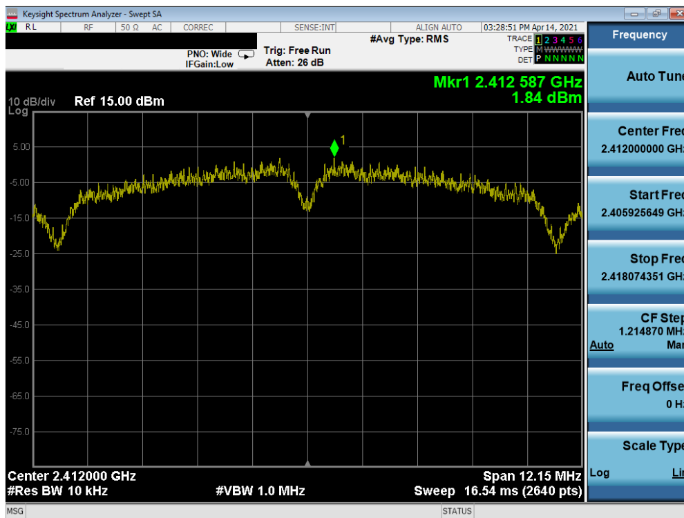
Plot 7-37. Power Spectral Density Plot SISO ANT2 (802.11b – Ch. 1) – N
