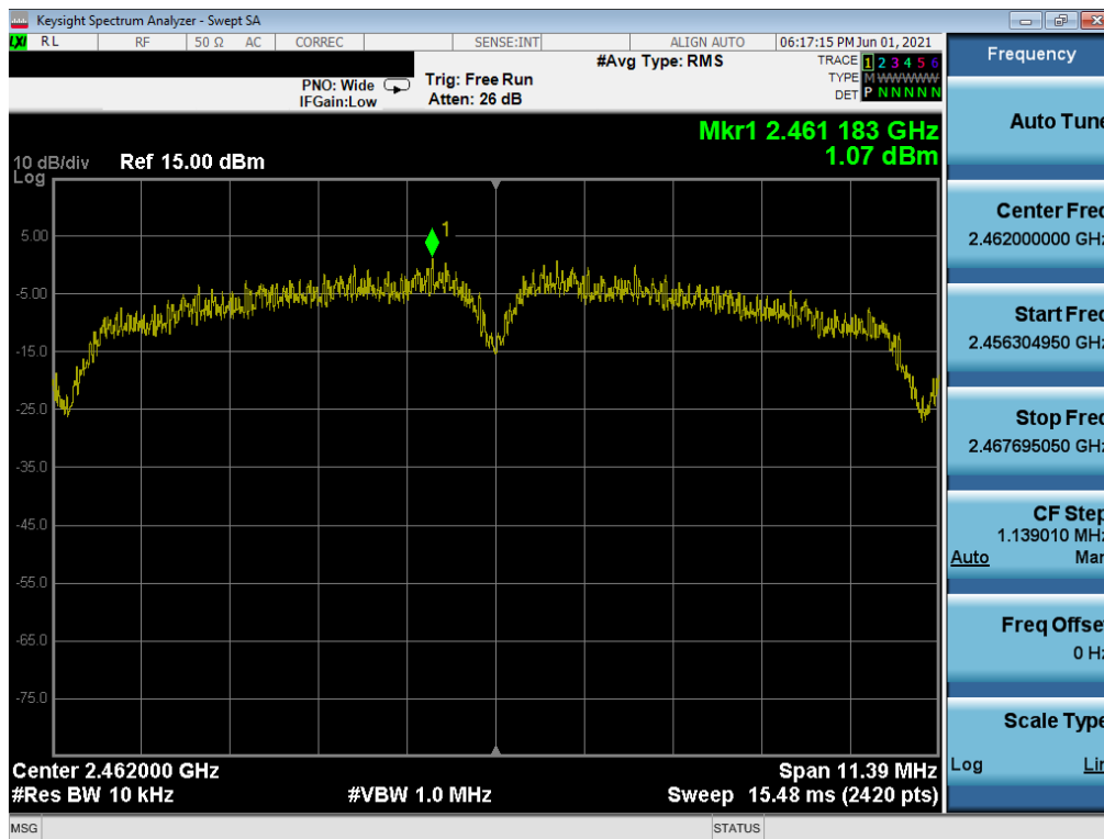
Plot 7-63. Power Spectral Density Plot MIMO ANT2 (802.11b – Ch. 11) – Q
