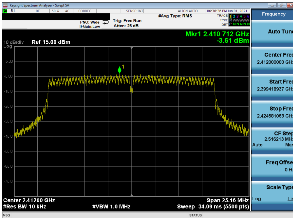
Plot 7-55. Power Spectral Density Plot MIMO ANT1 (802.11n – Ch. 1) – Q
