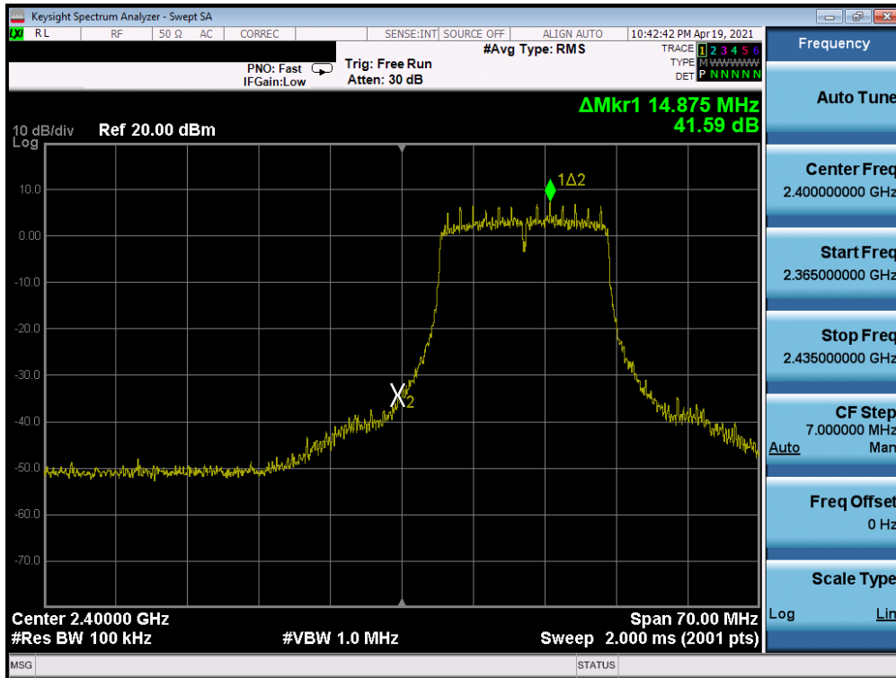
Plot 7-99. Band Edge Plot SISO ANT2 (802.11g- Ch. 1) – Q
