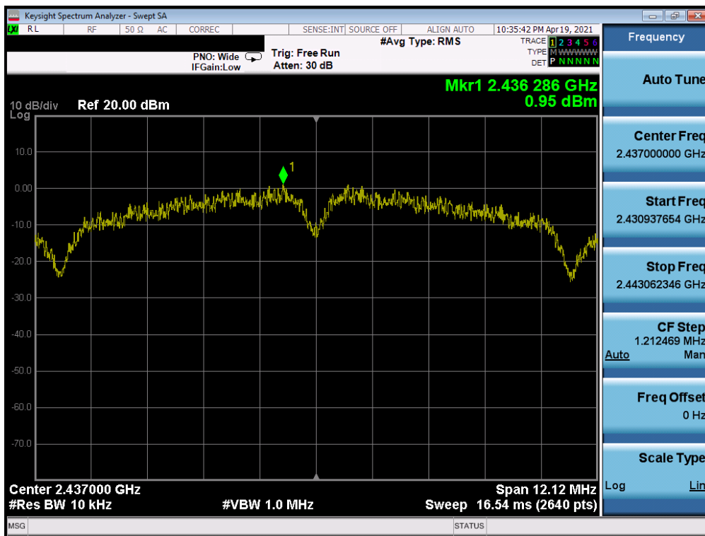
Plot 7-26. Power Spectral Density Plot SISO ANT2 (802.11b – Ch. 6) – Q
