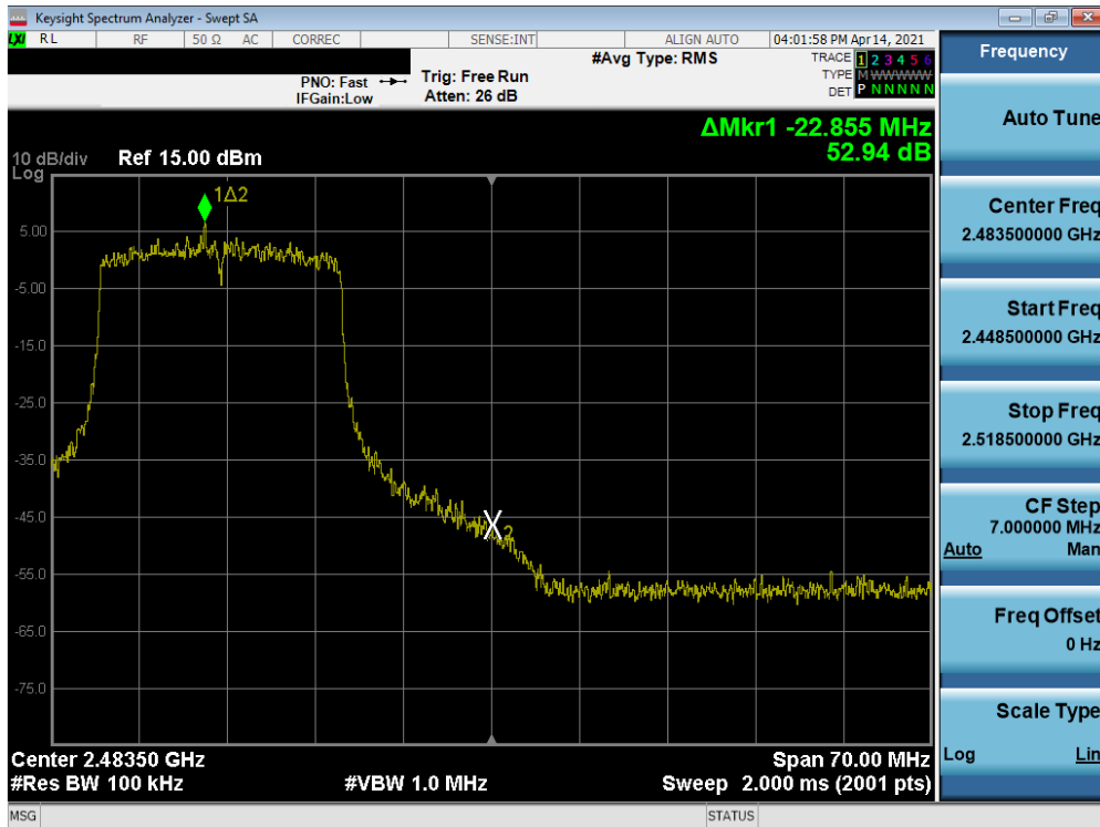
Plot 7-112. Band Edge Plot SISO ANT2 (802.11ax (2.4GHz) – Ch. 11) – N
