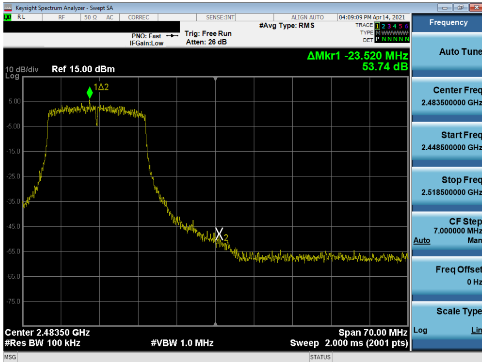
Plot 7-110. Band Edge Plot SISO ANT2 (802.11n (2.4GHz) – Ch. 11) – N
