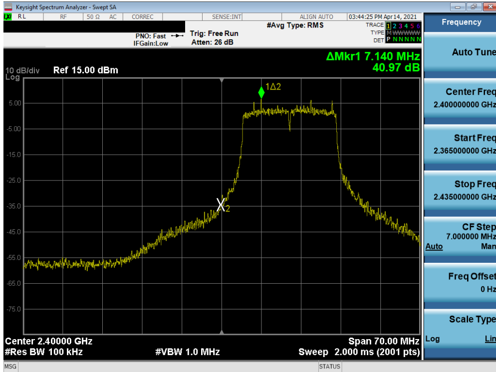
Plot 7-107. Band Edge Plot SISO ANT2 (802.11g- Ch. 1) – N
