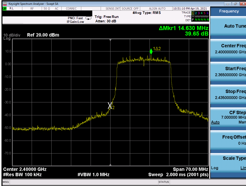
Plot 7-103. Band Edge Plot SISO ANT2 (802.11ax (2.4GHz) – Ch. 1) – Q
