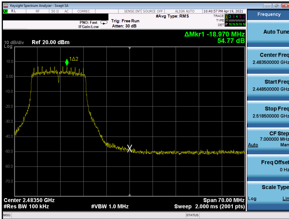
Plot 7-100. Band Edge Plot SISO ANT2 (802.11g - Ch. 11) – Q
