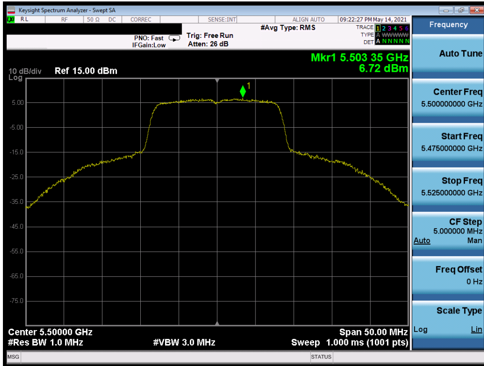
Plot 7-559. Power Spectral Density Plot MIMO ANT1 (20MHz BW 802.11a (UNII Band 2C) – Ch. 100)
