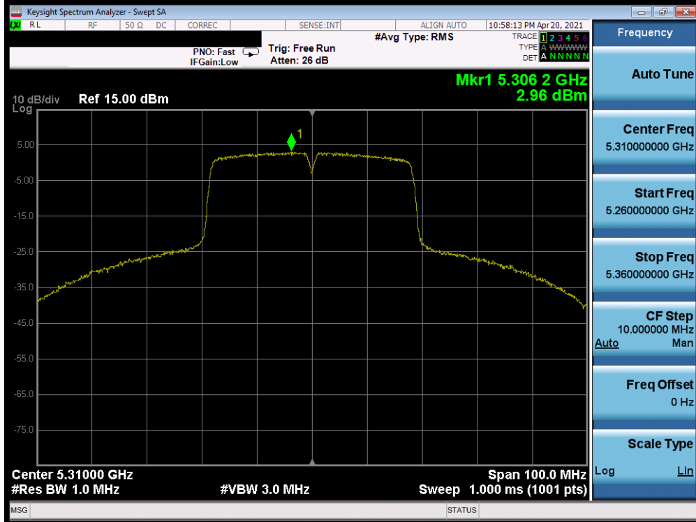
Plot 7-488. Power Spectral Density Plot SISO ANT1 (40MHz BW 802.11n (UNII Band 2A) – Ch. 62)
