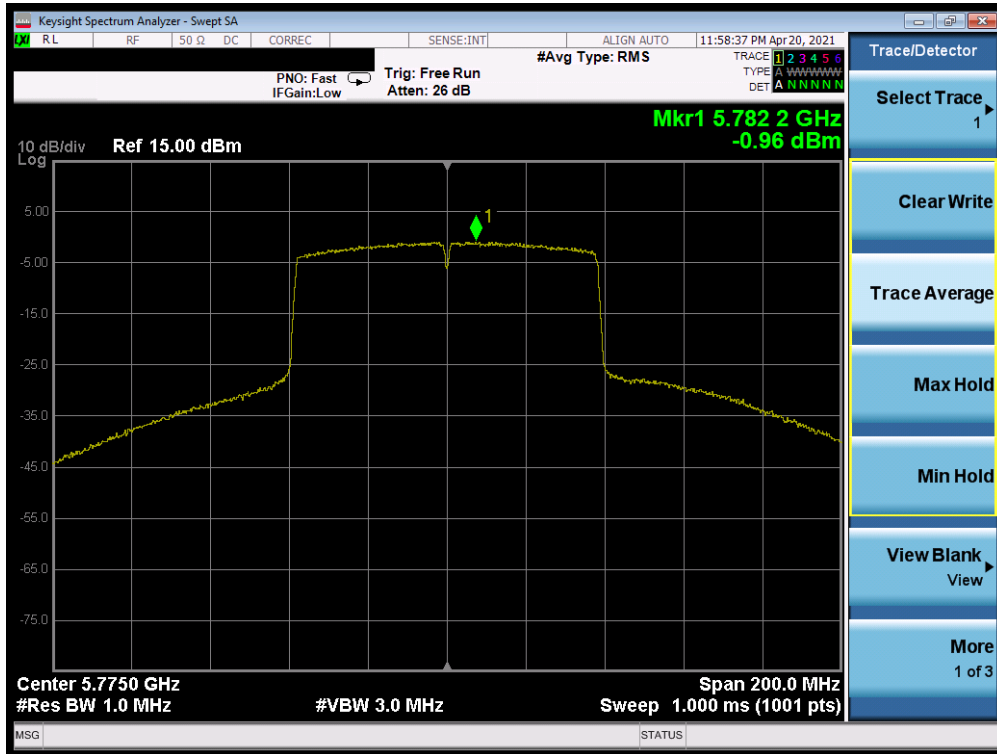
Plot 7-527. Power Spectral Density Plot SISO ANT1 (80MHz BW 802.11ac (UNII Band 3) – Ch. 155)
