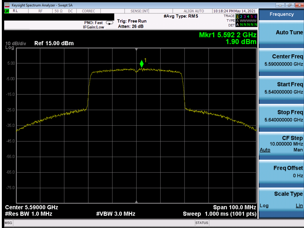
Plot 7-572. Power Spectral Density Plot MIMO ANT1 (40MHz BW 802.11ax (UNII Band 2C) – Ch. 118)
