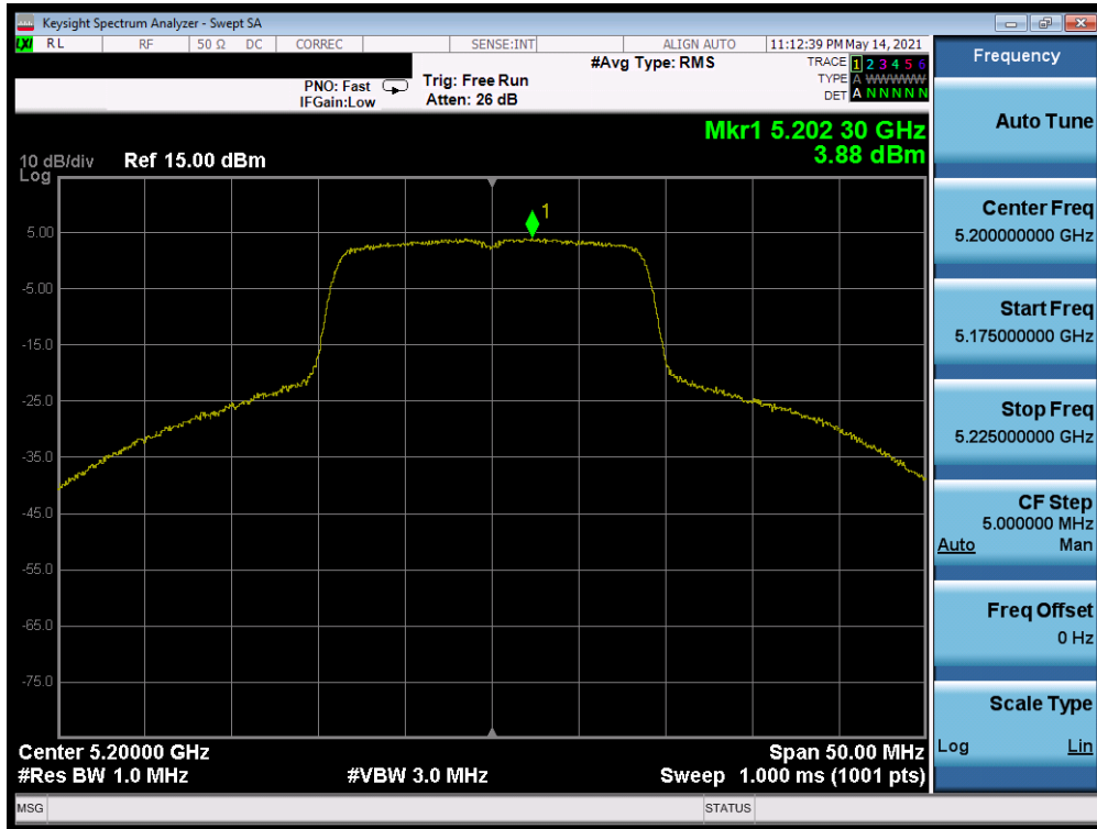
Plot 7-584. Power Spectral Density Plot MIMO ANT2 (20MHz BW 802.11n (UNII Band 1) – Ch. 40)
