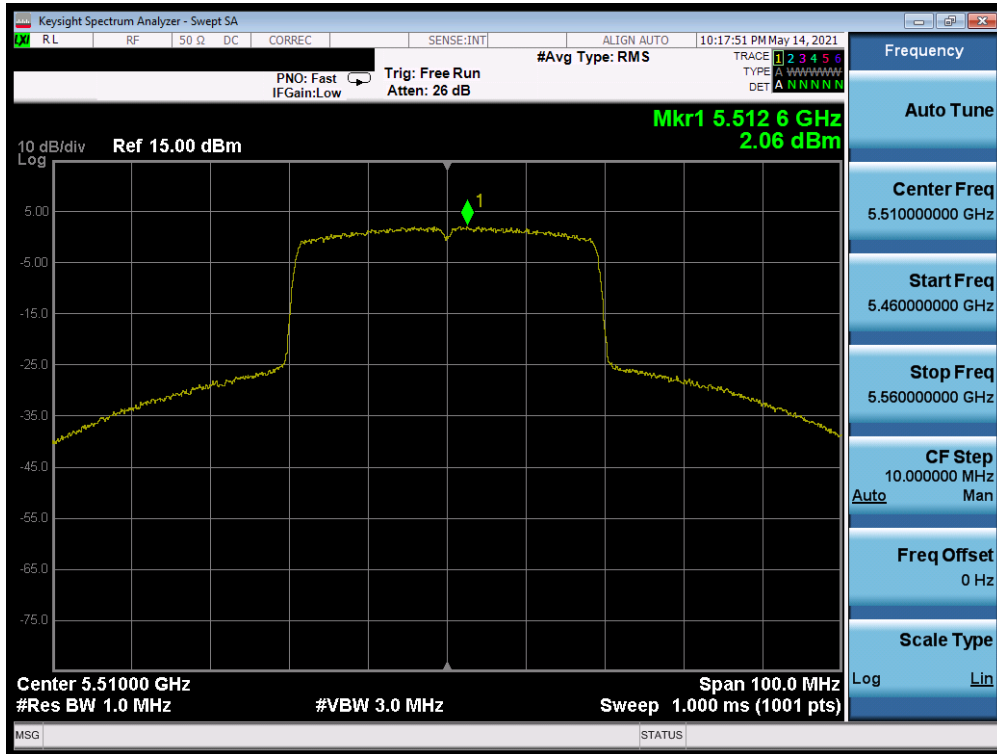
Plot 7-571. Power Spectral Density Plot MIMO ANT1 (40MHz BW 802.11ax (UNII Band 2C) – Ch. 102)
