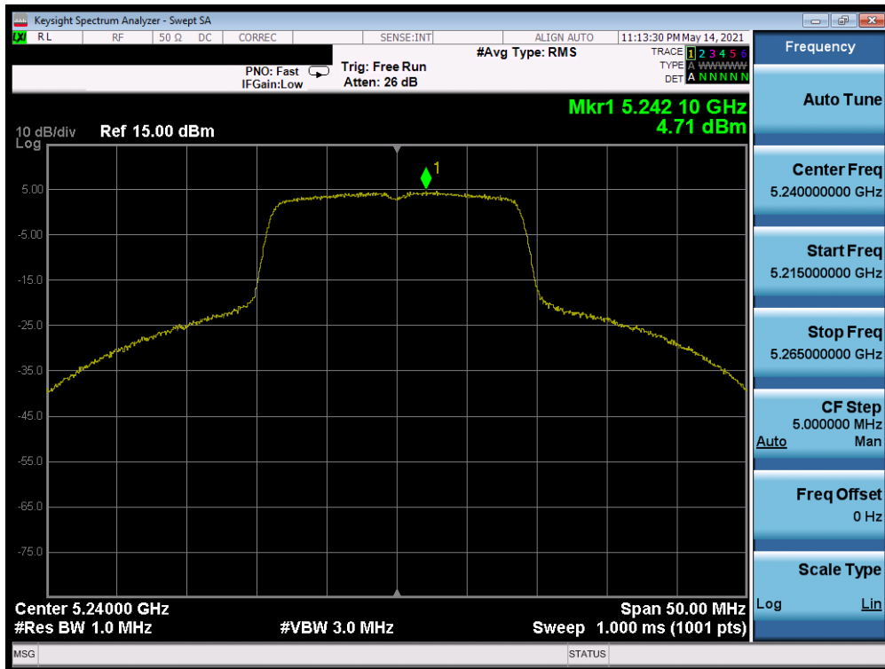
Plot 7-585. Power Spectral Density Plot MIMO ANT2 (20MHz BW 802.11n (UNII Band 1) – Ch. 48)
