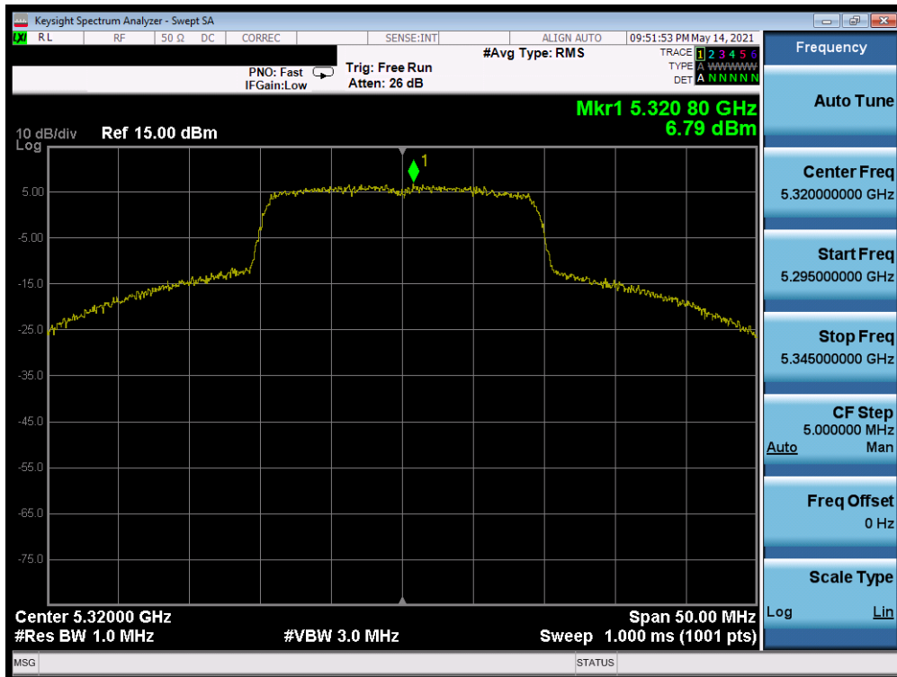
Plot 7-552. Power Spectral Density Plot MIMO ANT1 (20MHz BW 802.11ax (UNII Band 2A) – Ch. 64)
