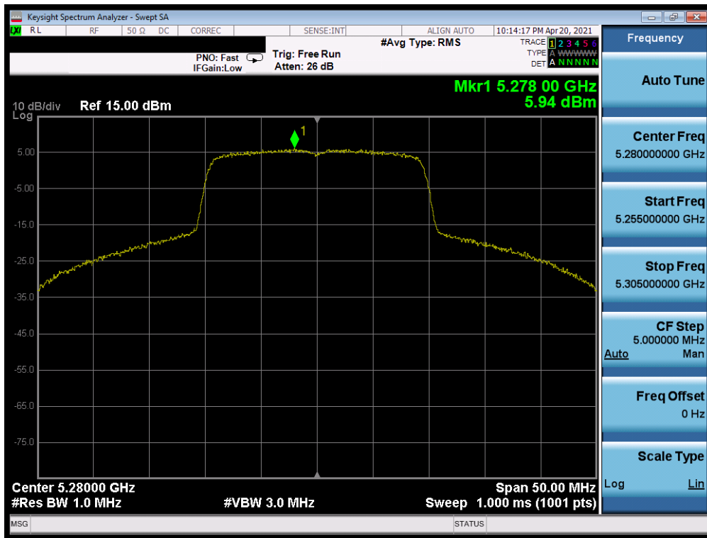
Plot 7-485. Power Spectral Density Plot SISO ANT1 (20MHz BW 802.11ax (UNII Band 2A) – Ch. 56)
