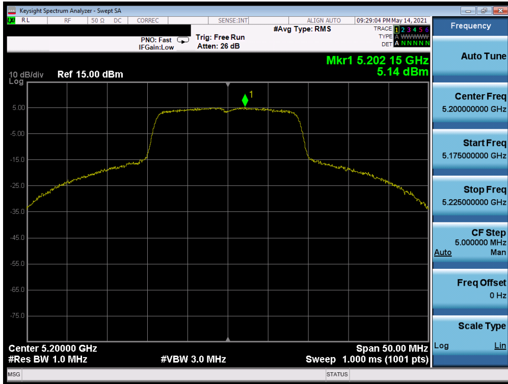
Plot 7-533. Power Spectral Density Plot MIMO ANT1 (20MHz BW 802.11n (UNII Band 1) – Ch. 40)
