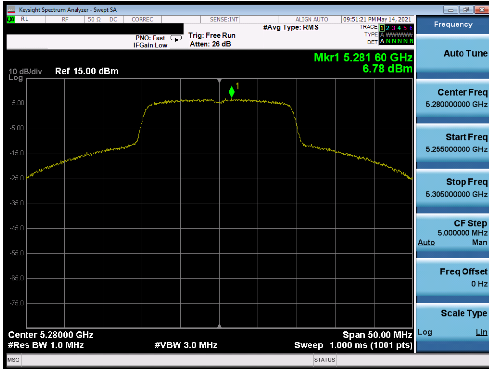
Plot 7-551. Power Spectral Density Plot MIMO ANT1 (20MHz BW 802.11ax (UNII Band 2A) – Ch. 56)
