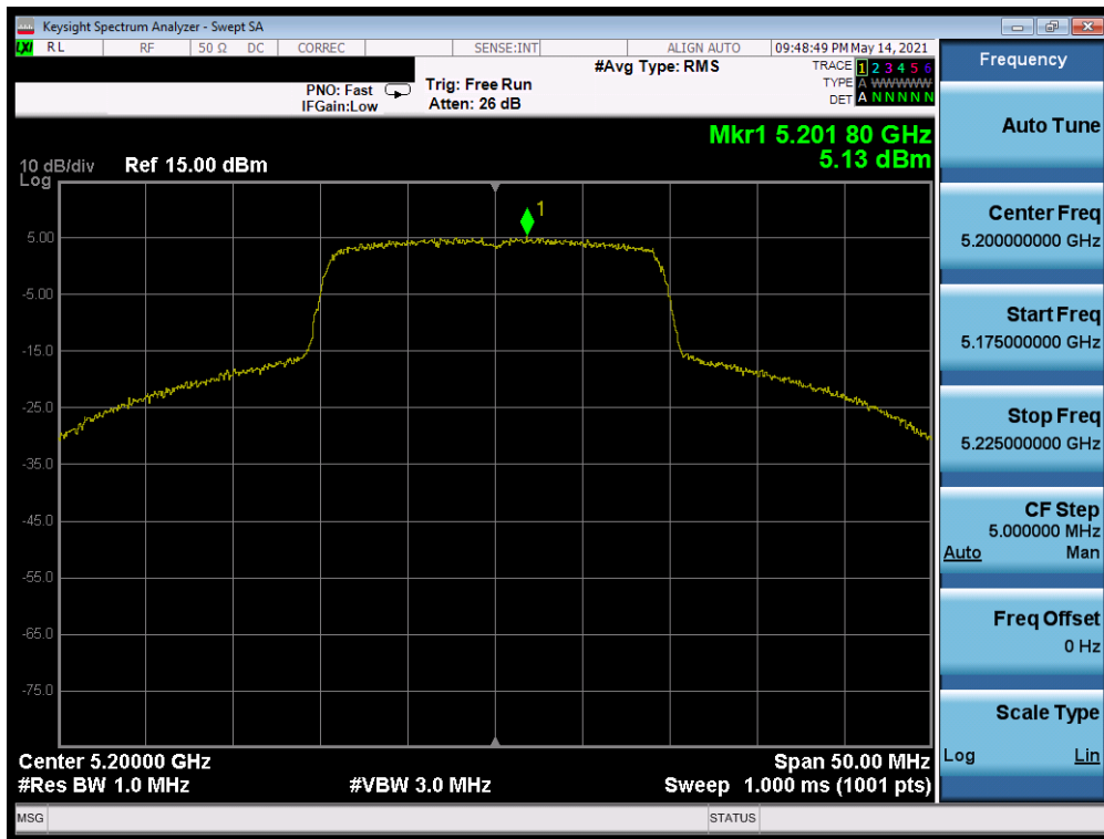
Plot 7-536. Power Spectral Density Plot MIMO ANT1 (20MHz BW 802.11ax (UNII Band 1) – Ch. 40)
