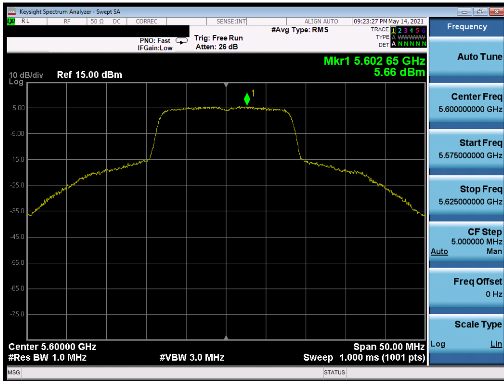
Plot 7-560. Power Spectral Density Plot MIMO ANT1 (20MHz BW 802.11a (UNII Band 2C) – Ch. 120)
