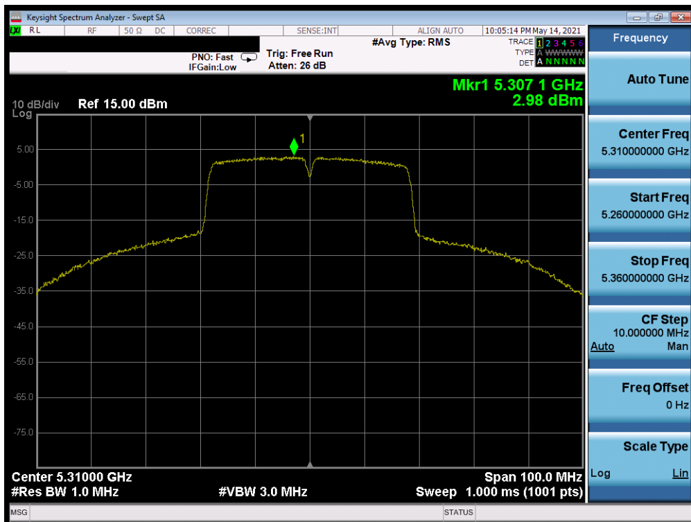
Plot 7-554. Power Spectral Density Plot MIMO ANT1 (40MHz BW 802.11n (UNII Band 2A) – Ch. 62)
