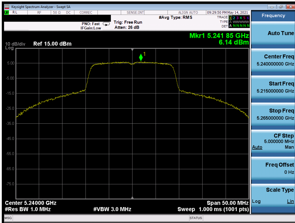
Plot 7-534. Power Spectral Density Plot MIMO ANT1 (20MHz BW 802.11n (UNII Band 1) – Ch. 48)
