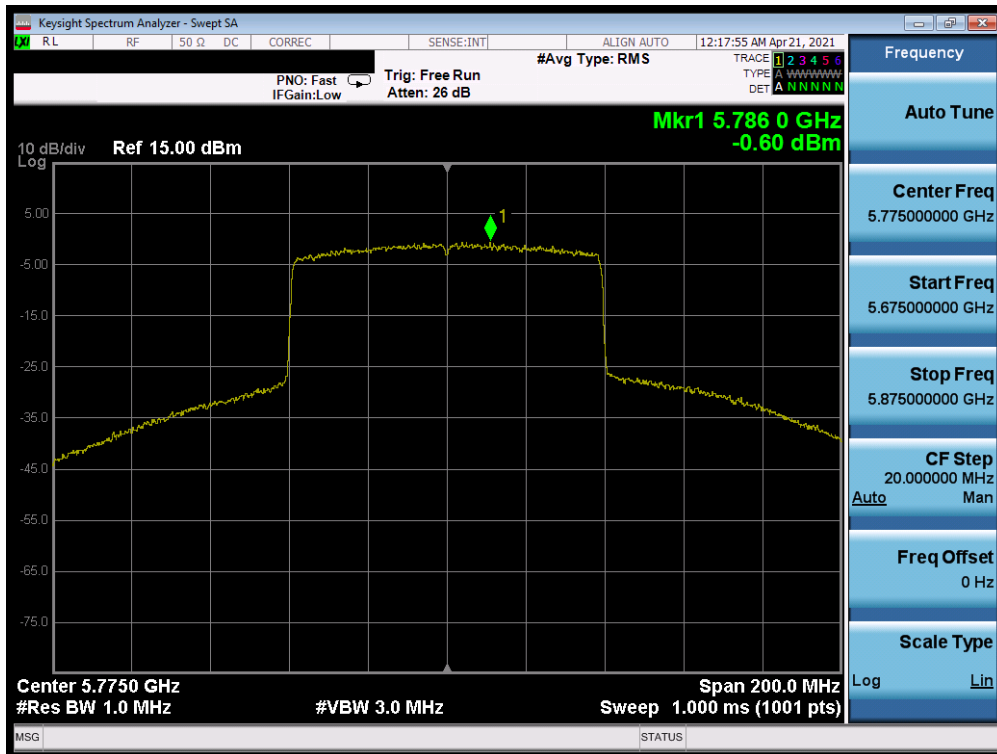
Plot 7-528. Power Spectral Density Plot SISO ANT1 (80MHz BW 802.11ax (UNII Band 3) – Ch. 155)
