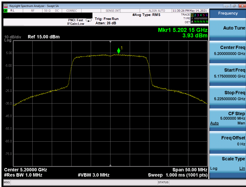
Plot 7-587. Power Spectral Density Plot MIMO ANT2 (20MHz BW 802.11ax (UNII Band 1) – Ch. 40)
