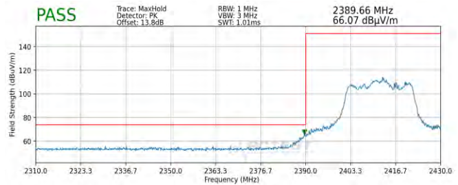
Plot 7-96. Radiated Restricted Lower Band Edge Measurement MIMO (Peak)
