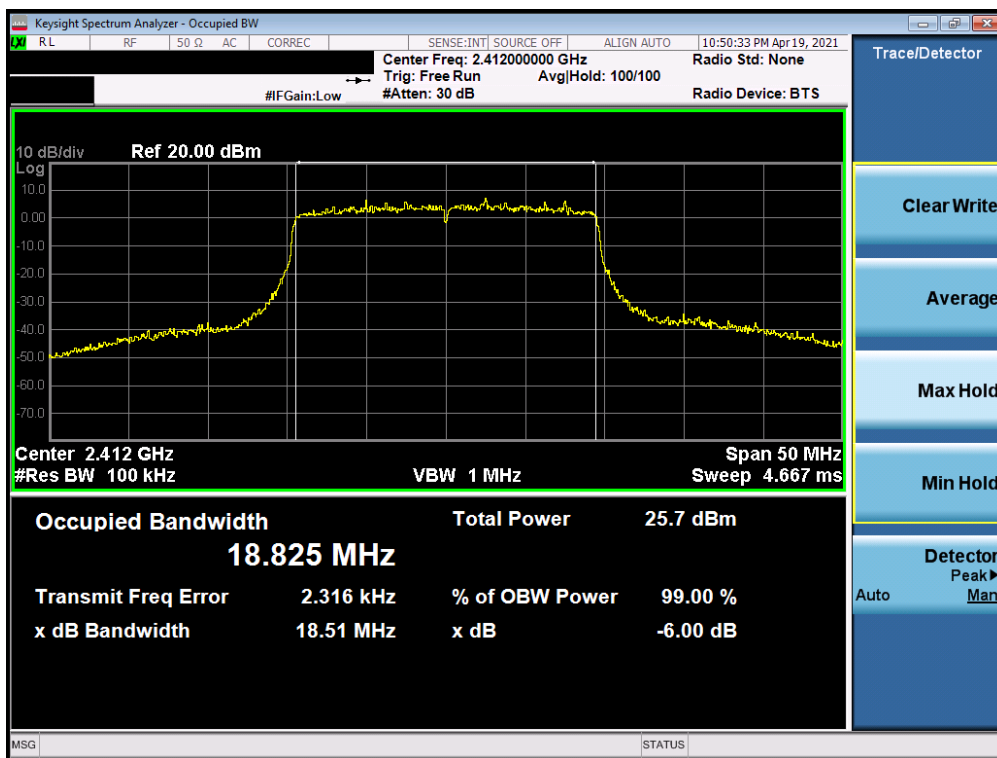
Plot 7-10. 6dB Bandwidth Plot SISO ANT2 (802.11ax (2.4GHz) – Ch. 1)
