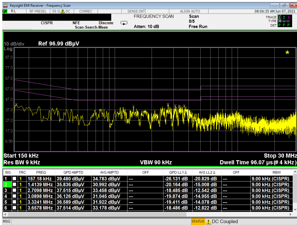
Plot 7-110. Line Conducted Plot with 802.11b (N) with WCP
