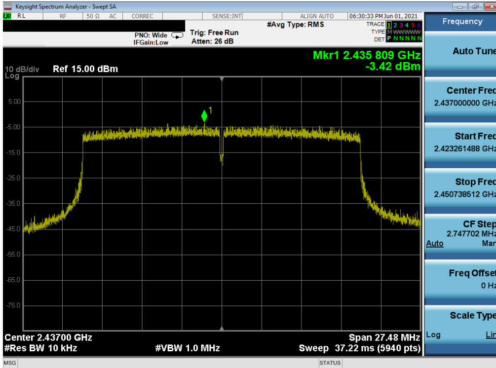
Plot 7-47. Power Spectral Density Plot MIMO ANT2 (802.11ax – Ch. 6)
