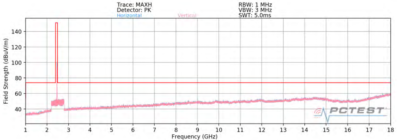
Plot 7-76. Radiated Spurious Plot above 1GHz SISO ANT2 (802.11b – Ch. 11) – CLOSED
