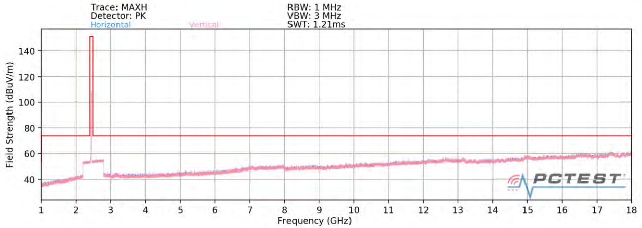
Plot 7-83. Radiated Spurious Plot above 1GHz CDD (802.11b – Ch. 6) – CLOSED
