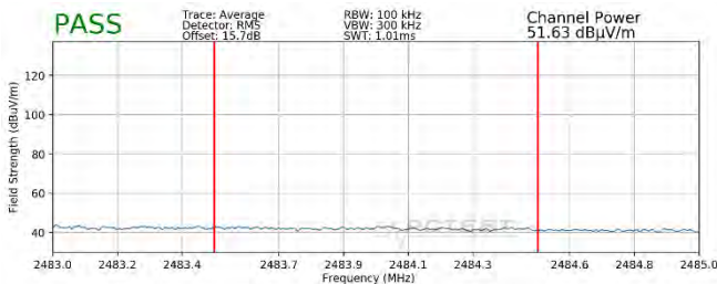
Plot 7-101. Radiated Restricted Upper Band Edge Measurement MIMO (Average)
