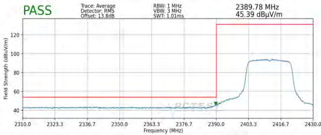
Plot 7-87. Radiated Restricted Lower Band Edge Measurement SISO ANT2 (Average)
