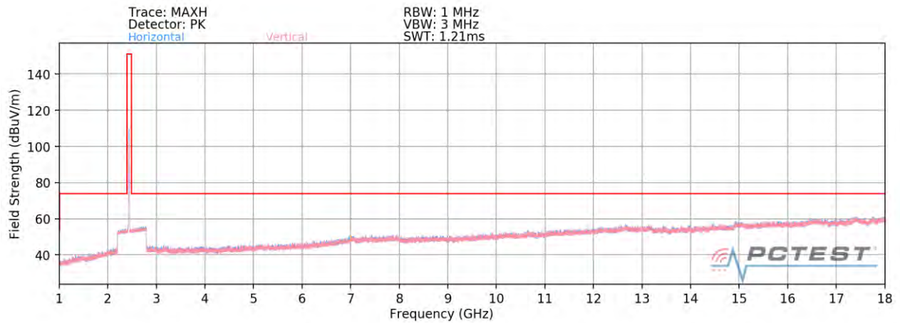
Plot 7-80. Radiated Spurious Plot above 1GHz CDD (802.11b – Ch. 6) – OPEN
