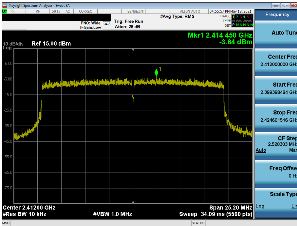
Plot 7-34. Power Spectral Density Plot MIMO ANT1 (802.11ax – Ch. 1)
