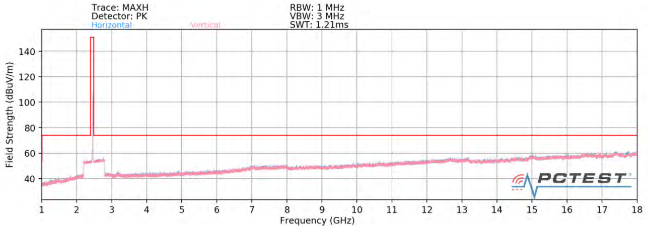
Plot 7-84. Radiated Spurious Plot above 1GHz CDD (802.11b – Ch. 11) – CLOSED
