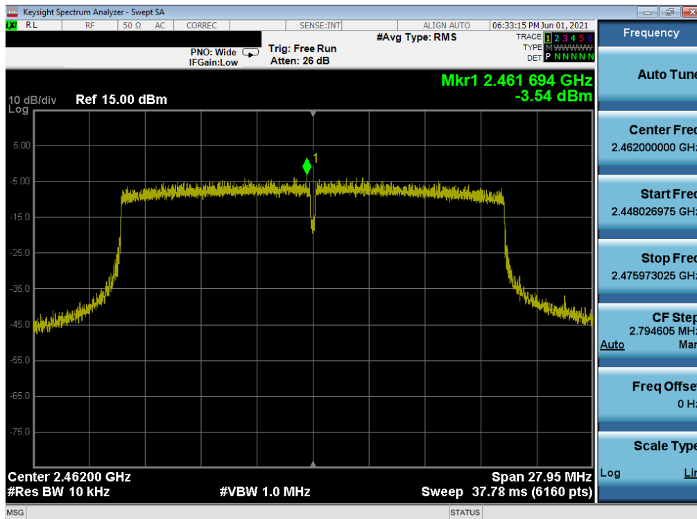
Plot 7-36. Power Spectral Density Plot MIMO ANT1 (802.11ax – Ch. 11)
