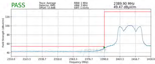
Plot 7-95. Radiated Restricted Lower Band Edge Measurement MIMO (Average)
