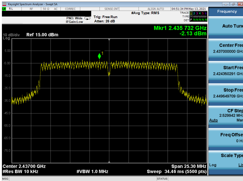
Plot 7-32. Power Spectral Density Plot MIMO ANT1 (802.11n – Ch. 6)
