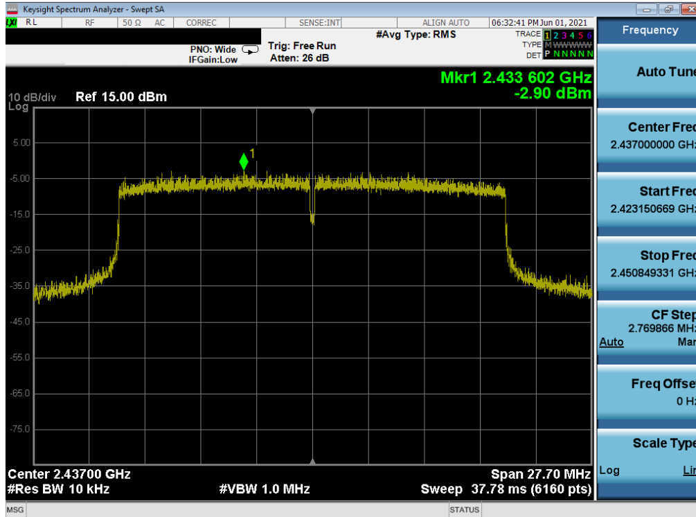
Plot 7-35. Power Spectral Density Plot MIMO ANT1 (802.11ax – Ch. 6)
