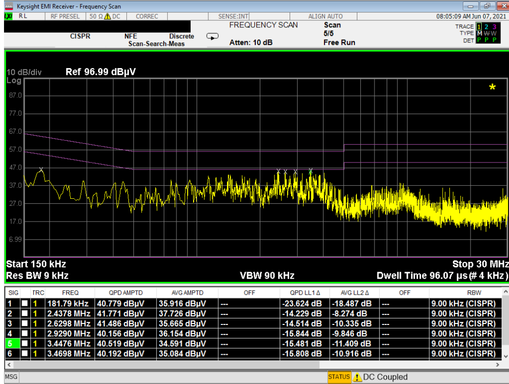
Plot 7-109. Line Conducted Plot with 802.11b (L1) with WCP
