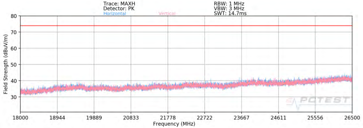
Plot 7-77. Radiated Spurious Plot above 18GHz SISO ANT2 – OPEN
