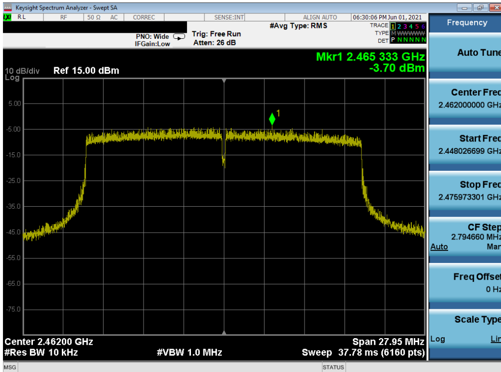
Plot 7-48. Power Spectral Density Plot MIMO ANT2 (802.11ax – Ch. 11)
