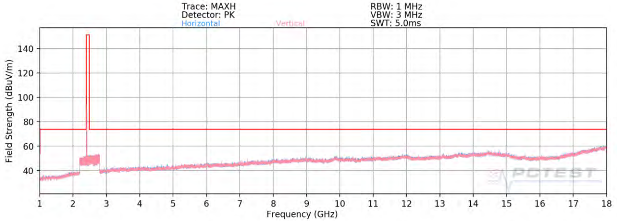
Plot 7-74. Radiated Spurious Plot above 1GHz SISO ANT2 (802.11b – Ch. 1) – CLOSED
