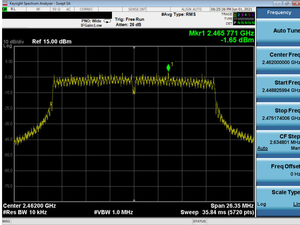
Plot 7-45. Power Spectral Density Plot MIMO ANT2 (802.11n – Ch. 11)
