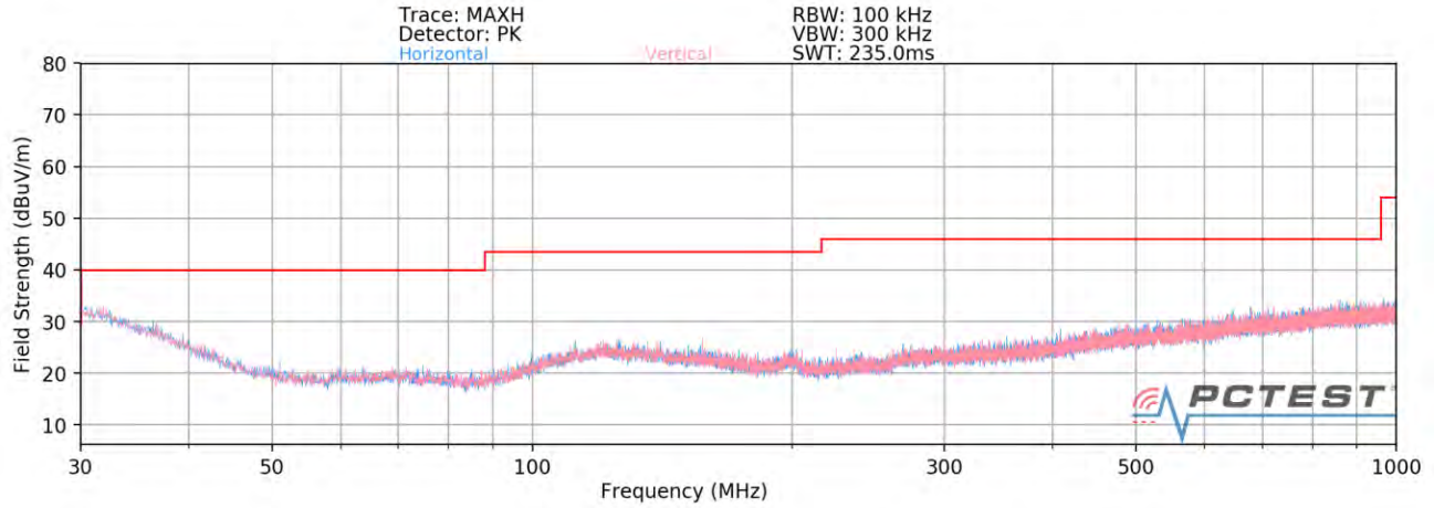
Plot 7-105. Radiated Spurious Plot below 1GHz MIMO – OPEN
