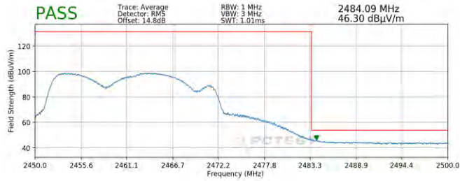
Plot 7-103. Radiated Restricted Band Edge Measurement MIMO with WCP (Average)
