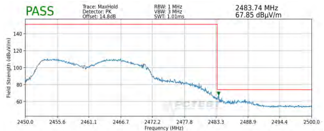
Plot 7-98. Radiated Restricted Upper Band Edge Measurement MIMO (Peak)
