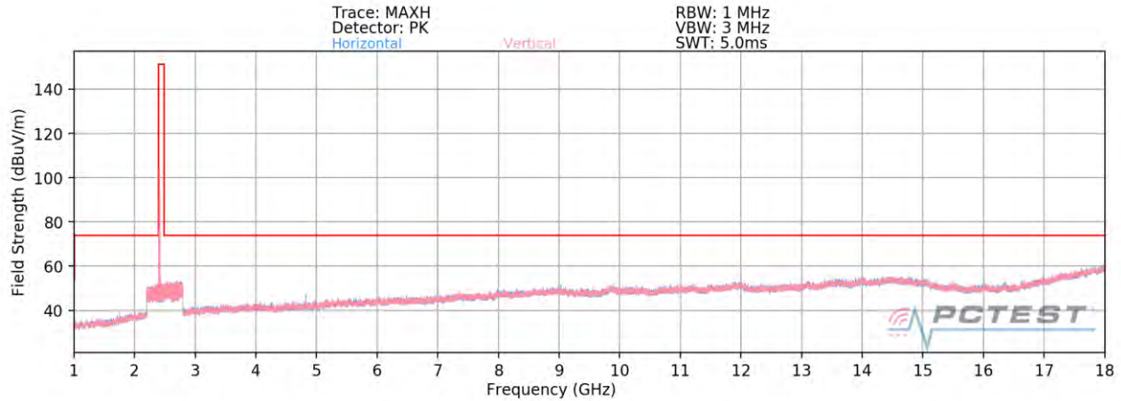
Plot 7-71. Radiated Spurious Plot above 1GHz SISO ANT2 (802.11b – Ch. 1) – OPEN
