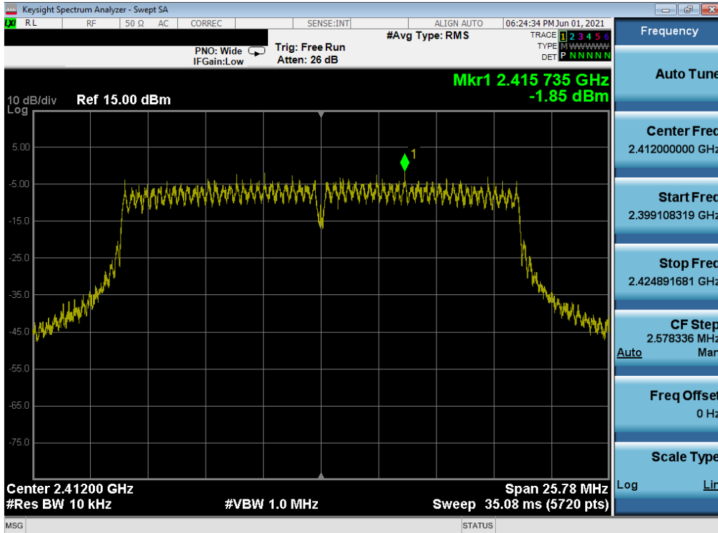
Plot 7-43. Power Spectral Density Plot MIMO ANT2 (802.11n – Ch. 1)
