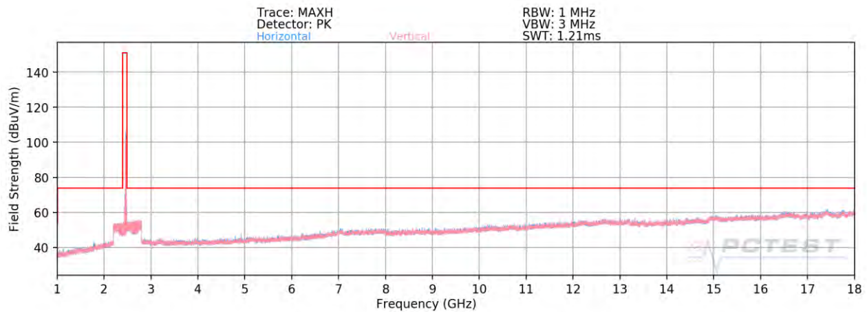
Plot 7-73. Radiated Spurious Plot above 1GHz SISO ANT2 (802.11b – Ch. 11) – OPEN
