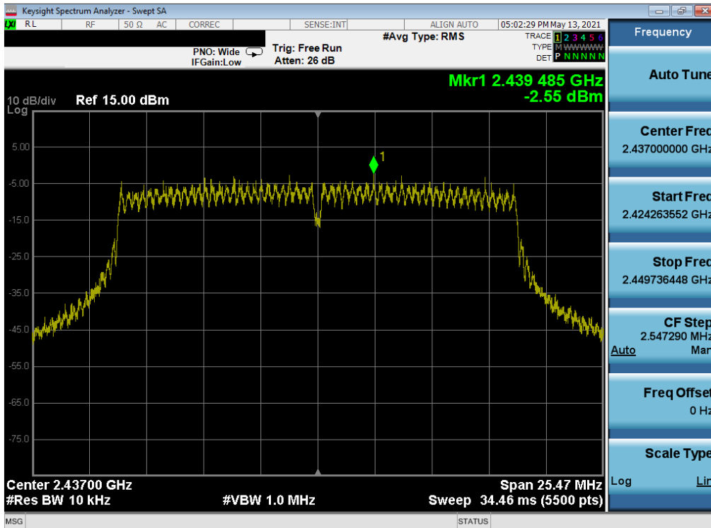
Plot 7-44. Power Spectral Density Plot MIMO ANT2 (802.11n – Ch. 6)
