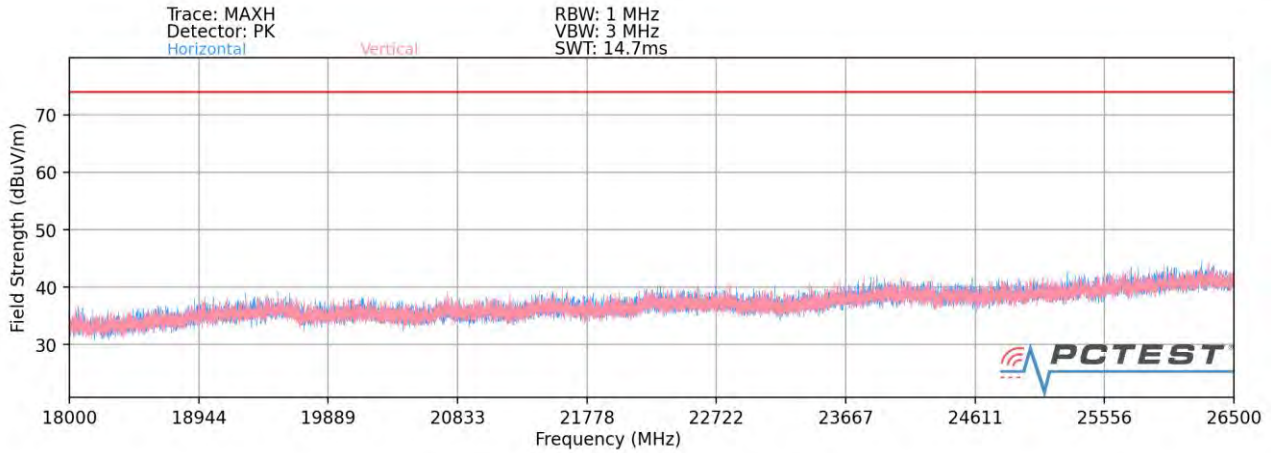
Plot 7-78. Radiated Spurious Plot above 18GHz SISO ANT2- CLOSED
