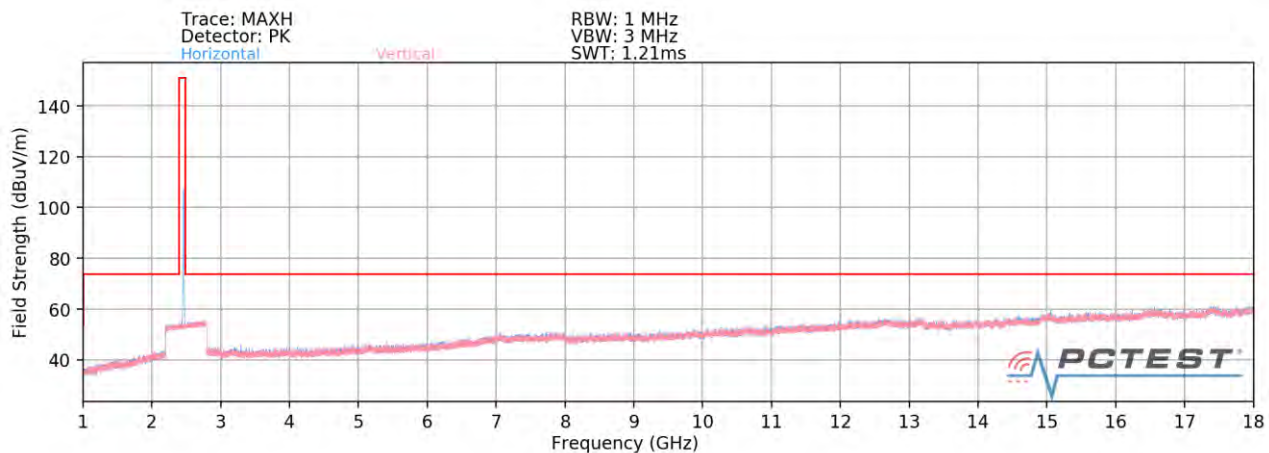
Plot 7-81. Radiated Spurious Plot above 1GHz CDD (802.11b – Ch. 11) – OPEN
