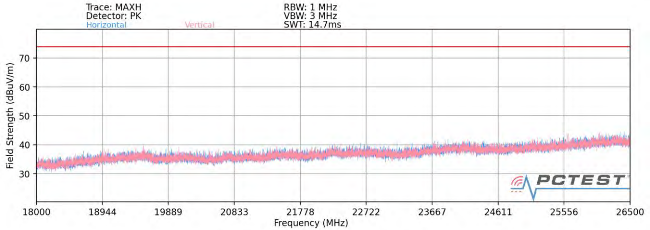
Plot 7-86. Radiated Spurious Plot above 18GHz CDD – CLOSED
