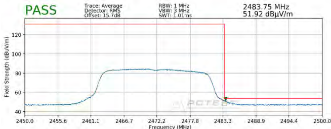
Plot 7-93. Radiated Restricted Upper Band Edge Measurement SISO ANT2 (Average)
