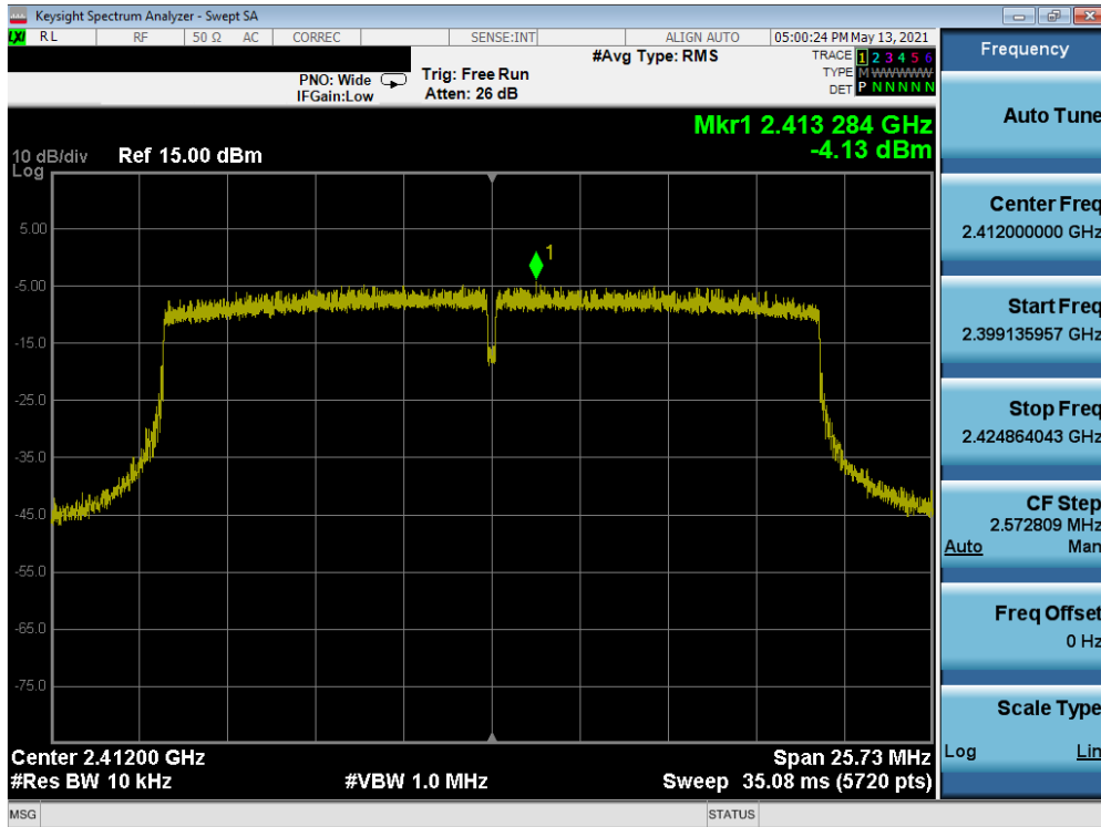
Plot 7-46. Power Spectral Density Plot MIMO ANT2 (802.11ax – Ch. 1)
