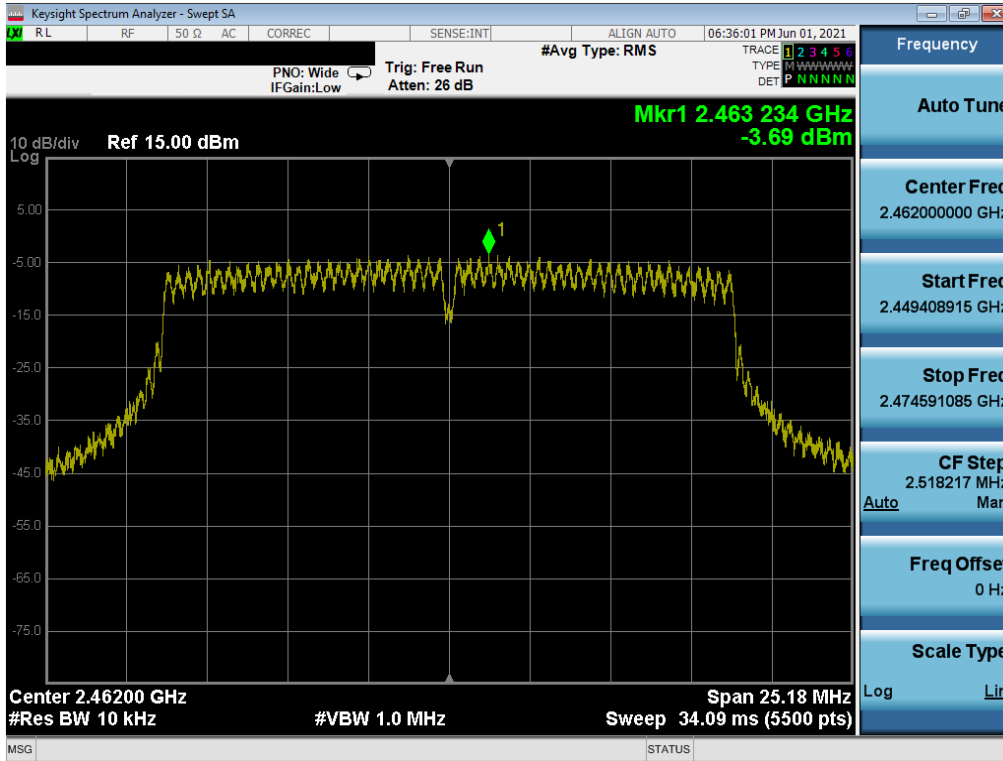
Plot 7-33. Power Spectral Density Plot MIMO ANT1 (802.11n – Ch. 11)
