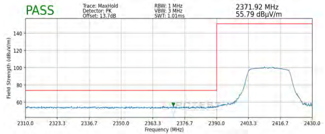
Plot 7-88. Radiated Restricted Lower Band Edge Measurement SISO ANT2 (Peak)
