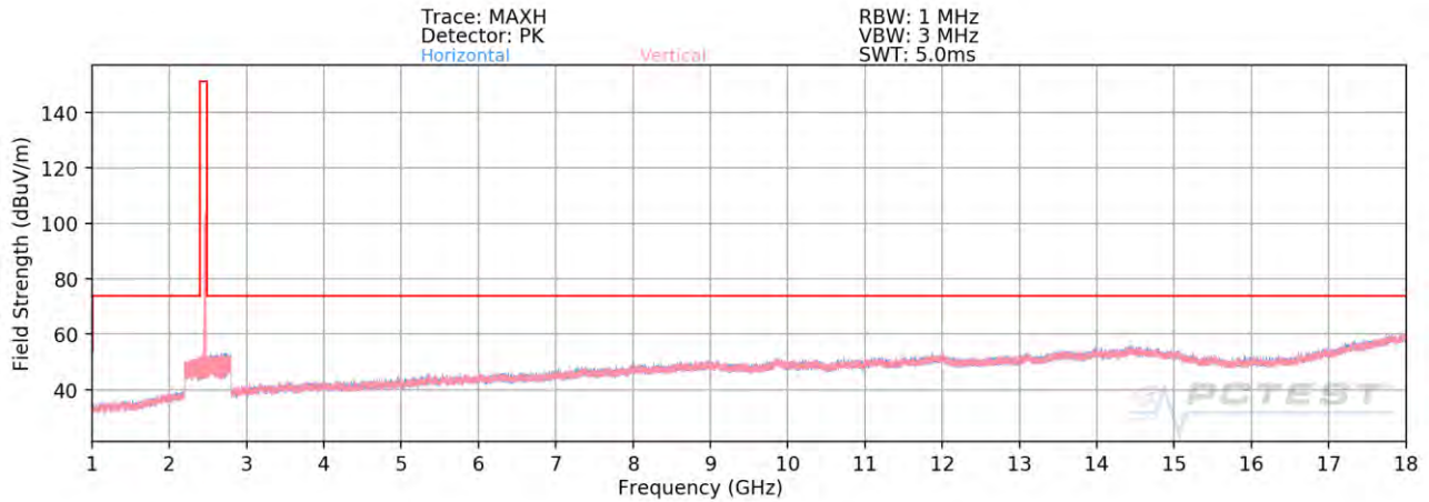
Plot 7-72. Radiated Spurious Plot above 1GHz SISO ANT2 (802.11b – Ch. 6) – OPEN
