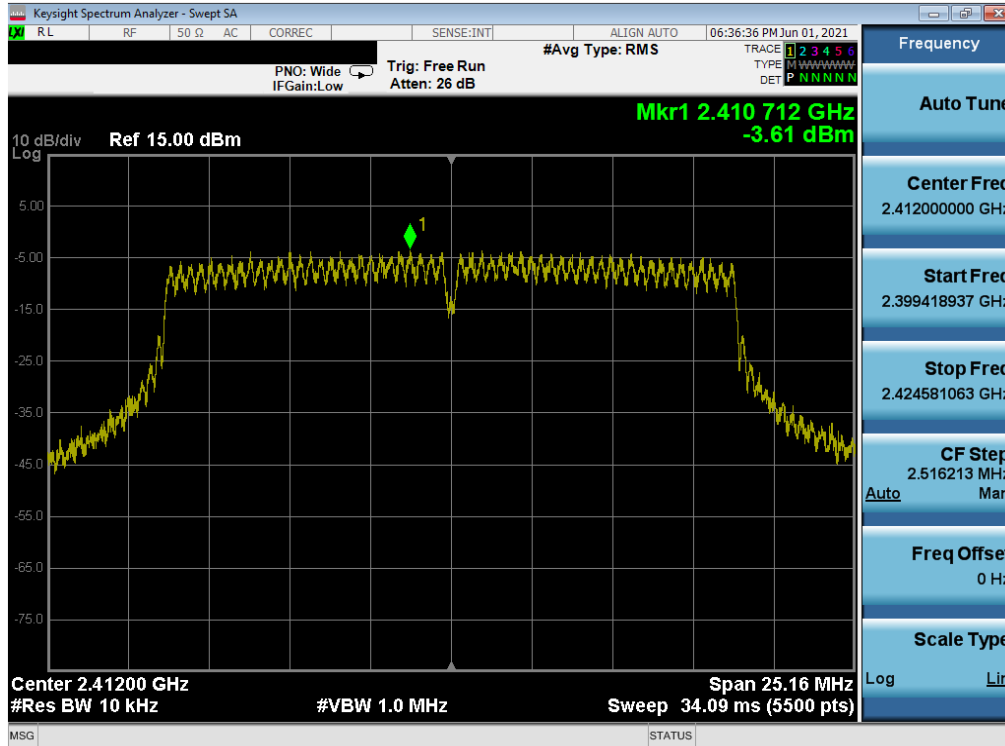
Plot 7-31. Power Spectral Density Plot MIMO ANT1 (802.11n – Ch. 1)
