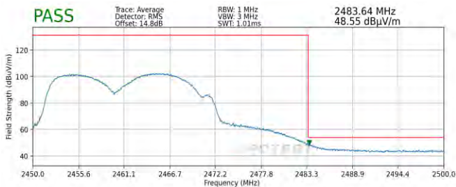
Plot 7-97. Radiated Restricted Upper Band Edge Measurement MIMO (Average)
