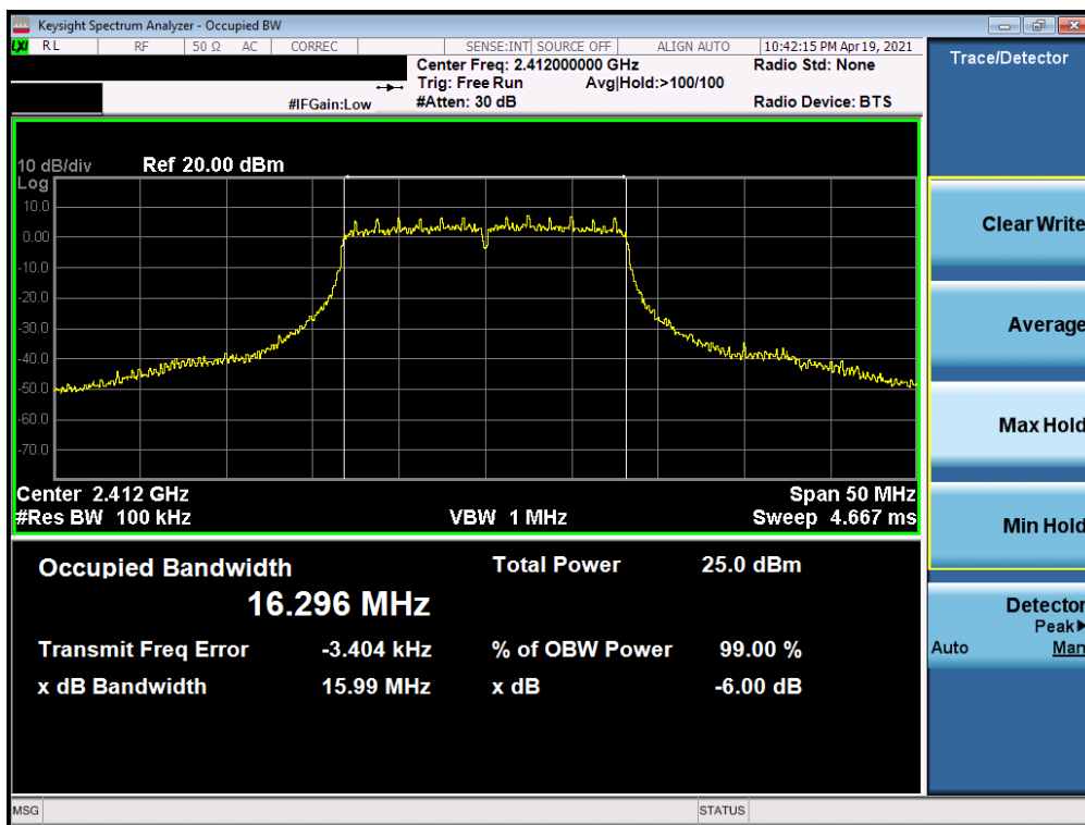
Plot 7-4. 6dB Bandwidth Plot SISO ANT2 (802.11g – Ch. 1)
