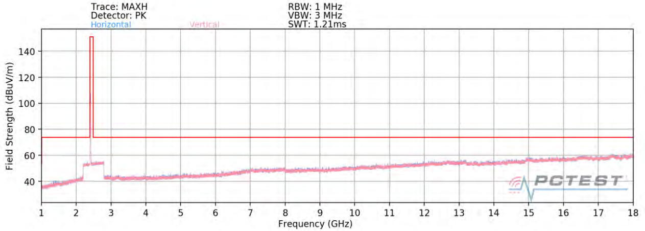
Plot 7-82. Radiated Spurious Plot above 1GHz CDD (802.11b – Ch. 1) – CLOSED
