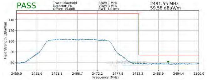
Plot 7-100. Radiated Restricted Upper Band Edge Measurement MIMO (Peak)
