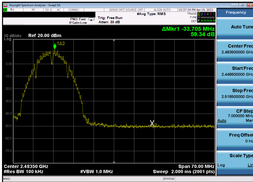
Plot 7-50. Band Edge Plot SISO ANT2 (802.11b – Ch. 11)
