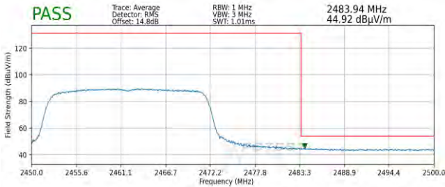
Plot 7-89. Radiated Restricted Upper Band Edge Measurement SISO ANT2 (Average)
