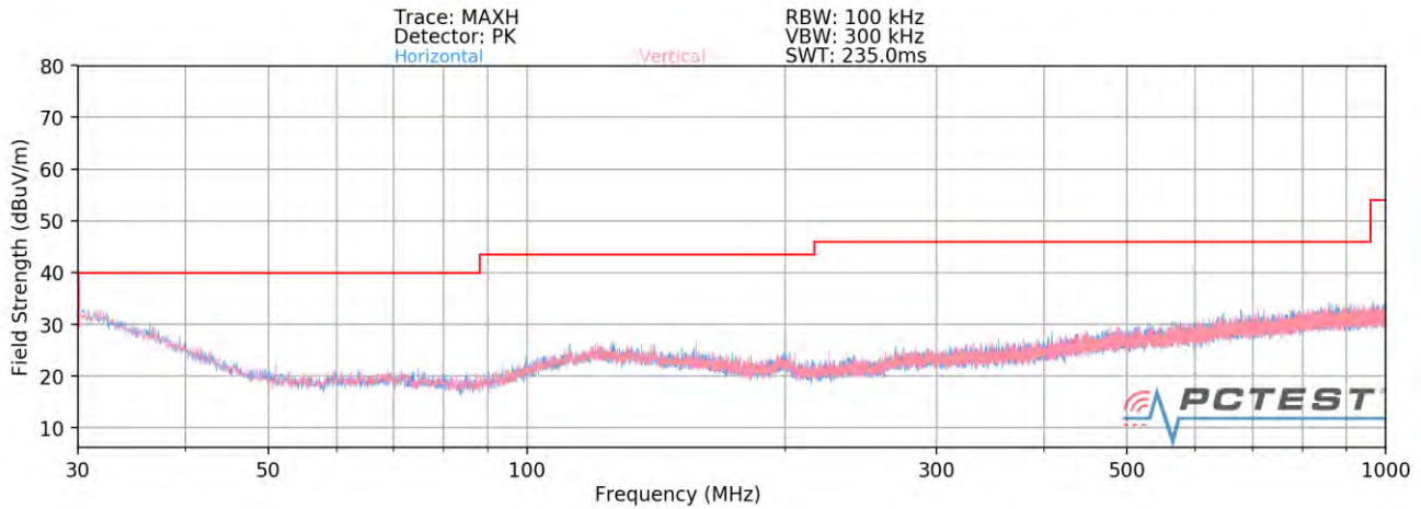
Plot 7-106. Radiated Spurious Plot below 1GHz MIMO – CLOSED
