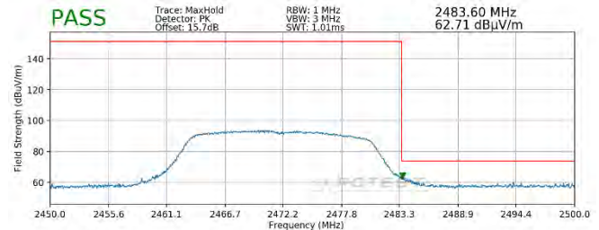
Plot 7-94. Radiated Restricted Upper Band Edge Measurement SISO ANT2 (Peak)
