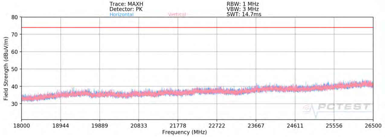
Plot 7-85. Radiated Spurious Plot above 18GHz CDD – OPEN
