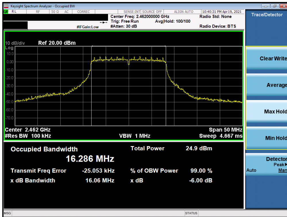
Plot 7-6. 6dB Bandwidth Plot SISO ANT (802.11g – Ch. 11)
