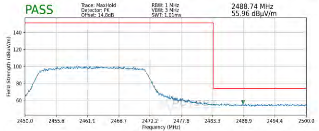
Plot 7-90. Radiated Restricted Upper Band Edge Measurement SISO ANT2 (Peak)
