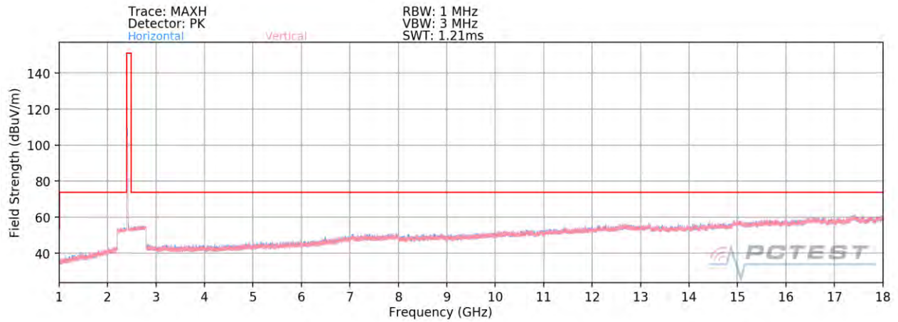
Plot 7-79. Radiated Spurious Plot above 1GHz CDD (802.11b – Ch. 1) – OPEN
