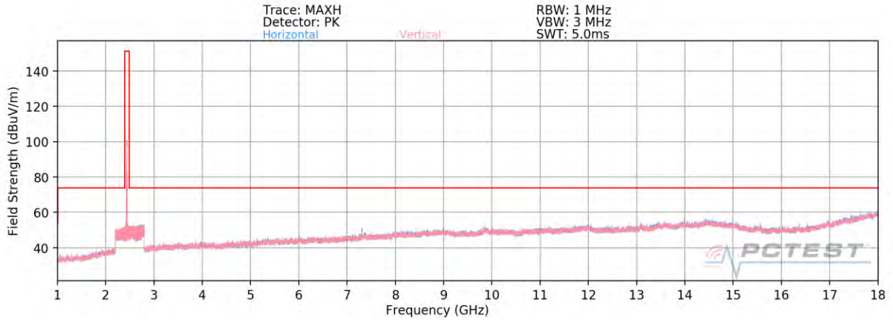
Plot 7-75. Radiated Spurious Plot above 1GHz SISO ANT2 (802.11b – Ch. 6) – CLOSED
