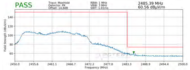
Plot 7-104. Radiated Restricted Band Edge Measurement MIMO with WCP (Peak)
