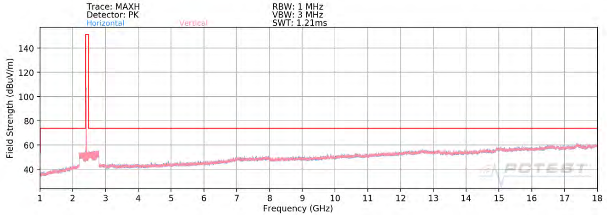
Plot 7-48. Radiated Spurious Plot above 1GHz SISO ANT2 (802.11ax OFDMA – 26 Tones – Ch. 1) – CLOSED
