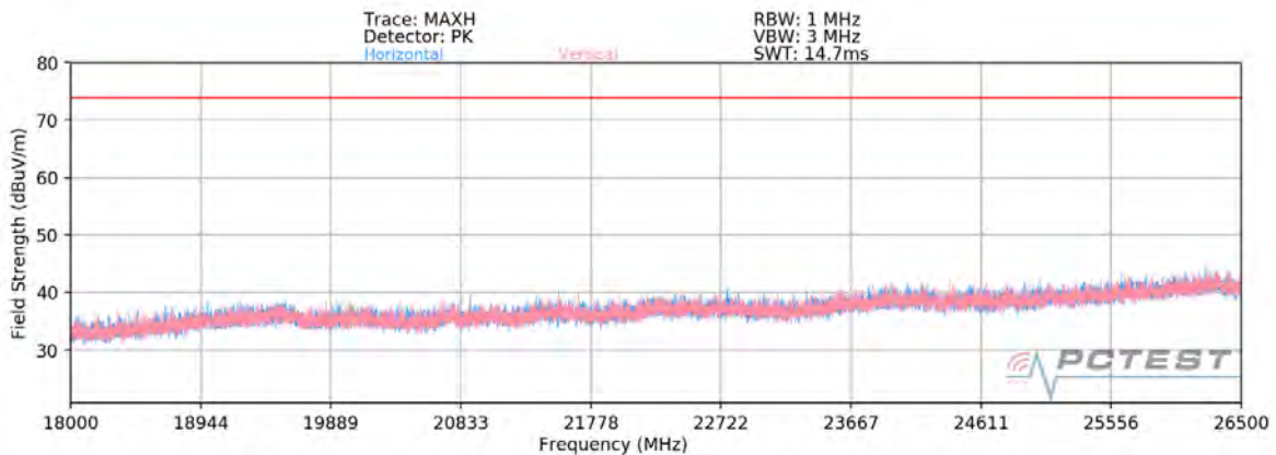
Plot 7-59. Radiated Spurious Plot above 18GHz SISO ANT2 (802.11ax OFDMA – 242 Tones) – OPEN
