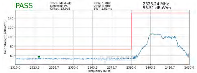
Plot 7-78. Radiated Restricted Lower Band Edge Measurement SISO ANT2 (Peak – 106 Tones)
