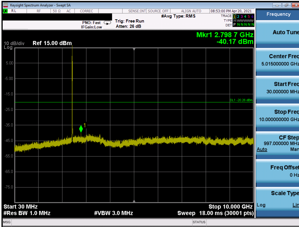
Plot 7-35. Conducted Spurious Plot SISO ANT2 (802.11ax OFDMA – 26 Tones – Ch. 6)
