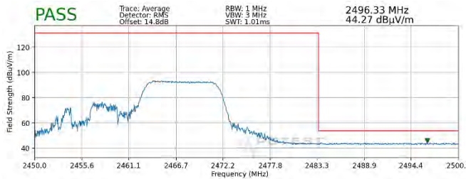
Plot 7-79. Radiated Restricted Upper Band Edge Measurement SISO ANT2 (Average – 106 Tones)
