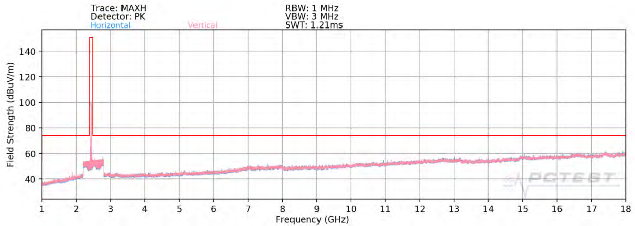
Plot 7-55. Radiated Spurious Plot above 1GHz SISO ANT2 (802.11ax OFDMA – 242 Tones – Ch. 6) – CLOSED
