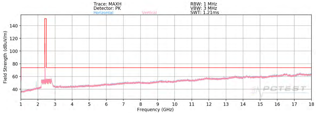
Plot 7-45. Radiated Spurious Plot above 1GHz SISO ANT2 (802.11ax OFDMA – 26 Tones – Ch. 1) – OPEN
