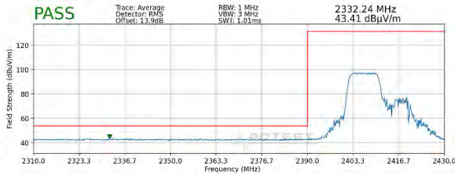
Plot 7-77. Radiated Restricted Lower Band Edge Measurement SISO ANT2 (Average – 106 Tones)
