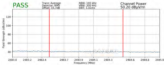
Plot 7-83. Radiated Restricted Upper Band Edge Measurement SISO ANT2 (Average – 106 Tones)
