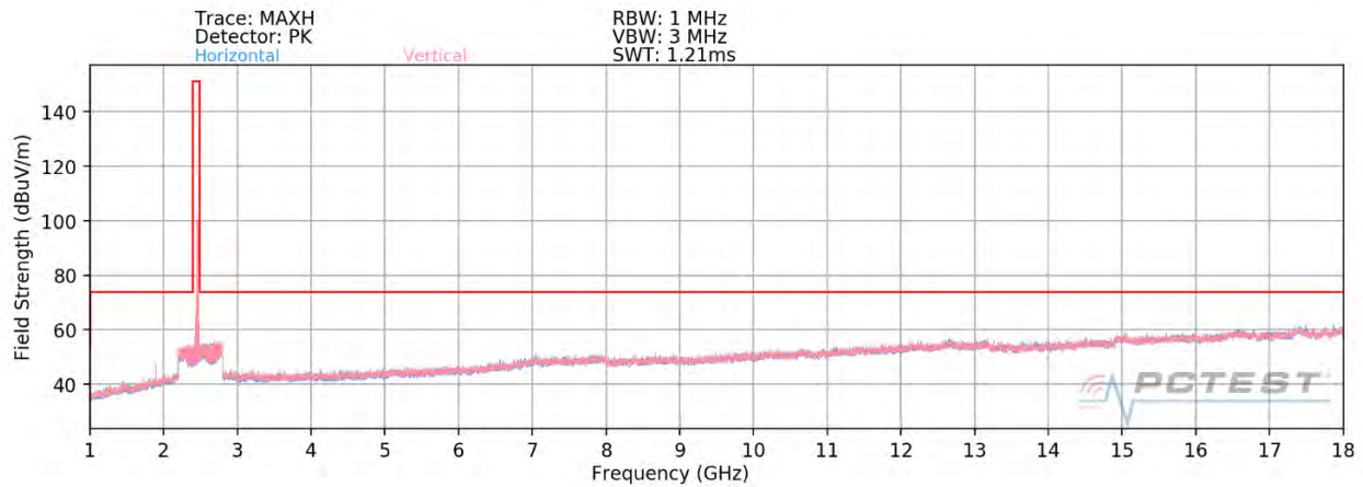
Plot 7-56. Radiated Spurious Plot above 1GHz SISO ANT2 (802.11ax OFDMA – 242 Tones – Ch. 11) – CLOSED
