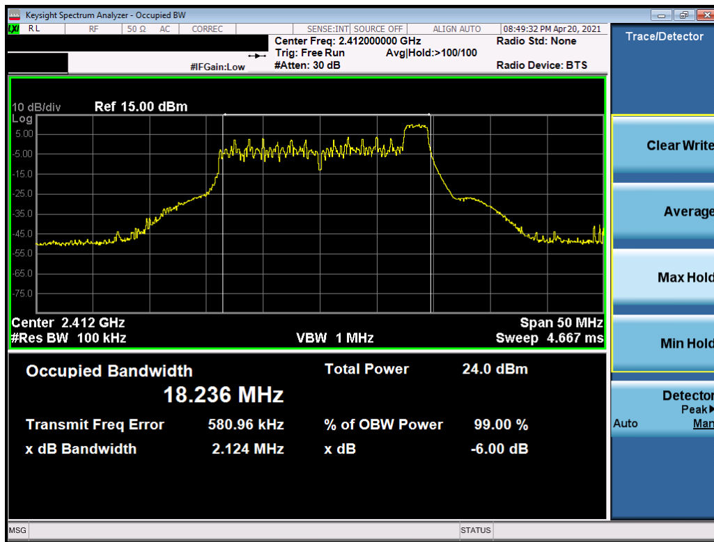
Plot 7-1. 6dB Bandwidth Plot SISO ANT2 (802.11ax OFDMA – 26 Tones – Ch. 1)
