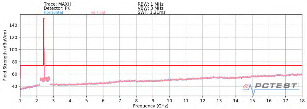
Plot 7-50. Radiated Spurious Plot above 1GHz SISO ANT2 (802.11ax OFDMA – 26 Tones – Ch. 11) – CLOSED
