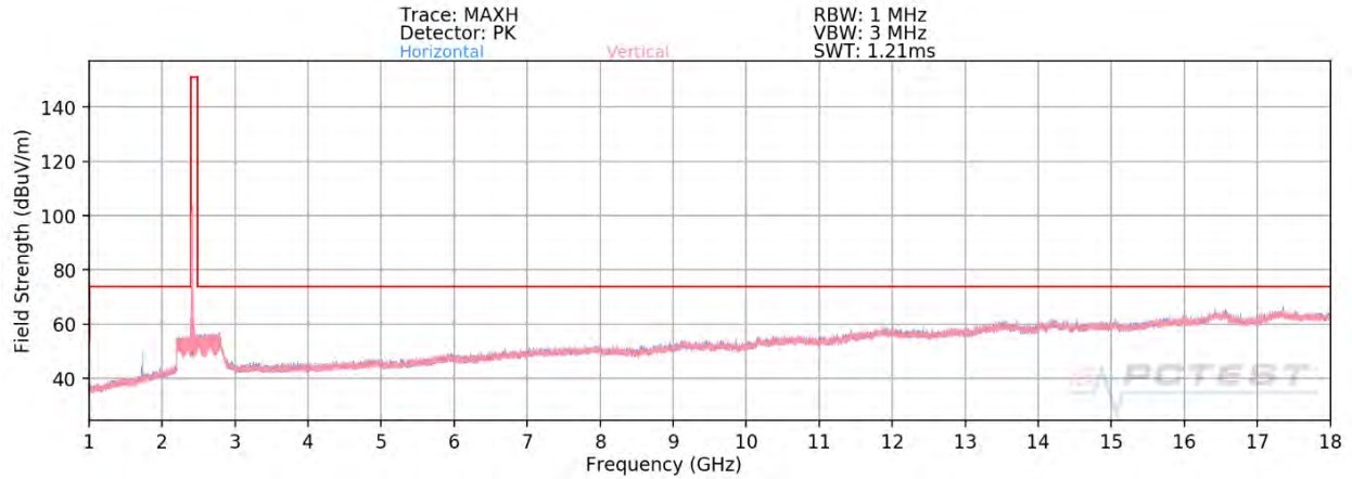
Plot 7-51. Radiated Spurious Plot above 1GHz SISO ANT2 (802.11ax OFDMA – 242 Tones – Ch. 1) – OPEN
