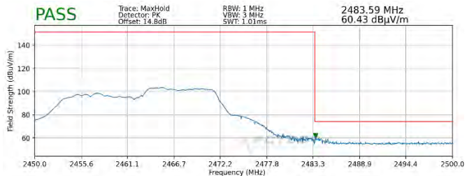
Plot 7-80. Radiated Restricted Upper Band Edge Measurement SISO ANT2 (Peak – 106 Tones)
