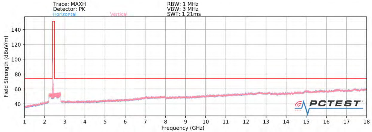
Plot 7-54. Radiated Spurious Plot above 1GHz SISO ANT2 (802.11ax OFDMA – 242 Tones – Ch. 1) – CLOSED
