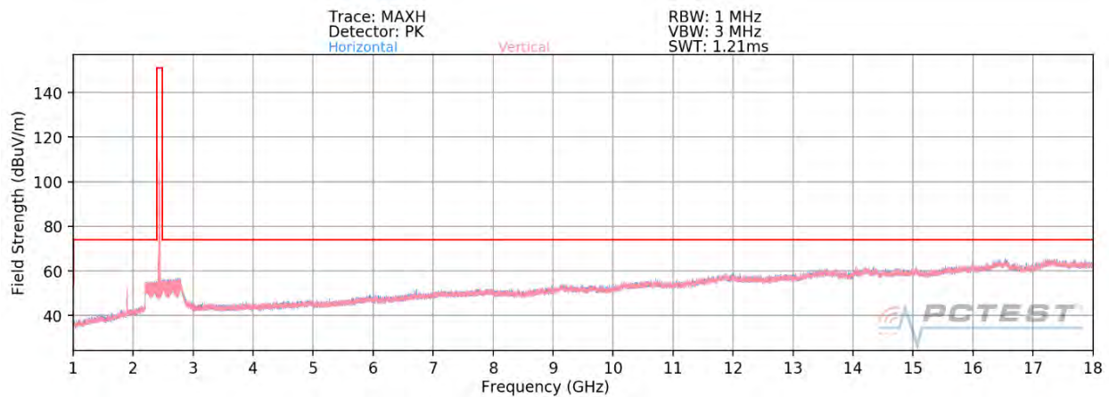
Plot 7-46. Radiated Spurious Plot above 1GHz SISO ANT2 (802.11ax OFDMA – 26 Tones – Ch. 6) – OPEN
