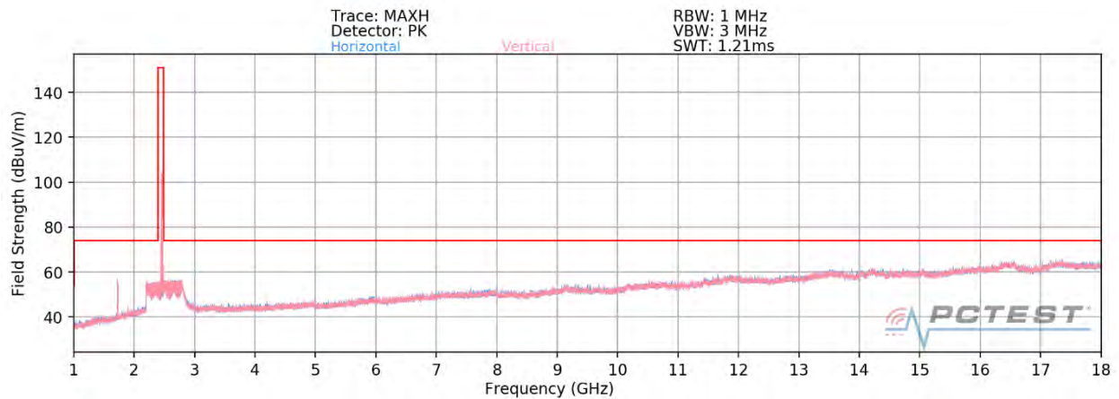
Plot 7-53. Radiated Spurious Plot above 1GHz SISO ANT2 (802.11ax OFDMA – 242 Tones – Ch. 11) – OPEN
