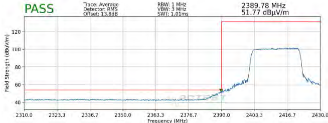
Plot 7-101. Radiated Restricted Lower Band Edge Measurement MIMO (Average – 242 Tones)
