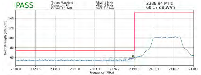
Plot 7-86. Radiated Restricted Lower Band Edge Measurement SISO ANT2 (Peak – 242 Tones)
