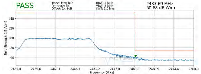
Plot 7-88. Radiated Restricted Upper Band Edge Measurement SISO ANT2 (Peak – 242 Tones)
