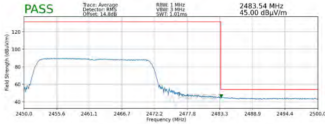
Plot 7-87. Radiated Restricted Upper Band Edge Measurement SISO ANT2 (Average – 242 Tones)
