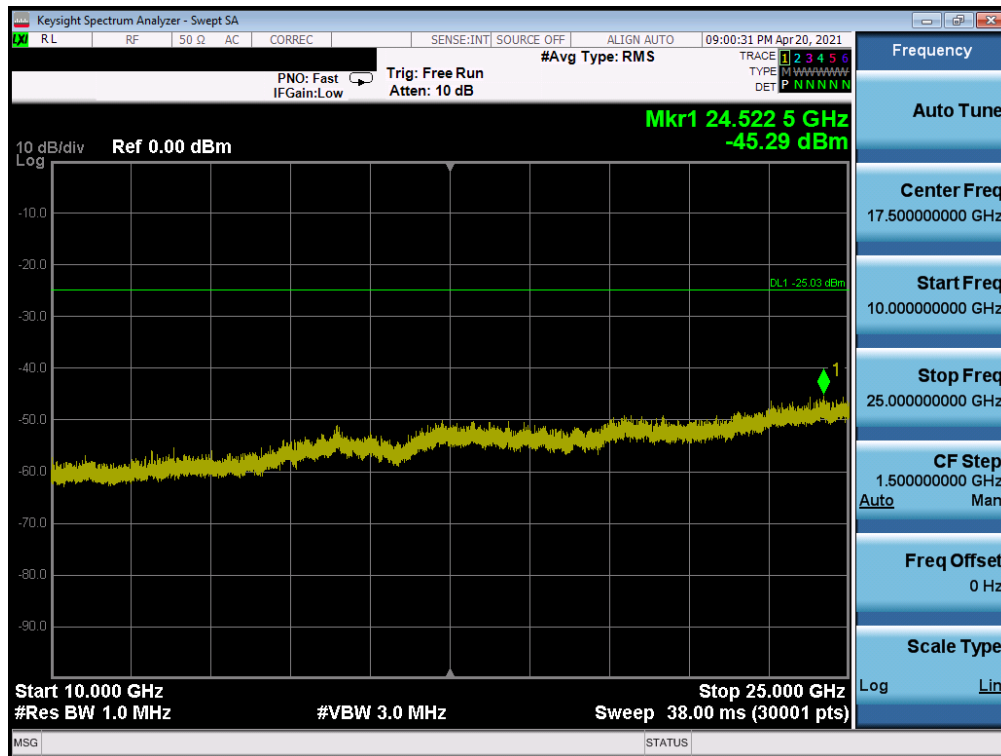
Plot 7-40. Conducted Spurious Plot SISO ANT2 (802.11ax OFDMA – 242 Tones – Ch. 1)
