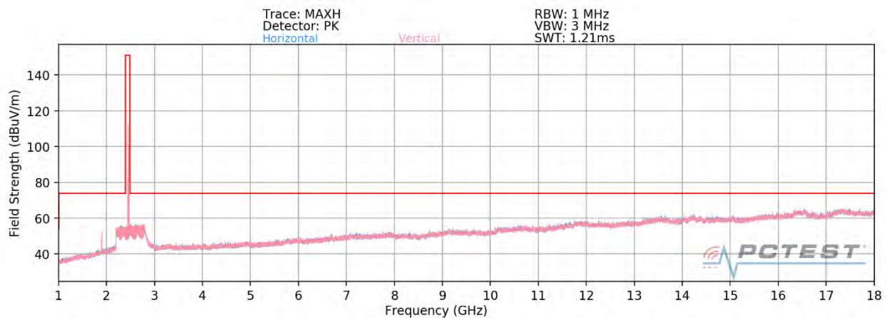
Plot 7-47. Radiated Spurious Plot above 1GHz SISO ANT2 (802.11ax OFDMA – 26 Tones – Ch. 11) – OPEN
