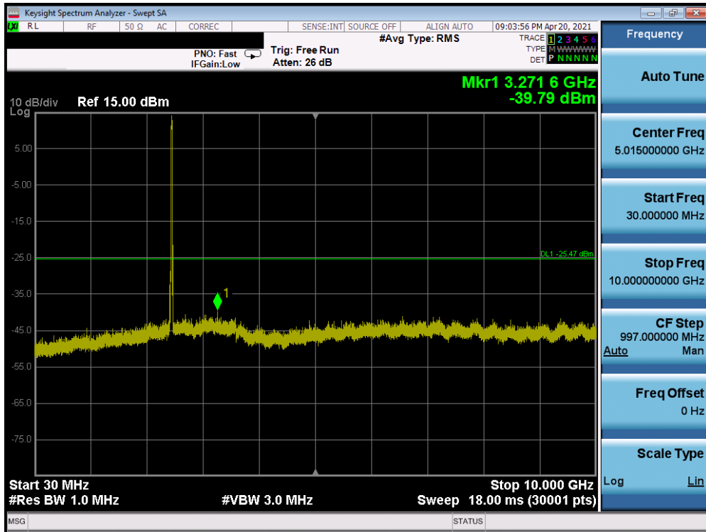
Plot 7-43. Conducted Spurious Plot SISO ANT2 (802.11ax OFDMA – 242 Tones – Ch. 11)
