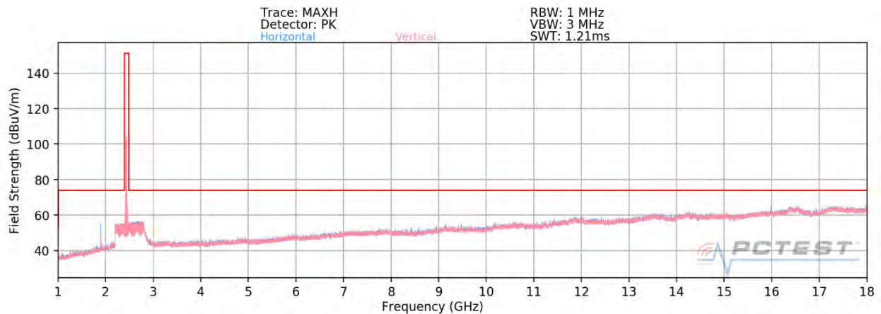
Plot 7-52. Radiated Spurious Plot above 1GHz SISO ANT2 (802.11ax OFDMA – 242 Tones – Ch. 6) – OPEN
