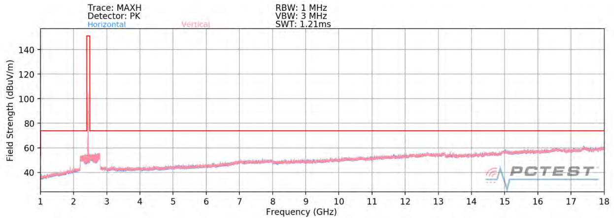
Plot 7-49. Radiated Spurious Plot above 1GHz SISO ANT2 (802.11ax OFDMA – 26 Tones – Ch. 6) – CLOSED
