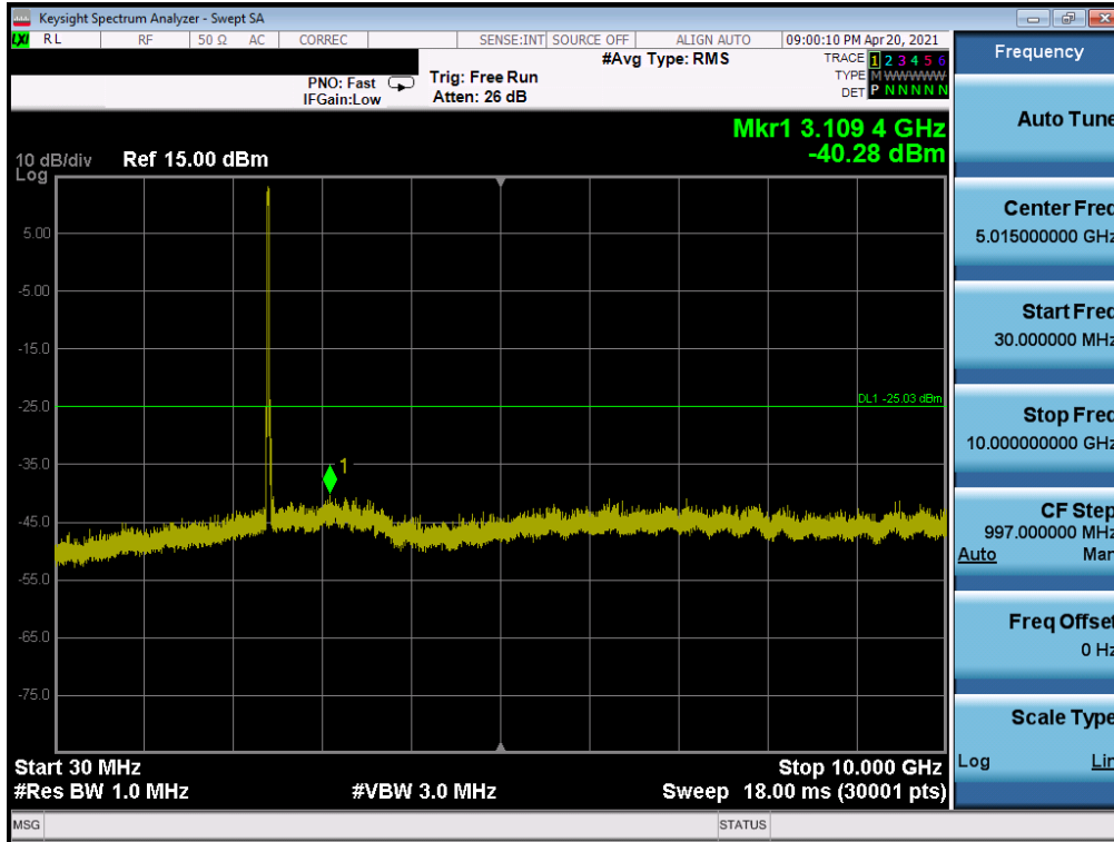
Plot 7-39. Conducted Spurious Plot SISO ANT2 (802.11ax OFDMA – 242 Tones – Ch. 1)
