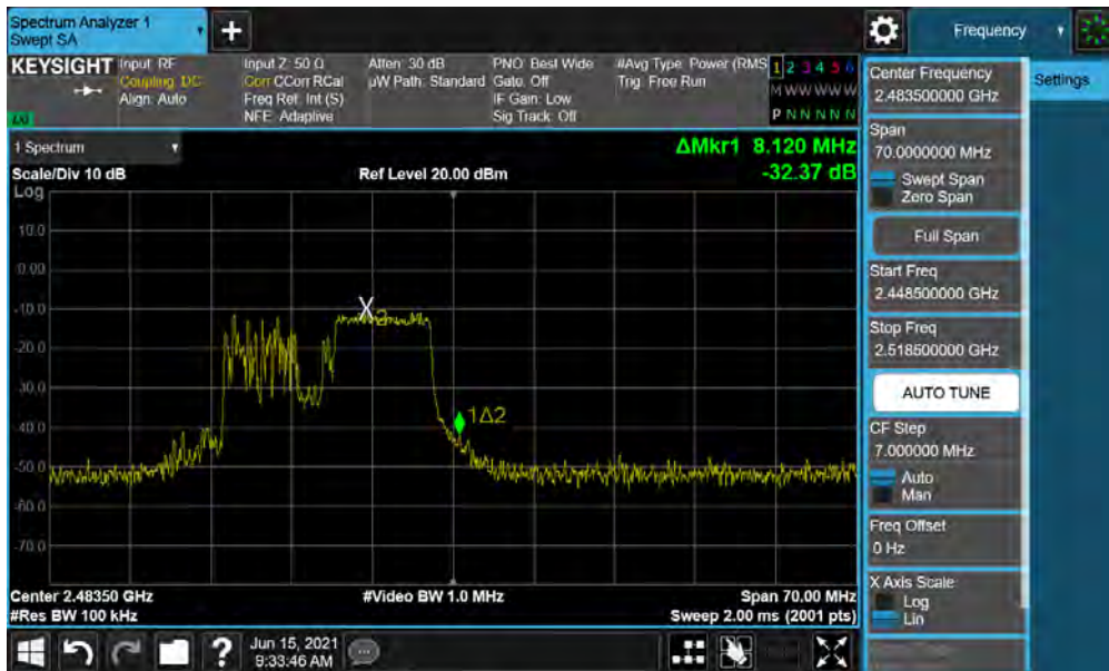
Plot 7-28. Band Edge Plot SISO ANT2 (802.11ax OFDMA – 106 Tones – Ch. 13)
