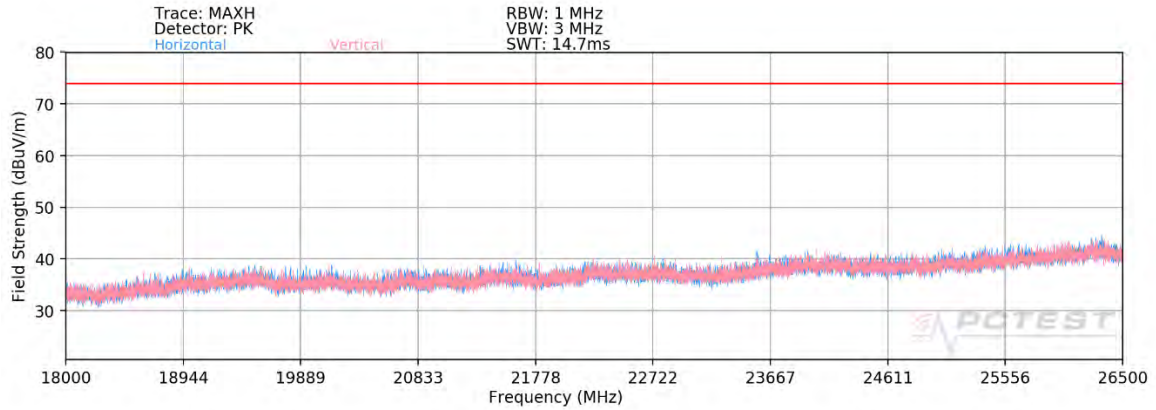
Plot 7-58. Radiated Spurious Plot above 18GHz SISO ANT2 (802.11ax OFDMA – 26 Tones) – CLOSED
