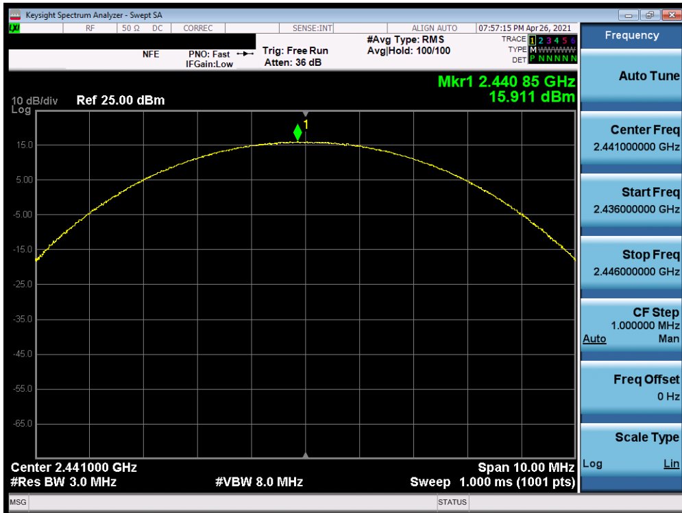
Plot 7-44. Peak Conducted Power (2Mbps, ePA – Ch. 39) – ANT0
