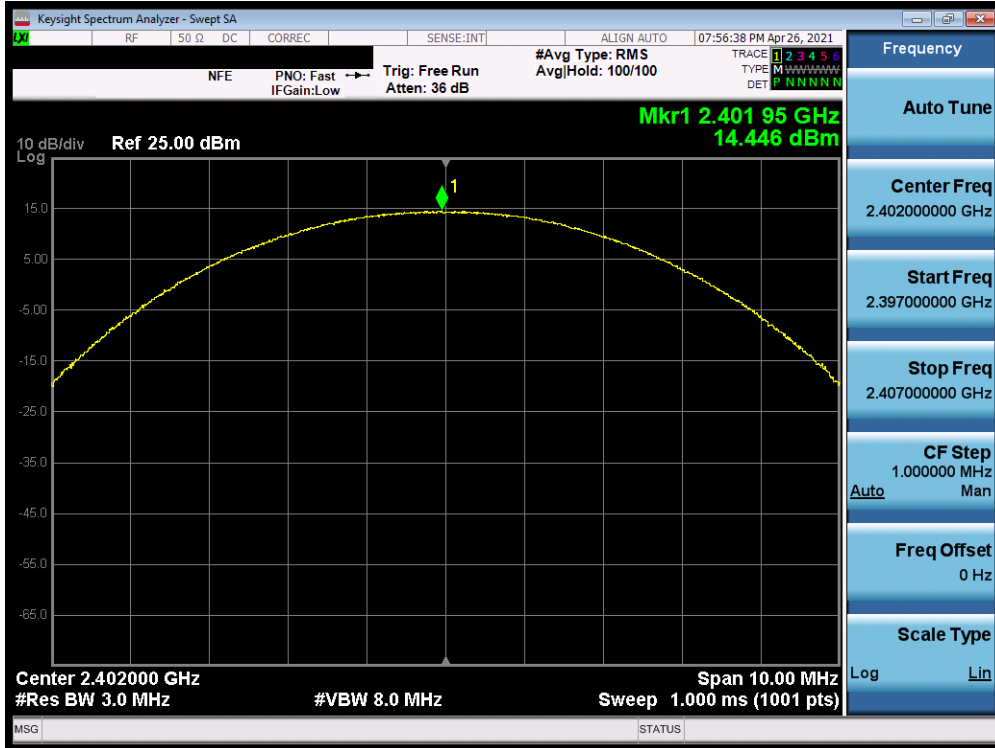
Plot 7-43. Peak Conducted Power (2Mbps, ePA – Ch. 0) – ANT0
