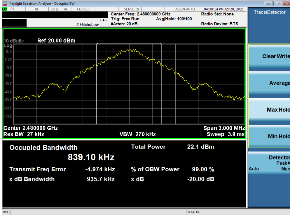
Plot 7-3. 20dB Bandwidth Plot (Bluetooth, 1Mbps, ePA – Ch. 78) – ANTO
