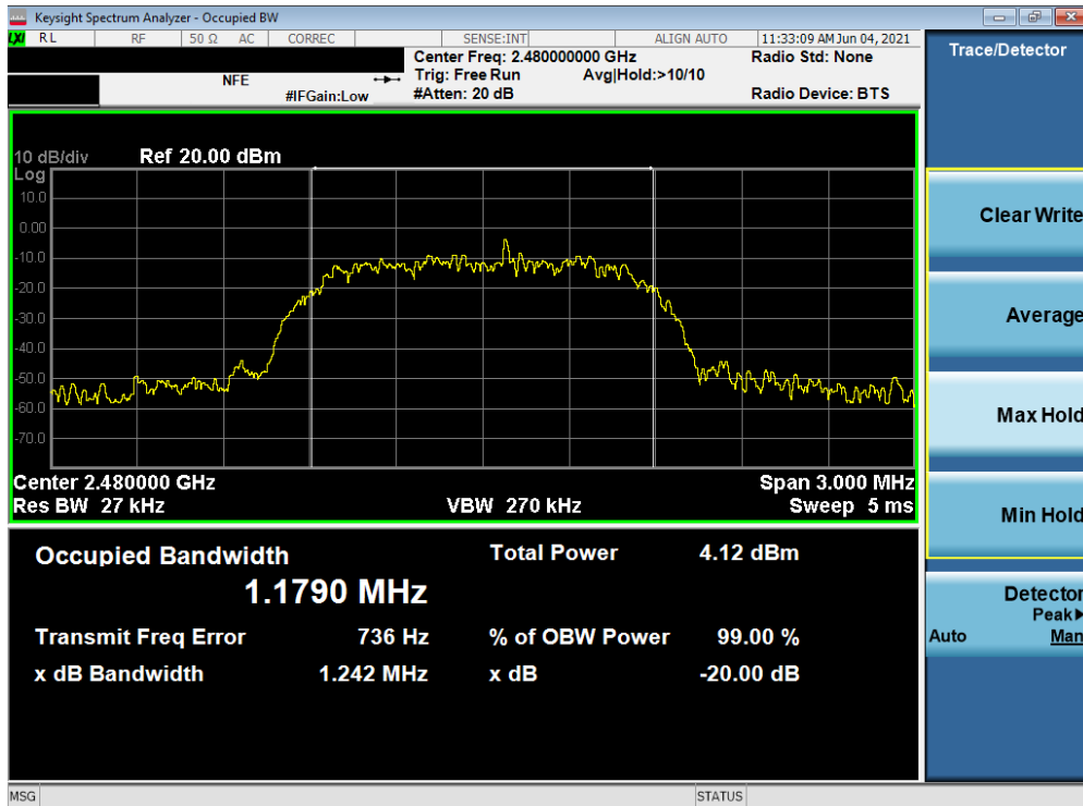
Plot 7-18. 20dB Bandwidth Plot (Bluetooth, 3Mbps, iPA – Ch. 78) – ANTO
