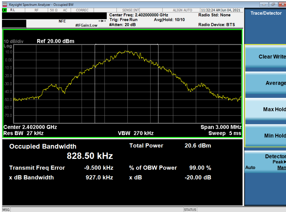
Plot 7-4. 20dB Bandwidth Plot (Bluetooth, 1Mbps, iPA – Ch. 0) – ANTO
