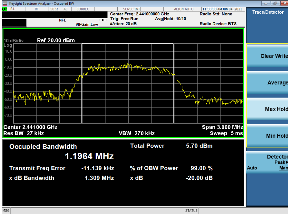
Plot 7-17. 20dB Bandwidth Plot (Bluetooth, 3Mbps, iPA – Ch. 39) – ANTO
