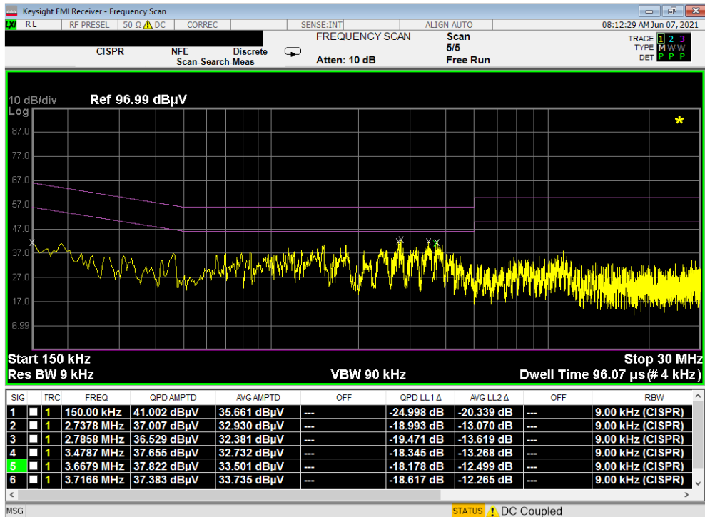
Plot 7-442. Line Conducted Plot with 802.11a UNII Band 2C (N) with WCP
