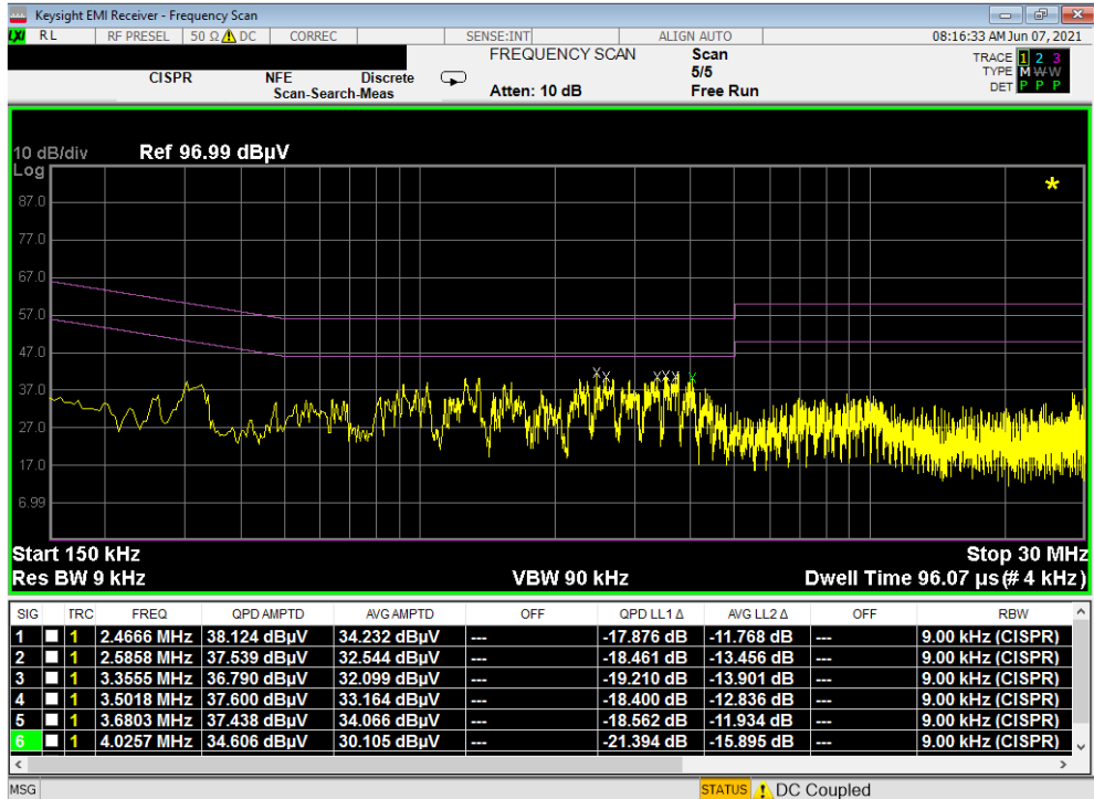
Plot 7-444. Line Conducted Plot with 802.11a UNII Band 3 (N) with WCP
