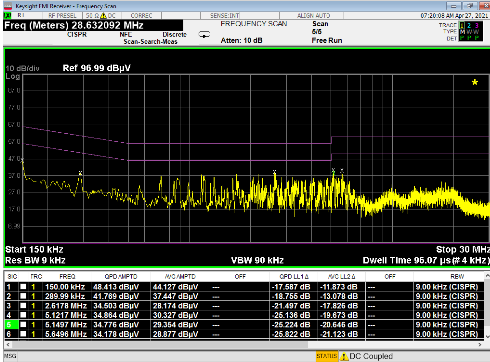
Plot 7-435. Line Conducted Plot with 802.11a UNII Band 3 (L1) - Closed
