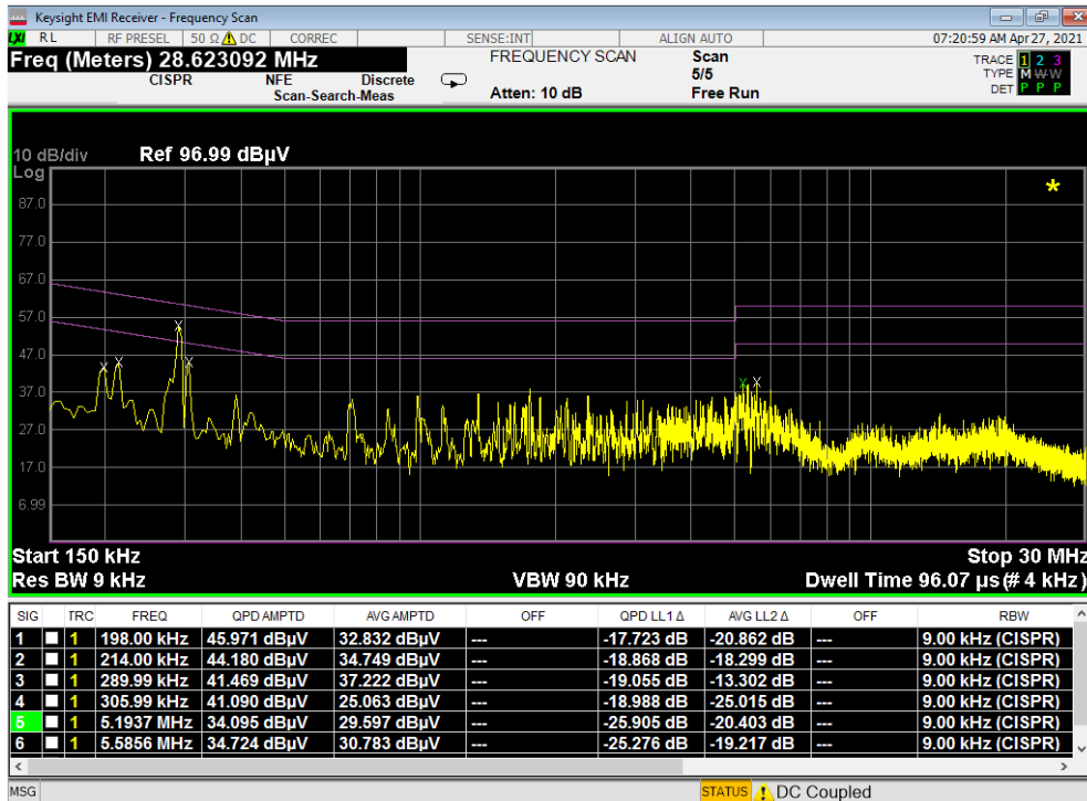
Plot 7-436. Line Conducted Plot with 802.11a UNII Band 3 (N) - Closed
