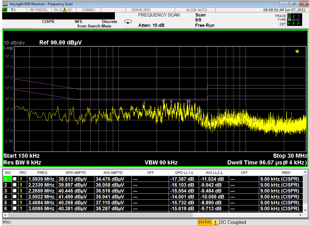
Plot 7-437. Line Conducted Plot with 802.11a UNII Band 1 (L1) with WCP
