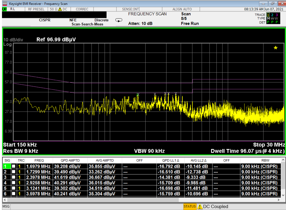
Plot 7-441. Line Conducted Plot with 802.11a UNII Band 2C (L1) with WCP
