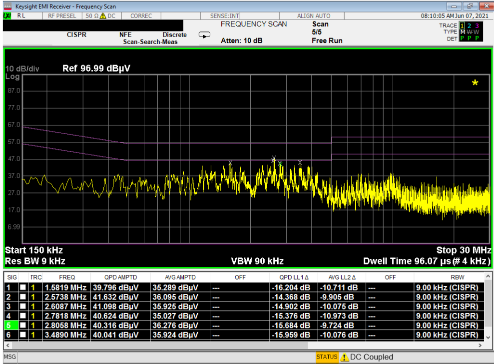
Plot 7-439. Line Conducted Plot with 802.11a UNII Band 2A (L1) with WCP
