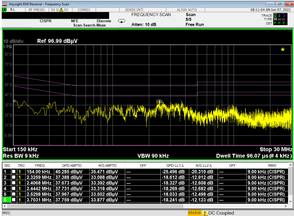
Plot 7-440. Line Conducted Plot with 802.11a UNII Band 2A (N) with WCP
