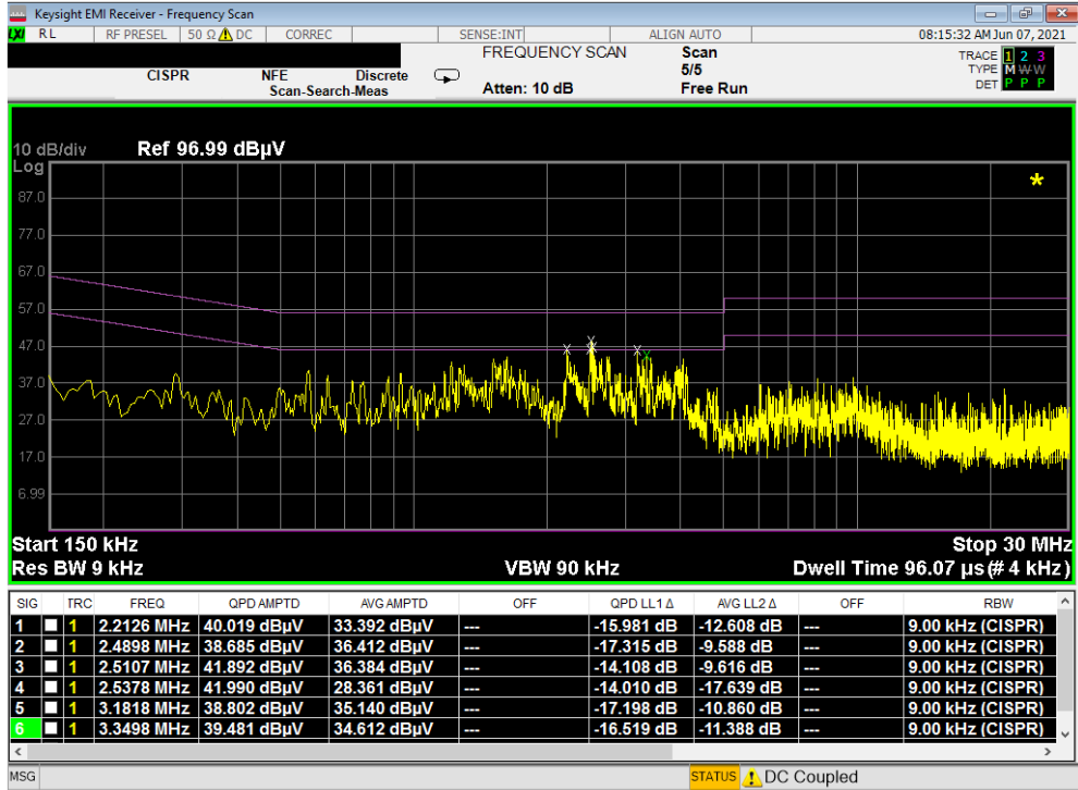
Plot 7-443. Line Conducted Plot with 802.11a UNII Band 3 (L1) with WCP
