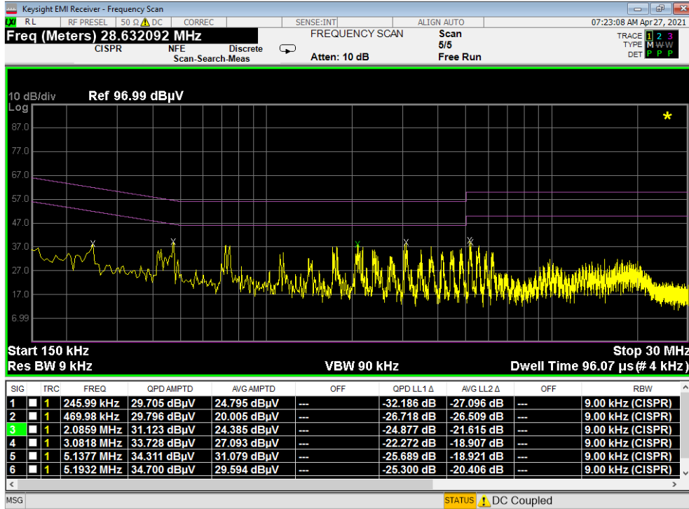
Plot 7-433. Line Conducted Plot with 802.11a UNII Band 2C (L1) - Closed
