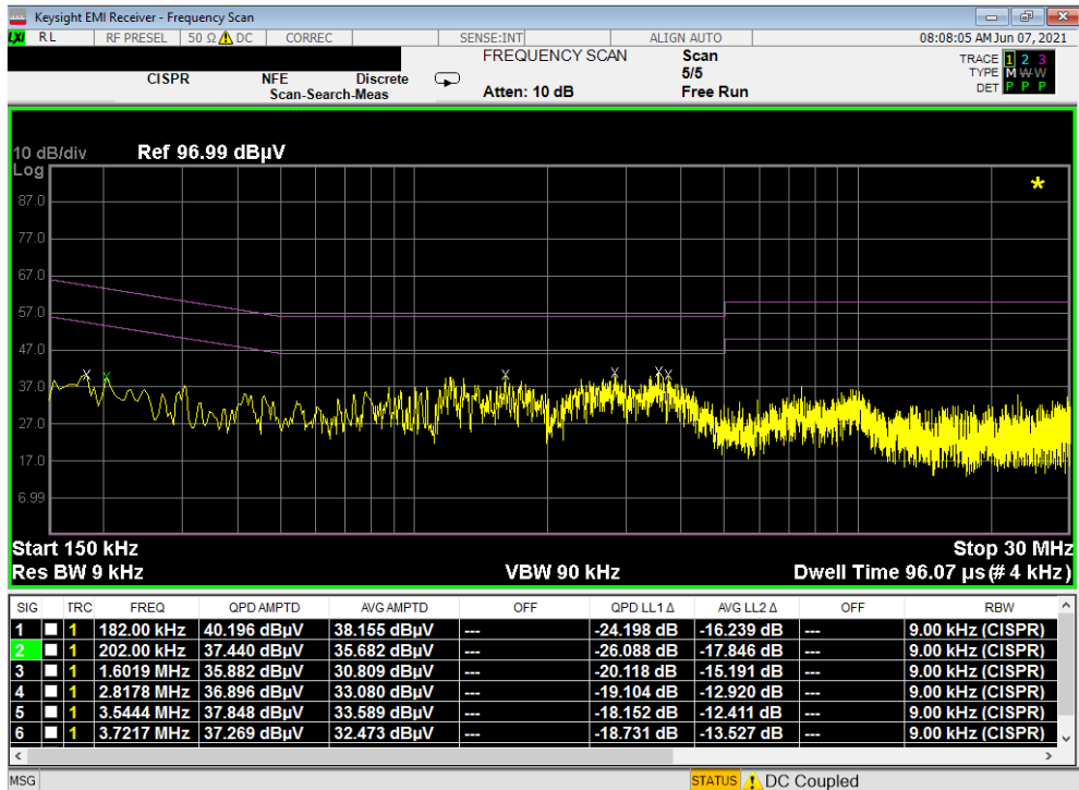
Plot 7-438. Line Conducted Plot with 802.11a UNII Band 1 (N) with WCP
