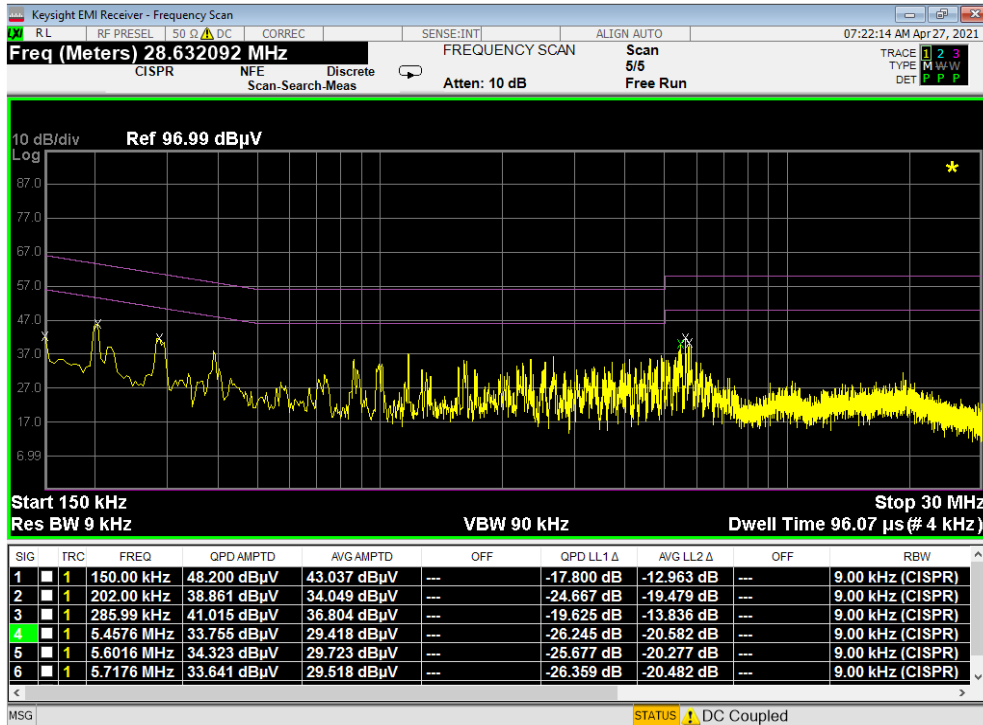
Plot 7-434. Line Conducted Plot with 802.11a UNII Band 2C (N) - Closed
