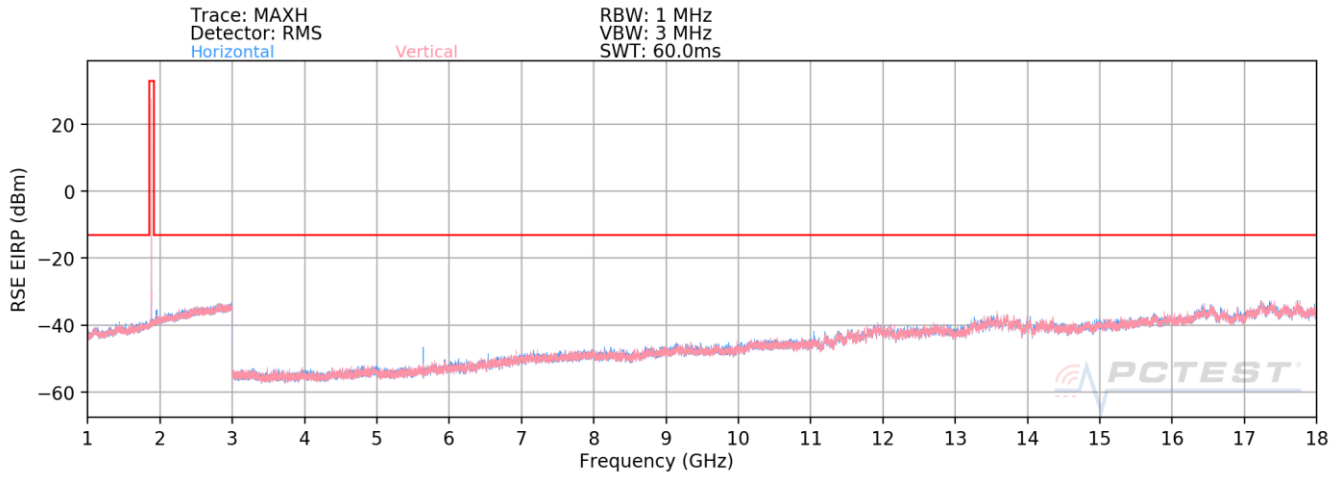
Plot 7-18. Radiated Spurious Plot (GPRS PCS - Open)
