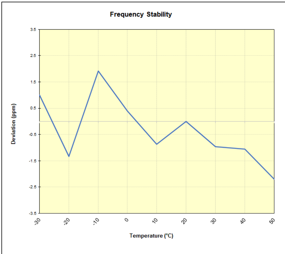
Plot 7-20. GSM/GPRS PCS Frequency Stability Chart
