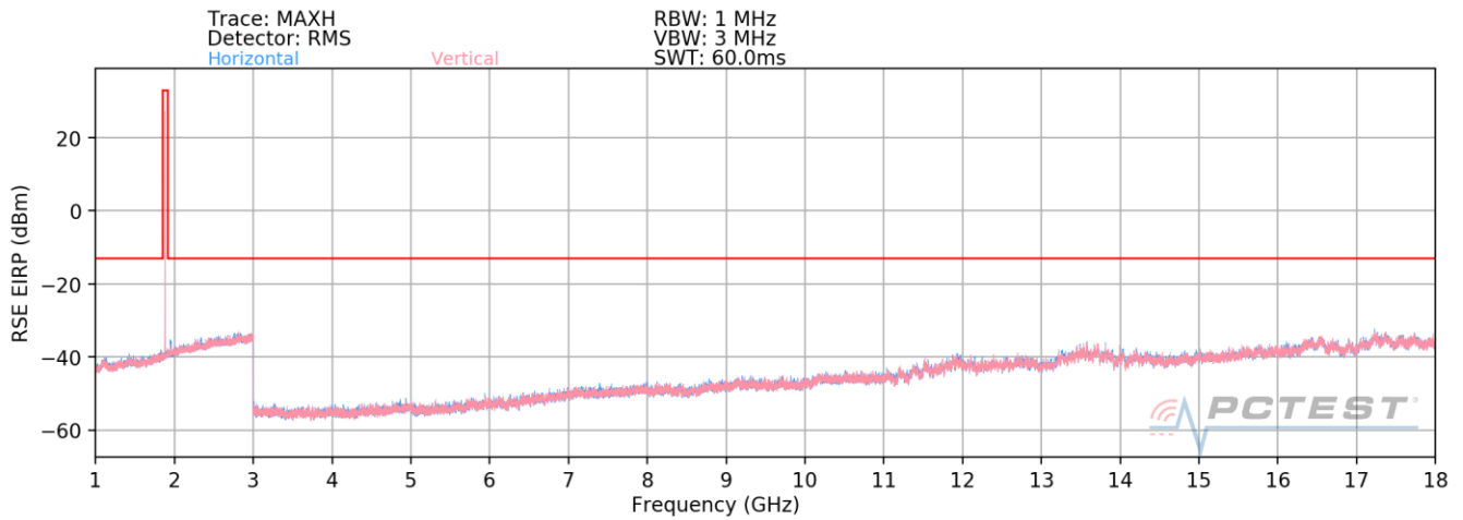
Plot 7-19. Radiated Spurious Plot (GPRS PCS - Closed)
