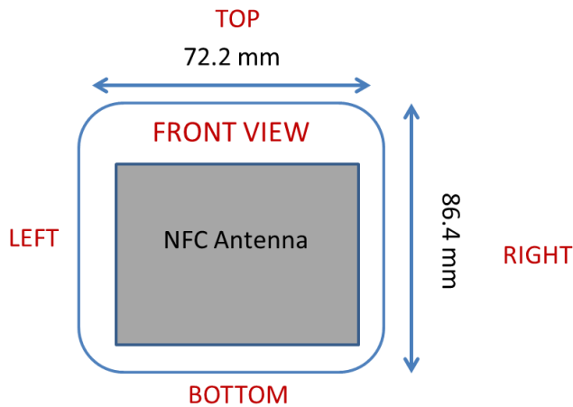
Figure E-4 NFC Antenna Location – Closed Configuration
