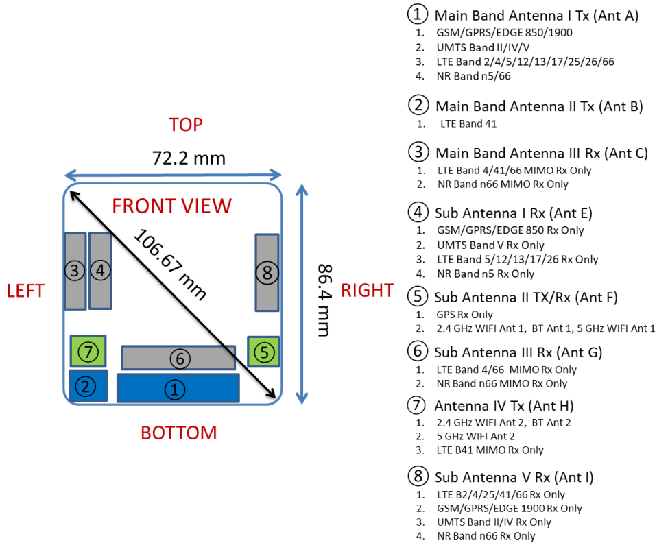
Figure E-3 DUT Antenna Locations – Closed Configuration
