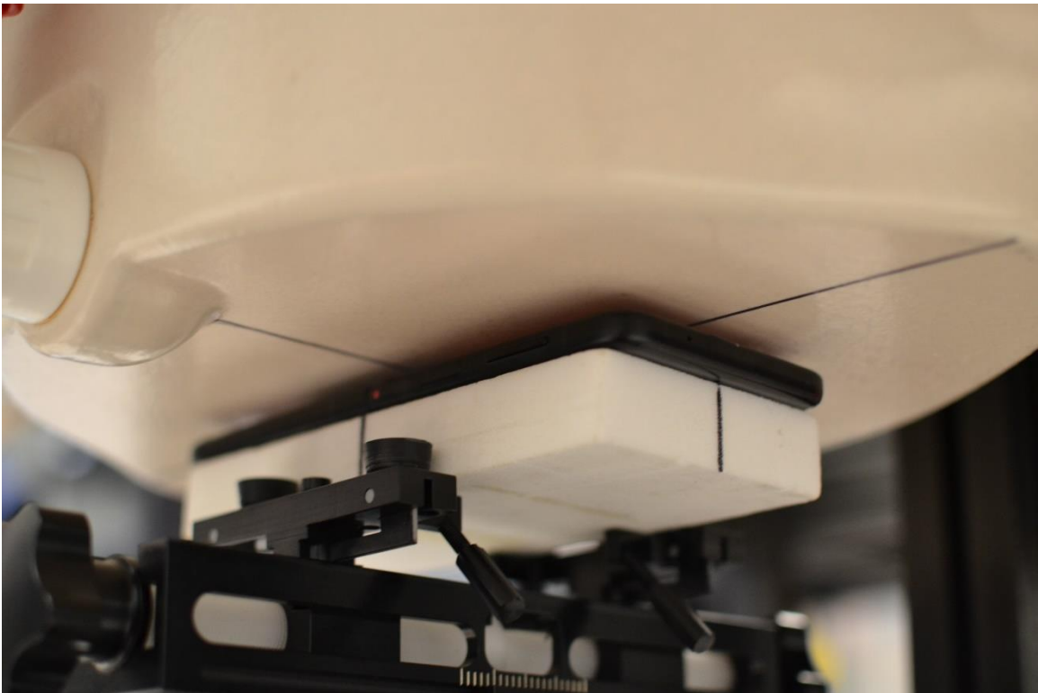
SAR Test Setup Photo 10 – Hotspot, Front Side, 6 mm
