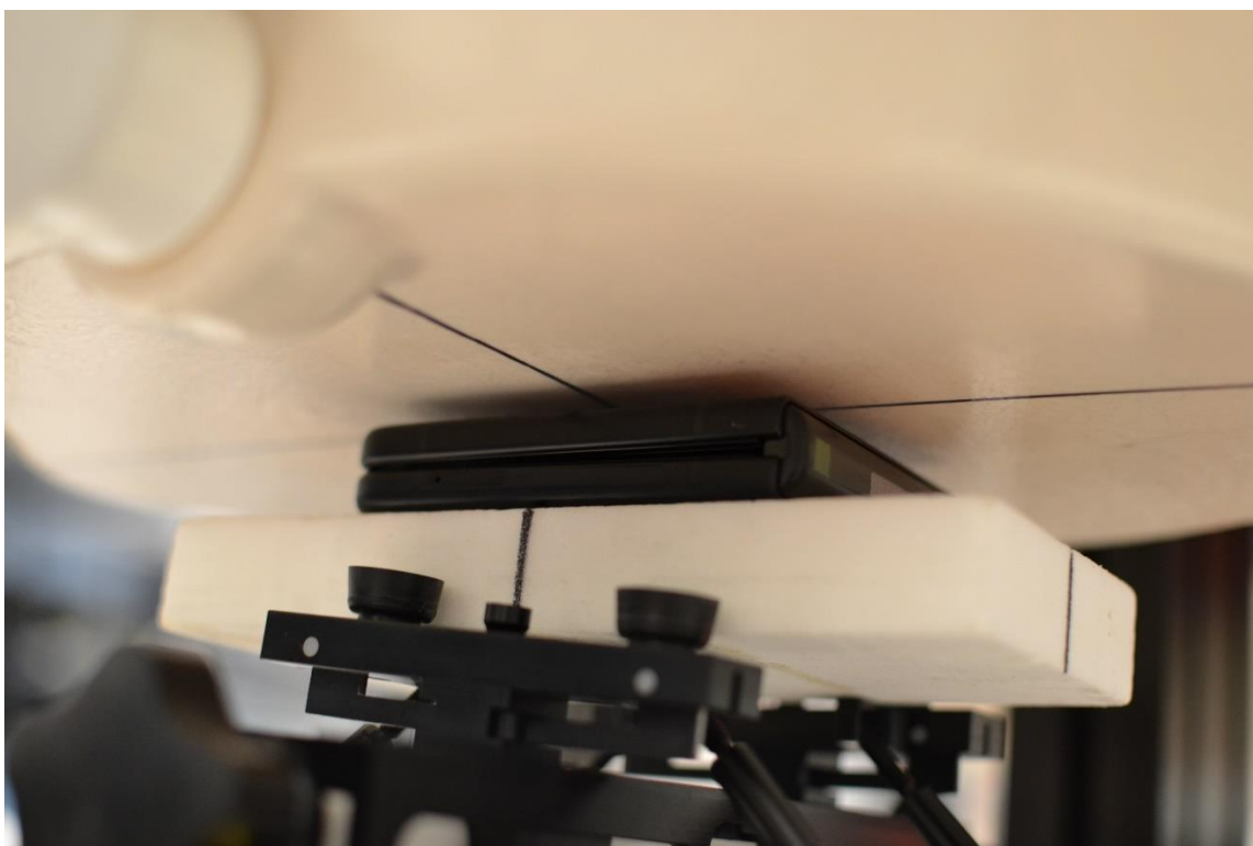
SAR Test Setup Photo 23 – Closed Hotspot, Back Side, 5 mm
