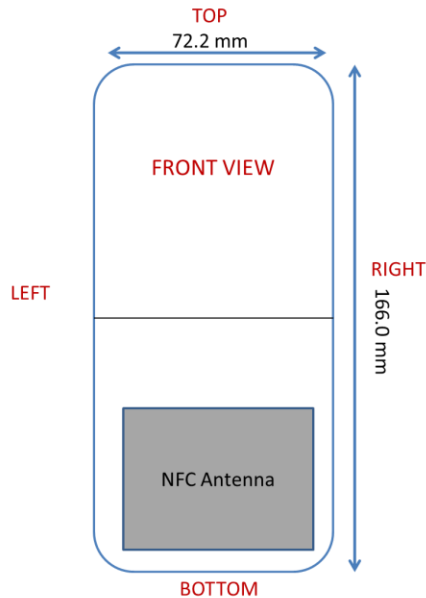
Figure E-2 NFC Antenna Location – Open Configuration
