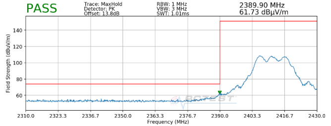
Plot 7-104. Radiated Restricted Band Edge Measurement MIMO with WCP (Peak)
