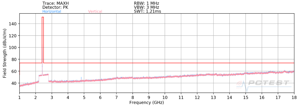
Plot 7-79. Radiated Spurious Plot above 1GHz CDD (802.11b – Ch. 1) – OPEN
