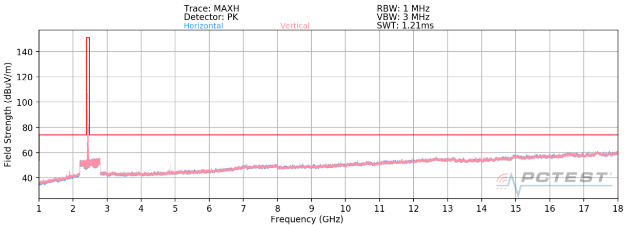
Plot 7-72. Radiated Spurious Plot above 1GHz SISO ANT2 (802.11b – Ch. 6) – OPEN
