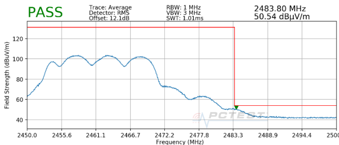
Plot 7-97. Radiated Restricted Upper Band Edge Measurement MIMO (Average)
