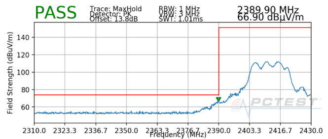
Plot 7-96. Radiated Restricted Lower Band Edge Measurement MIMO (Peak)
