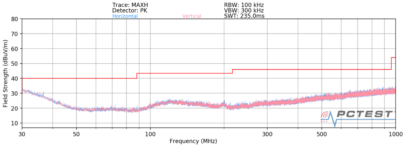
Plot 7-106. Radiated Spurious Plot below 1GHz MIMO – CLOSED
