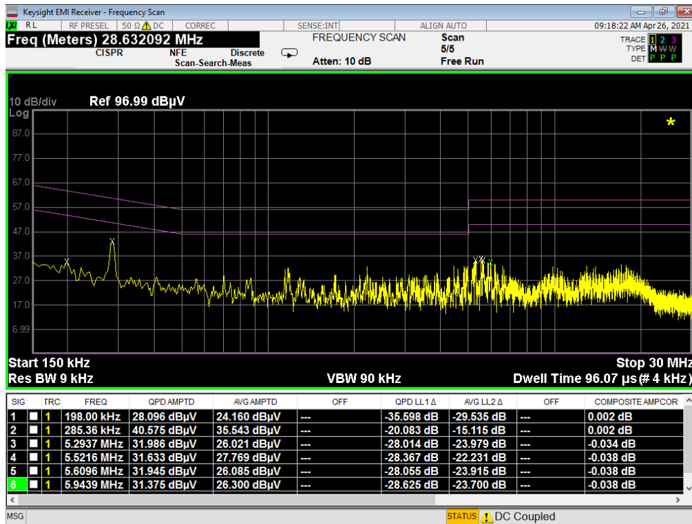
Plot 7-110. Line Conducted Plot with 802.11b (N) – CLOSED
