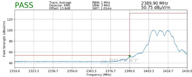
Plot 7-103. Radiated Restricted Band Edge Measurement MIMO with WCP (Average)
