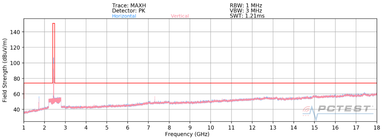
Plot 7-75. Radiated Spurious Plot above 1GHz SISO ANT2 (802.11b – Ch. 6) – CLOSED
