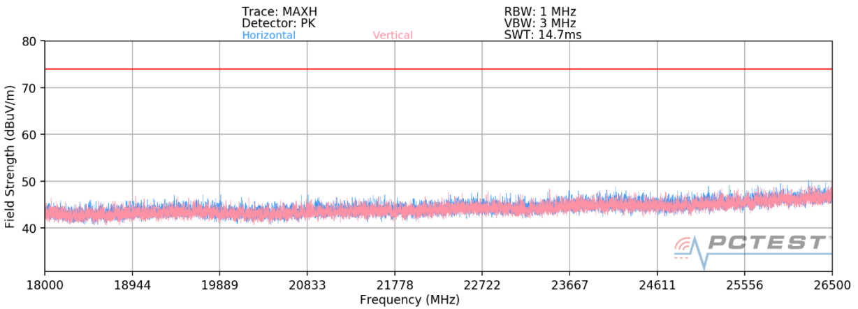
Plot 7-78. Radiated Spurious Plot above 18GHz SISO ANT2- CLOSED
