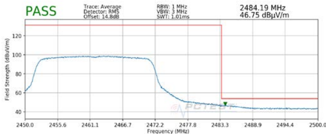
Plot 7-89. Radiated Restricted Upper Band Edge Measurement SISO ANT2 (Average)
