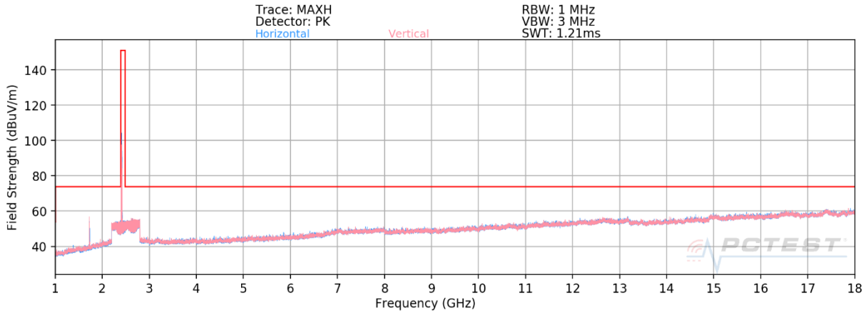
Plot 7-74. Radiated Spurious Plot above 1GHz SISO ANT2 (802.11b – Ch. 1) – CLOSED
