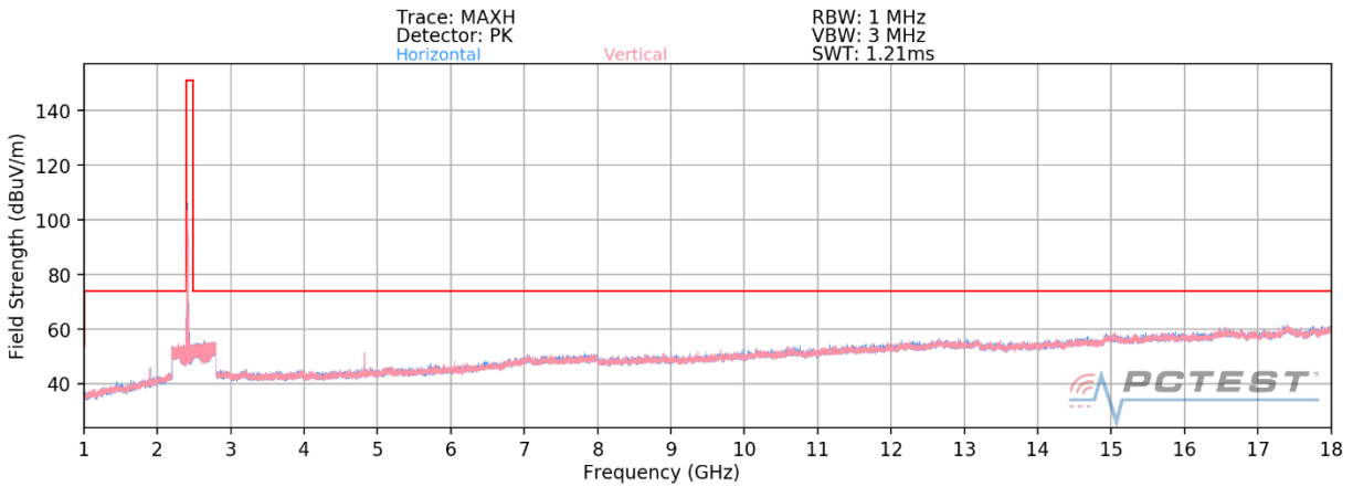
Plot 7-71. Radiated Spurious Plot above 1GHz SISO ANT2 (802.11b – Ch. 1) – OPEN
