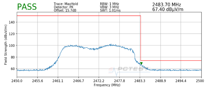
Plot 7-102. Radiated Restricted Upper Band Edge Measurement MIMO (Peak)
