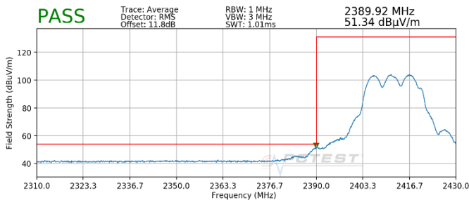
Plot 7-95. Radiated Restricted Lower Band Edge Measurement MIMO (Average)
