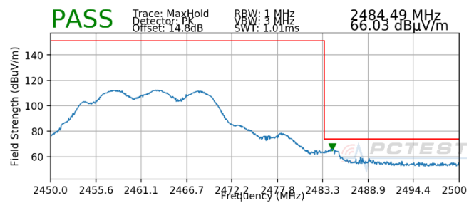
Plot 7-98. Radiated Restricted Upper Band Edge Measurement MIMO (Peak)
