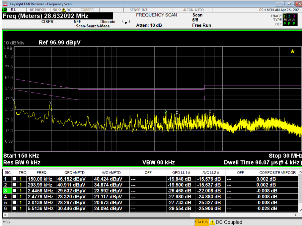
Plot 7-109. Line Conducted Plot with 802.11b (L1) – CLOSED
