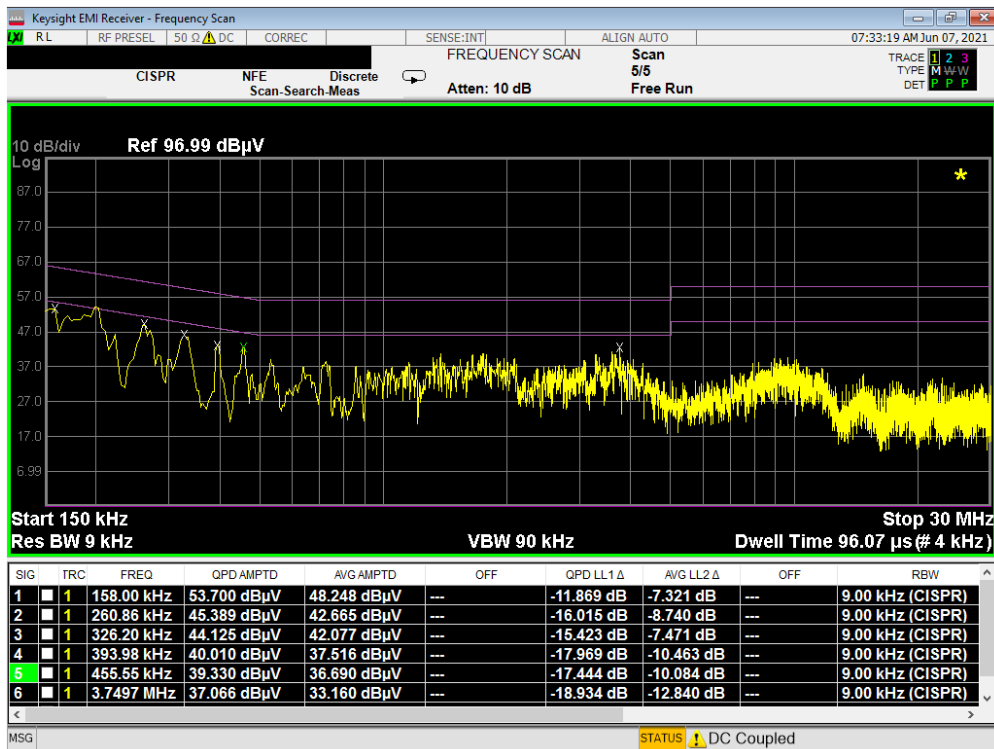
Plot 7-112. Line Conducted Plot with 802.11b with WCP
