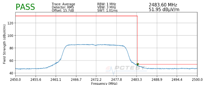
Plot 7-93. Radiated Restricted Upper Band Edge Measurement SISO ANT2 (Average)
