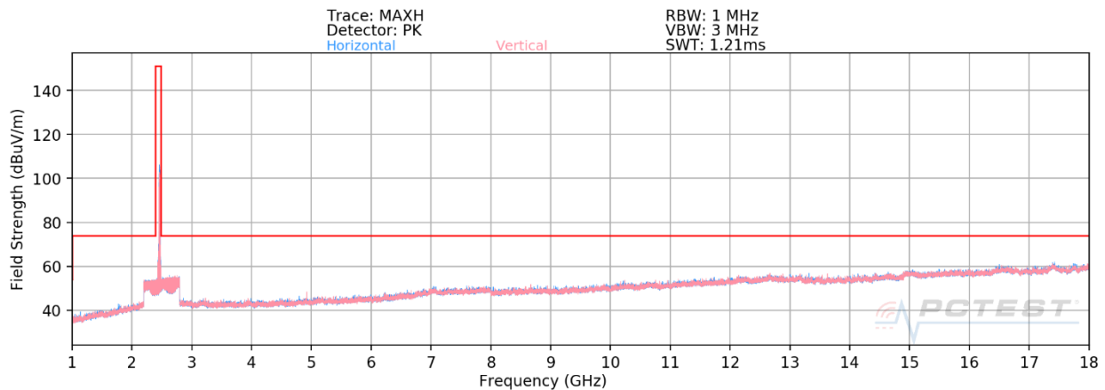
Plot 7-73. Radiated Spurious Plot above 1GHz SISO ANT2 (802.11b – Ch. 11) – OPEN
