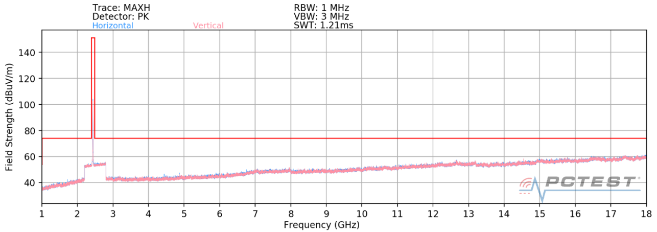
Plot 7-80. Radiated Spurious Plot above 1GHz CDD (802.11b – Ch. 6) – OPEN
