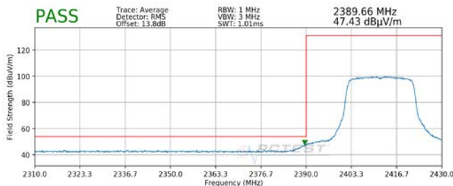
Plot 7-87. Radiated Restricted Lower Band Edge Measurement SISO ANT2 (Average)
