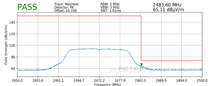
Plot 7-94. Radiated Restricted Upper Band Edge Measurement SISO ANT2 (Peak)
