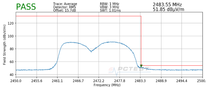
Plot 7-101. Radiated Restricted Upper Band Edge Measurement MIMO (Average)
