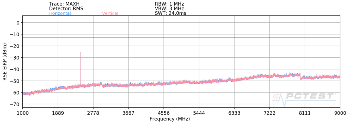
Plot 7-22. Radiated Spurious Plot (LTE Band 26) – Closed
