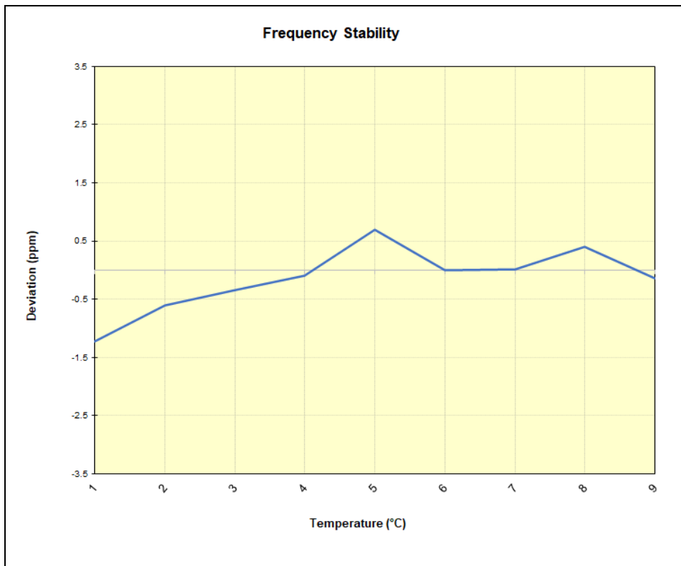
Plot 7-103. LTE Band 25/2 Frequency Stability Chart
