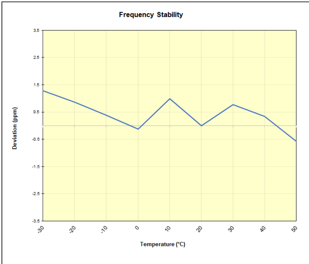
Plot 7-104. GSM/GPRS PCS Frequency Stability Chart
