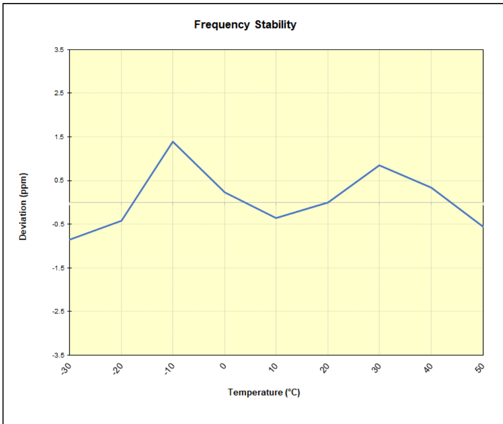
Plot 7-105. WCDMA PCS Frequency Stability Chart
