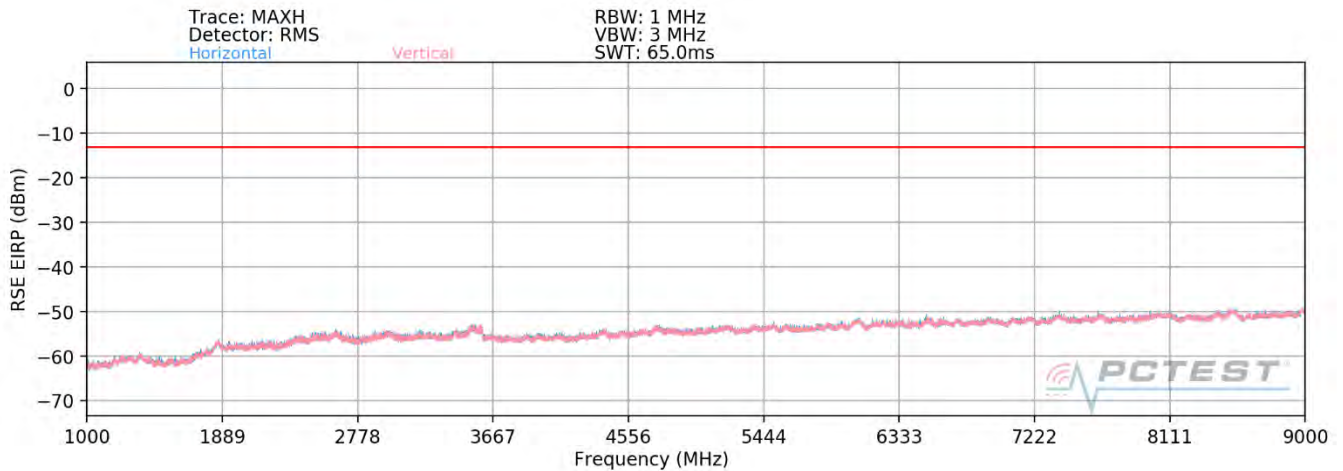
Plot 7-87. Radiated Spurious Plot (NR Band n5) – Half
