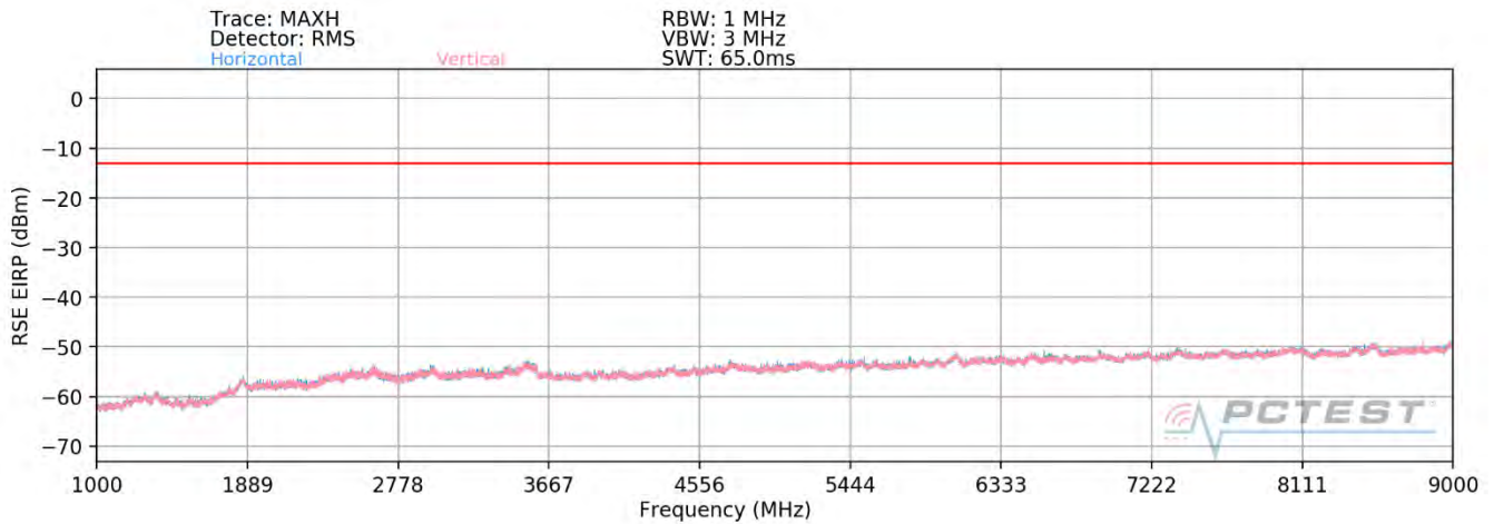
Plot 7-91. Radiated Spurious Plot (WCDMA Cell) – Half
