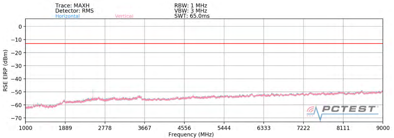
Plot 7-89. Radiated Spurious Plot (GPRS Cell) – Open
