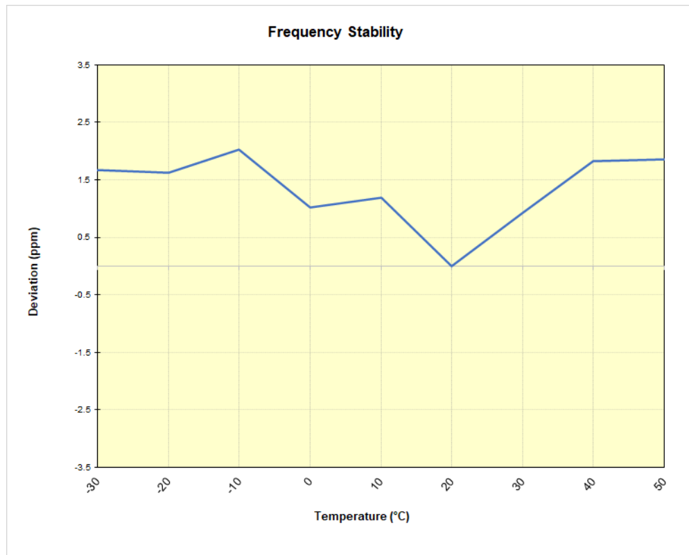
Plot 7-94. GSM/GPRS Cell Frequency Stability Chart
