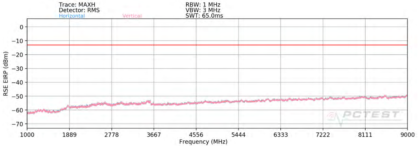
Plot 7-90. Radiated Spurious Plot (WCDMA Cell) – Closed
