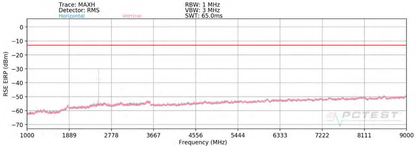
Plot 7-84. Radiated Spurious Plot (LTE Band 26/5) – Closed
