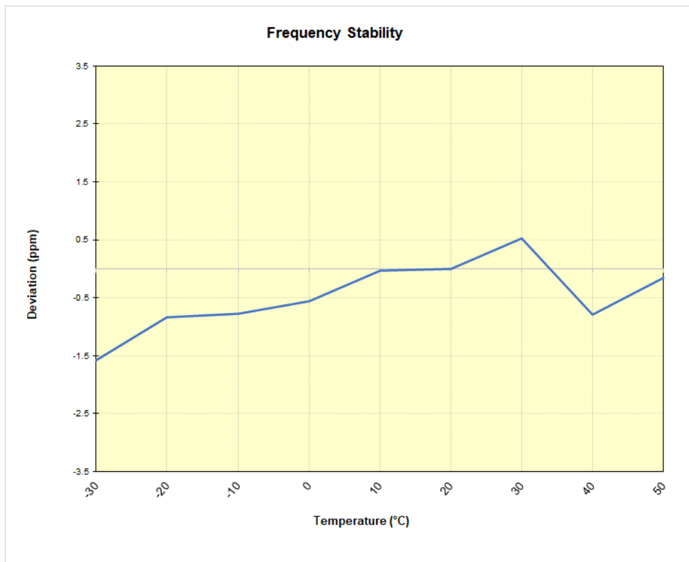
Plot 7-93. NR Band n5 Frequency Stability Chart
