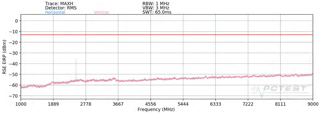
Plot 7-86. Radiated Spurious Plot (NR Band n5) – Closed
