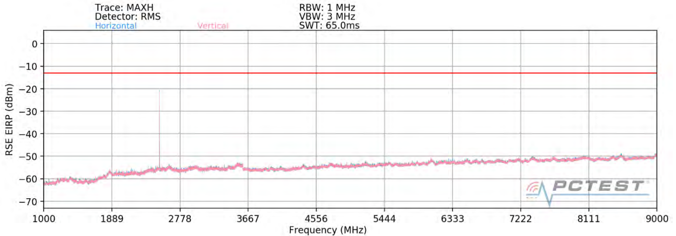
Plot 7-88. Radiated Spurious Plot (GPRS Cell) – Closed
