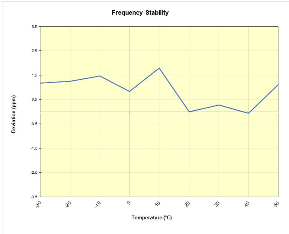
Plot 7-95. WCDMA Cell Frequency Stability Chart
