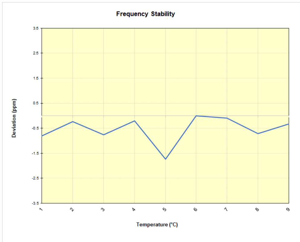
Plot 7-92. LTE Band 26/5 Frequency Stability Chart
