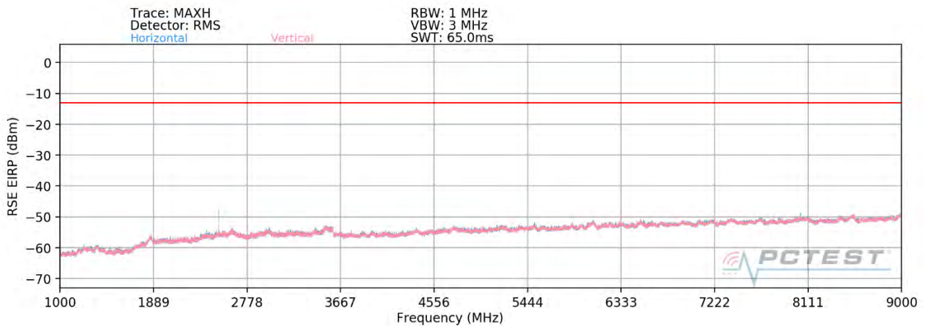
Plot 7-85. Radiated Spurious Plot (LTE Band 26/5) - Half
