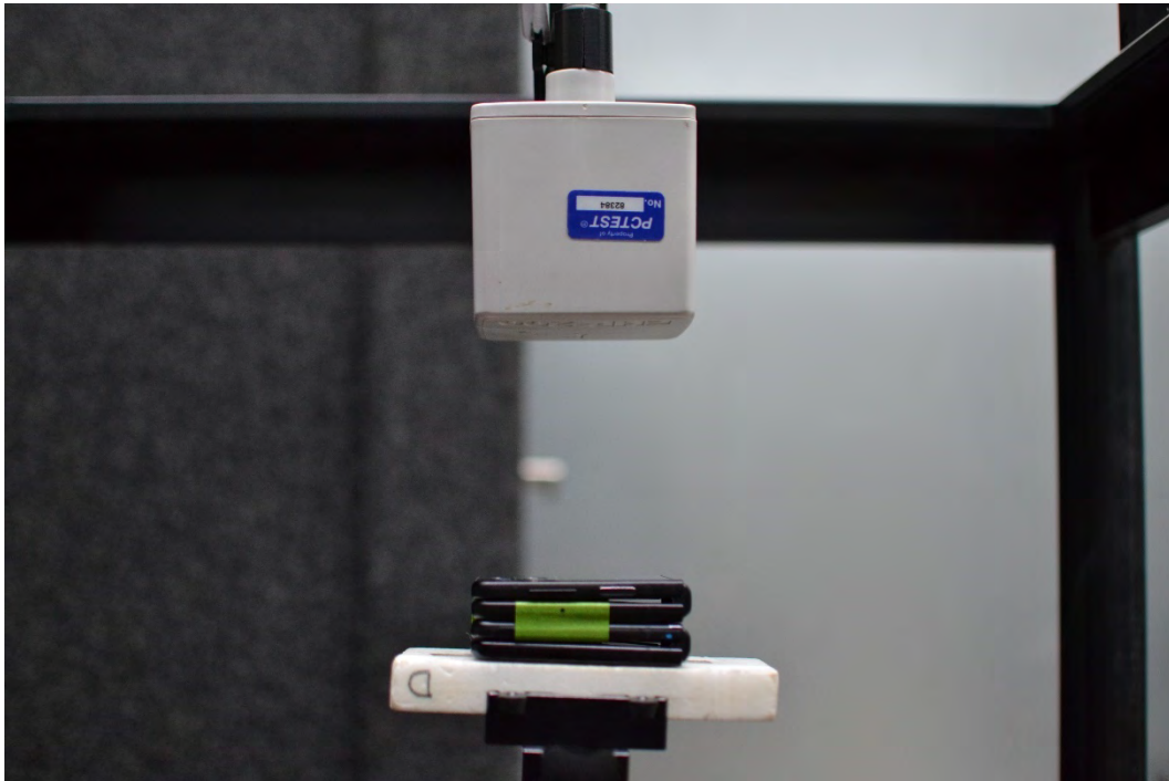
Plot 11. H-field – 15cm
