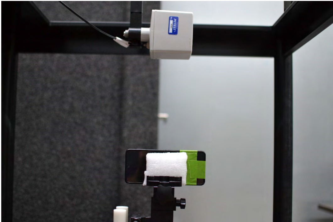
Plot 24. E-field – 20cm
