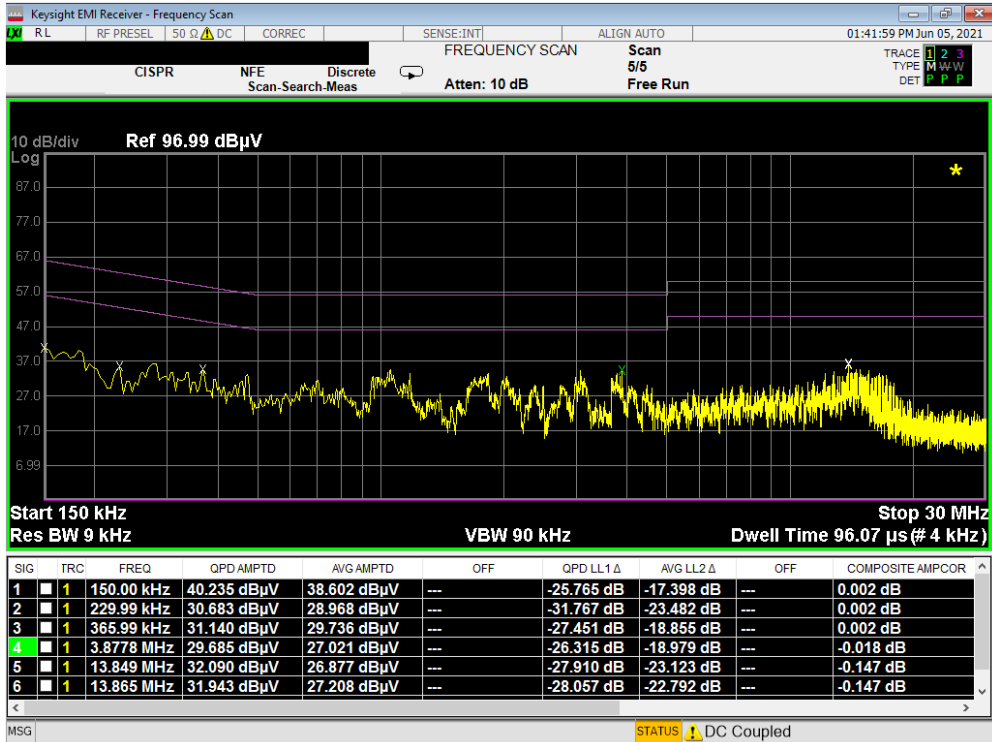
Plot 7-10. Line-Conducted Test Plot (N) - Device to Device WPT_Variant N
