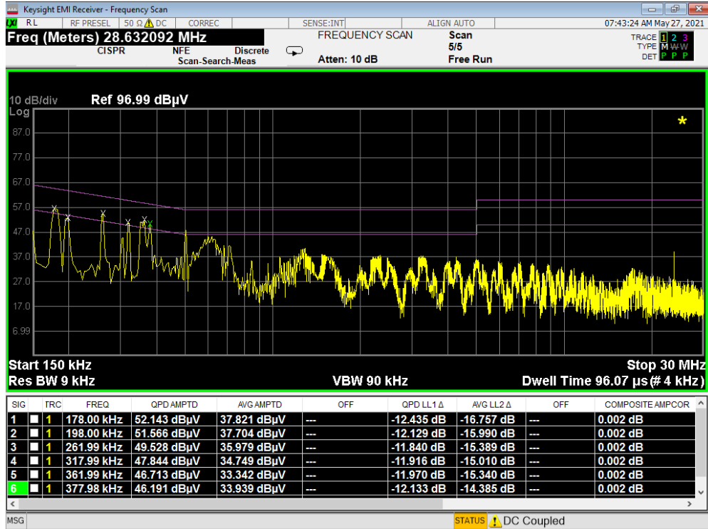
Plot 7-7. Line-Conducted Test Plot (L1) - Device to Device WPT_Variant Q
