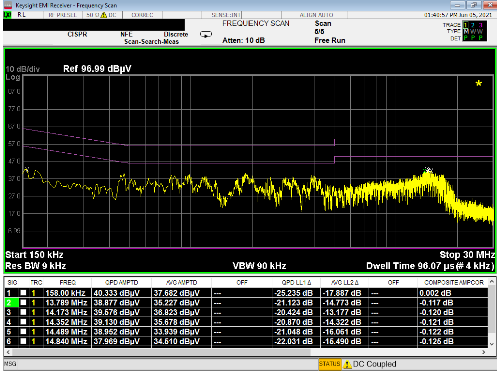
Plot 7-9. Line-Conducted Test Plot (L1) - Device to Device WPT_Variant N
