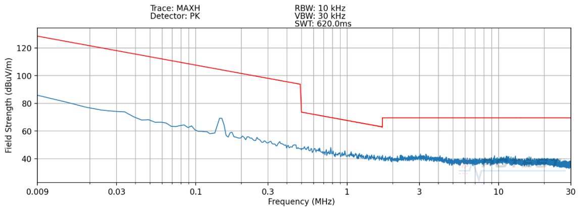
Plot 7-5 Radiated Spurious Plot 9kHz – 30MHz (Pol. Y – Device to Device WPT) _Variant N
