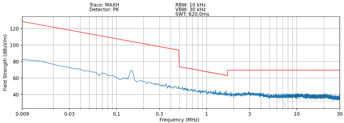
Plot 7-2 Radiated Spurious Plot 9kHz – 30MHz (Pol. Y – Device to Device WPT) _Variant Q
