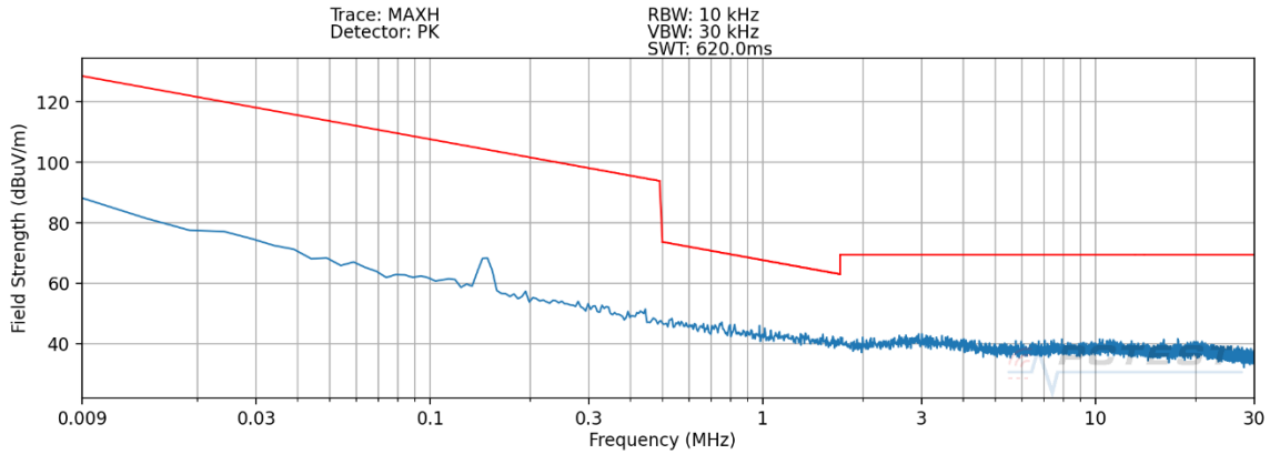
Plot 7-1. Radiated Spurious Plot 9kHz – 30MHz (Pol. X – Device to Device WPT) _Variant Q
