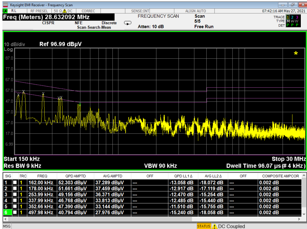
Plot 7-8. Line-Conducted Test Plot (N) - Device to Device WPT_Variant Q
