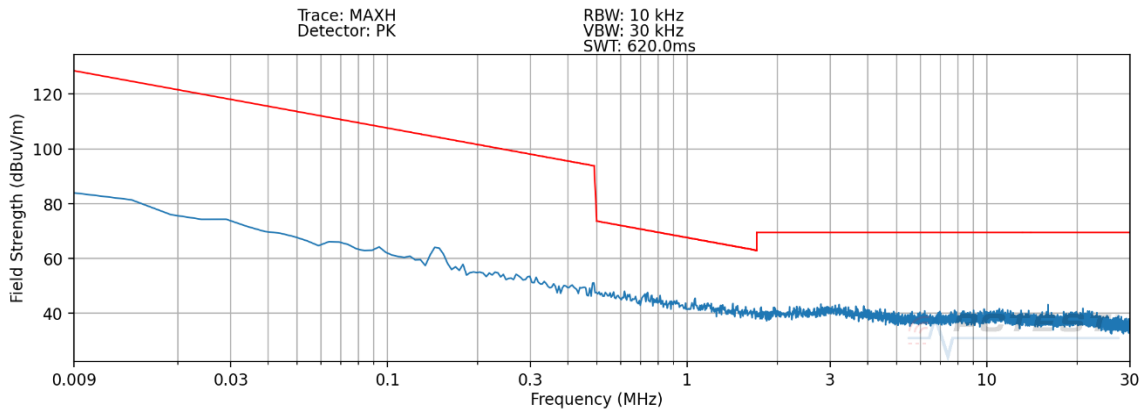
Plot 7-6. Radiated Spurious Plot 9kHz – 30MHz (Pol. Z – Device to Device WPT) _Variant N
