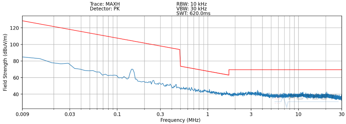
Plot 7-4. Radiated Spurious Plot 9kHz – 30MHz (Pol. X – Device to Device WPT) _Variant N
