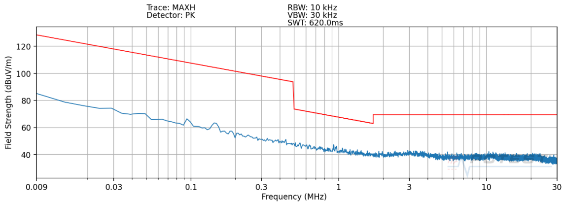
Plot 7-3. Radiated Spurious Plot 9kHz – 30MHz (Pol. Z – Device to Device WPT) _Variant Q
