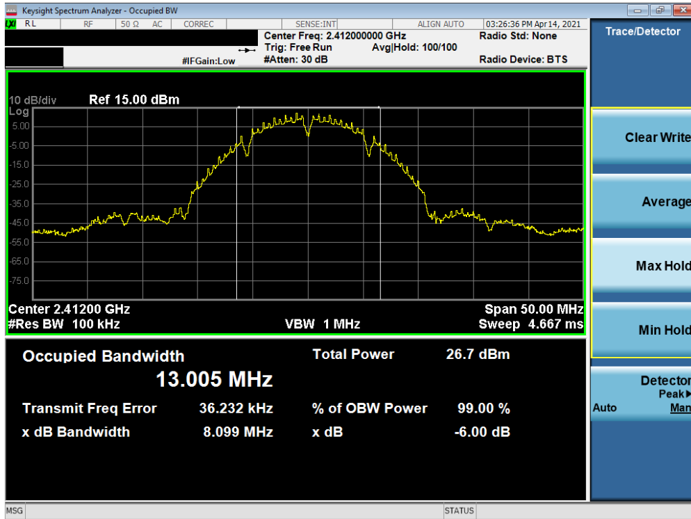
Plot 7-13. 6dB Bandwidth Plot SISO ANT2 (802.11b - Ch. 1) - N
