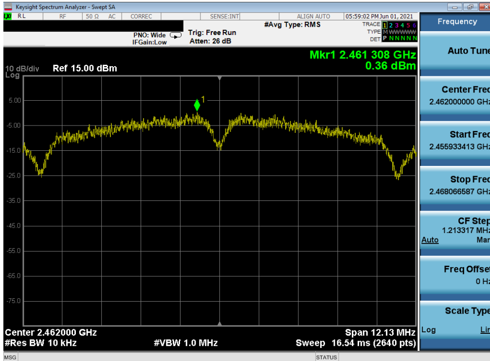
Plot 7-87. Power Spectral Density Plot MIMO ANT2 (802.11b (2.4GHz) – Ch. 11) – N
