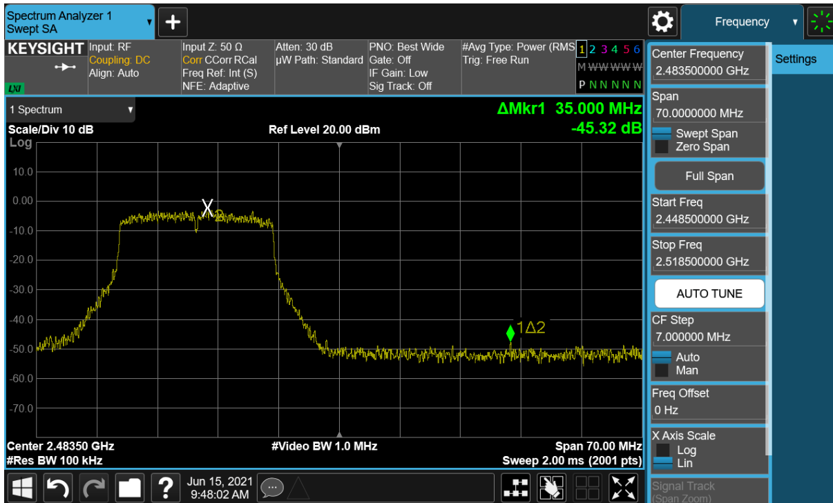
Plot 7-107. Band Edge Plot SISO ANT2 (802.11n (2.4GHz) – Ch. 12) – Q
