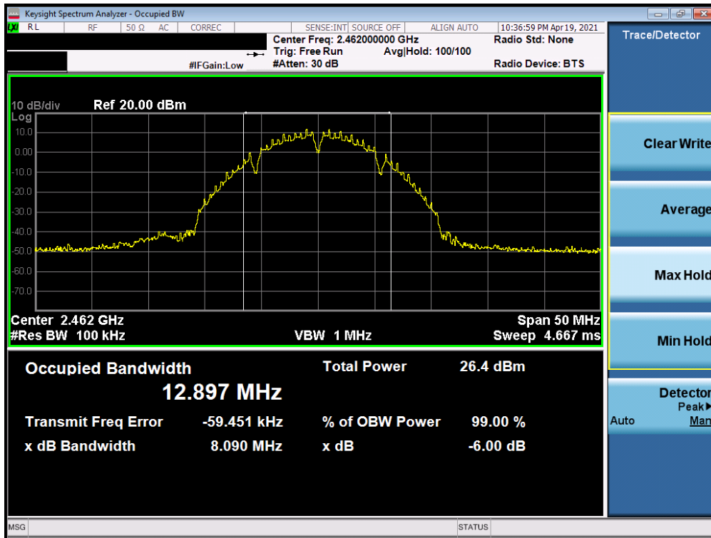
Plot 7-3. 6dB Bandwidth Plot SISO ANT2 (802.11b – Ch. 11) – Q
