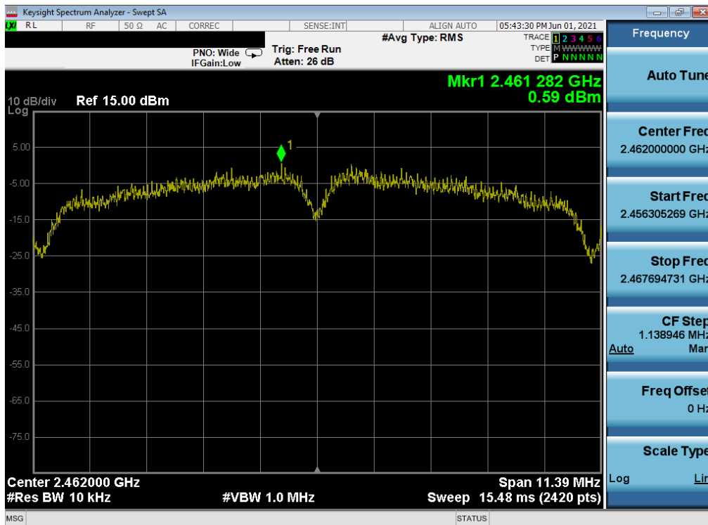
Plot 7-75. Power Spectral Density Plot MIMO ANT1 (802.11b (2.4GHz) – Ch. 11) – N
