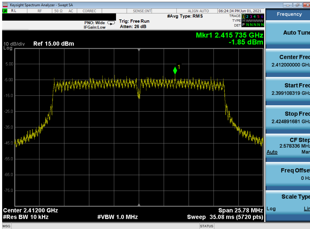
Plot 7-67. Power Spectral Density Plot MIMO ANT2 (802.11n – Ch. 1) – Q
