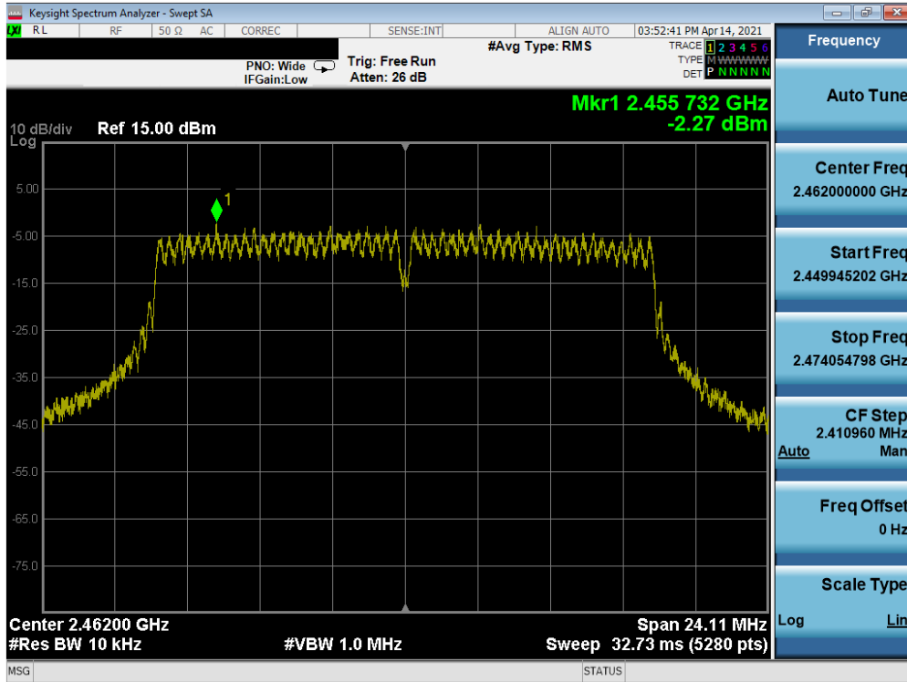
Plot 7-42. Power Spectral Density Plot SISO ANT2 (802.11g – Ch. 11) – N
