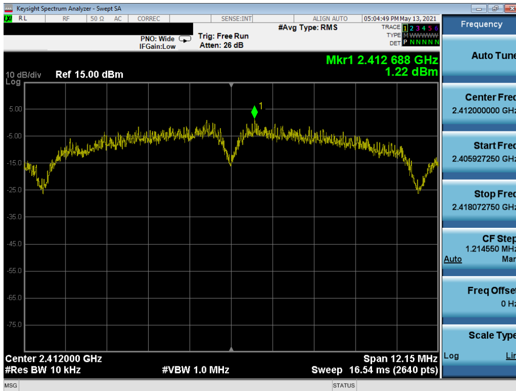
Plot 7-61. Power Spectral Density Plot MIMO ANT2 (802.11b – Ch. 1) – Q
