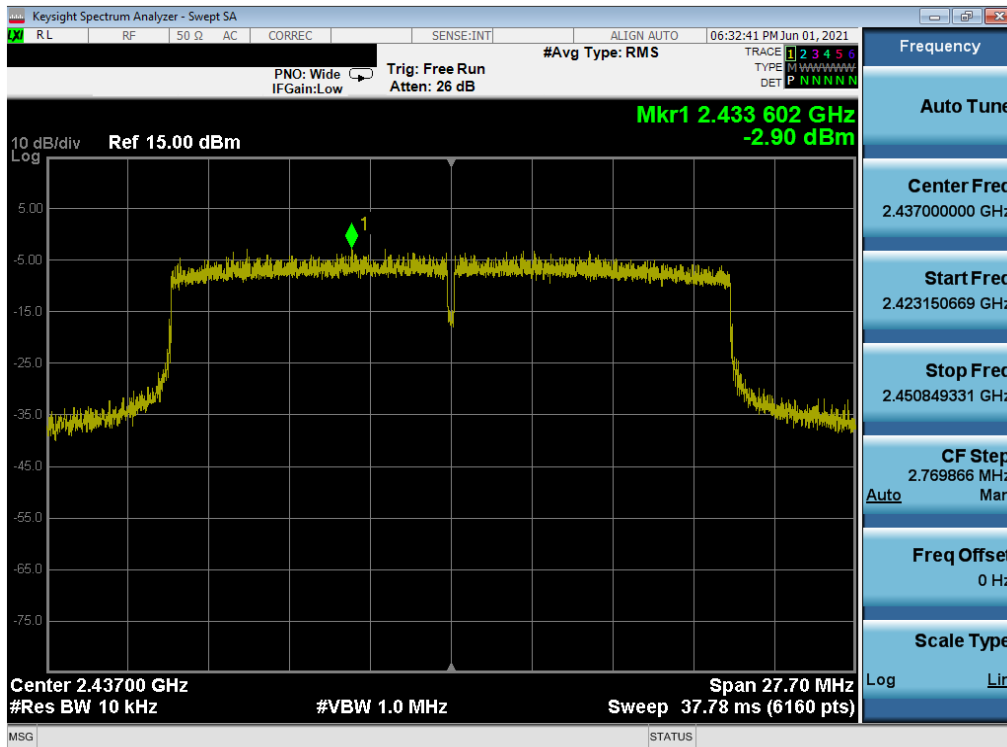
Plot 7-59. Power Spectral Density Plot MIMO ANT1 (802.11ax – Ch. 6) – Q
