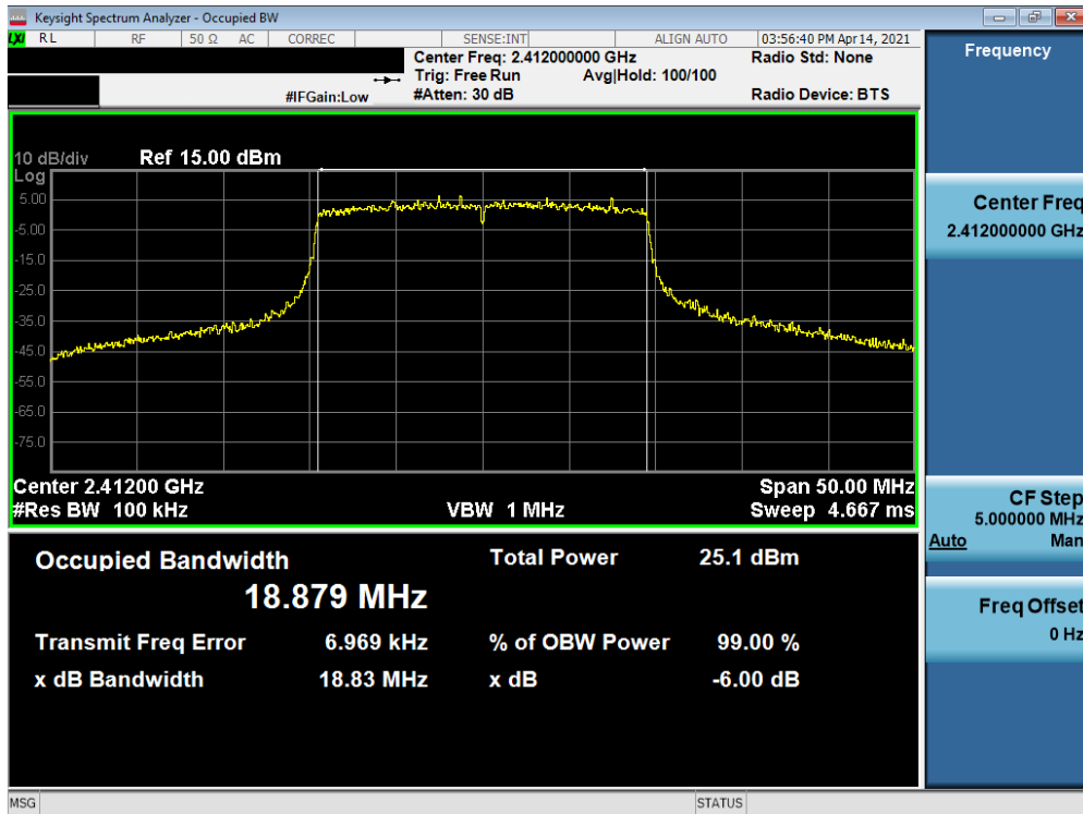
Plot 7-22. 6dB Bandwidth Plot SISO ANT2 (802.11ax (2.4GHz) – Ch. 1) – N
