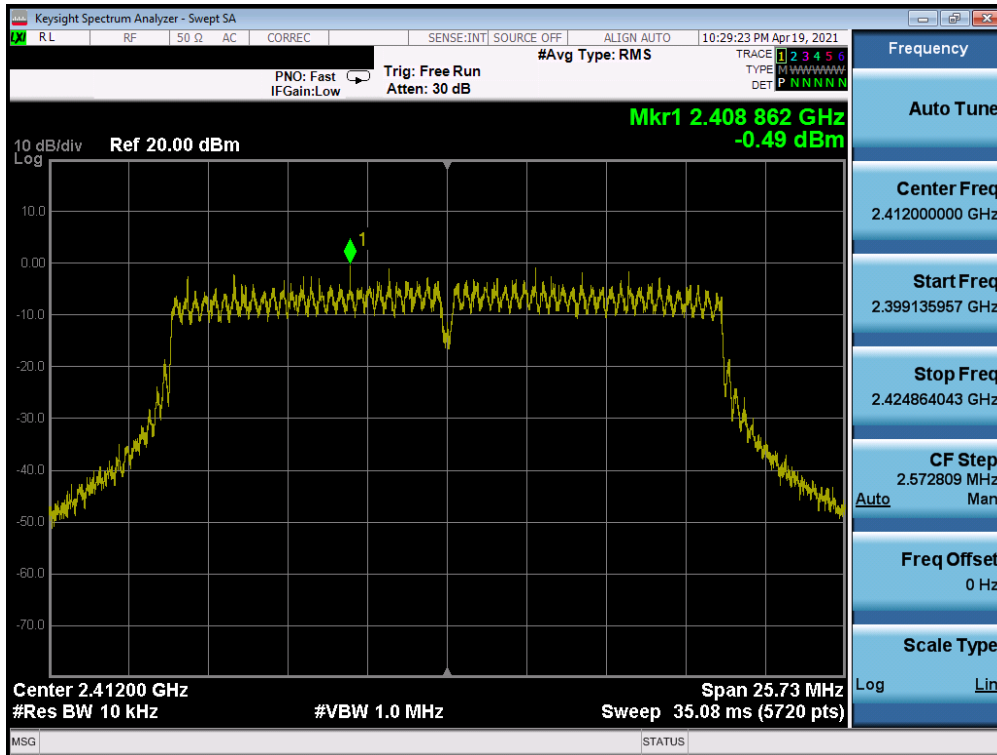
Plot 7-31. Power Spectral Density Plot SISO ANT2 (802.11n (2.4GHz) – Ch. 1) – Q
