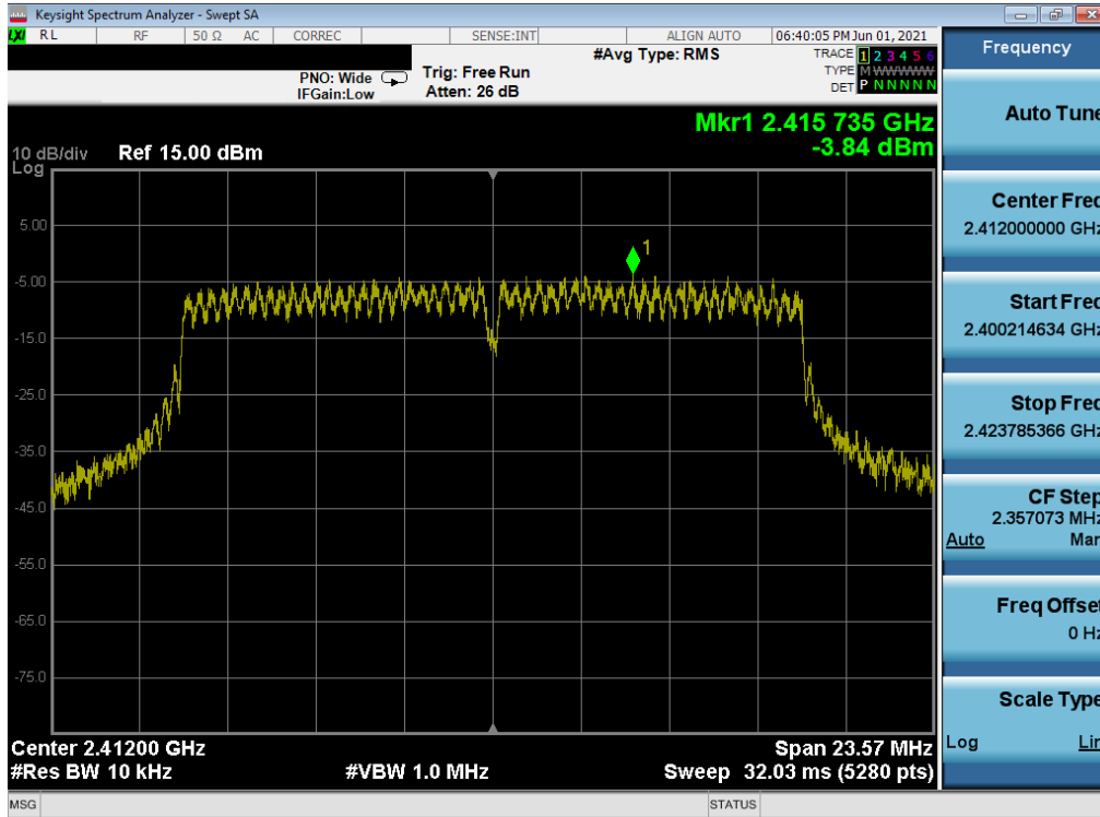
Plot 7-52. Power Spectral Density Plot MIMO ANT1 (802.11g – Ch. 1) – Q
