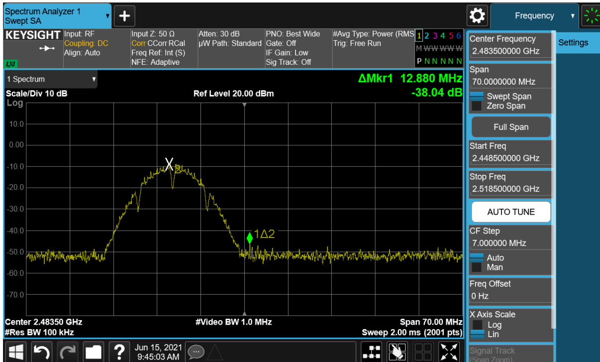
Plot 7-100. Band Edge Plot SISO ANT2 (802.11b – Ch. 13) – Q
