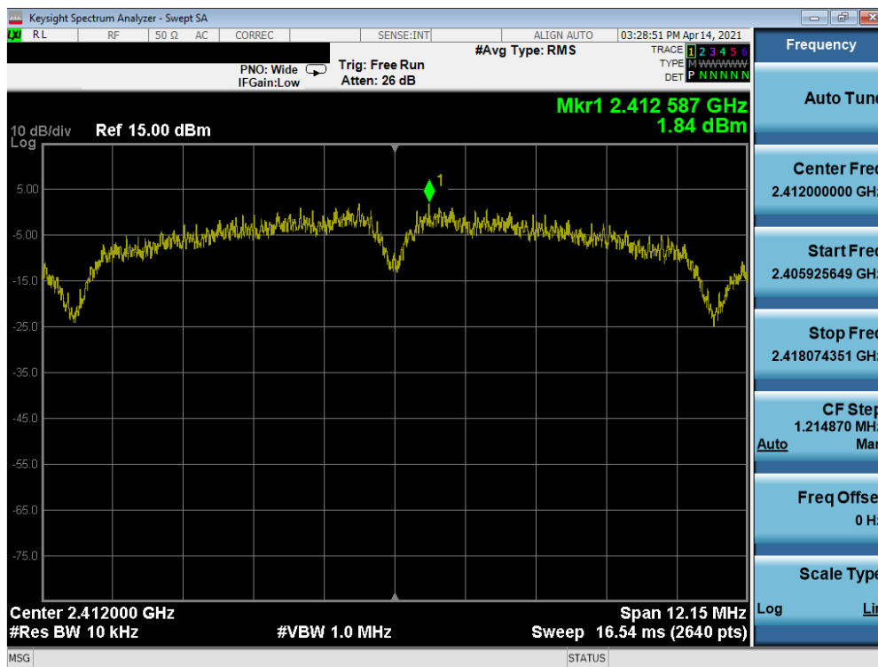
Plot 7-37. Power Spectral Density Plot SISO ANT2 (802.11b – Ch. 1) – N
