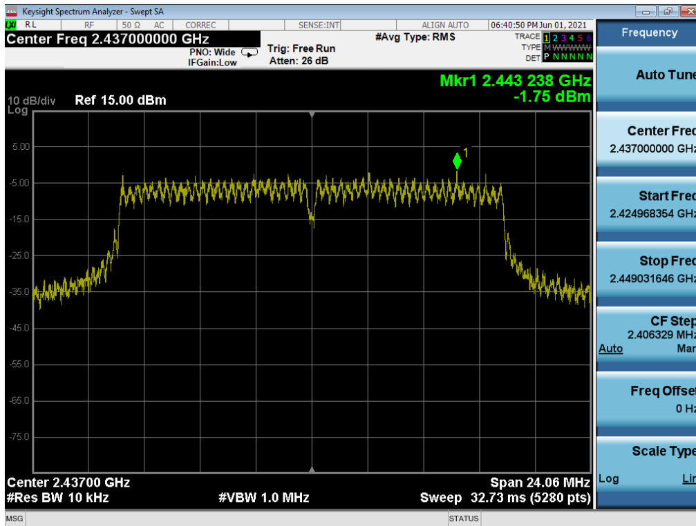
Plot 7-53. Power Spectral Density Plot MIMO ANT1 (802.11g – Ch. 6) – Q
