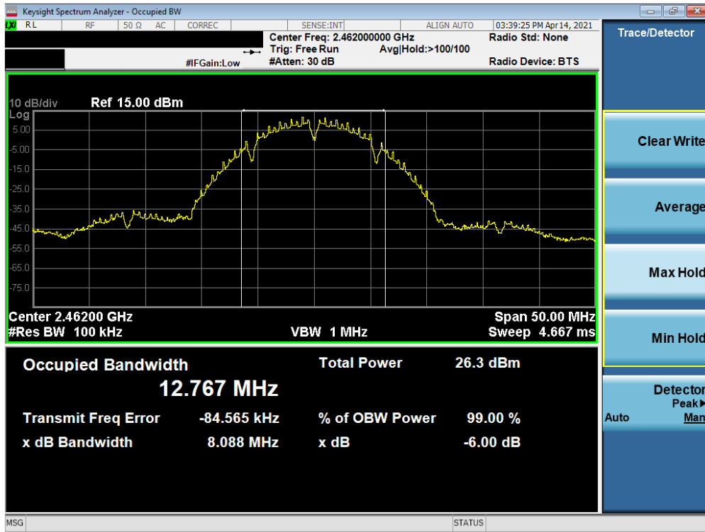
Plot 7-15. 6dB Bandwidth Plot SISO ANT2 (802.11b – Ch. 11) – N
