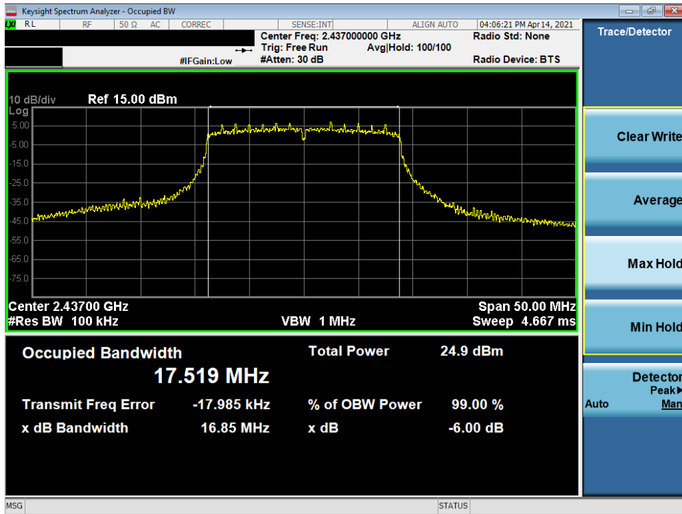
Plot 7-20. 6dB Bandwidth Plot SISO ANT2 (802.11n (2.4GHz) – Ch. 6) – N
