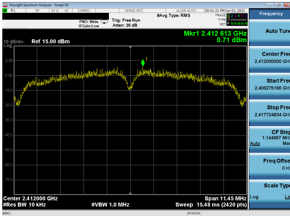
Plot 7-73. Power Spectral Density Plot MIMO ANT1 (802.11b (2.4GHz) – Ch. 1) – N
