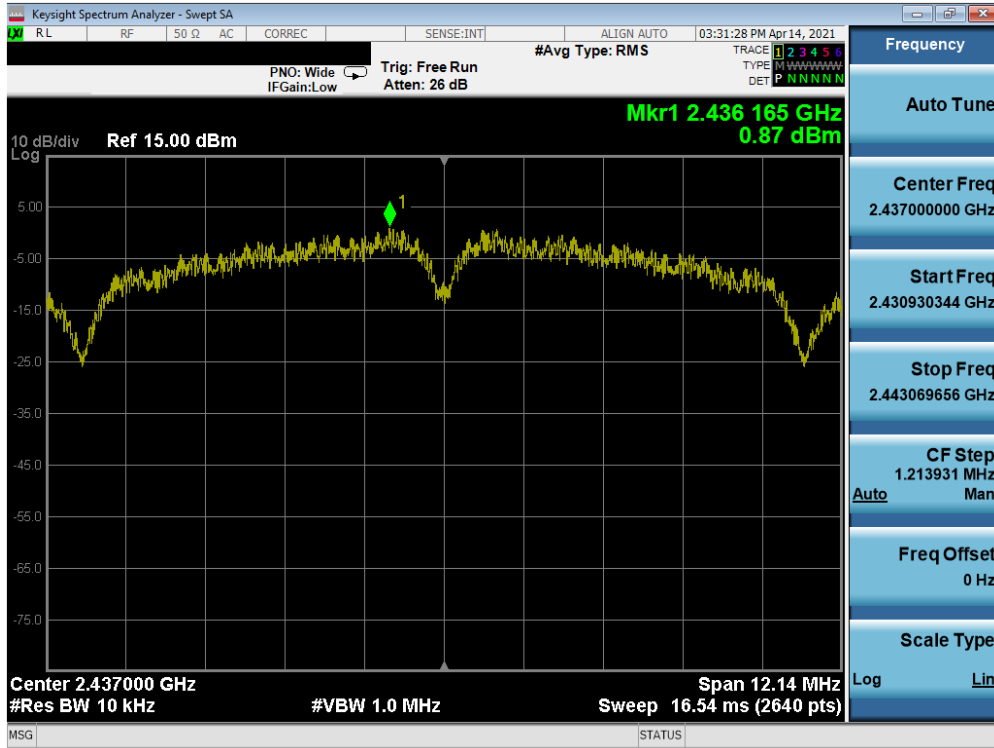
Plot 7-38. Power Spectral Density Plot SISO ANT2 (802.11b – Ch. 6) – N
