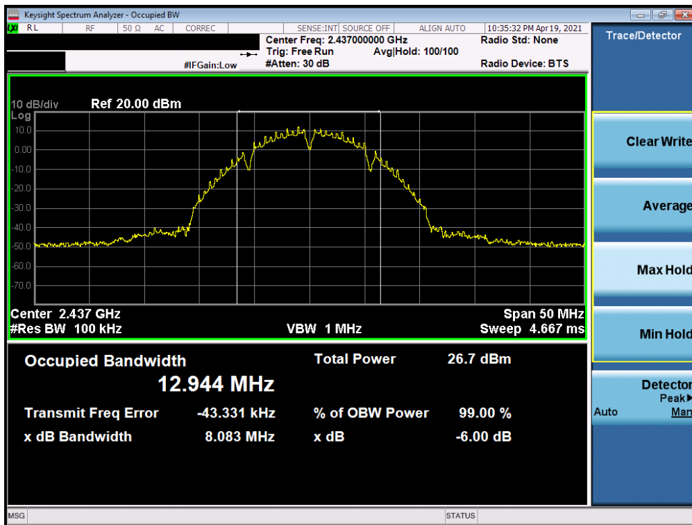
Plot 7-2. 6dB Bandwidth Plot SISO ANT2 (802.11b – Ch. 6) – Q
