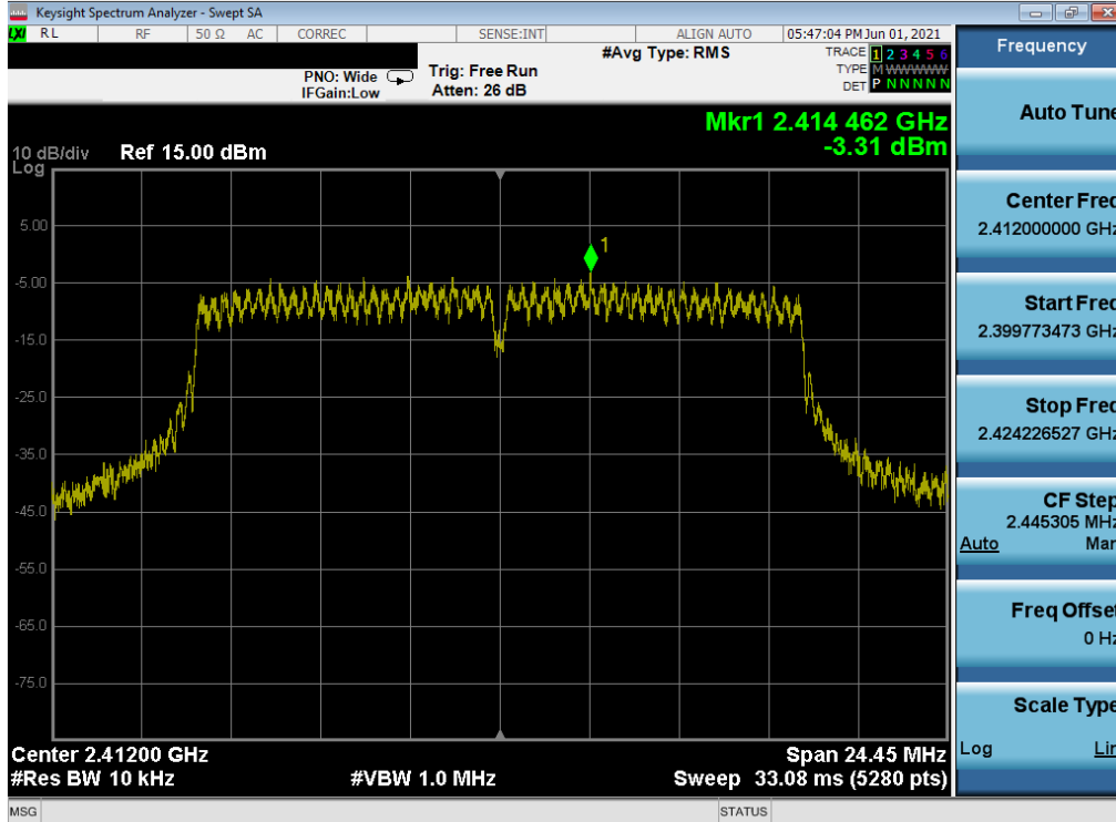
Plot 7-76. Power Spectral Density Plot MIMO ANT1 (802.11g (2.4GHz) – Ch. 1) – N
