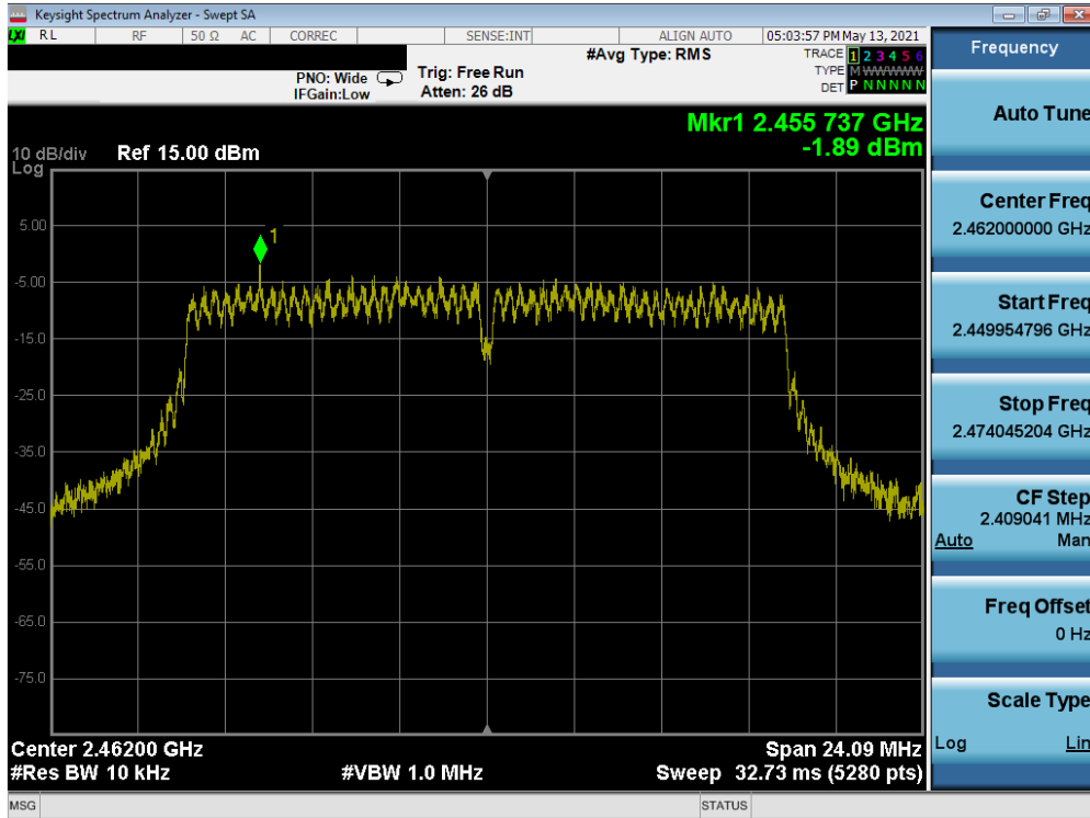
Plot 7-66. Power Spectral Density Plot MIMO ANT2 (802.11g – Ch. 11) – Q
