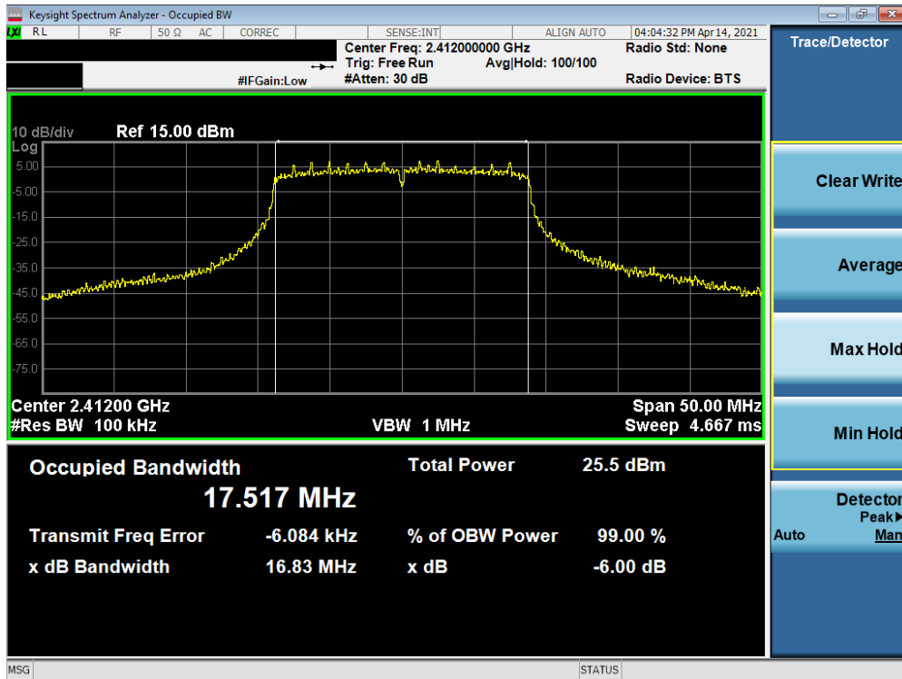
Plot 7-19. 6dB Bandwidth Plot SISO ANT2 (802.11n (2.4GHz) – Ch. 1) – N
