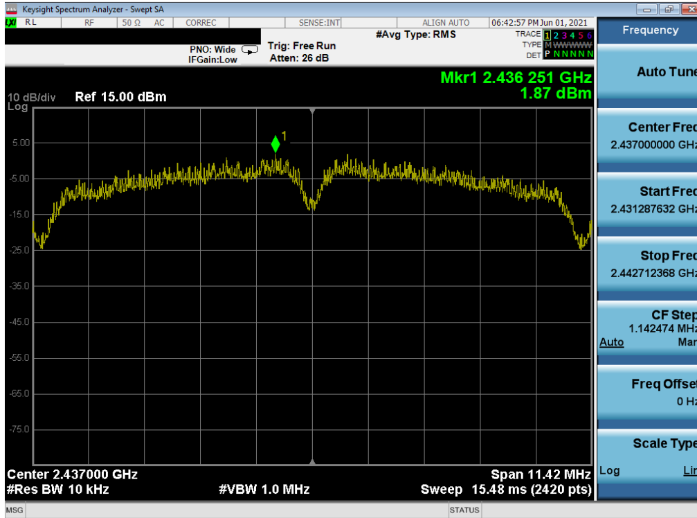
Plot 7-50. Power Spectral Density Plot MIMO ANT1 (802.11b – Ch. 6) – Q
