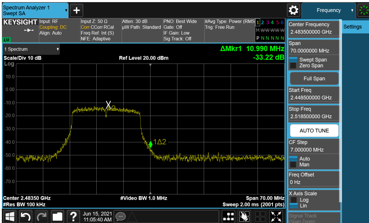
Plot 7-108. Band Edge Plot SISO ANT2 (802.11n (2.4GHz) – Ch. 13) – Q
