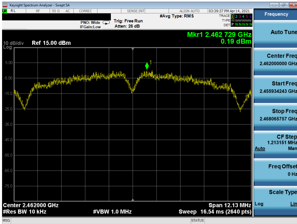
Plot 7-39. Power Spectral Density Plot SISO ANT2 (802.11b – Ch. 11) – N
