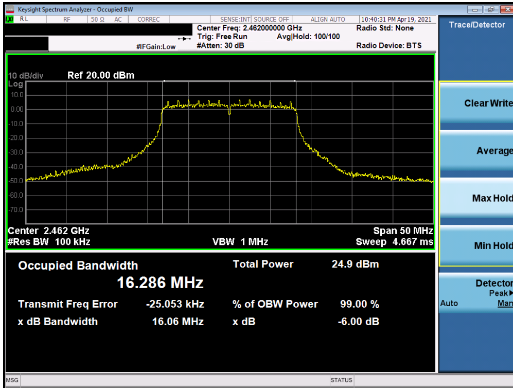
Plot 7-6. 6dB Bandwidth Plot SISO ANT (802.11g - Ch. 11) - Q
