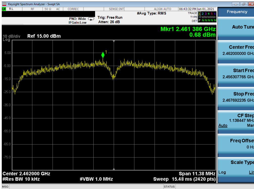
Plot 7-51. Power Spectral Density Plot MIMO ANT1 (802.11b – Ch. 11) – Q
