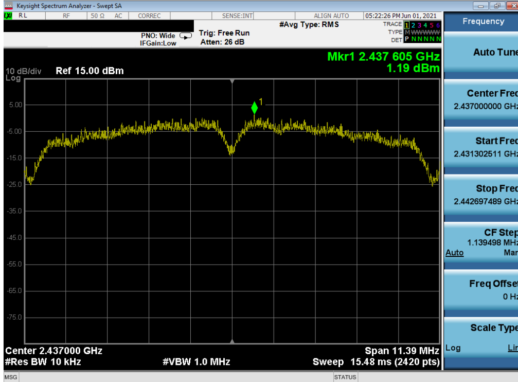
Plot 7-86. Power Spectral Density Plot MIMO ANT2 (802.11b (2.4GHz) – Ch. 6) – N
