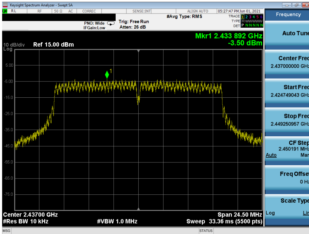
Plot 7-89. Power Spectral Density Plot MIMO ANT2 (802.11g (2.4GHz) – Ch. 6) – N
