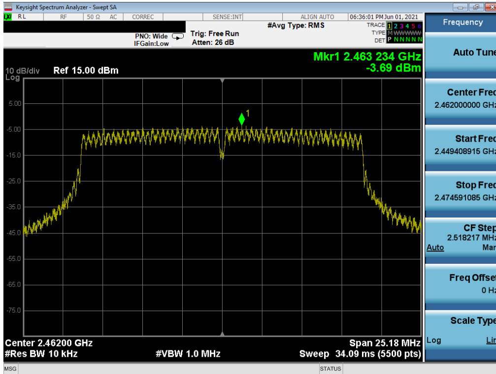
Plot 7-57. Power Spectral Density Plot MIMO ANT1 (802.11n – Ch. 11) – Q
