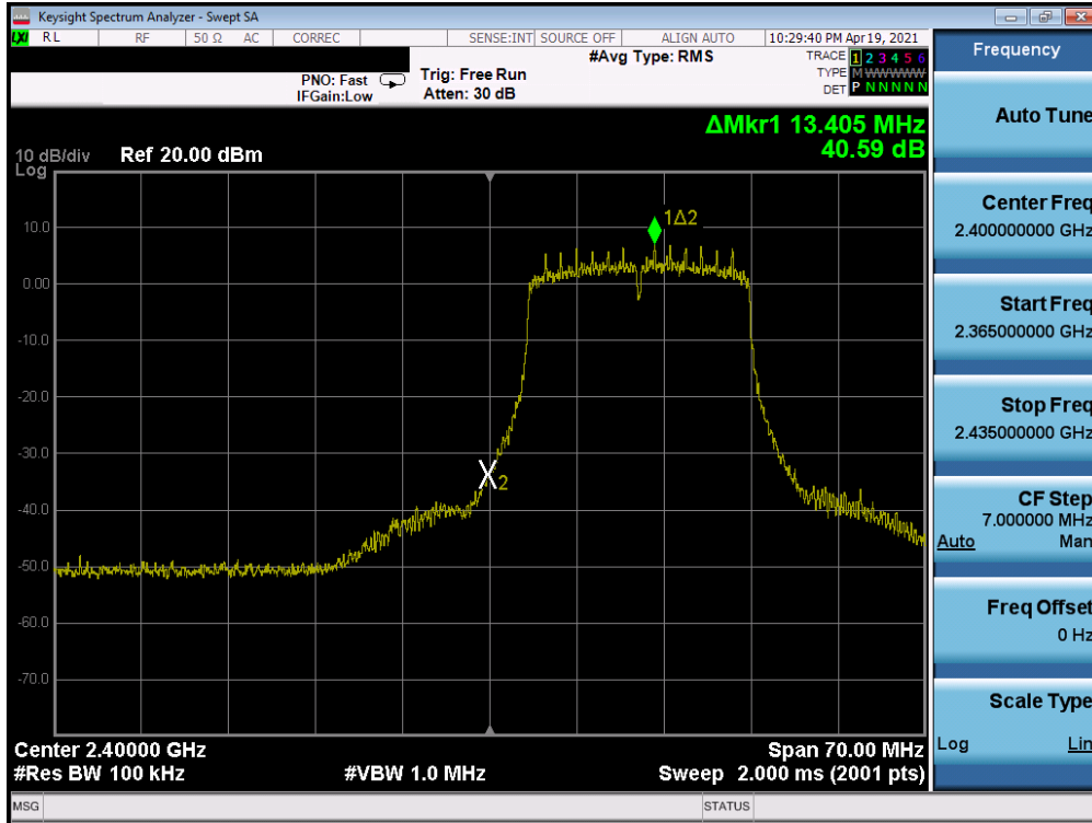
Plot 7-105. Band Edge Plot SISO ANT2 (802.11n (2.4GHz) – Ch. 1) – Q
