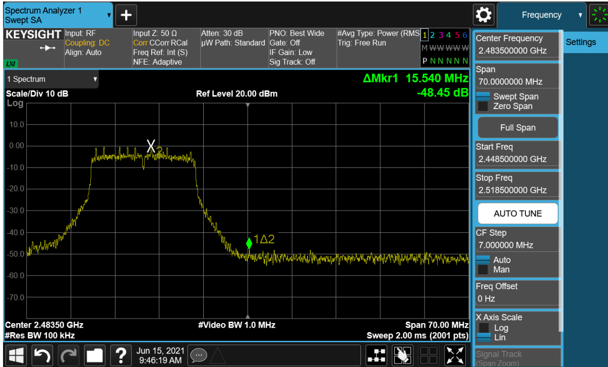
Plot 7-103. Band Edge Plot SISO ANT2 (802.11g– Ch. 12) – Q
