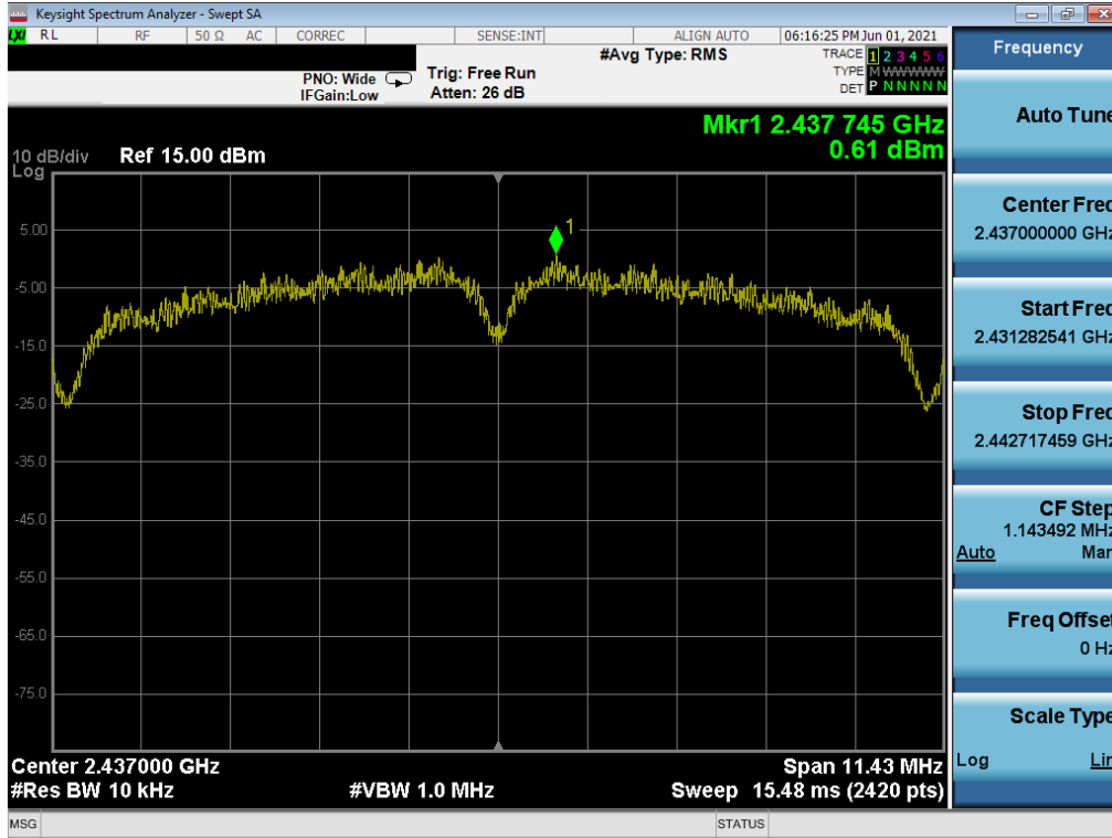
Plot 7-62. Power Spectral Density Plot MIMO ANT2 (802.11b – Ch. 6) – Q
