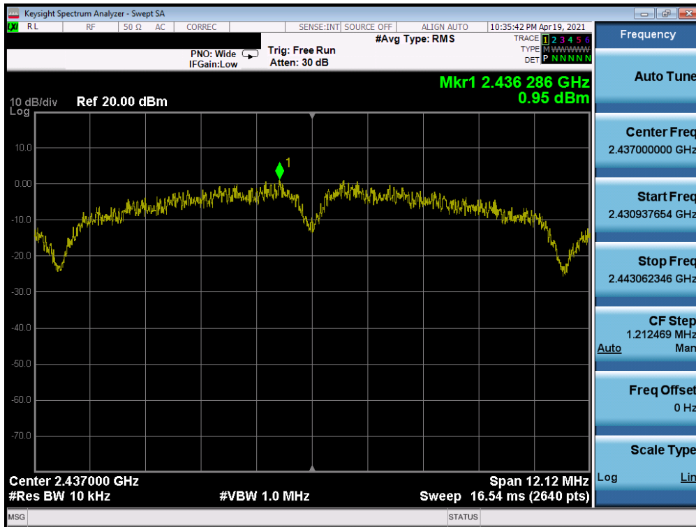
Plot 7-26. Power Spectral Density Plot SISO ANT2 (802.11b – Ch. 6) – Q
