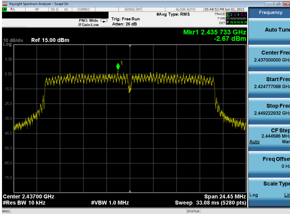
Plot 7-80. Power Spectral Density Plot MIMO ANT1 (802.11n (2.4GHz) – Ch. 6) – N
