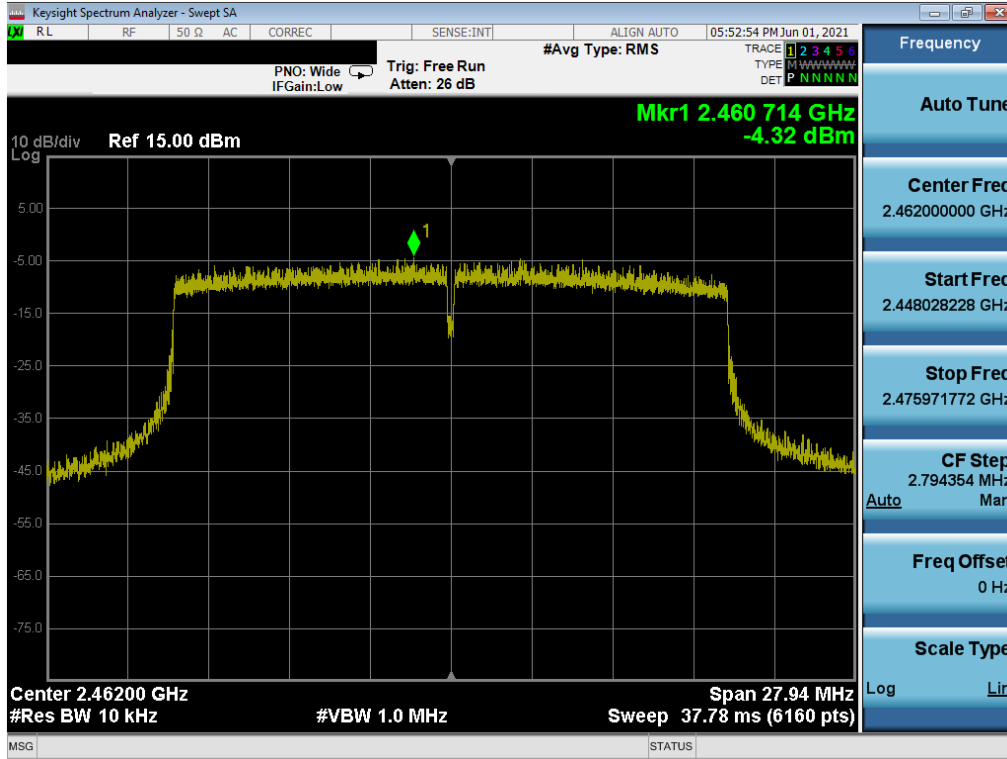
Plot 7-84. Power Spectral Density Plot MIMO ANT1 (802.11ax (2.4GHz) – Ch. 11) – N
