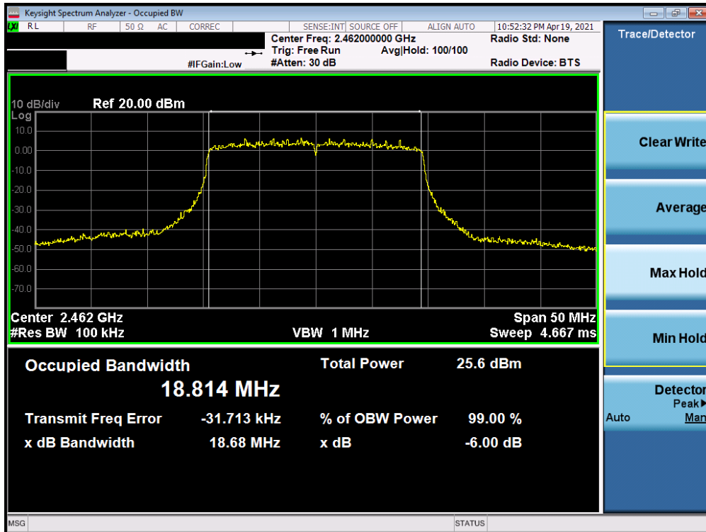
Plot 7-12. 6dB Bandwidth Plot SISO ANT2 (802.11ax (2.4GHz) – Ch. 11) – Q
