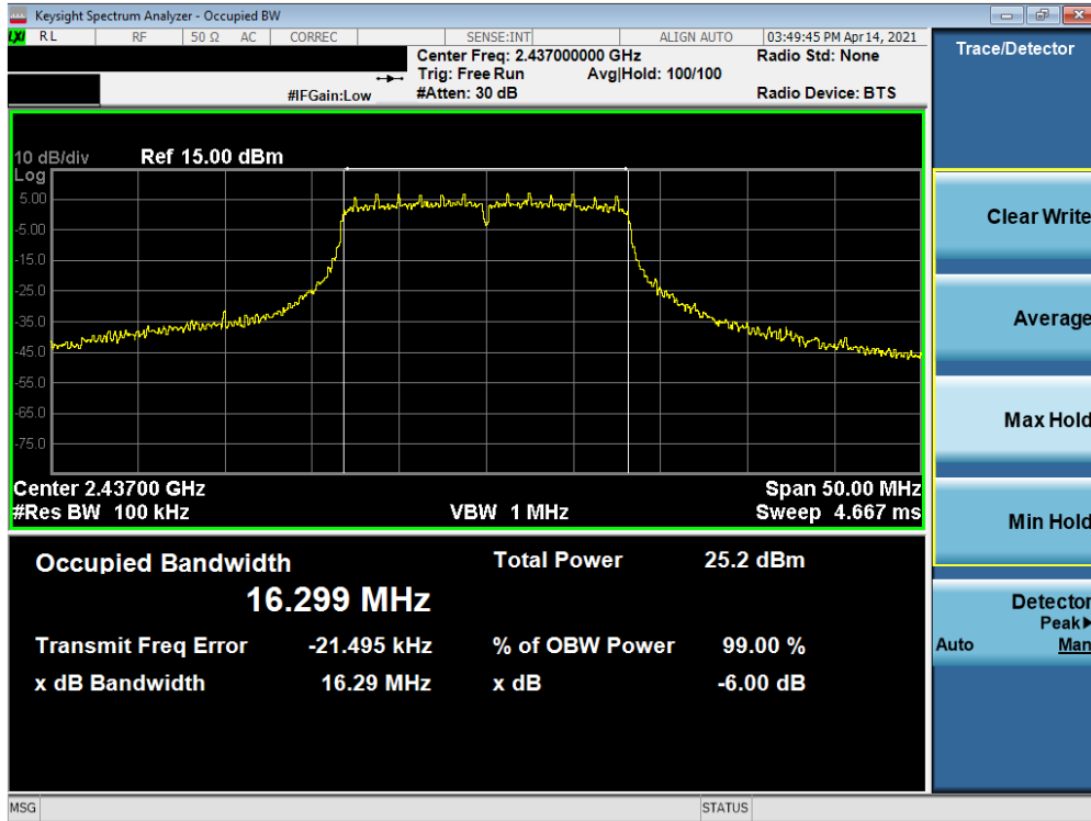
Plot 7-17. 6dB Bandwidth Plot SISO ANT2 (802.11g – Ch. 6) – N
