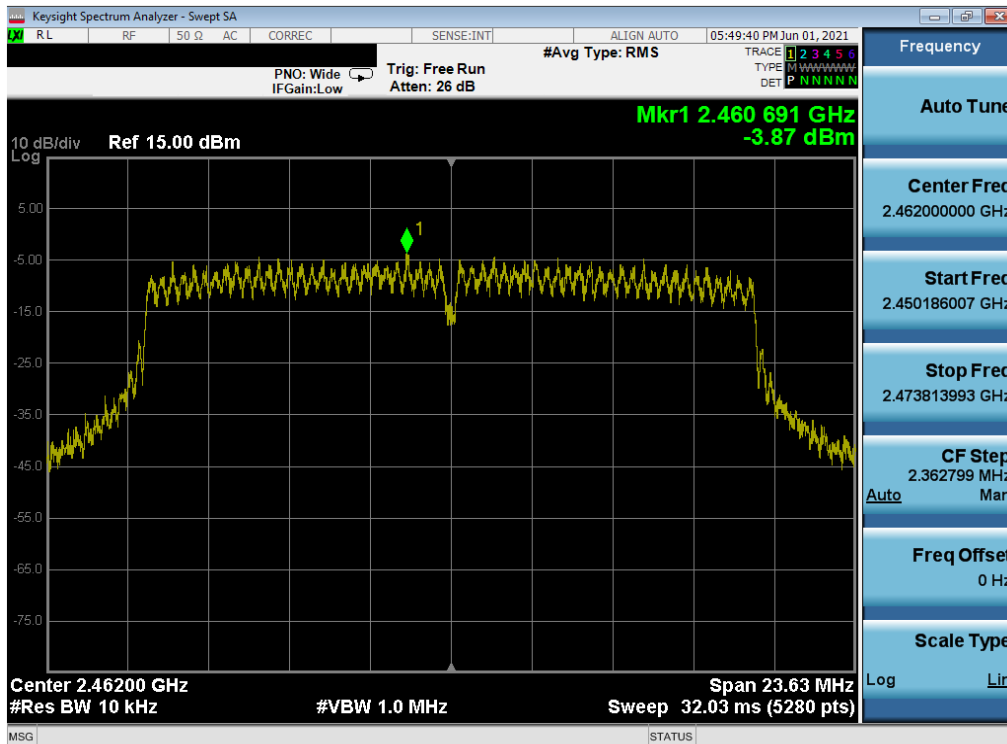
Plot 7-81. Power Spectral Density Plot MIMO ANT1 (802.11n (2.4GHz) – Ch. 11) – N
