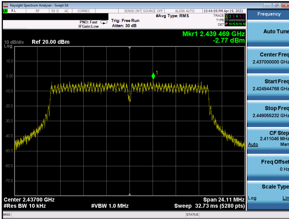
Plot 7-29. Power Spectral Density Plot SISO ANT2 (802.11g – Ch. 6) – Q
