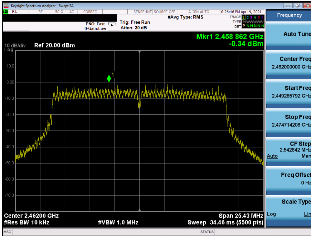
Plot 7-33. Power Spectral Density Plot SISO ANT2 (802.11n (2.4GHz) – Ch. 11) – Q
