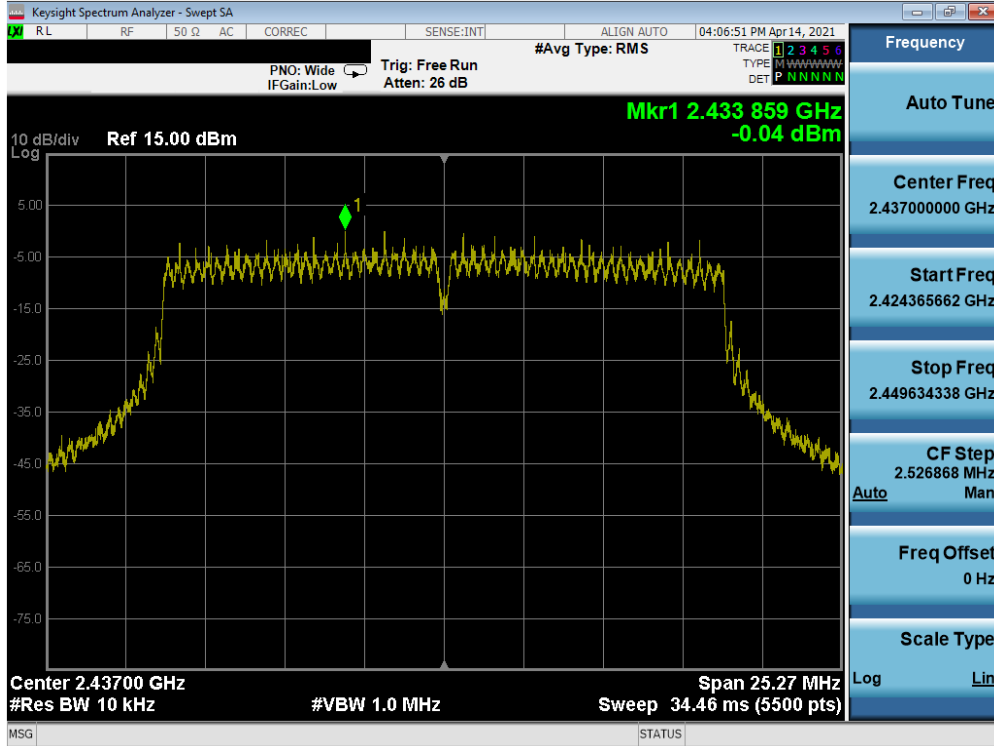
Plot 7-44. Power Spectral Density Plot SISO ANT2 (802.11n (2.4GHz) – Ch. 6) – N
