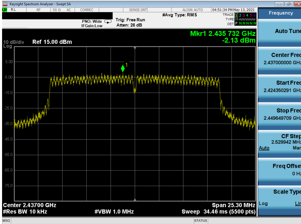
Plot 7-56. Power Spectral Density Plot MIMO ANT1 (802.11n – Ch. 6) – Q
