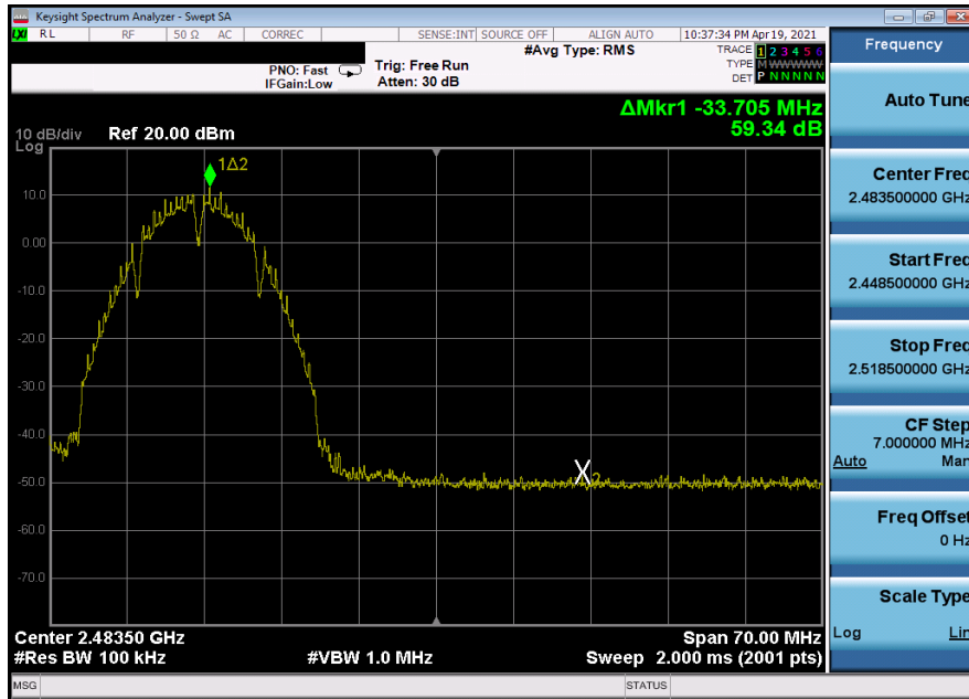
Plot 7-98. Band Edge Plot SISO ANT2 (802.11b – Ch. 11) – Q
