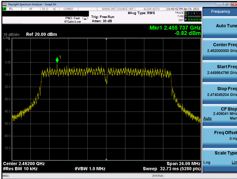
Plot 7-30. Power Spectral Density Plot SISO ANT2 (802.11g – Ch. 11) – Q
