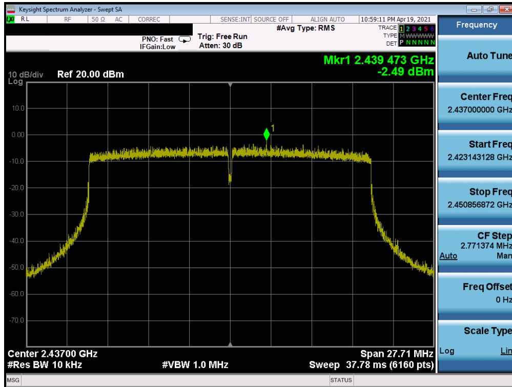
Plot 7-35. Power Spectral Density Plot SISO ANT2 (802.11ax (2.4GHz) – Ch. 6) – Q
