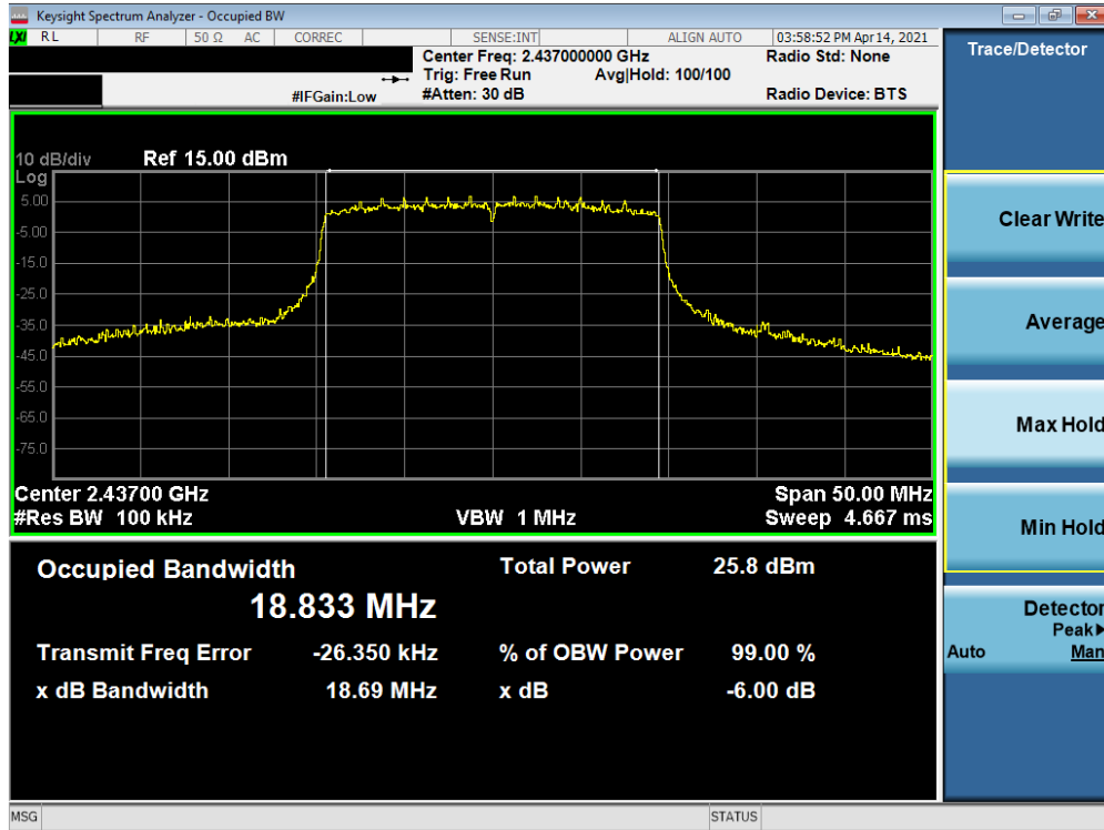
Plot 7-23. 6dB Bandwidth Plot SISO ANT2 (802.11ax (2.4GHz) – Ch. 6) – N
