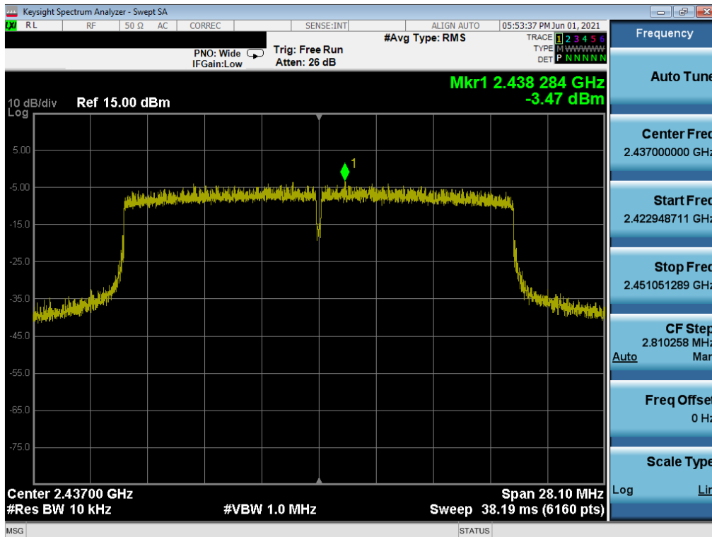
Plot 7-83. Power Spectral Density Plot MIMO ANT1 (802.11ax (2.4GHz) – Ch. 6) – N
