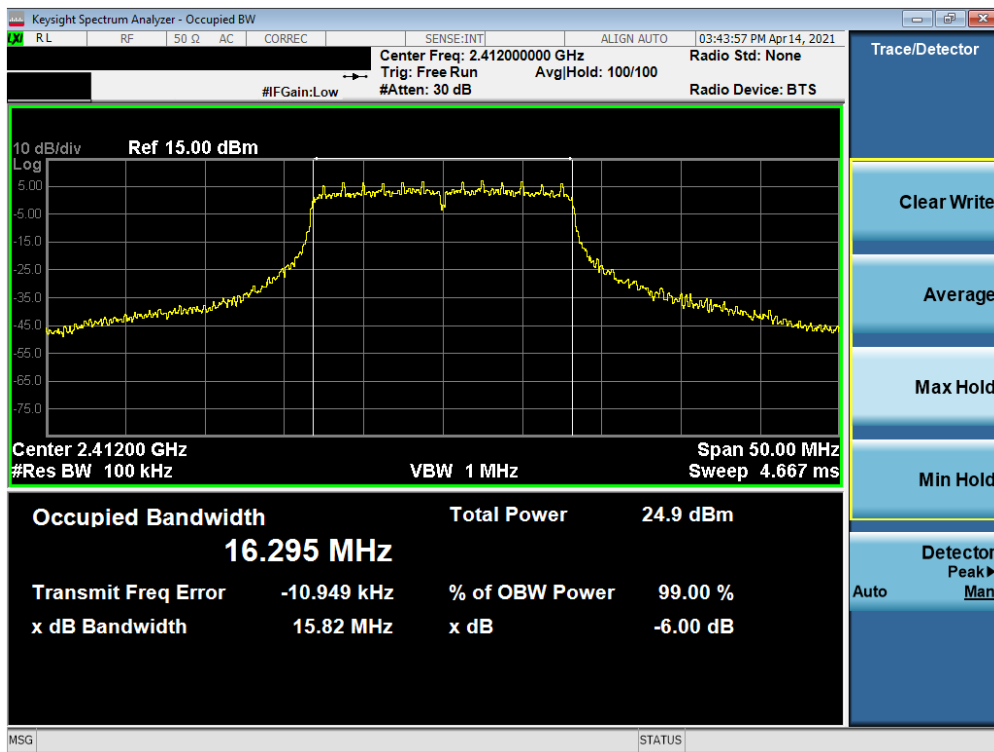
Plot 7-16. 6dB Bandwidth Plot SISO ANT2 (802.11g – Ch. 1) – N
