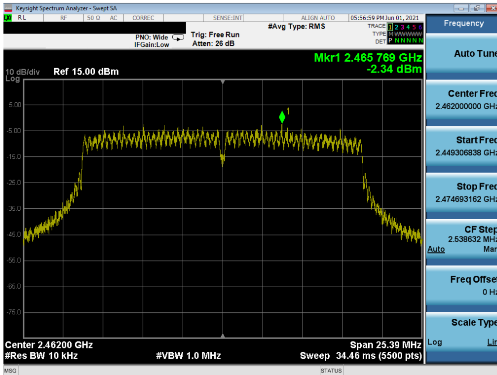
Plot 7-93. Power Spectral Density Plot MIMO ANT2 (802.11n (2.4GHz) – Ch. 11) – N
