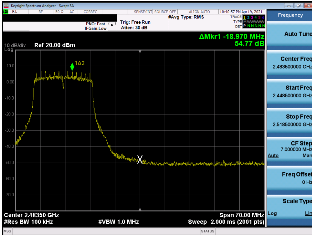
Plot 7-102. Band Edge Plot SISO ANT2 (802.11g - Ch. 11) – Q
