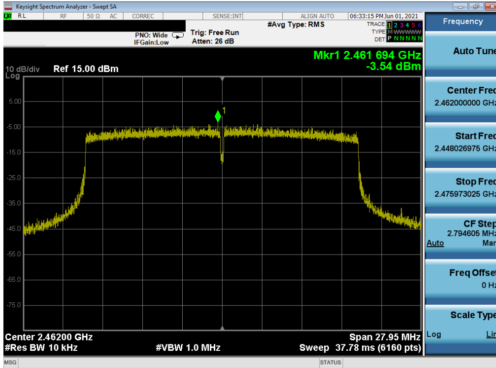
Plot 7-60. Power Spectral Density Plot MIMO ANT1 (802.11ax – Ch. 11) – Q
