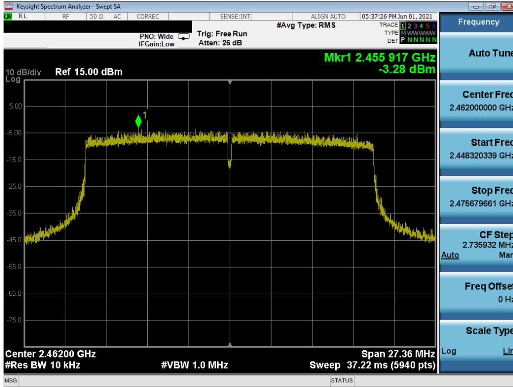
Plot 7-96. Power Spectral Density Plot MIMO ANT2 (802.11ax (2.4GHz) – Ch. 11) – N
