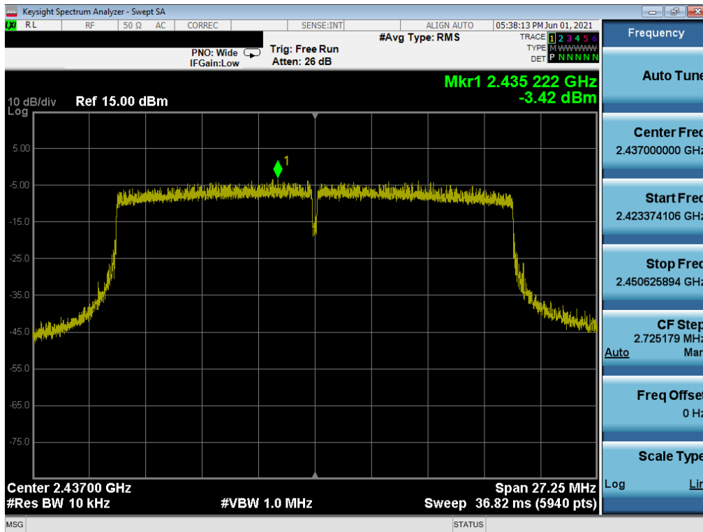
Plot 7-95. Power Spectral Density Plot MIMO ANT2 (802.11ax (2.4GHz) – Ch. 6) – N
