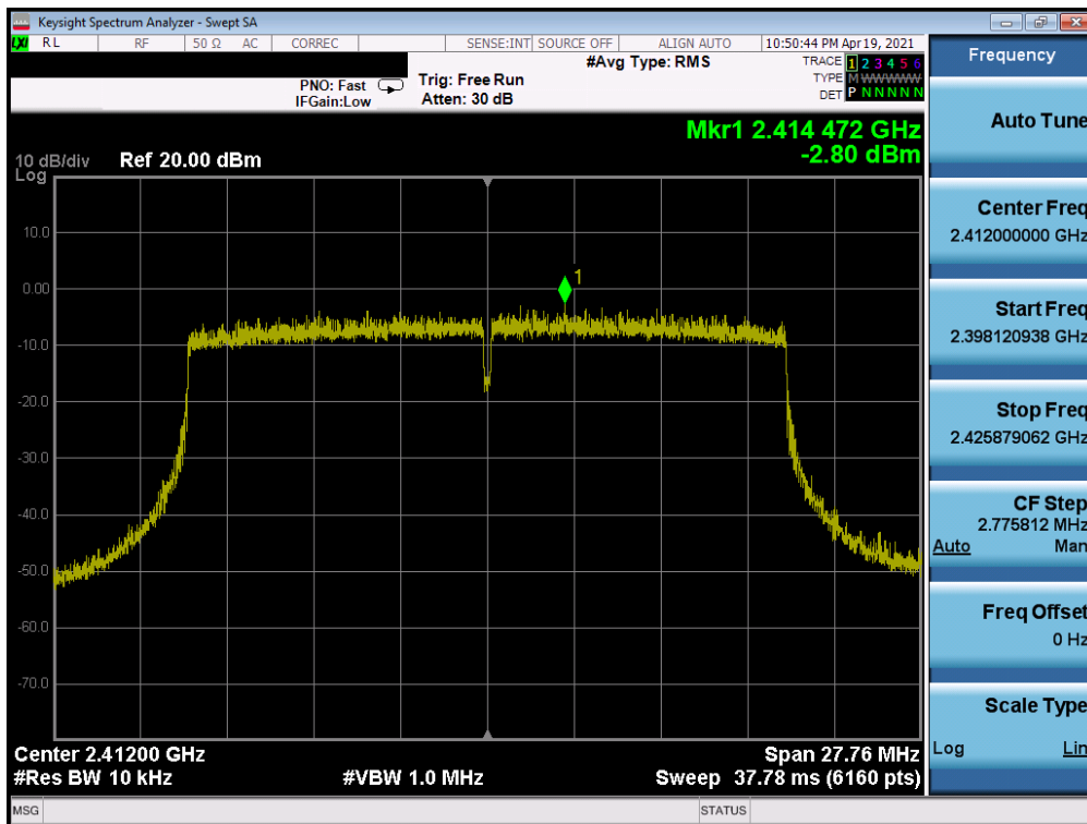
Plot 7-34. Power Spectral Density Plot SISO ANT2 (802.11ax (2.4GHz) – Ch. 1) – Q
