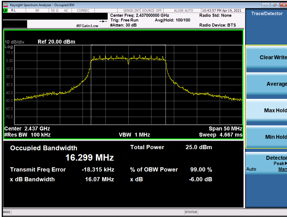
Plot 7-5. 6dB Bandwidth Plot SISO ANT2 (802.11g - Ch. 6) - Q
