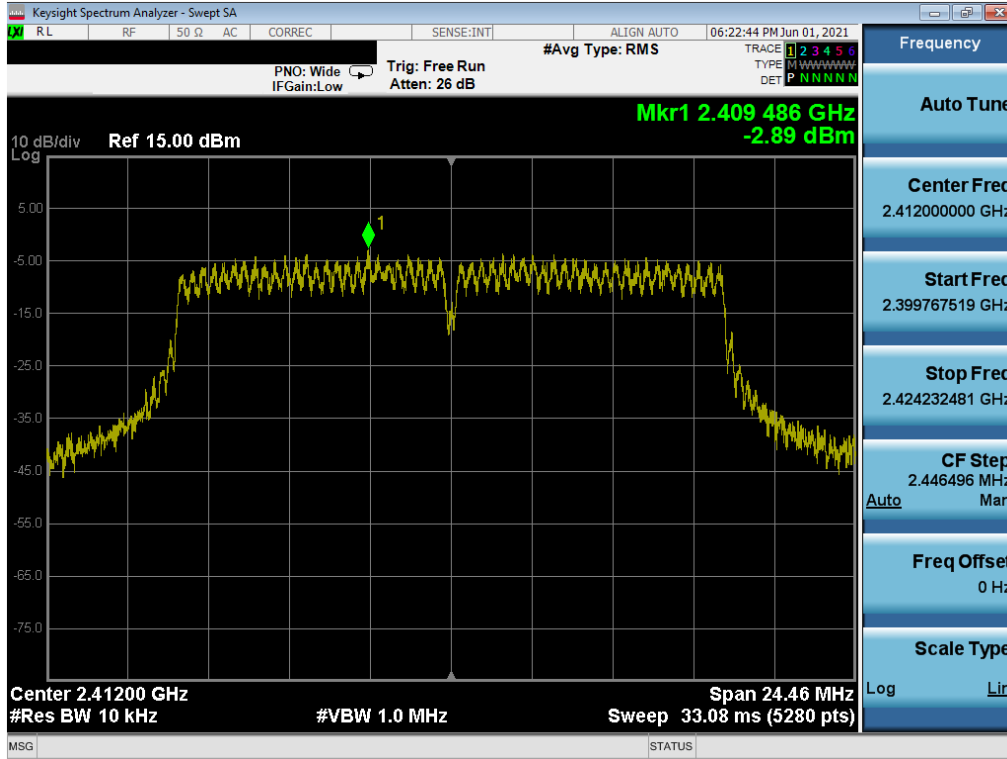
Plot 7-64. Power Spectral Density Plot MIMO ANT2 (802.11g – Ch. 1) – Q
