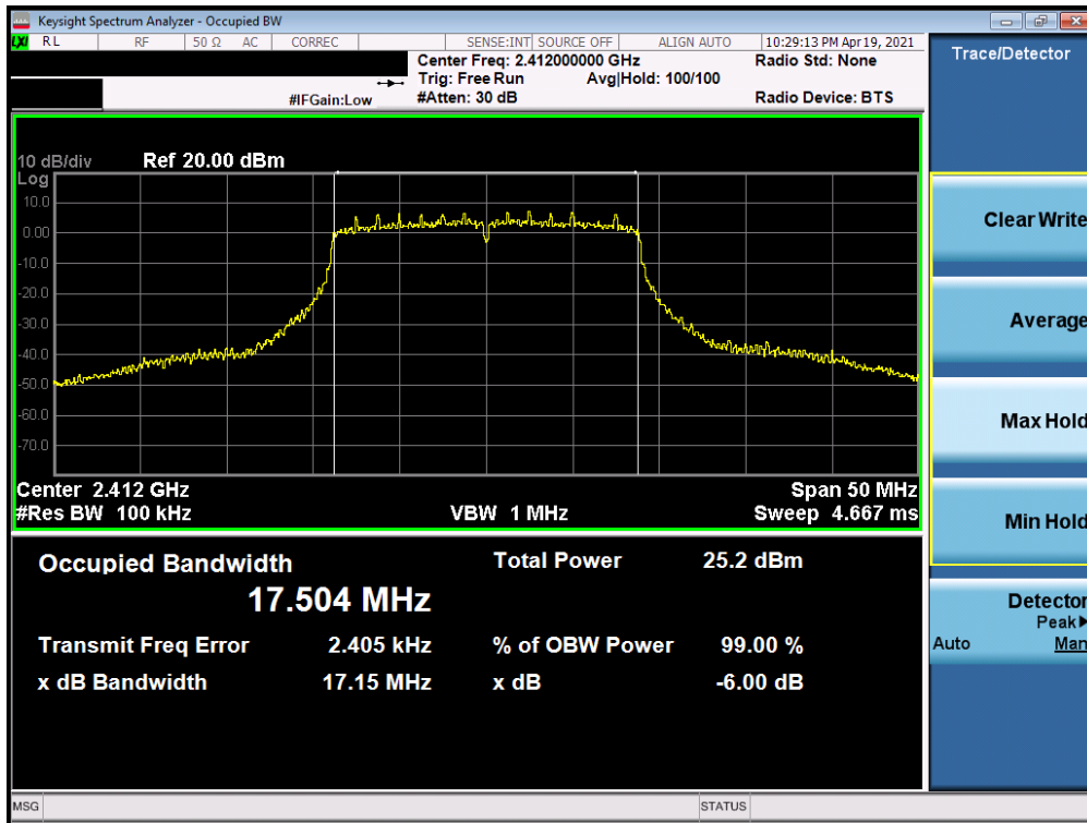
Plot 7-7. 6dB Bandwidth Plot SISO ANT2 (802.11n (2.4GHz) - Ch. 1) - Q
