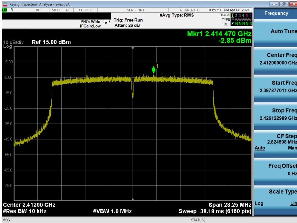
Plot 7-46. Power Spectral Density Plot SISO ANT2 (802.11ax (2.4GHz) – Ch. 1) – N
