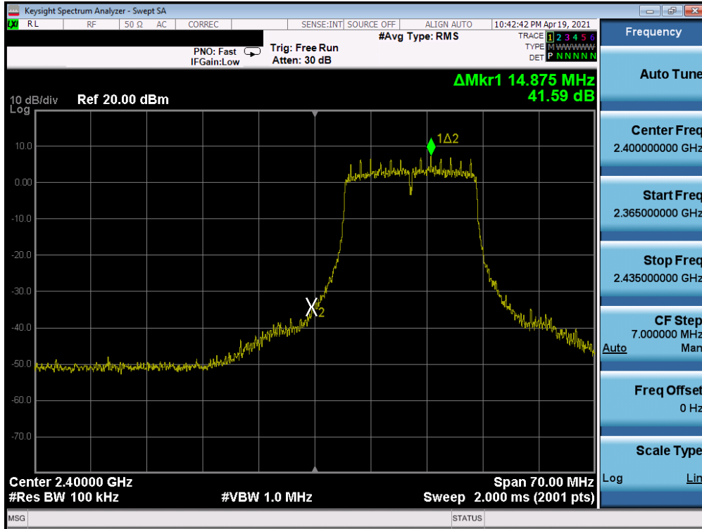
Plot 7-101. Band Edge Plot SISO ANT2 (802.11g- Ch. 1) – Q
