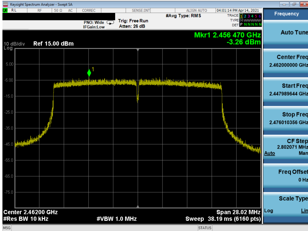
Plot 7-48. Power Spectral Density Plot SISO ANT2 (802.11ax (2.4GHz) – Ch. 11) – N
