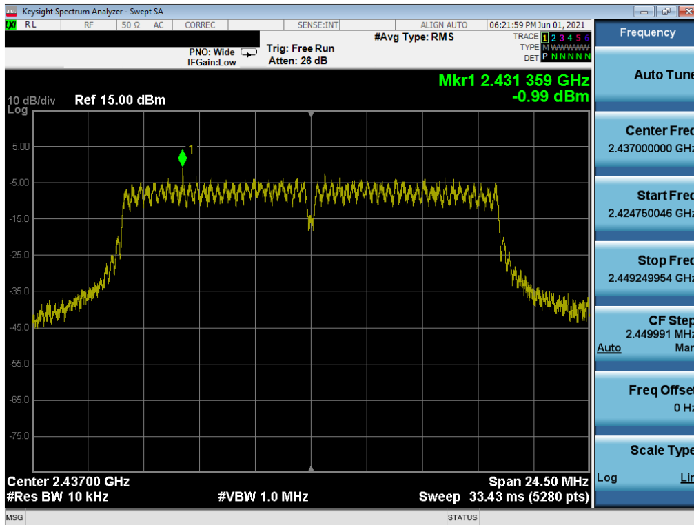
Plot 7-65. Power Spectral Density Plot MIMO ANT2 (802.11g – Ch. 6) – Q
