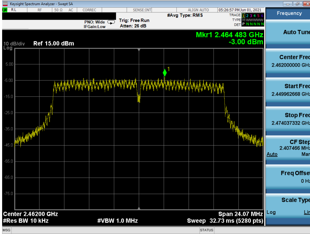
Plot 7-90. Power Spectral Density Plot MIMO ANT2 (802.11g (2.4GHz) – Ch. 11) – N
