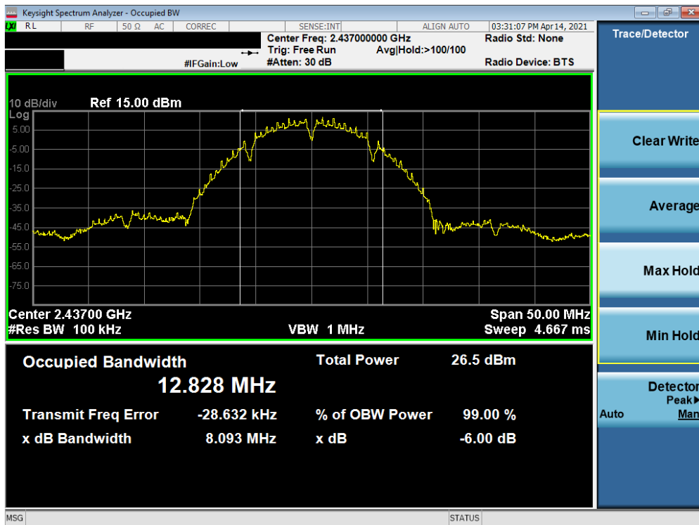
Plot 7-14. 6dB Bandwidth Plot SISO ANT2 (802.11b - Ch. 6) - N
