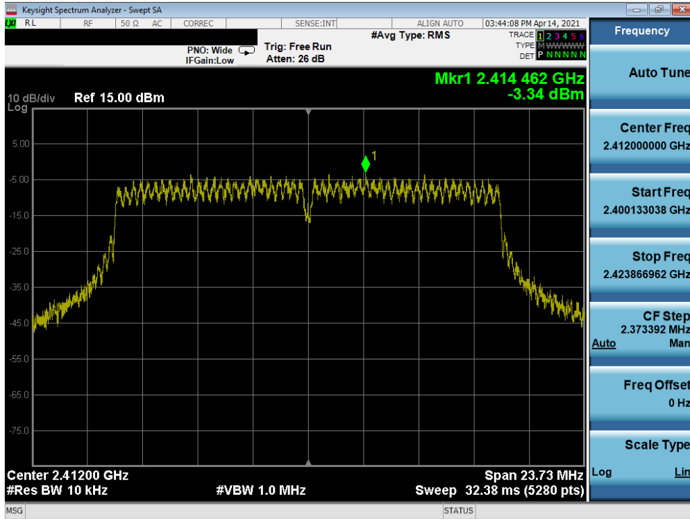
Plot 7-40. Power Spectral Density Plot SISO ANT2 (802.11g – Ch. 1) – N
