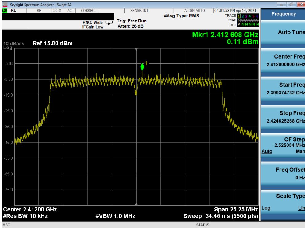
Plot 7-43. Power Spectral Density Plot SISO ANT2 (802.11n (2.4GHz) – Ch. 1) – N
