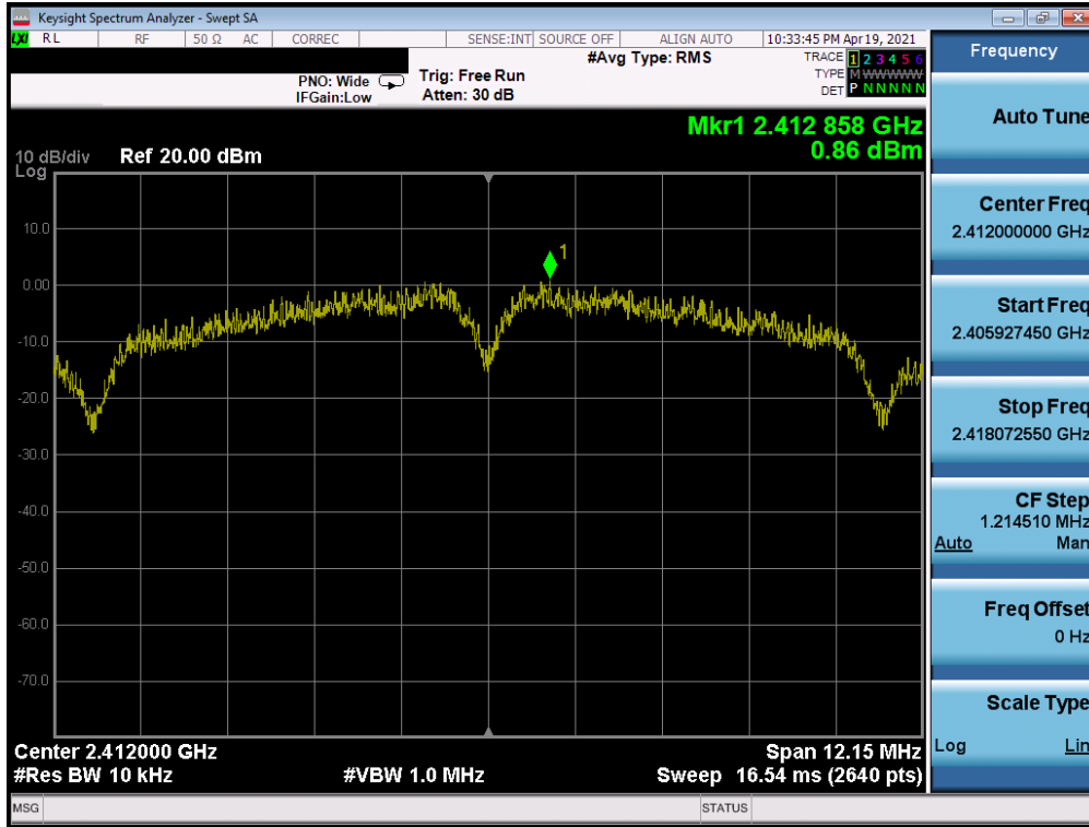
Plot 7-25. Power Spectral Density Plot SISO ANT2 (802.11b – Ch. 1) – Q
