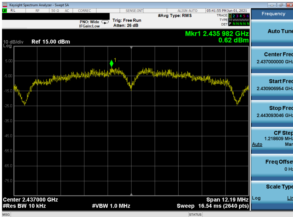
Plot 7-74. Power Spectral Density Plot MIMO ANT1 (802.11b (2.4GHz) – Ch. 6) – N
