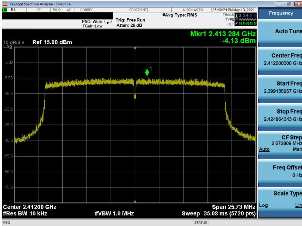
Plot 7-70. Power Spectral Density Plot MIMO ANT2 (802.11ax – Ch. 1) – Q
