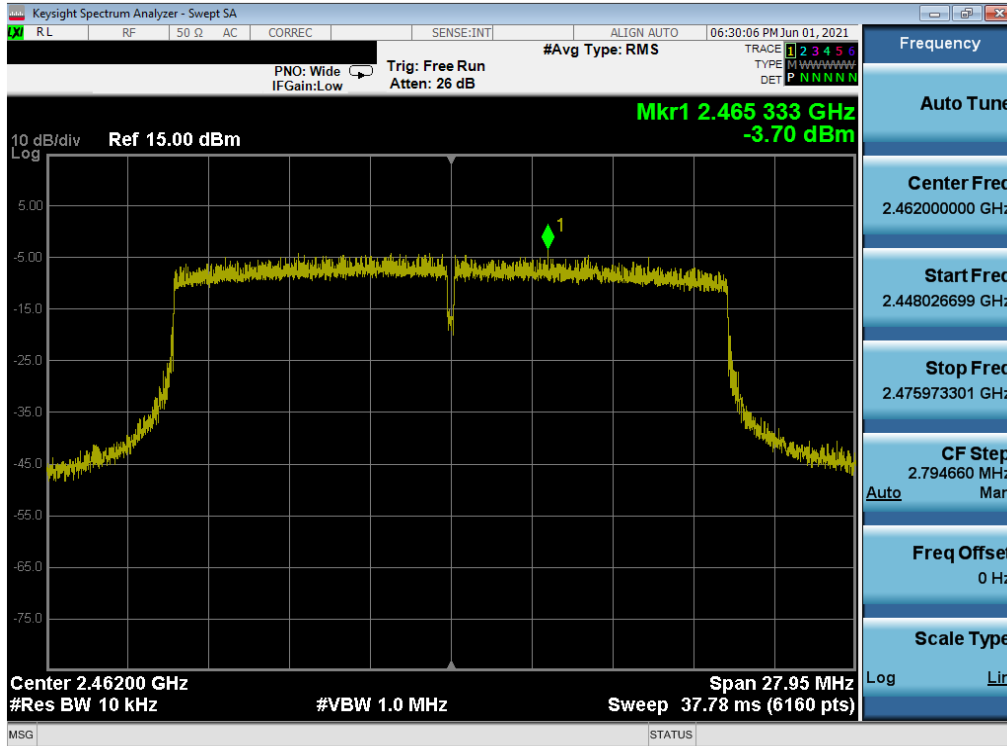
Plot 7-72. Power Spectral Density Plot MIMO ANT2 (802.11ax – Ch. 11) – Q
