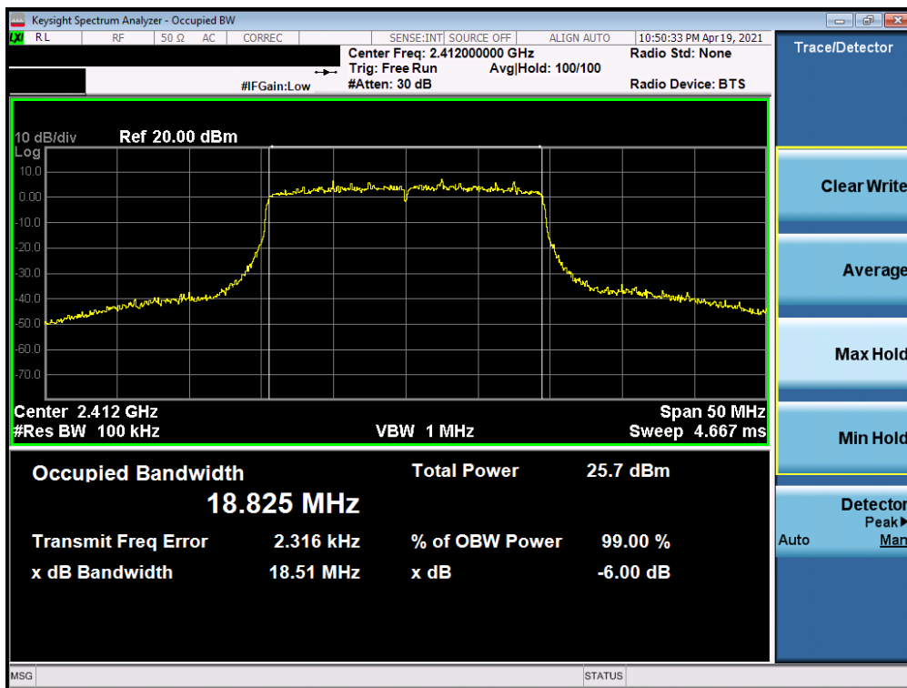
Plot 7-10. 6dB Bandwidth Plot SISO ANT2 (802.11ax (2.4GHz) – Ch. 1) – Q
