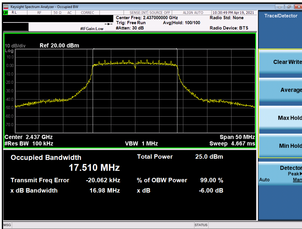
Plot 7-8. 6dB Bandwidth Plot SISO ANT2 (802.11n (2.4GHz) - Ch. 6) - Q
