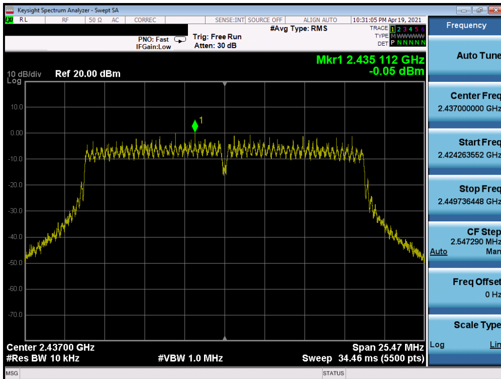
Plot 7-32. Power Spectral Density Plot SISO ANT2 (802.11n (2.4GHz) – Ch. 6) – Q
