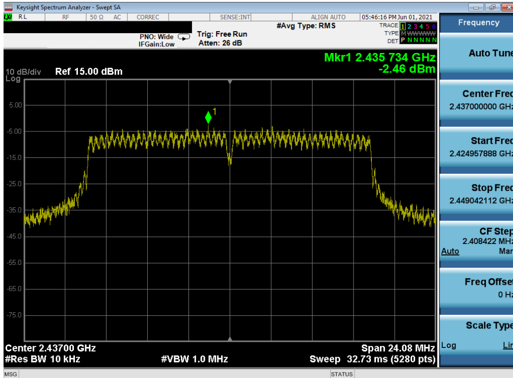
Plot 7-77. Power Spectral Density Plot MIMO ANT1 (802.11g (2.4GHz) – Ch. 6) – N
