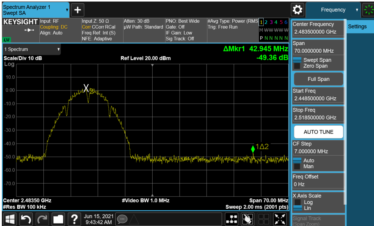
Plot 7-99. Band Edge Plot SISO ANT2 (802.11b – Ch. 12) -- Q
