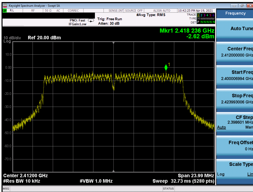
Plot 7-28. Power Spectral Density Plot SISO ANT2 (802.11g – Ch. 1) – Q
