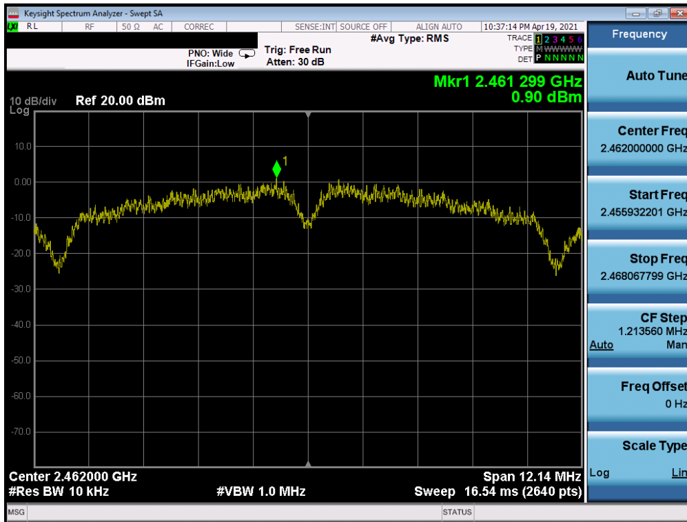
Plot 7-27. Power Spectral Density Plot SISO ANT2 (802.11b – Ch. 11) – Q
