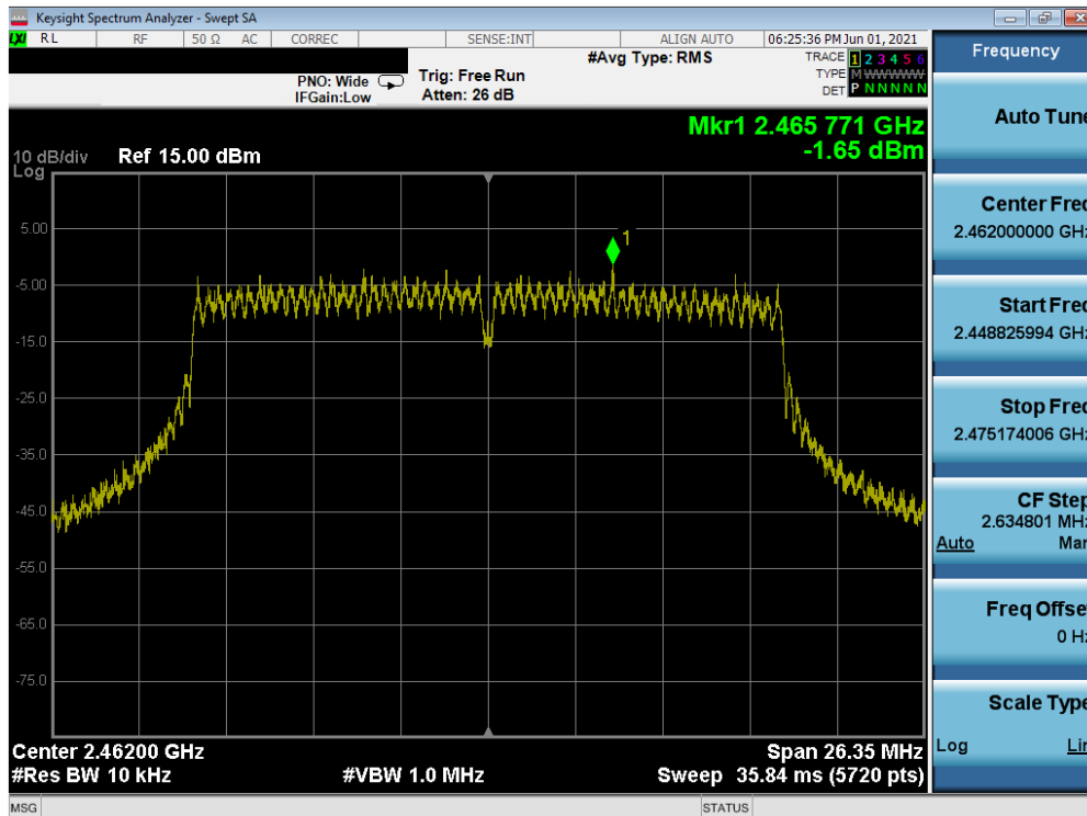
Plot 7-69. Power Spectral Density Plot MIMO ANT2 (802.11n – Ch. 11) – Q
