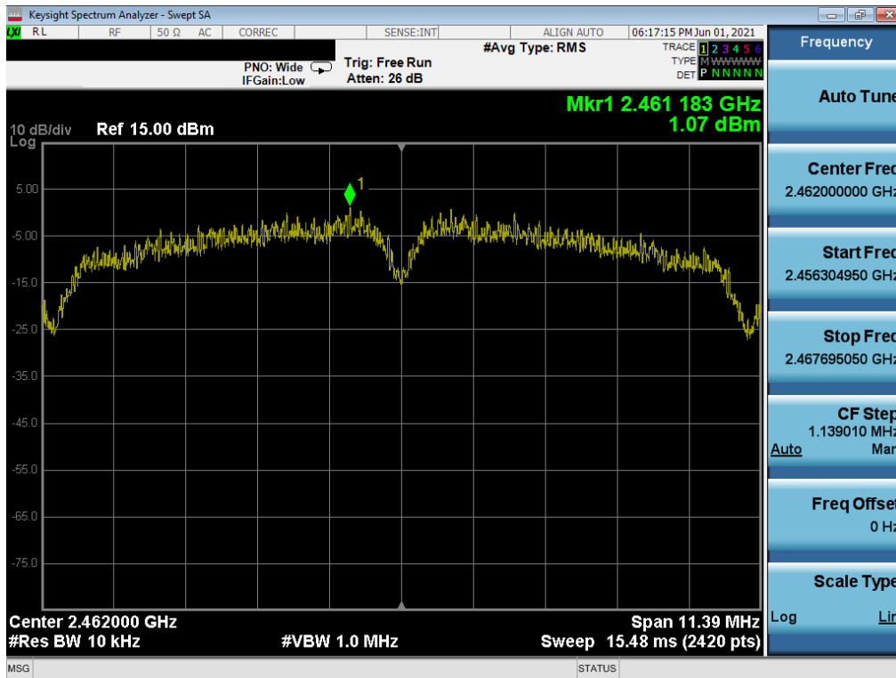
Plot 7-63. Power Spectral Density Plot MIMO ANT2 (802.11b – Ch. 11) – Q
