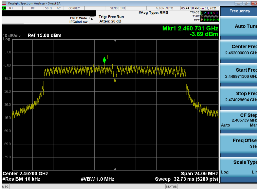
Plot 7-78. Power Spectral Density Plot MIMO ANT1 (802.11g (2.4GHz) – Ch. 11 – N
