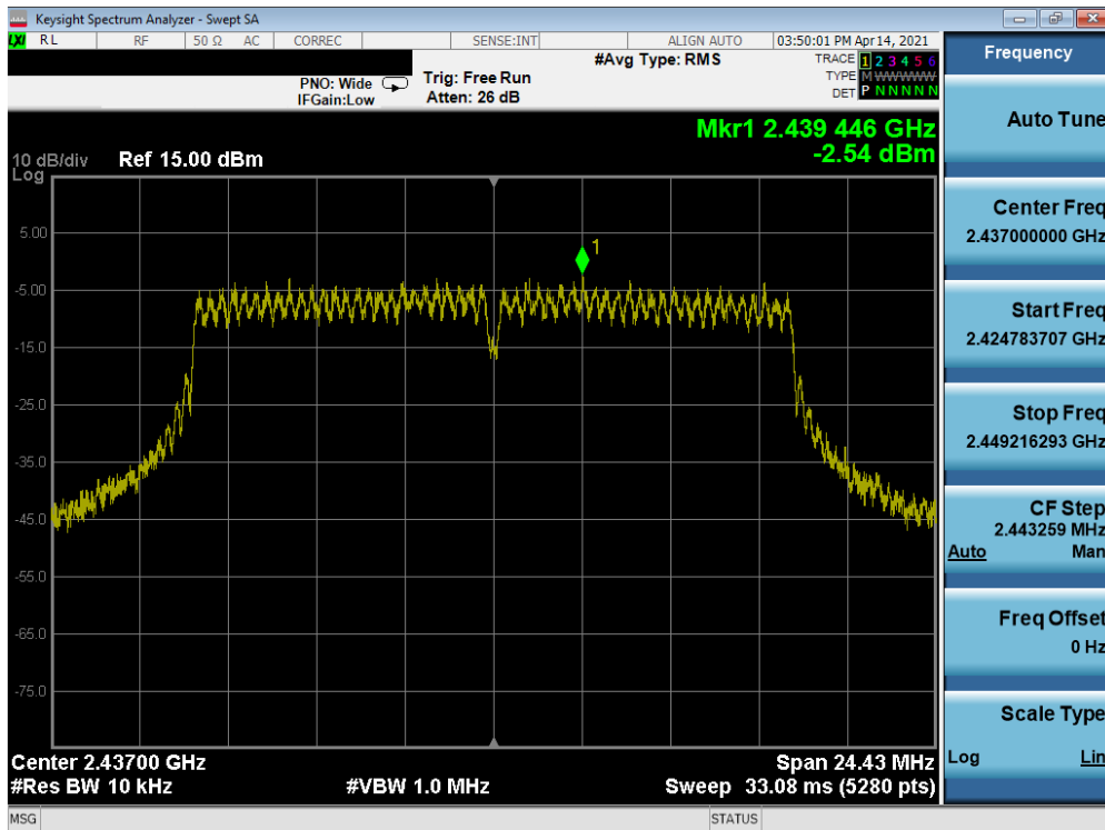
Plot 7-41. Power Spectral Density Plot SISO ANT2 (802.11g – Ch. 6) – N
