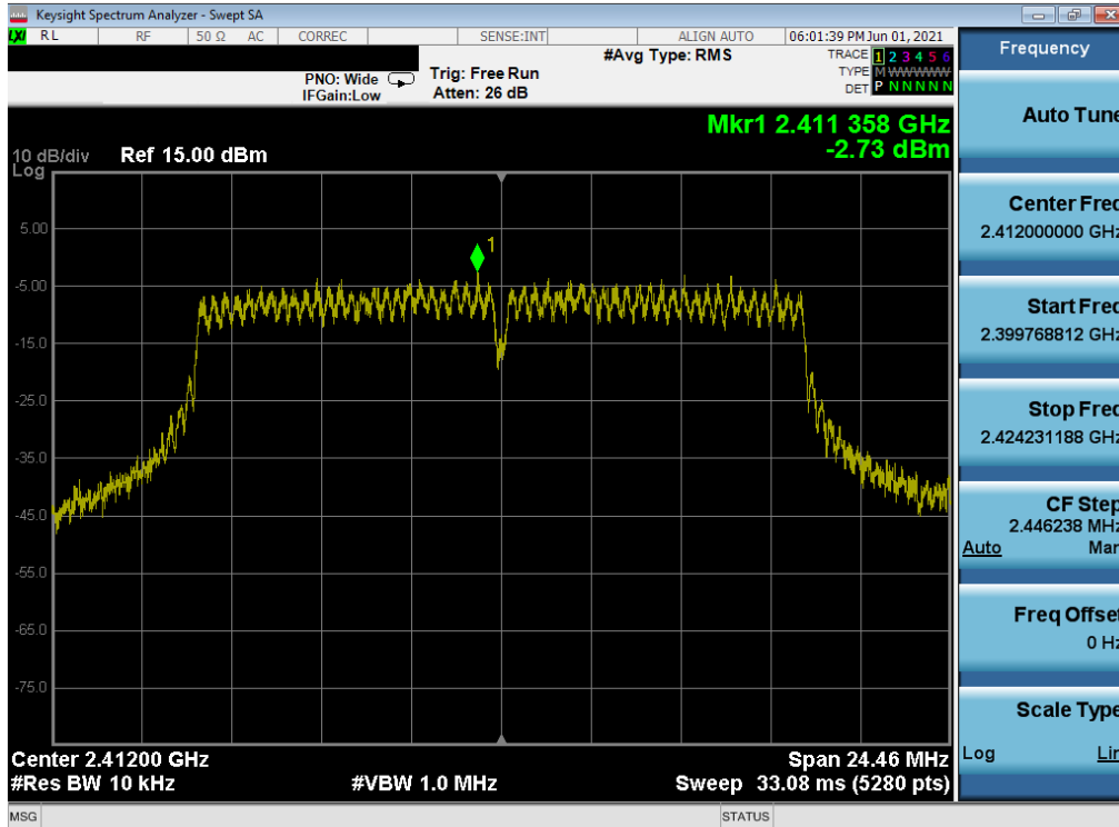
Plot 7-88. Power Spectral Density Plot MIMO ANT2 (802.11g (2.4GHz) – Ch. 1) – N
