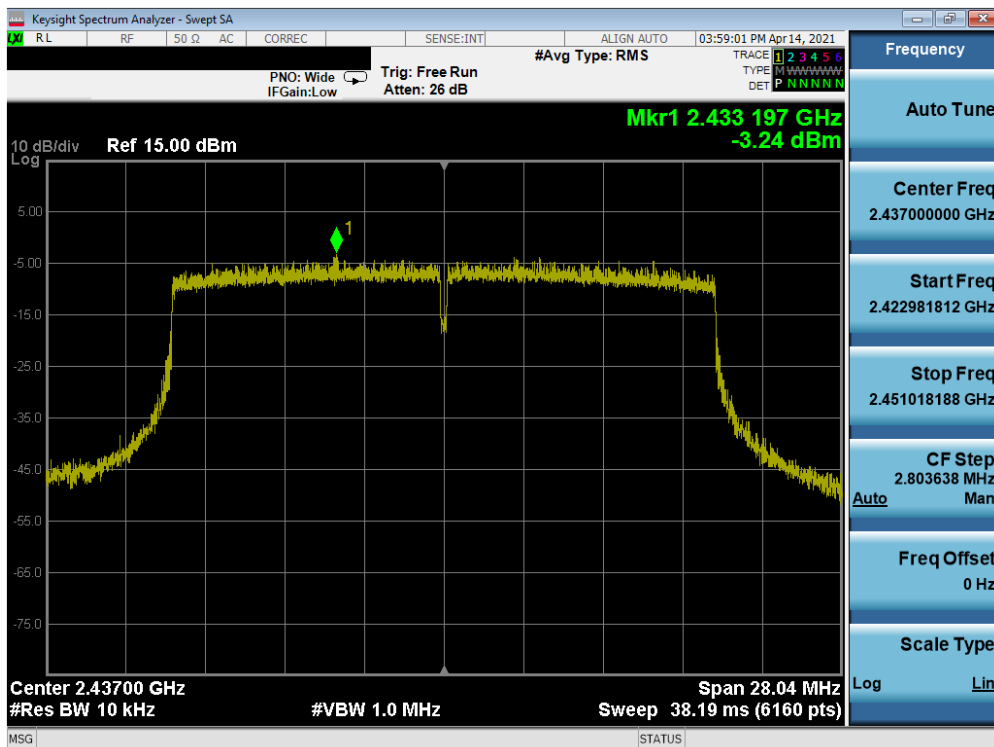
Plot 7-47. Power Spectral Density Plot SISO ANT2 (802.11ax (2.4GHz) – Ch. 6) – N
