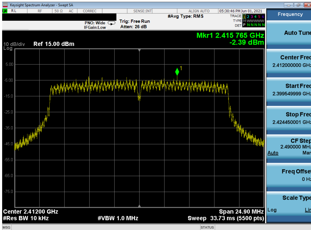
Plot 7-91. Power Spectral Density Plot MIMO ANT2 (802.11n (2.4GHz) – Ch. 1) – N
