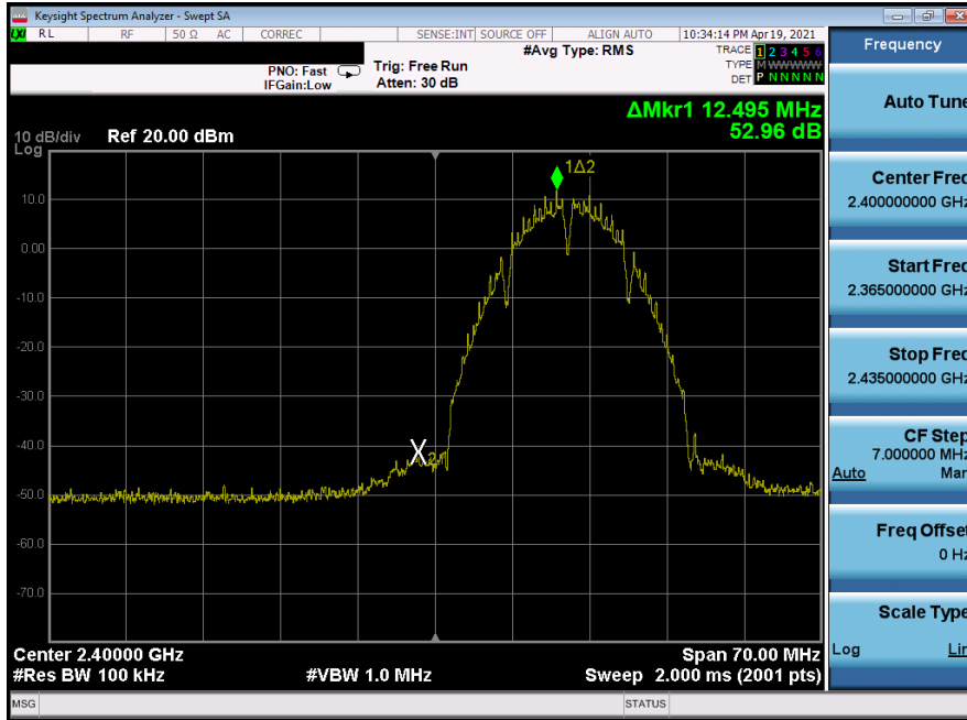
Plot 7-97. Band Edge Plot SISO ANT2 (802.11b – Ch. 1) -- Q
