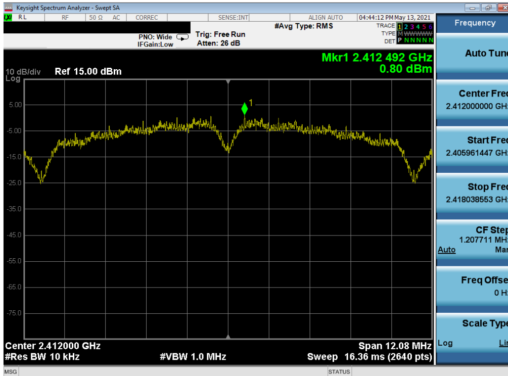
Plot 7-49. Power Spectral Density Plot MIMO ANT1 (802.11b – Ch. 1) – Q
