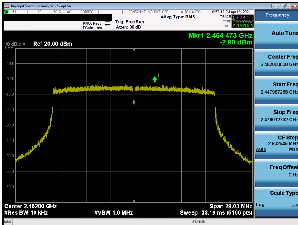
Plot 7-36. Power Spectral Density Plot SISO ANT2 (802.11ax (2.4GHz) – Ch. 11) – Q
