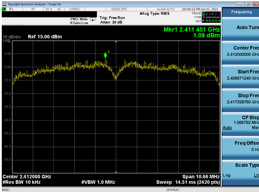
Plot 7-85. Power Spectral Density Plot MIMO ANT2 (802.11b (2.4GHz) – Ch. 1) – N
