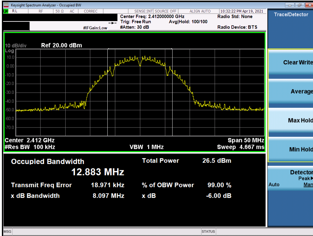
Plot 7-1. 6dB Bandwidth Plot SISO ANT2 (802.11b – Ch. 1) – Q
