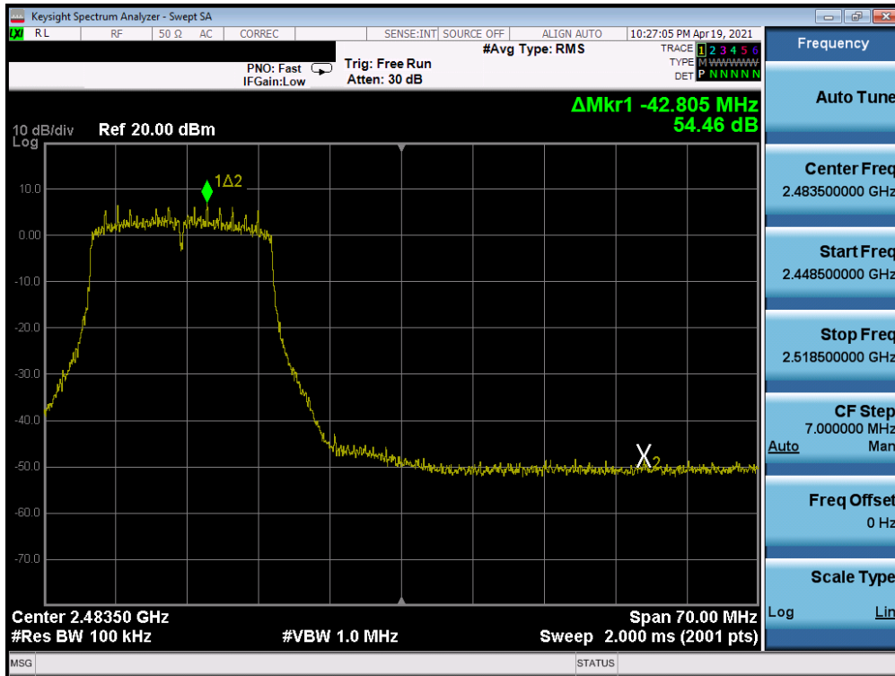
Plot 7-106. Band Edge Plot SISO ANT2 (802.11n (2.4GHz) – Ch. 11) – Q
