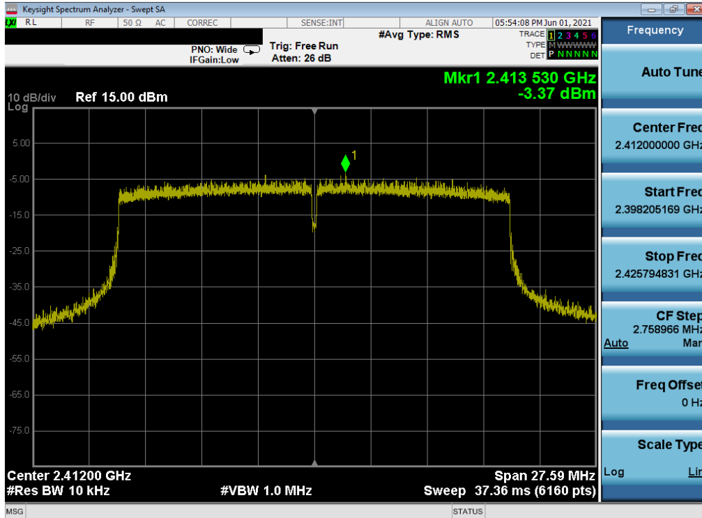
plot 7-82. Power Spectral Density Plot MIMO ANT1 (802.11ax (2.4GHz) – Ch. 1) – N
