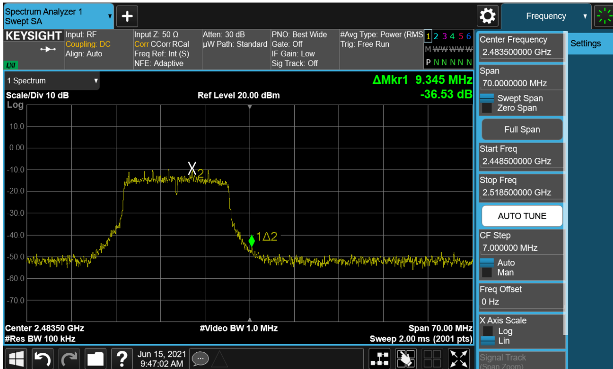
Plot 7-104. Band Edge Plot SISO ANT2 (802.11g – Ch. 13) – Q
