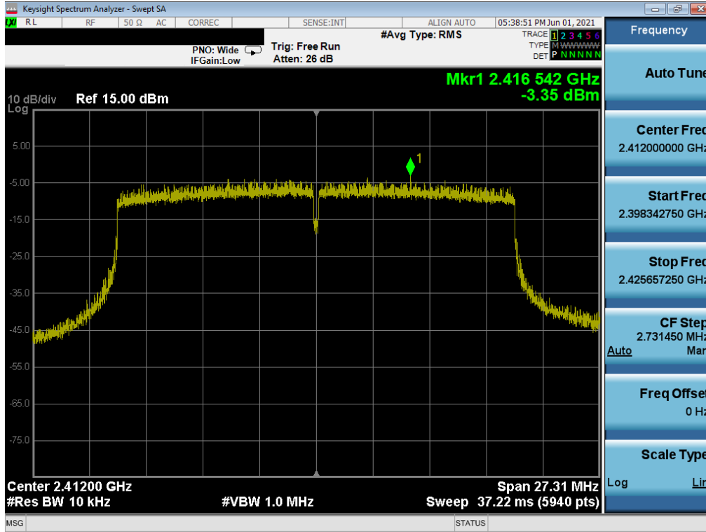
Plot 7-94. Power Spectral Density Plot MIMO ANT2 (802.11ax (2.4GHz) – Ch. 1) – N
