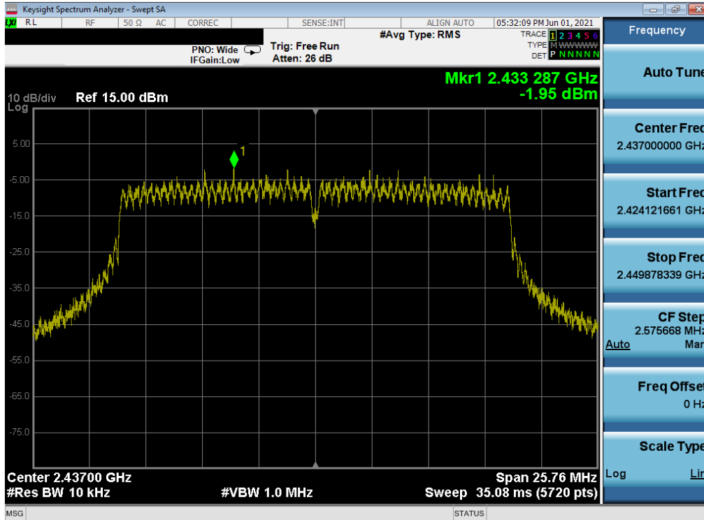
Plot 7-92. Power Spectral Density Plot MIMO ANT2 (802.11n (2.4GHz) – Ch. 6) – N
