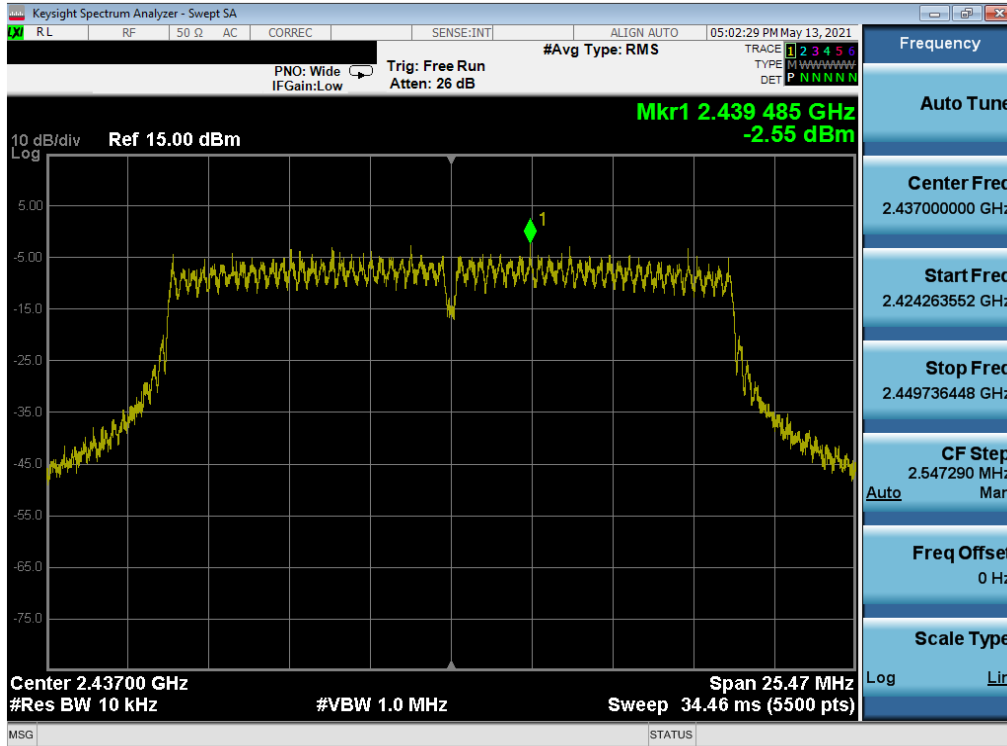
Plot 7-68. Power Spectral Density Plot MIMO ANT2 (802.11n – Ch. 6) – Q
