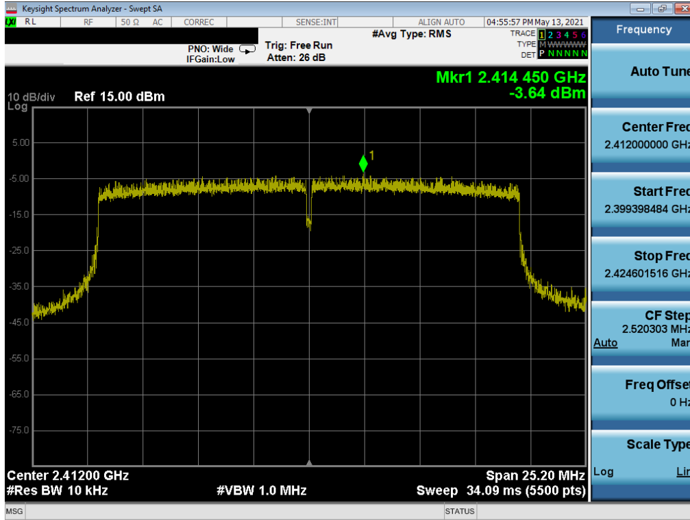
Plot 7-58. Power Spectral Density Plot MIMO ANT1 (802.11ax – Ch. 1) – Q
