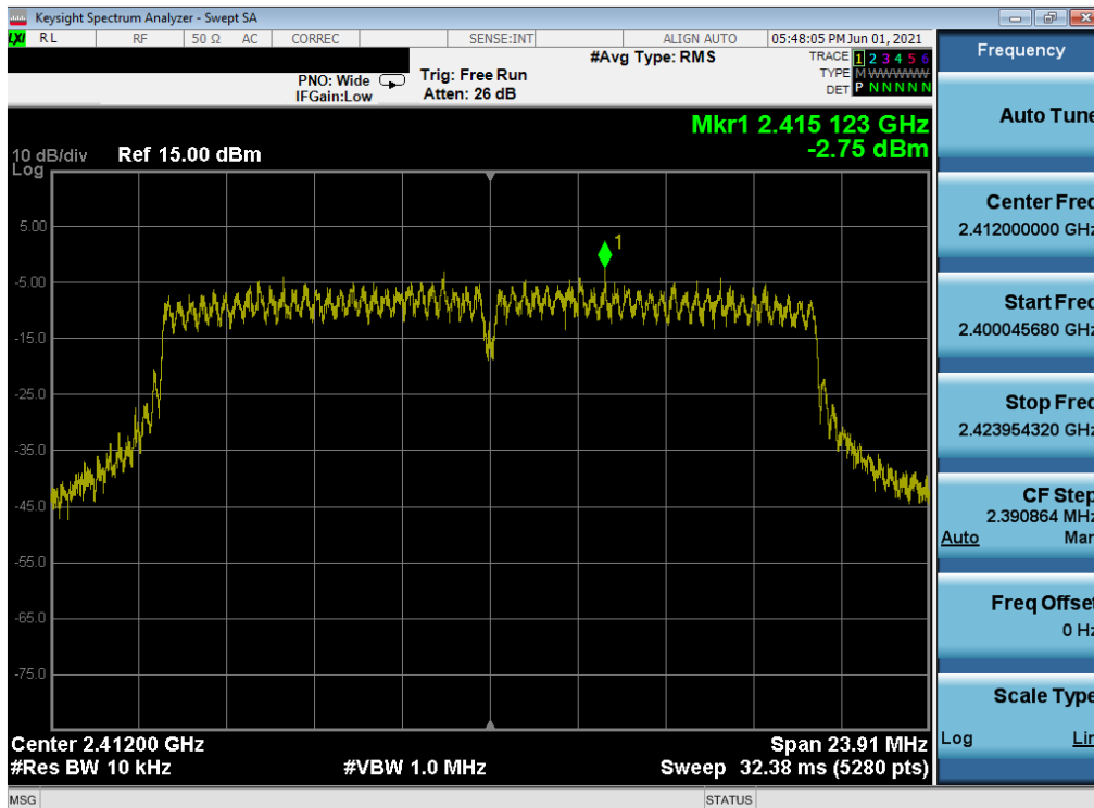
Plot 7-79. Power Spectral Density Plot MIMO ANT1 (802.11n (2.4GHz) – Ch. 1) – N
