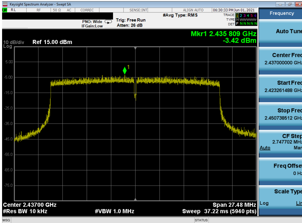
Plot 7-71. Power Spectral Density Plot MIMO ANT2 (802.11ax – Ch. 6) – Q
