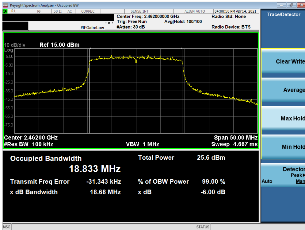
Plot 7-24. 6dB Bandwidth Plot SISO ANT2 (802.11ax (2.4GHz) – Ch. 11) – N
