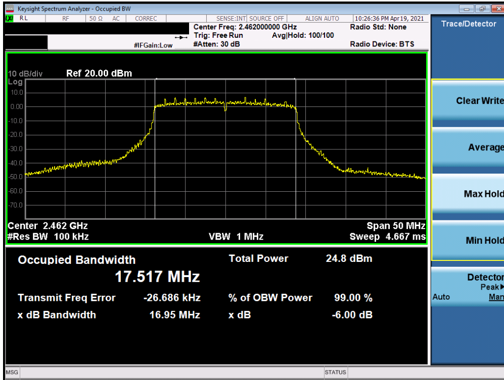
Plot 7-9. 6dB Bandwidth Plot SISO ANT2 (802.11n (2.4GHz) – Ch. 11) – Q
