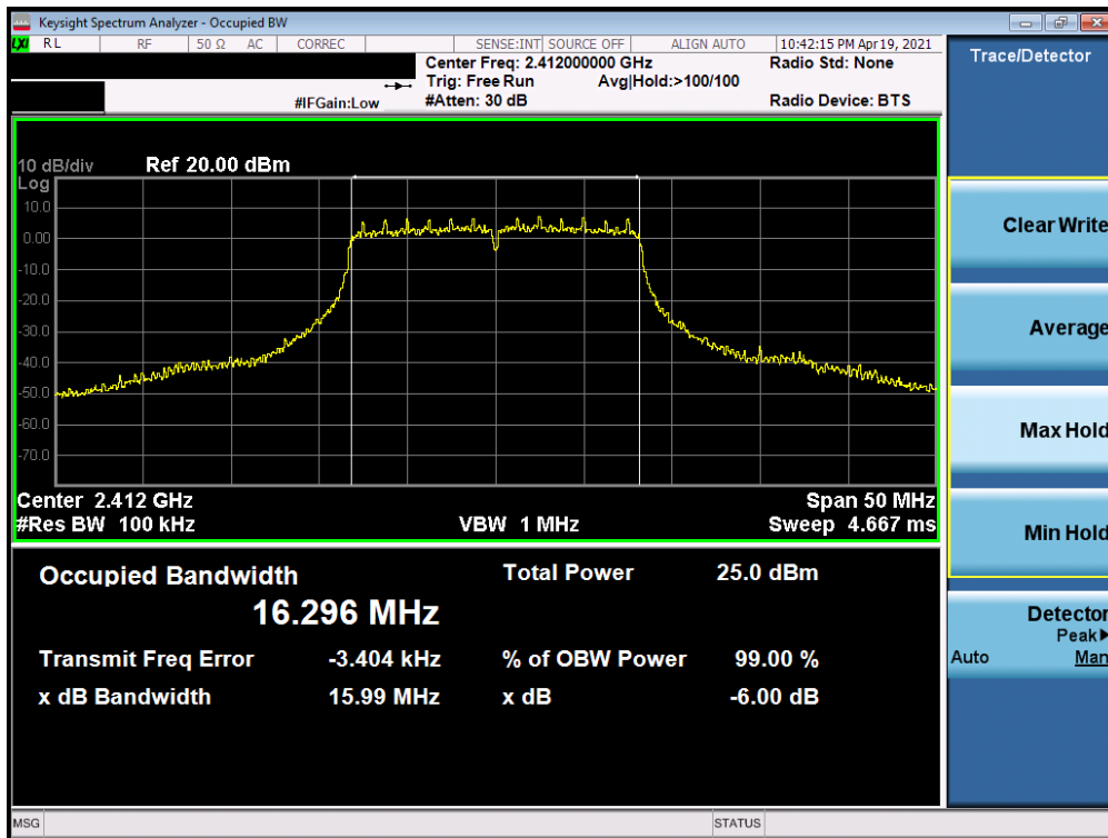
Plot 7-4. 6dB Bandwidth Plot SISO ANT2 (802.11g – Ch. 1) – Q
