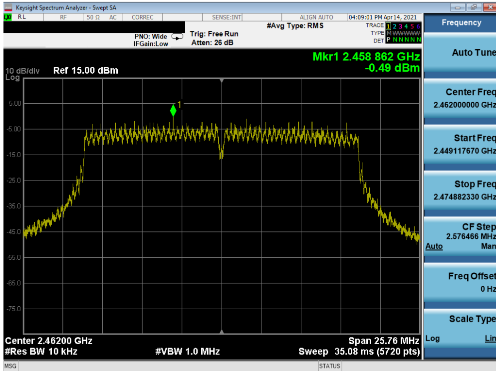
Plot 7-45. Power Spectral Density Plot SISO ANT2 (802.11n (2.4GHz) – Ch. 11) – N
