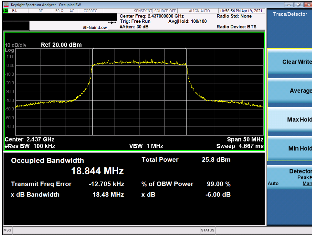
Plot 7-11. 6dB Bandwidth Plot SISO ANT2 (802.11ax (2.4GHz) – Ch. 6) – Q
