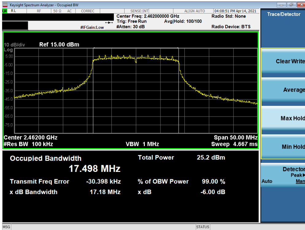
Plot 7-21. 6dB Bandwidth Plot SISO ANT2 (802.11n (2.4GHz) – Ch. 11) – N
