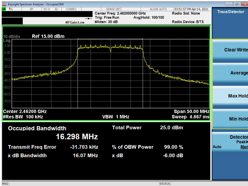
Plot 7-18. 6dB Bandwidth Plot SISO ANT2 (802.11g – Ch. 11) – N
