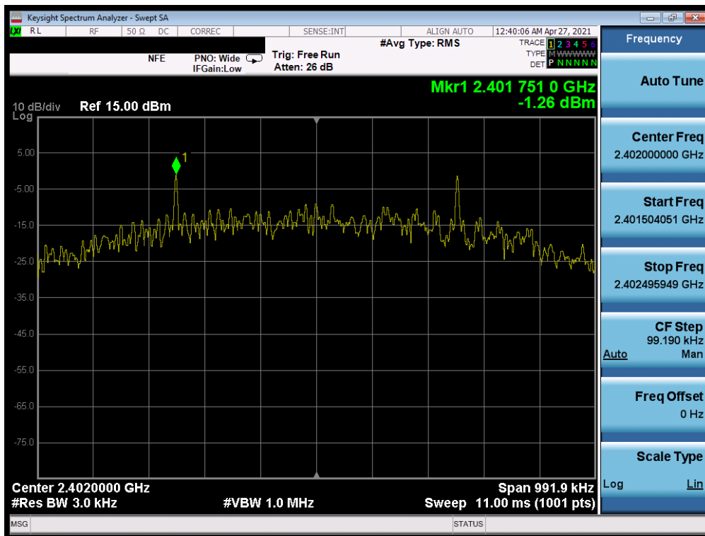
Plot 7-64. Power Spectral Density Plot (Bluetooth (LE), 500kbps – Ch. 0) - Q
