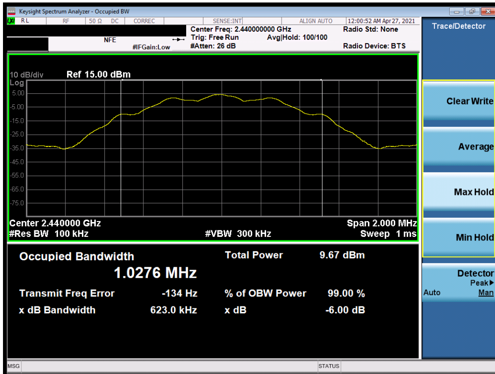
Plot 7-14. 6dB Bandwidth Plot (Bluetooth (LE), 125kbps – Ch. 19) - Q
