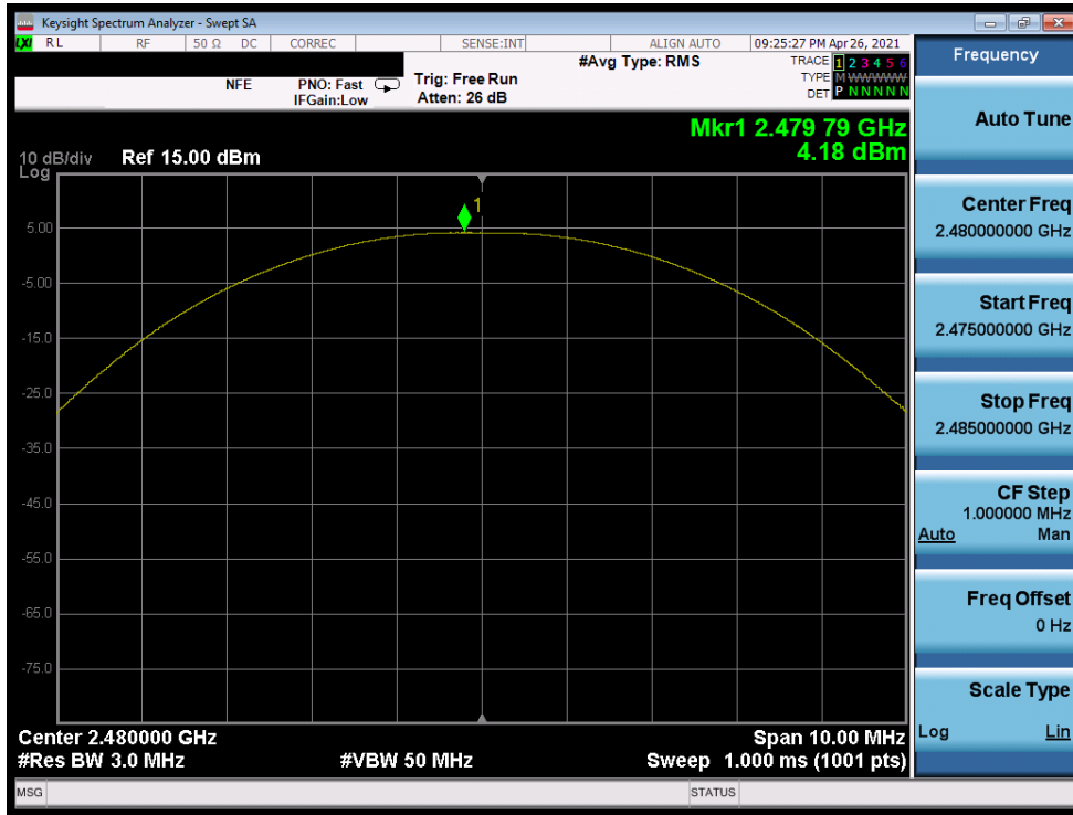
Plot 7-33. Peak Power Plot (Bluetooth (LE), 1Mbps – Ch. 39) - N
