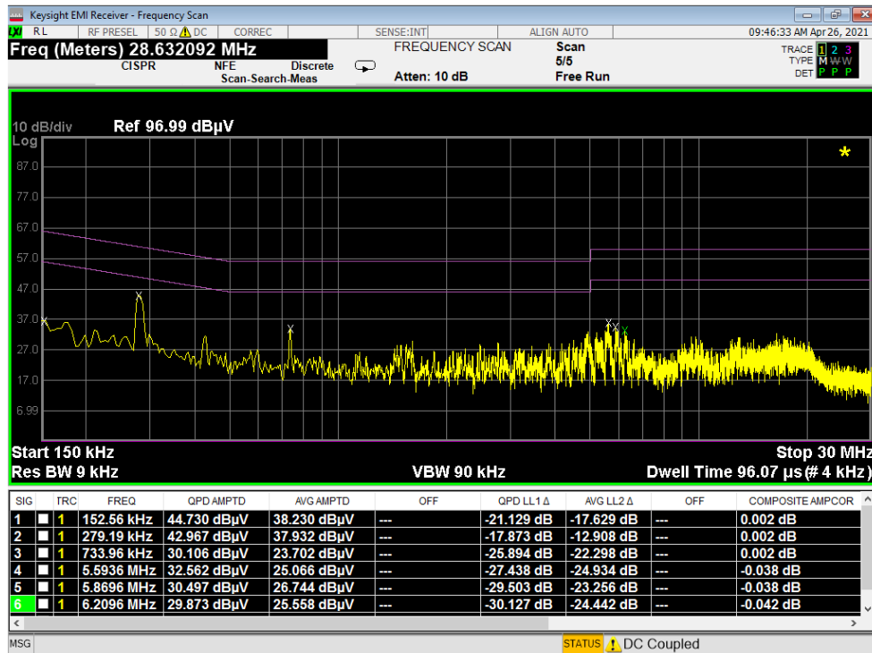
Plot 7-108. Line Conducted Plot with Bluetooth LE (N) - N (CLOSED)
