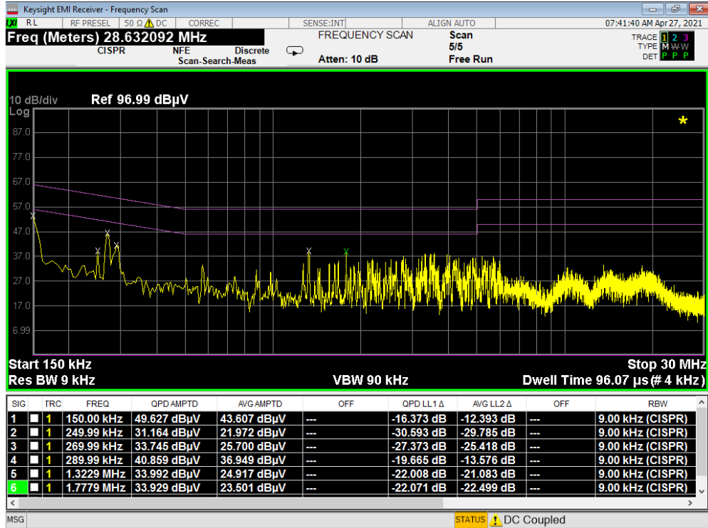
Plot 7-111. Line Conducted Plot with Bluetooth LE (L1) - Q (CLOSED)
