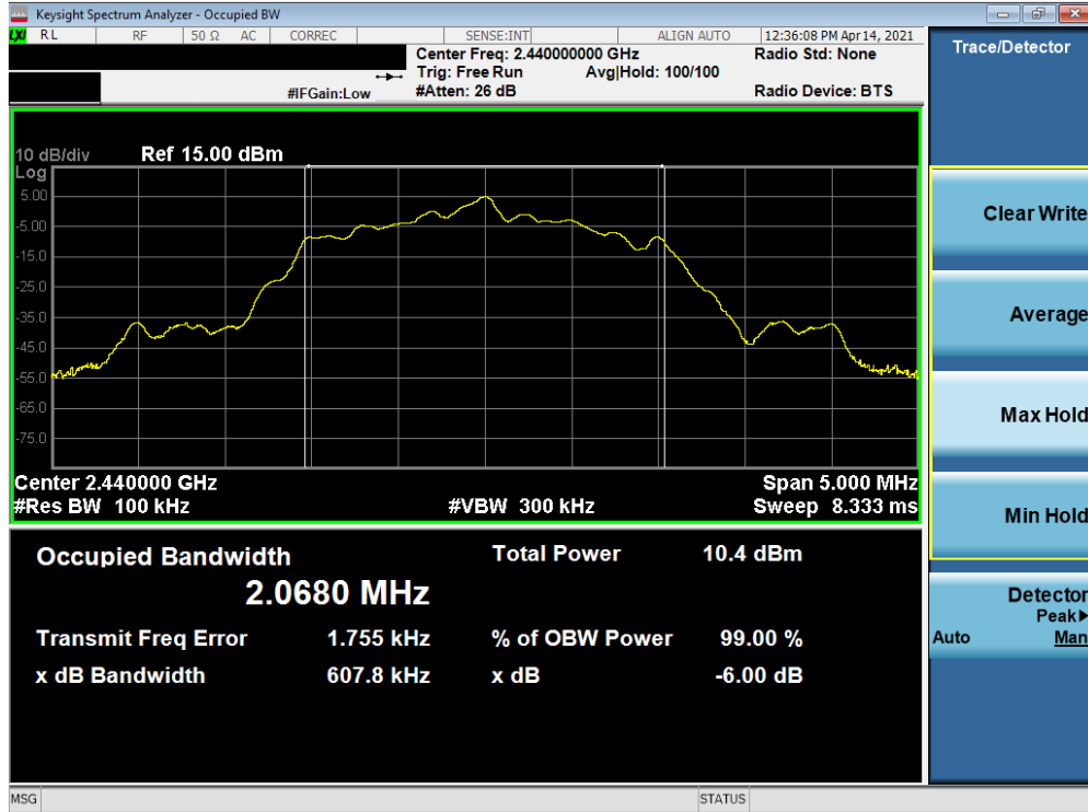
Plot 7-11. 6dB Bandwidth Plot (Bluetooth (LE), 2Mbps – Ch. 19) - N
