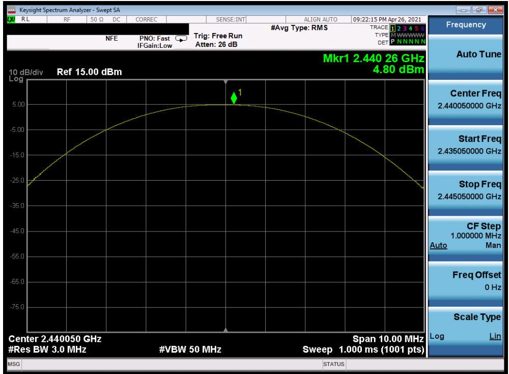
Plot 7-29. Peak Power Plot (Bluetooth (LE), 500kbps – Ch. 19) - N
