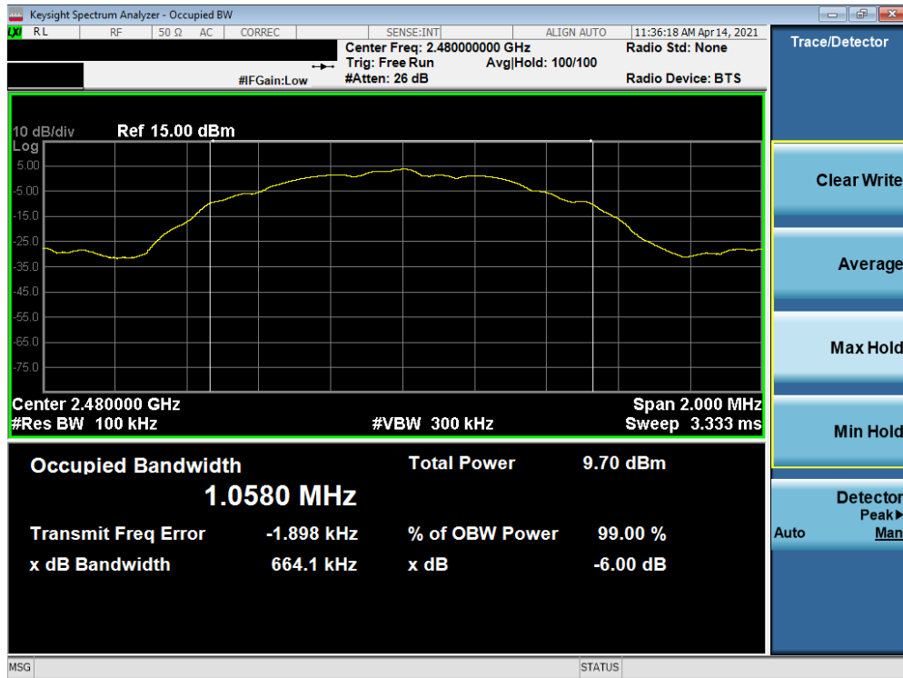
Plot 7-9. 6dB Bandwidth Plot (Bluetooth (LE), 1Mbps – Ch. 39) - N
