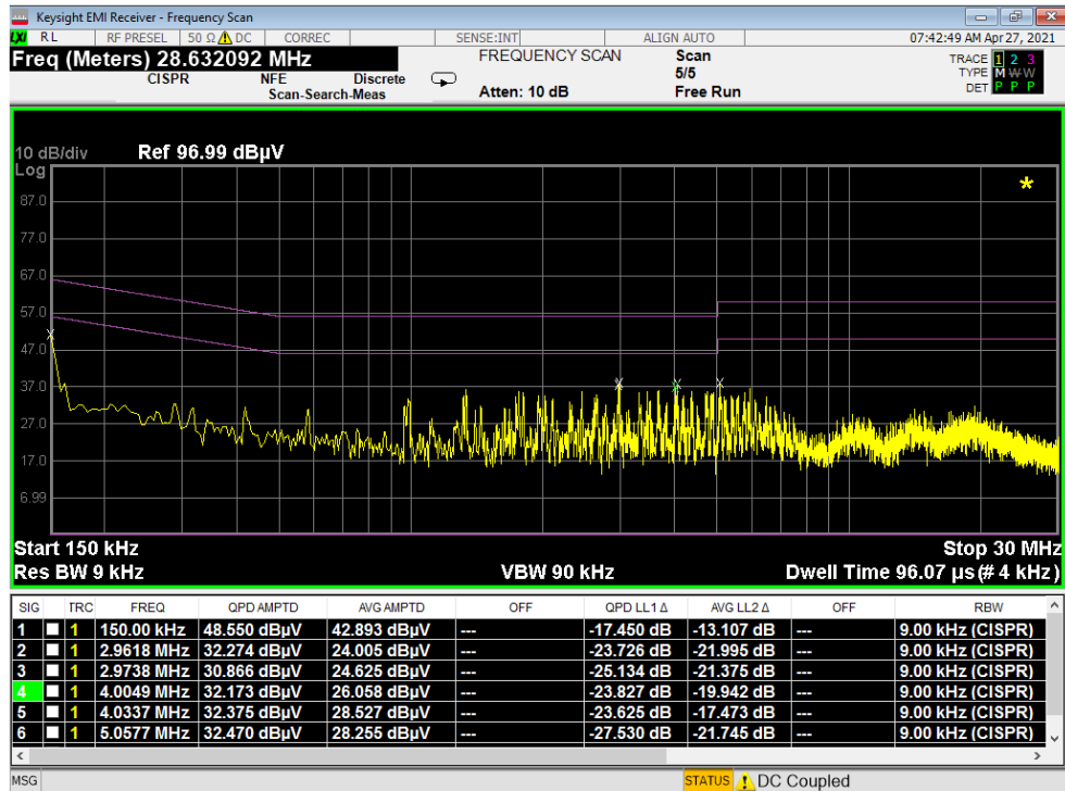
Plot 7-112. Line Conducted Plot with Bluetooth LE (N) - Q (CLOSED)
