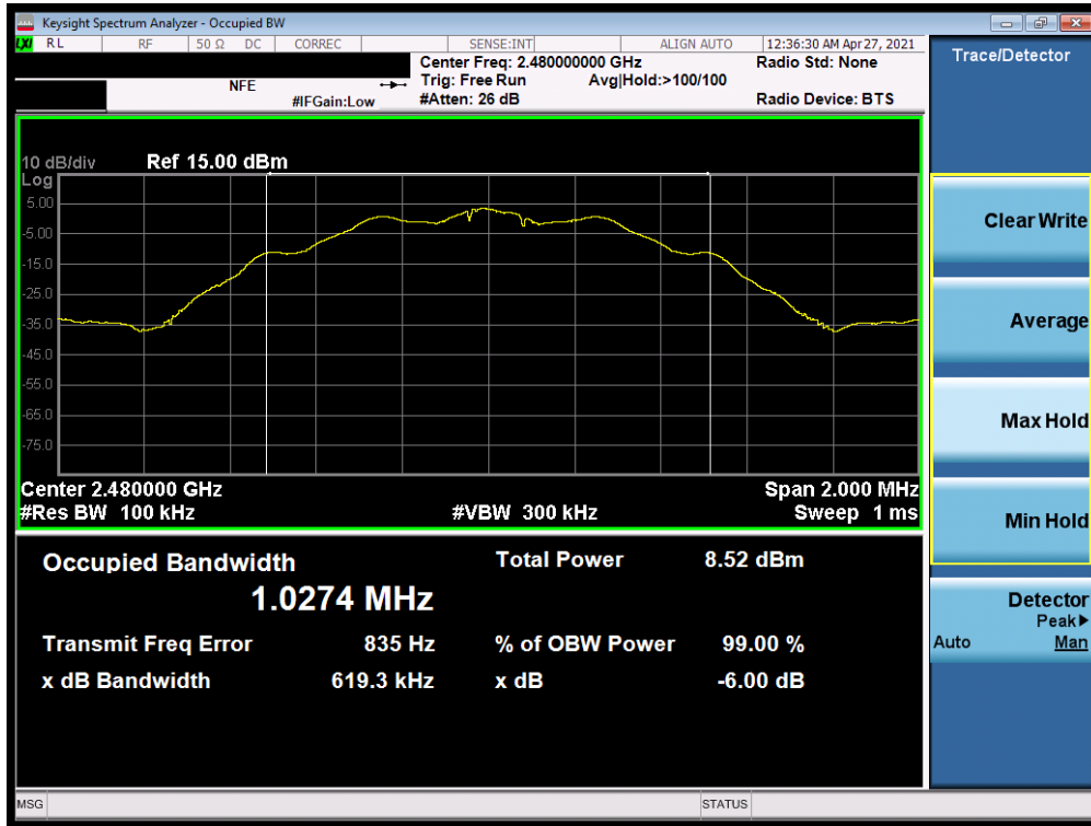
Plot 7-15. 6dB Bandwidth Plot (Bluetooth (LE), 125kbps – Ch. 39) – Q
