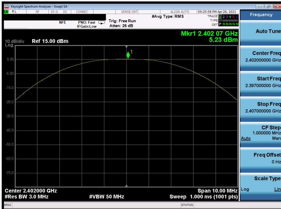
Plot 7-34. Peak Power Plot (Bluetooth (LE), 2Mbps – Ch. 0) - N
