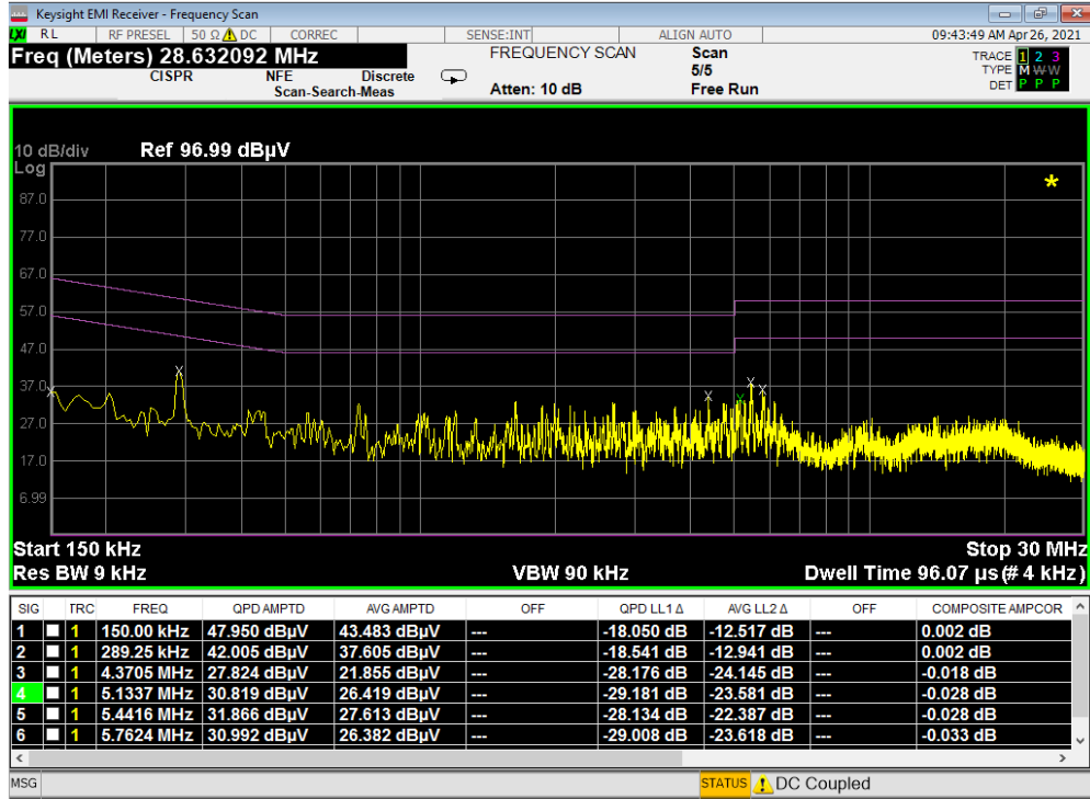
Plot 7-107. Line Conducted Plot with Bluetooth LE (L1) - N (CLOSED)
