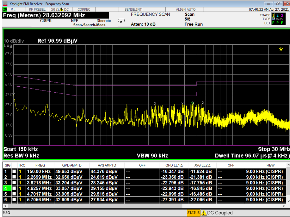
Plot 7-109. Line Conducted Plot with Bluetooth LE (L1) - Q (OPEN)
