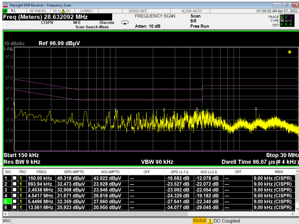
Plot 7-110. Line Conducted Plot with Bluetooth LE (N) - Q (OPEN)
