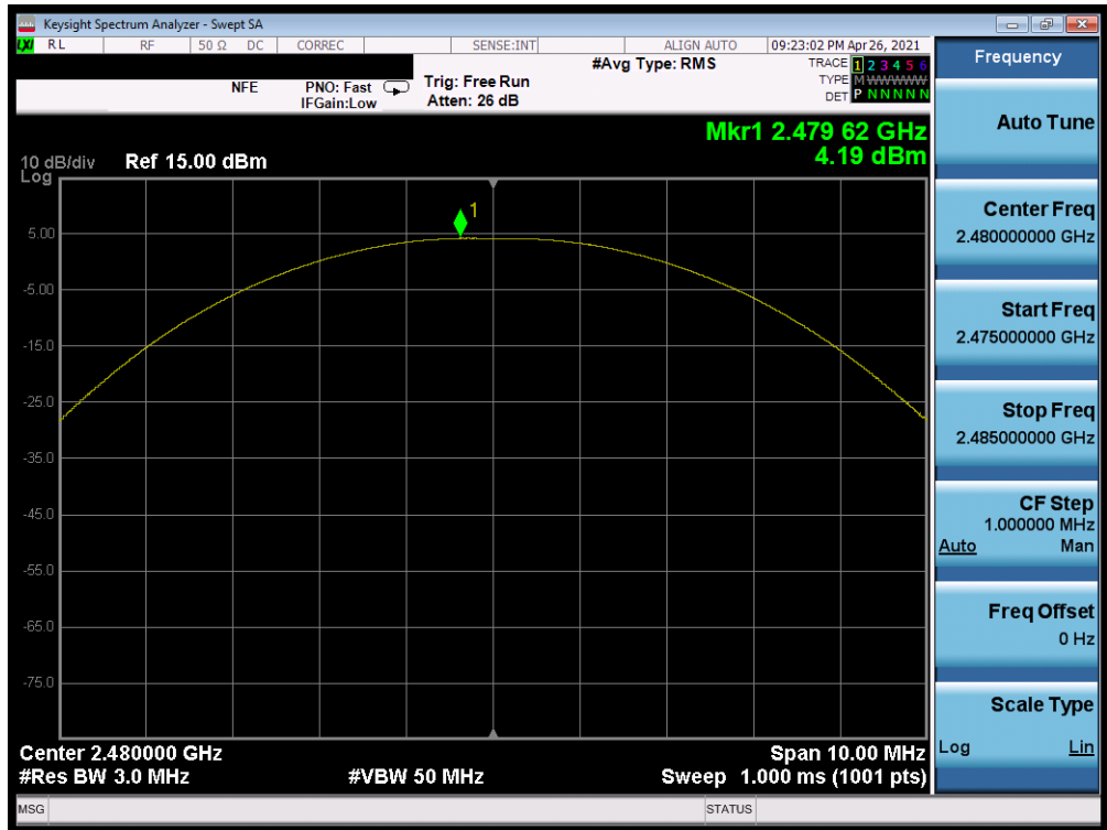
Plot 7-30. Peak Power Plot (Bluetooth (LE), 500kbps – Ch. 39) - N
