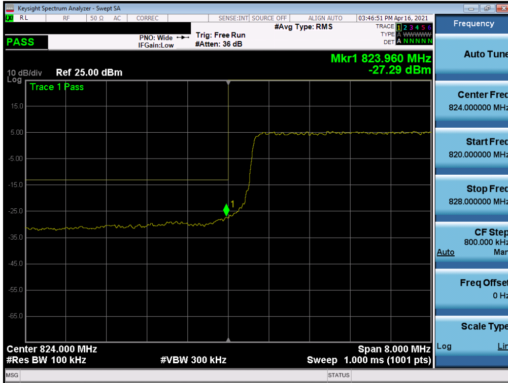
Plot 7-58. Lower Band Edge Plot (LTE Band 26/5 - 10MHz QPSK – Full RB)
