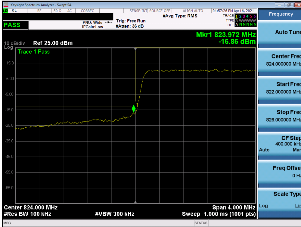
Plot 7-62. Lower Band Edge Plot (LTE Band 26/5 - 3MHz QPSK – Full RB)
