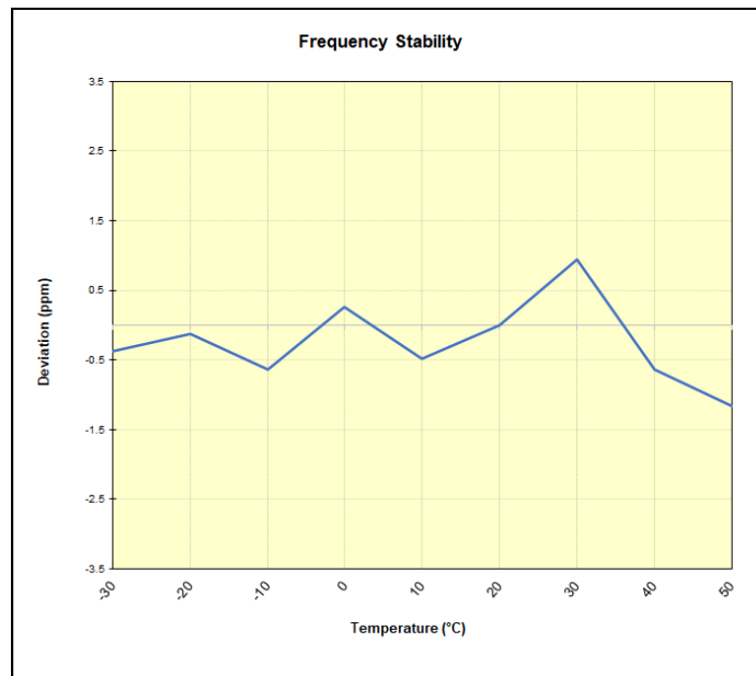
Plot 7-86. GSM/GPRS Cell Frequency Stability Chart
