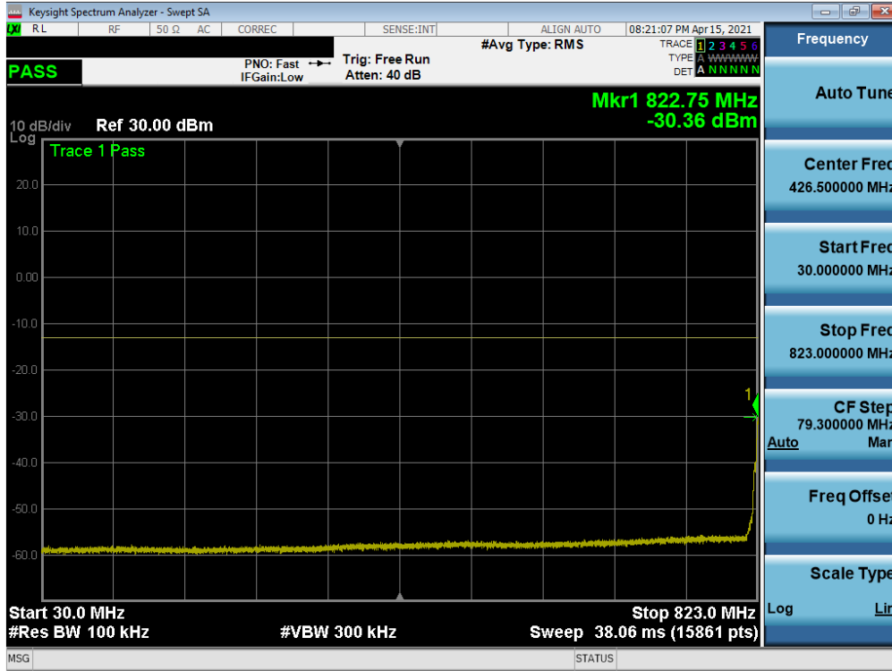
Plot 7-47. Conducted Spurious Plot (WCDMA Ch. 4132)
