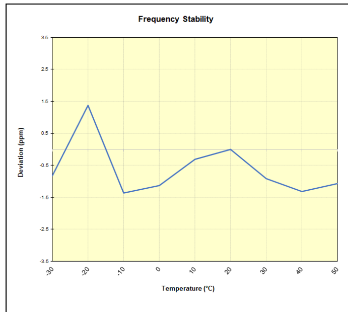
Plot 7-87. WCDMA Cell Frequency Stability Chart
