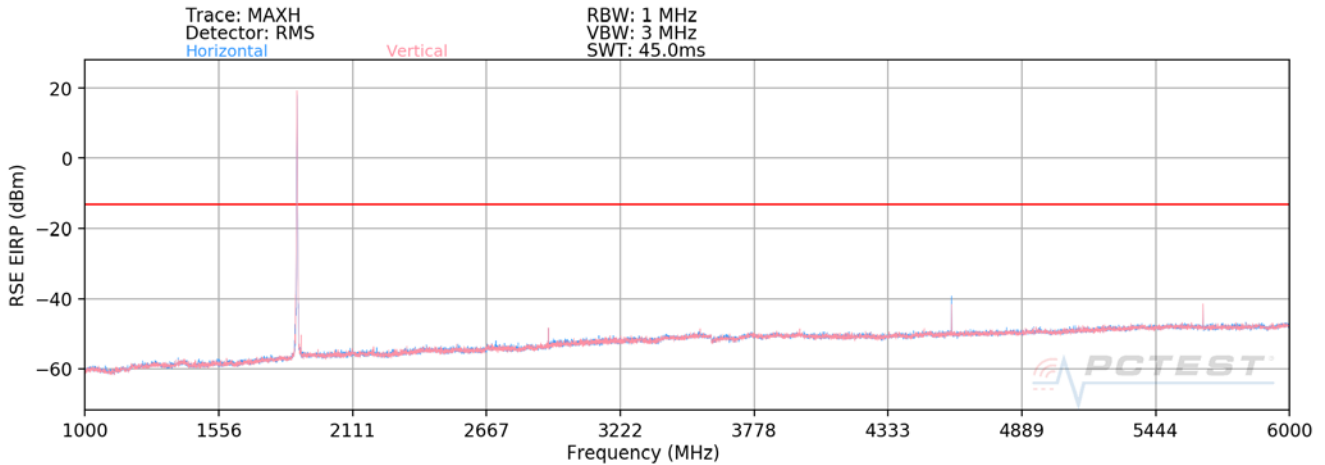
Plot 7-80. Radiated Spurious Plot 1 – 6 GHz (EN-DC n5 + B2)
