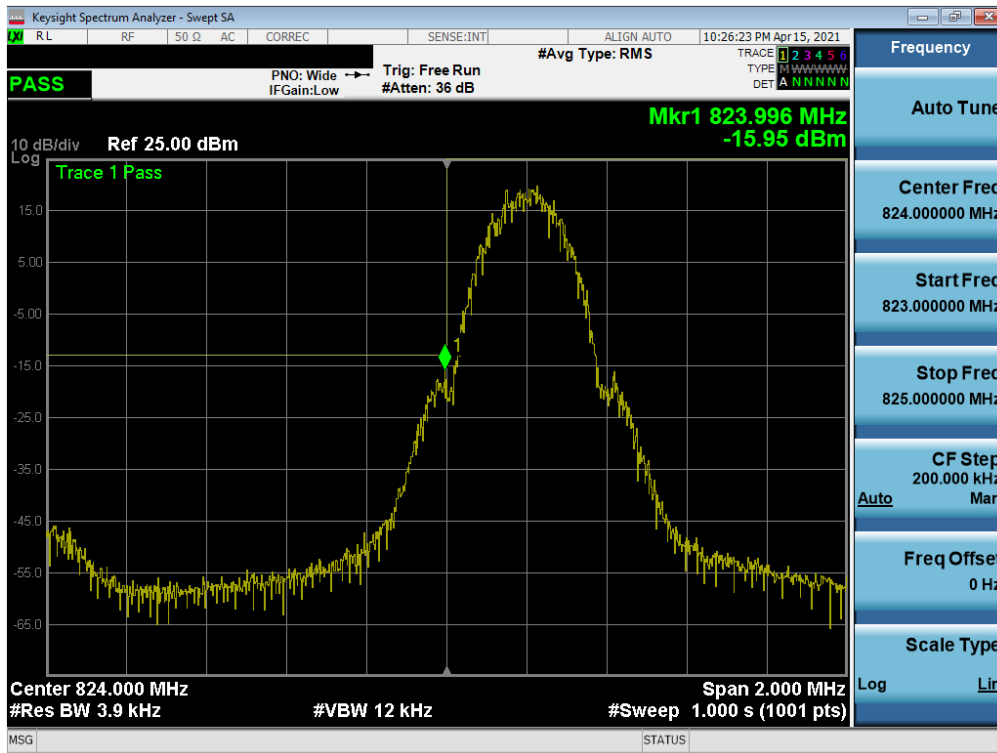
Plot 7-74. Lower Band Edge Plot (GPRS Cell – Ch. 128)
