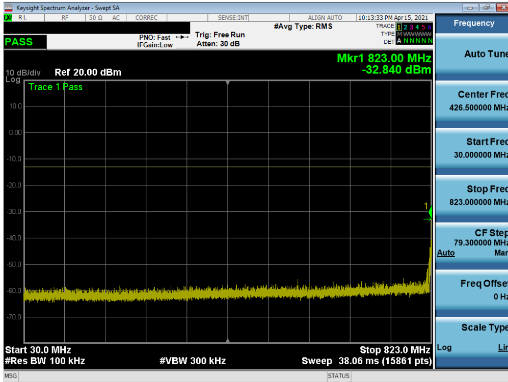
Plot 7-38. Conducted Spurious Plot (GPRS Ch. 128)
