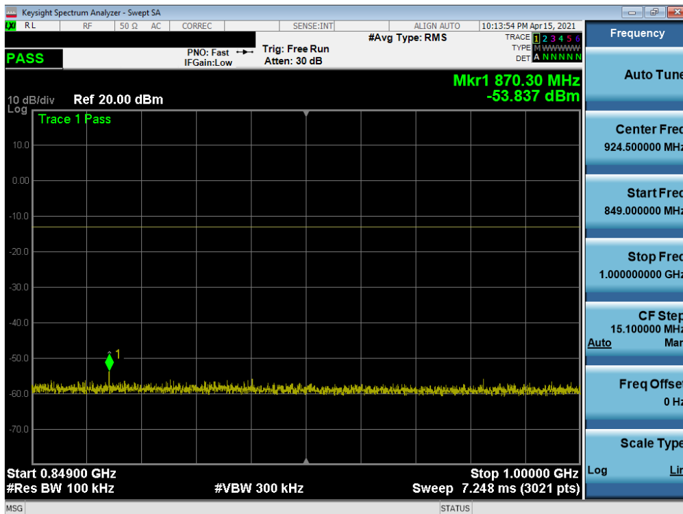
Plot 7-39. Conducted Spurious Plot (GPRS Ch. 128)
