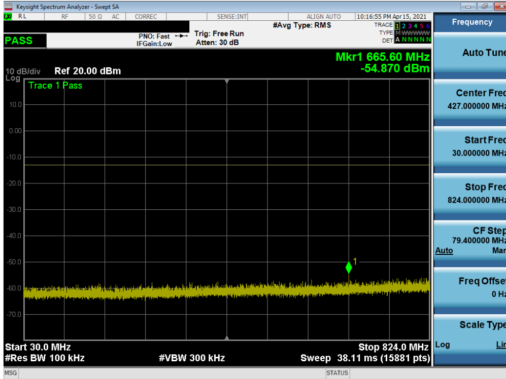
Plot 7-44. Conducted Spurious Plot (GPRS Ch. 251)
