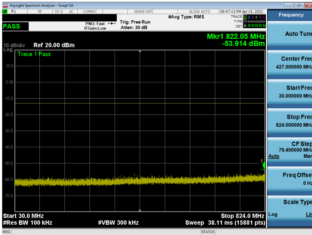
Plot 7-41. Conducted Spurious Plot (GPRS Ch. 190)
