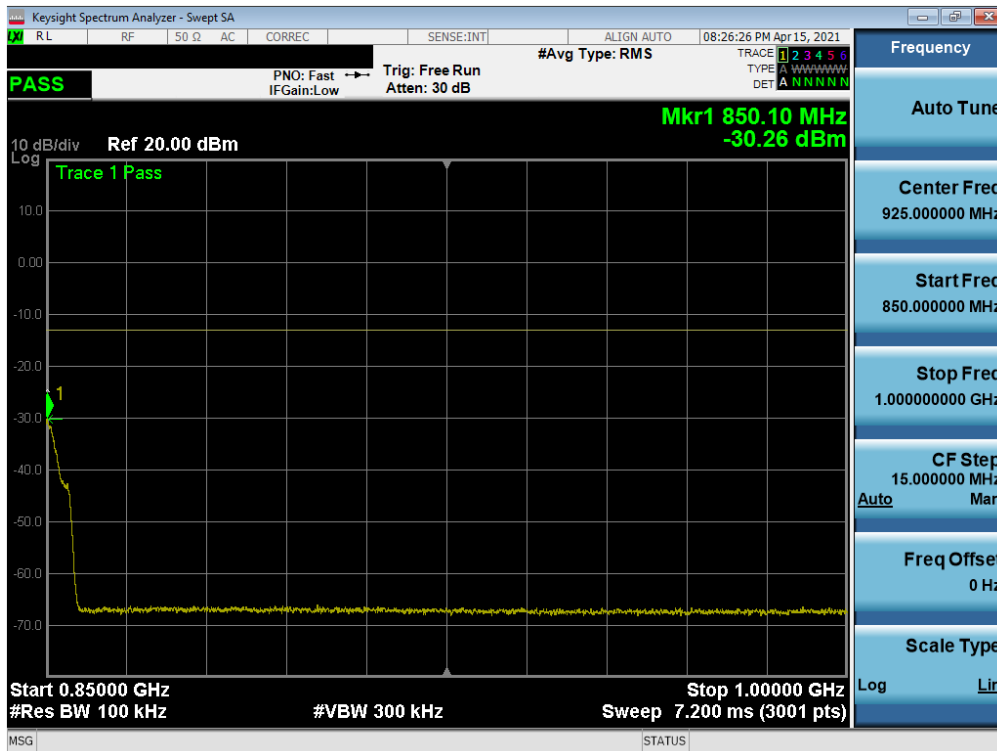
Plot 7-54. Conducted Spurious Plot (WCDMA Ch. 4233)
