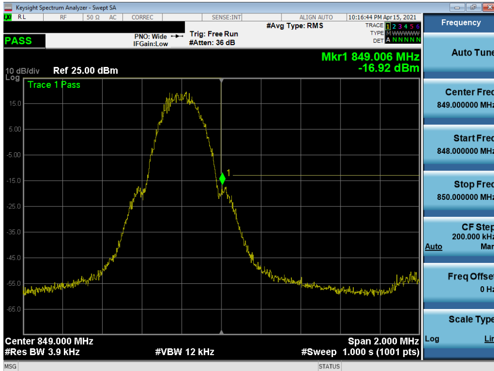
Plot 7-75. Upper Band Edge Plot (GPRS Cell – Ch. 251)
