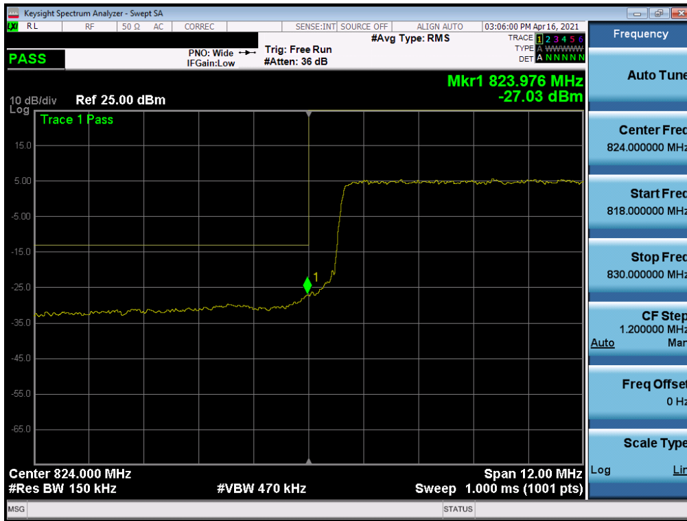
Plot 7-56. Lower Band Edge Plot (LTE Band 26 - 15MHz QPSK – Full RB)
