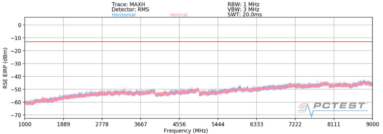
Plot 7-78. Radiated Spurious Plot (LTE Band 26/5)
