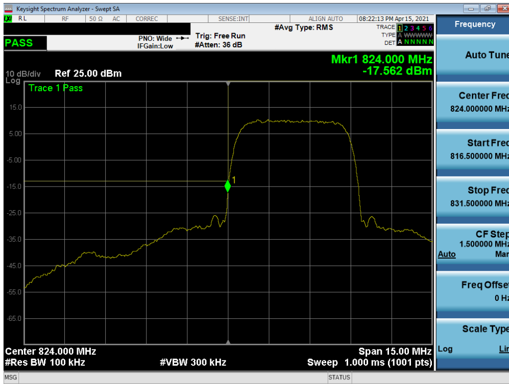
Plot 7-76. Lower Band Edge Plot (WCDMA Cell – Ch. 4132)
