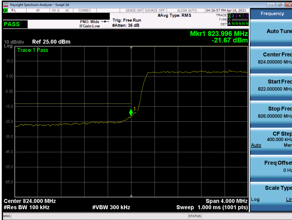
Plot 7-60. Lower Band Edge Plot (LTE Band 26/5 - 5MHz QPSK – Full RB)
