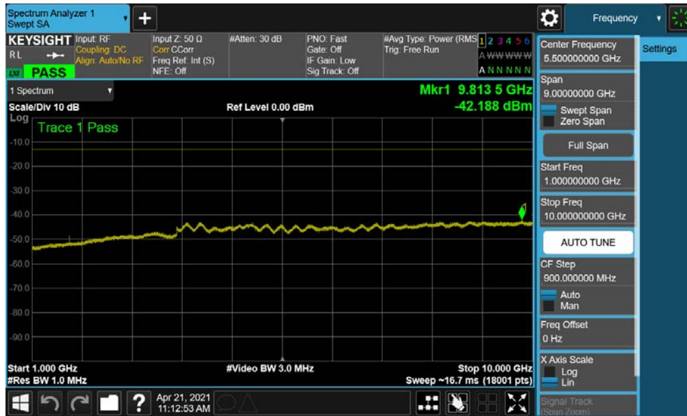
Plot 7-37. Conducted Spurious Plot (NR Band n5 - 20.0MHz - 1 RB)
