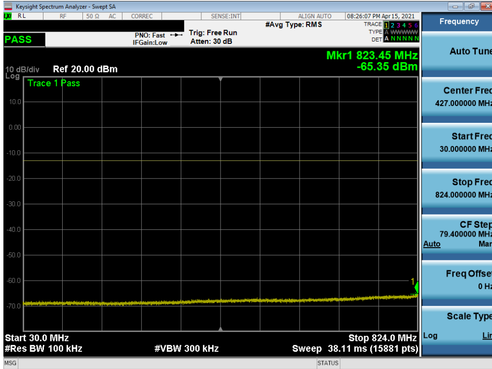
Plot 7-53. Conducted Spurious Plot (WCDMA Ch. 4233)
