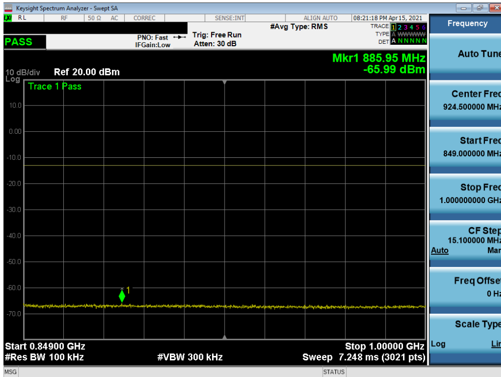
Plot 7-48. Conducted Spurious Plot (WCDMA Ch. 4132)
