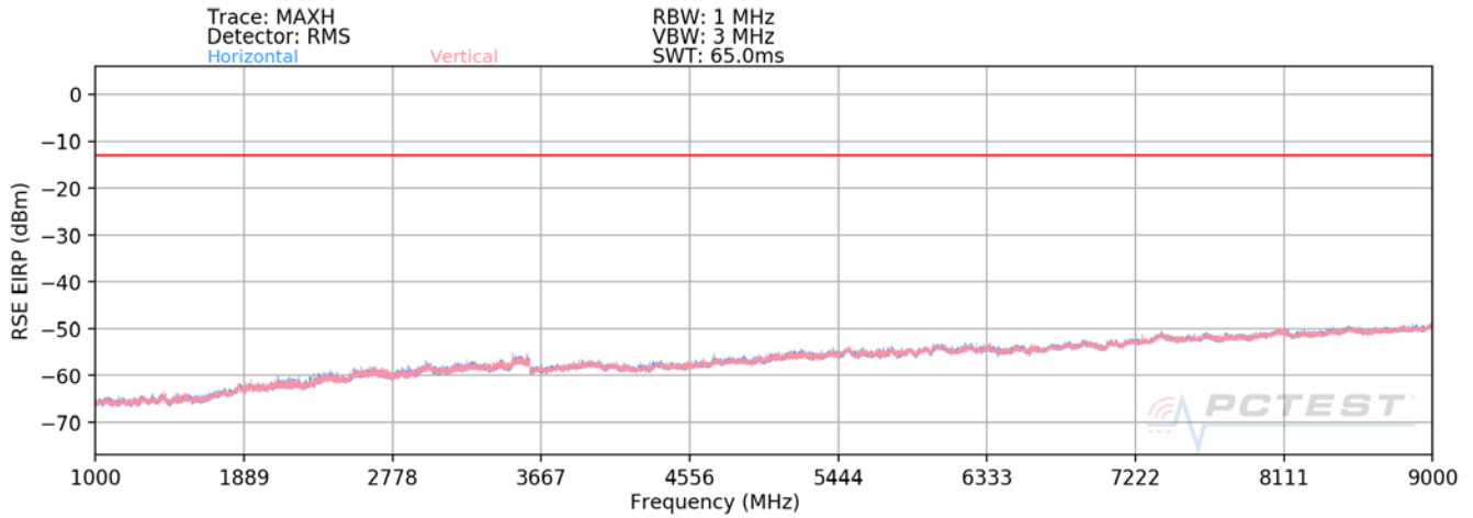
Plot 7-79. Radiated Spurious Plot (NR Band n5)
