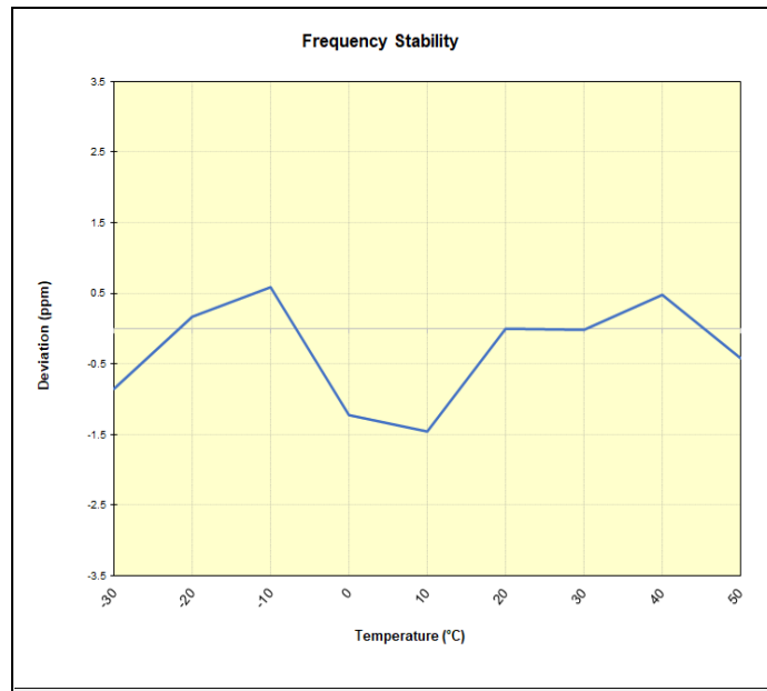
Plot 7-85. NR Band n5 Frequency Stability Chart
