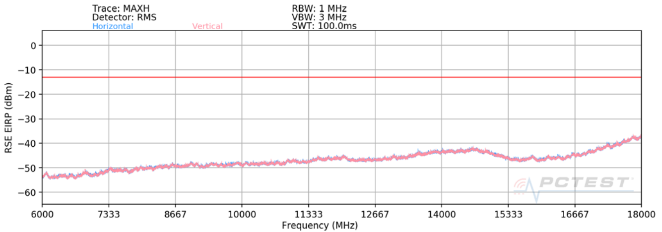
Plot 7-81. Radiated Spurious Plot 6 – 18 GHz (EN-DC n5 + B2)
