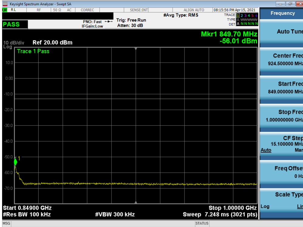
Plot 7-51. Conducted Spurious Plot (WCDMA Ch. 4183)
