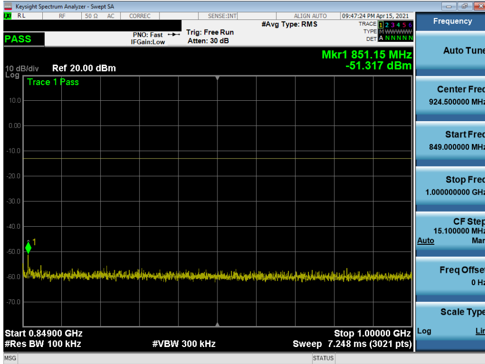
Plot 7-42. Conducted Spurious Plot (GPRS Ch. 190)
