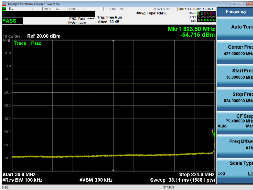
Plot 7-50. Conducted Spurious Plot (WCDMA Ch. 4183)
