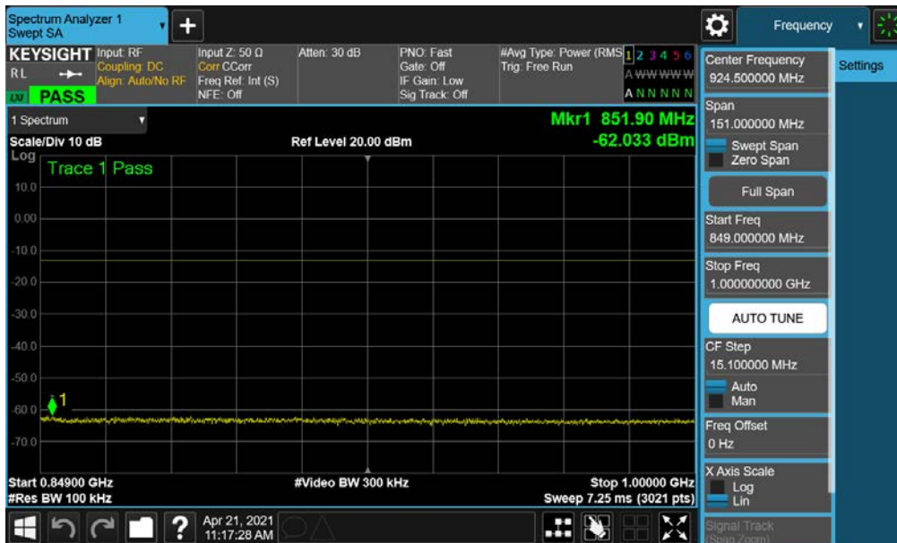
Plot 7-36. Conducted Spurious Plot (NR Band n5 - 20.0MHz - 1 RB)
