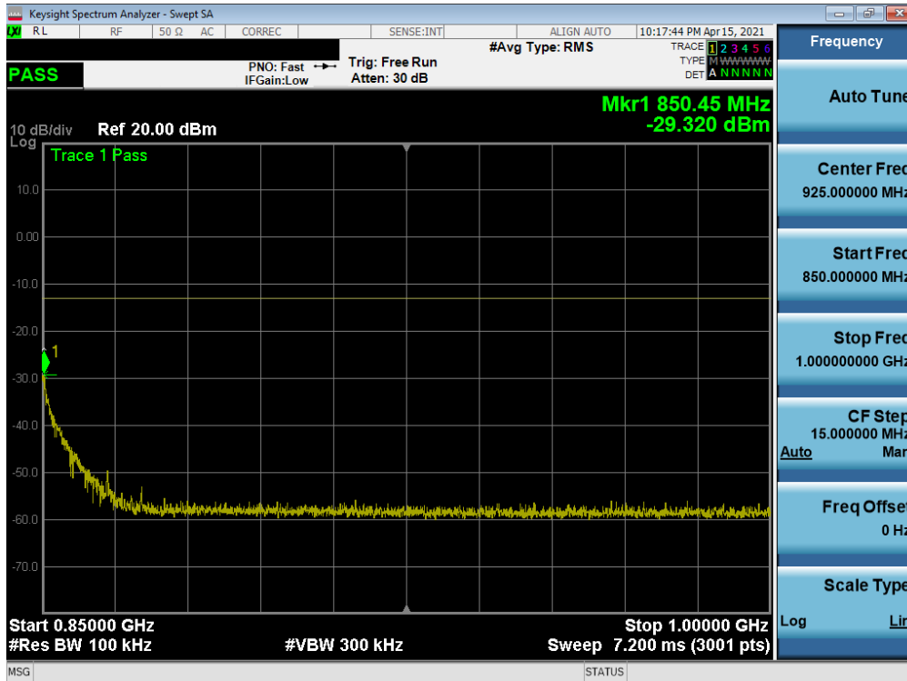
Plot 7-45. Conducted Spurious Plot (GPRS Ch. 251)
