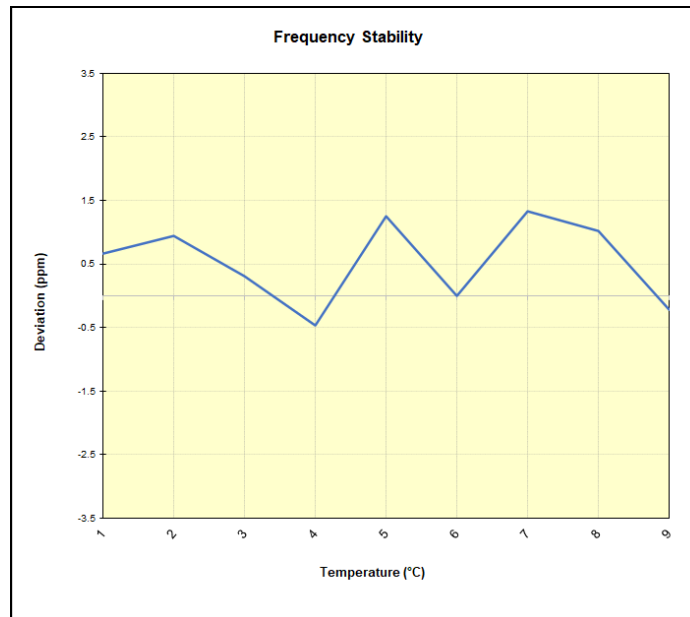
Plot 7-84. LTE Band 26/5 Frequency Stability Chart
