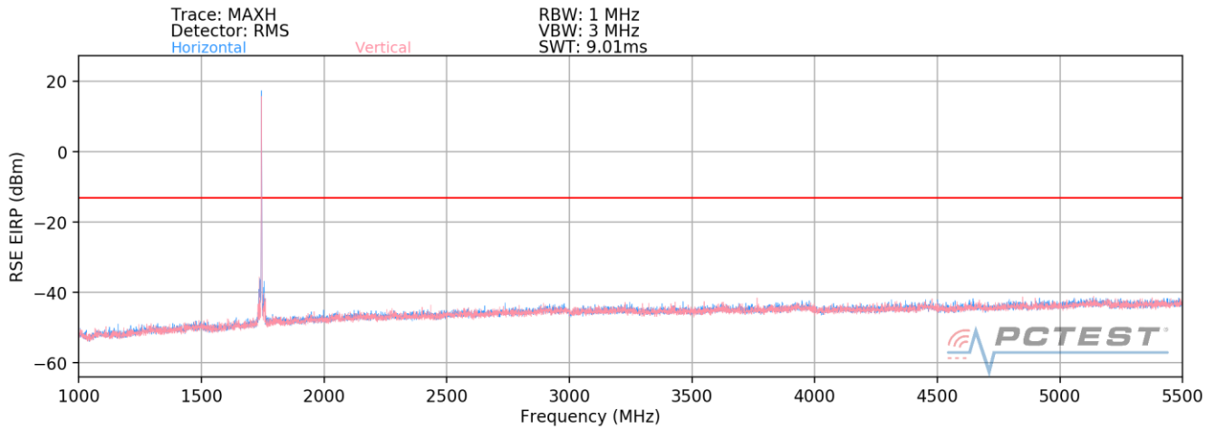
Plot 7-3. Radiated Spurious Plot (NR Band n66-B14 - Closed)
