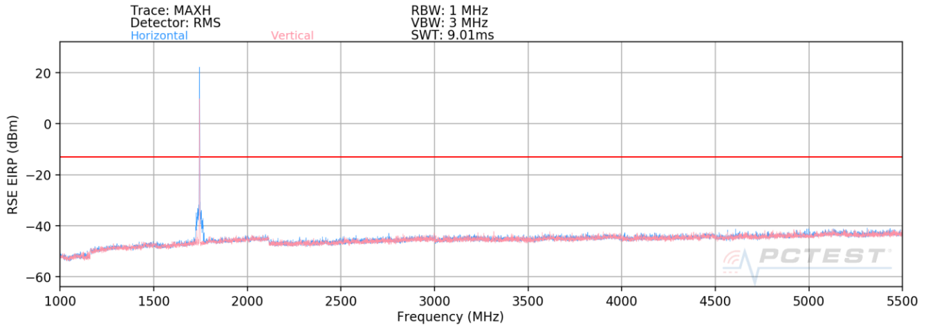
Plot 7-1. Radiated Spurious Plot (NR Band n66-B14 - Open)
