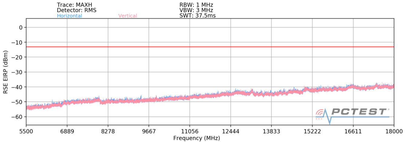
Plot 7-4. Radiated Spurious Plot (NR Band n66-B14 - Closed)
