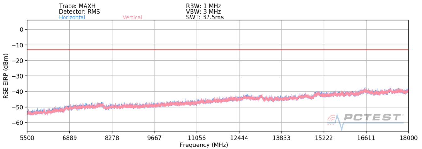
Plot 7-2. Radiated Spurious Plot (NR Band n66-B14 - Open)
