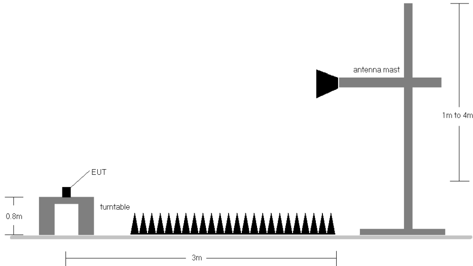
Figure 7-1. Test Instrument & Measurement Setup
