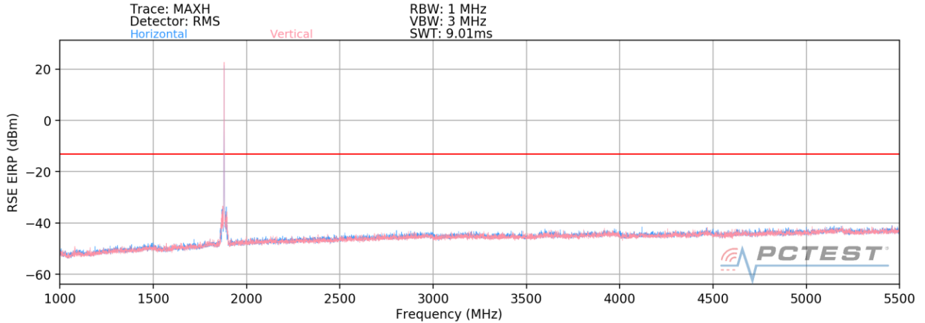
Plot 7-3. Radiated Spurious Plot (NR Band n2-B14 - Closed)
