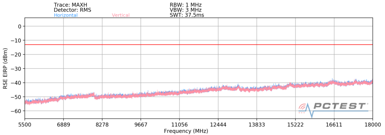
Plot 7-4. Radiated Spurious Plot (NR Band n2-B14 - Closed)
