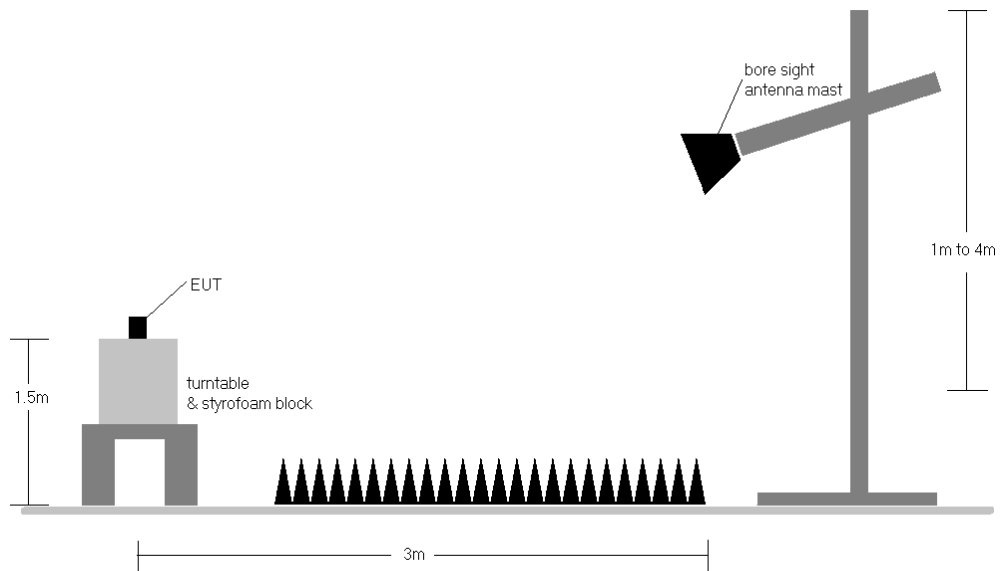
Figure 7-2. Test Instrument & Measurement Setup >1 GHz
