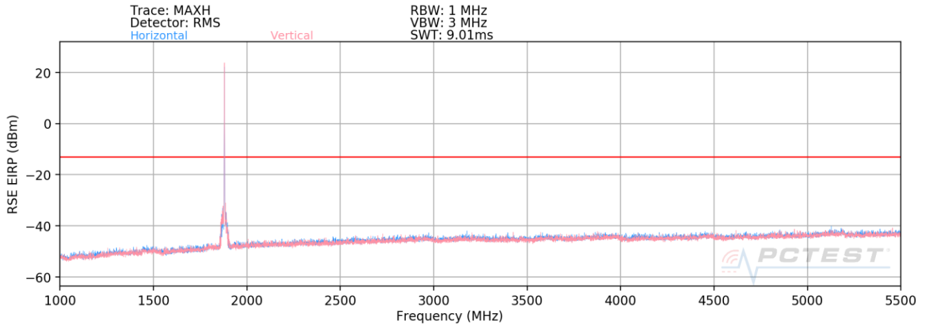
Plot 7-1. Radiated Spurious Plot (NR Band n2-B14 - Open)
