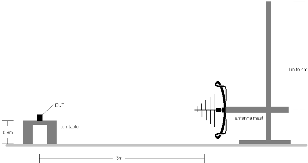
Figure 7-1. Test Instrument & Measurement Setup < 1GHz
