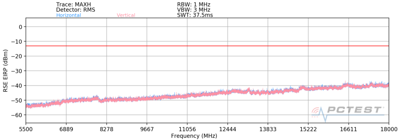
Plot 7-2. Radiated Spurious Plot (NR Band n2-B14 - Open)
