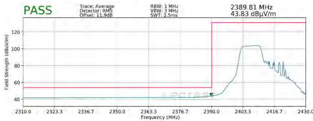
Plot 7-85. Radiated Restricted Lower Band Edge Measurement SISO ANT1 (Average – 106 Tones)
