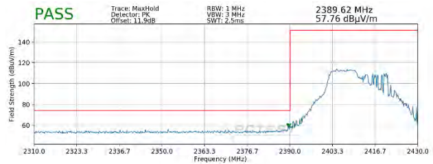
Plot 7-86. Radiated Restricted Lower Band Edge Measurement SISO ANT1 (Peak – 106 Tones)
