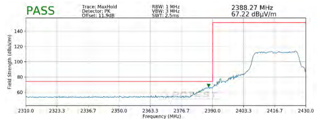
Plot 7-120. Radiated Restricted Lower Band Edge Measurement MIMO (Peak – 242 Tones)
