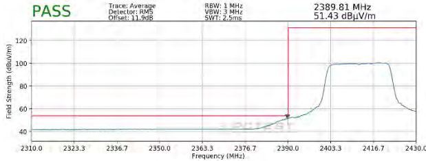
Plot 7-117. Radiated Restricted Lower Band Edge Measurement MIMO (Average – 242 Tones)
