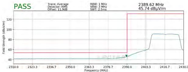
Plot 7-105. Radiated Restricted Lower Band Edge Measurement SISO ANT2 (Average – 242 Tones)
