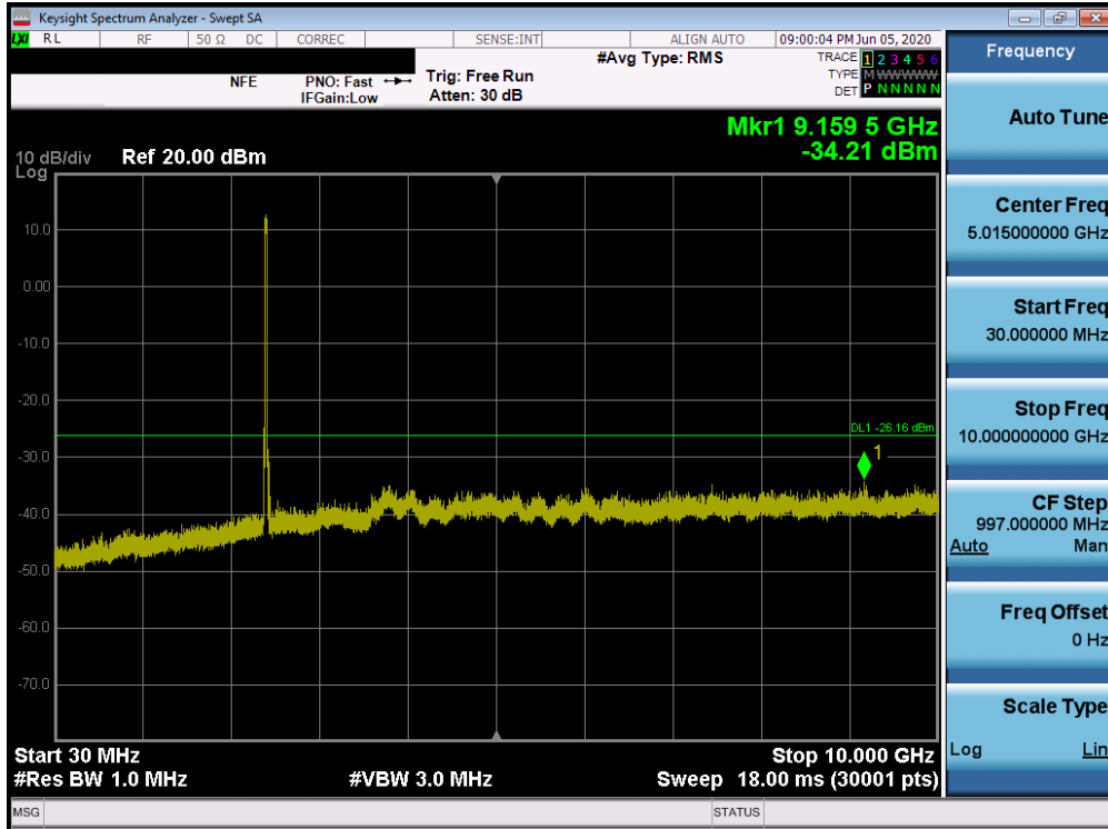
Plot 7-45. Conducted Spurious Plot SISO ANT1 (802.11ax OFDMA – 242 Tones – Ch. 1)
