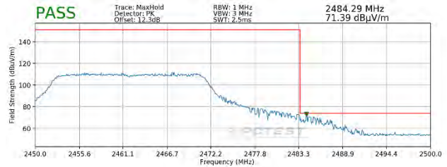
Plot 7-98. Radiated Restricted Upper Band Edge Measurement SISO ANT1 (Peak – 242 Tones)
