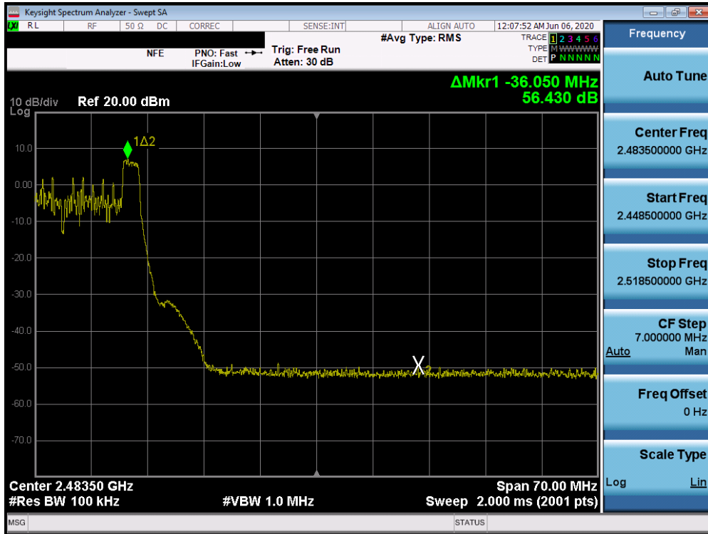
Plot 7-29. Band Edge Plot SISO ANT1 (802.11ax OFDMA – 52 Tones – Ch. 9)
