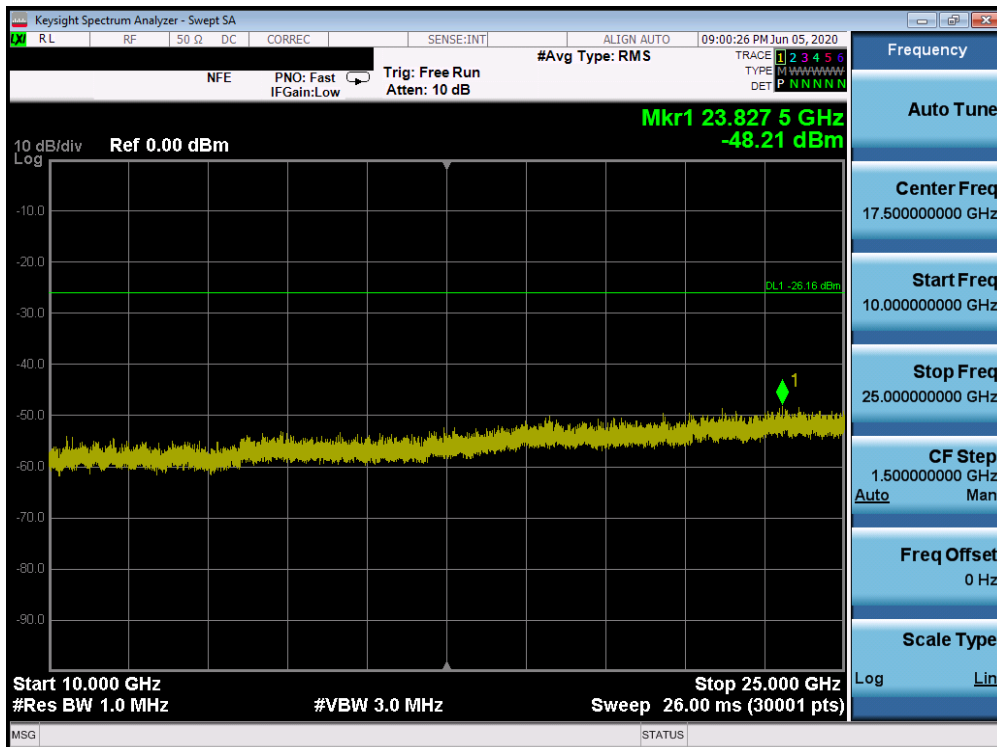
Plot 7-46. Conducted Spurious Plot SISO ANT1 (802.11ax OFDMA – 242 Tones – Ch. 1)
