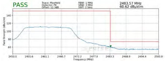
Plot 7-112. Radiated Restricted Upper Band Edge Measurement SISO ANT1 (Peak)
