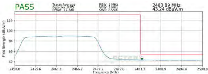
Plot 7-119. Radiated Restricted Upper Band Edge Measurement SISO ANT2 (Average)
