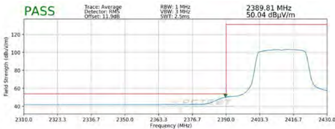
Plot 7-113. Radiated Restricted Lower Band Edge Measurement SISO ANT2 (Average)
