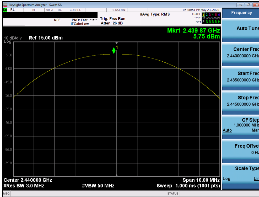
Plot 7-17. Peak Power Plot (Bluetooth (LE), 500kbps – Ch. 19)
