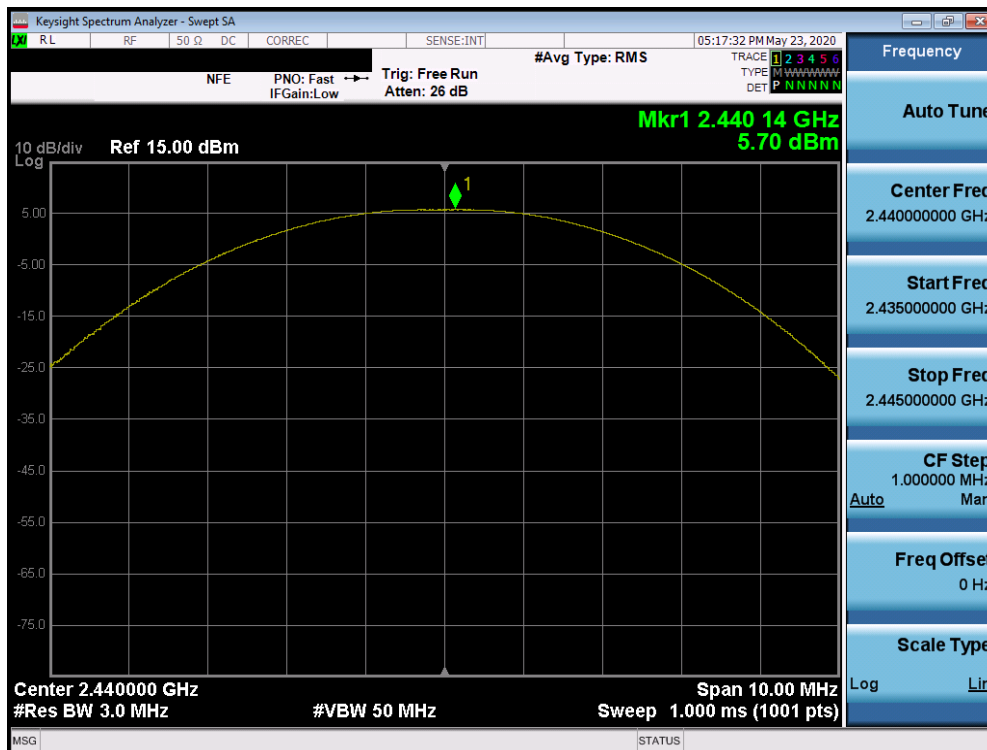
Plot 7-20. Peak Power Plot (Bluetooth (LE), 1Mbps – Ch. 19)
