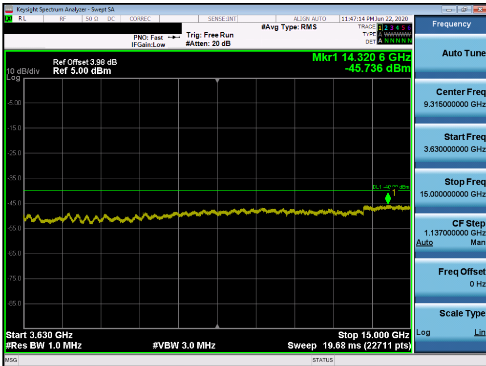
Plot 7-66. Conducted Spurious Plot (Band 48 – 20.0MHz QPSK – PCC 1/99 SCC 1/0 – Low Channel)
