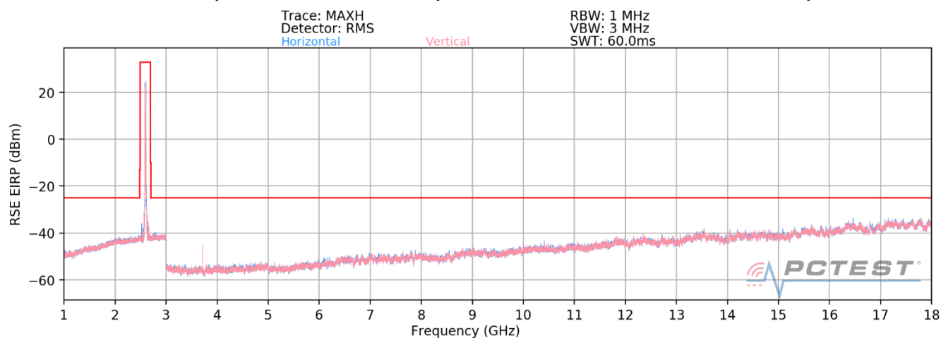
Plot 7-69. Radiated Spurious Plot 1GHz - 18GHz (ULCA Band 41 Mid Channel – PCC/SCC: 1RB) – OPEN
