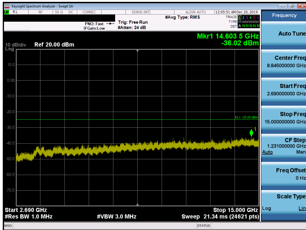
Plot 7-33. Conducted Spurious Plot (Band 41 – 20.0MHz QPSK – Left Carrier 1/99 Right Carrier 1/0 – Mid Channel)
