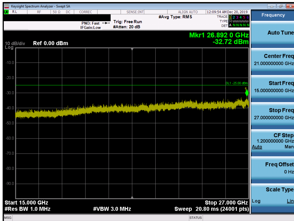
Plot 7-34. Conducted Spurious Plot (Band 41 – 20.0MHz QPSK – Left Carrier 1/99 Right Carrier 1/0 – Mid Channel)
