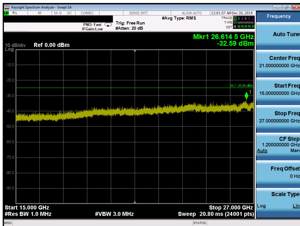
Plot 7-30. Conducted Spurious Plot (Band 41 – 20.0MHz QPSK – Left Carrier 1/99 Right Carrier 1/0 – Low Channel)
