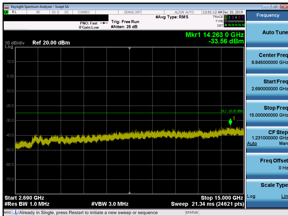
Plot 7-29. Conducted Spurious Plot (Band 41 – 20.0MHz QPSK – Left Carrier 1/99 Right Carrier 1/0 – Low Channel)
