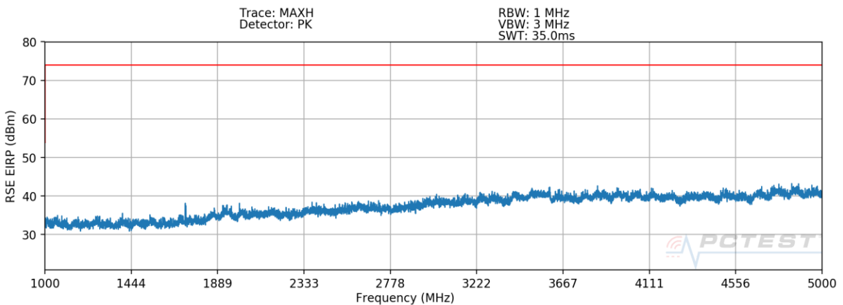
Plot 7-6. Radiated Spurious Plot above 1GHz – V – OPEN
