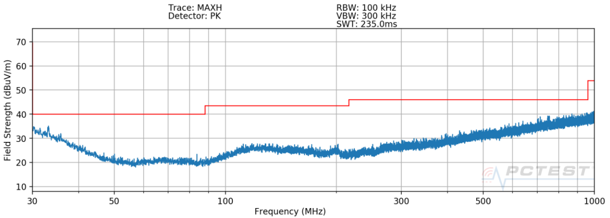
Plot 7-2. Radiated Spurious Plot below 1GHz – V – OPEN
