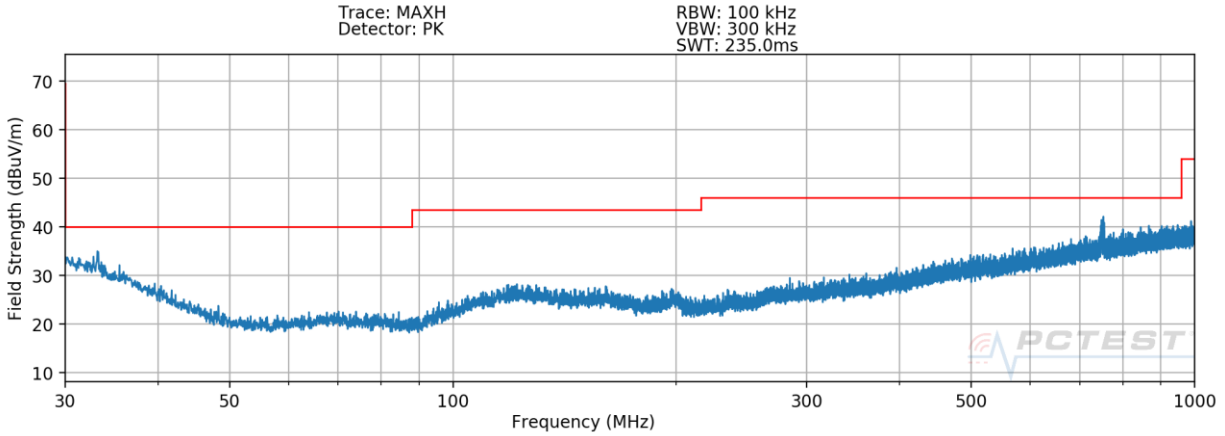
Plot 7-4. Radiated Spurious Plot below 1GHz – V – CLOSED
