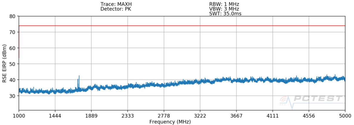
Plot 7-7. Radiated Spurious Plot above 1GHz – H – CLOSED
