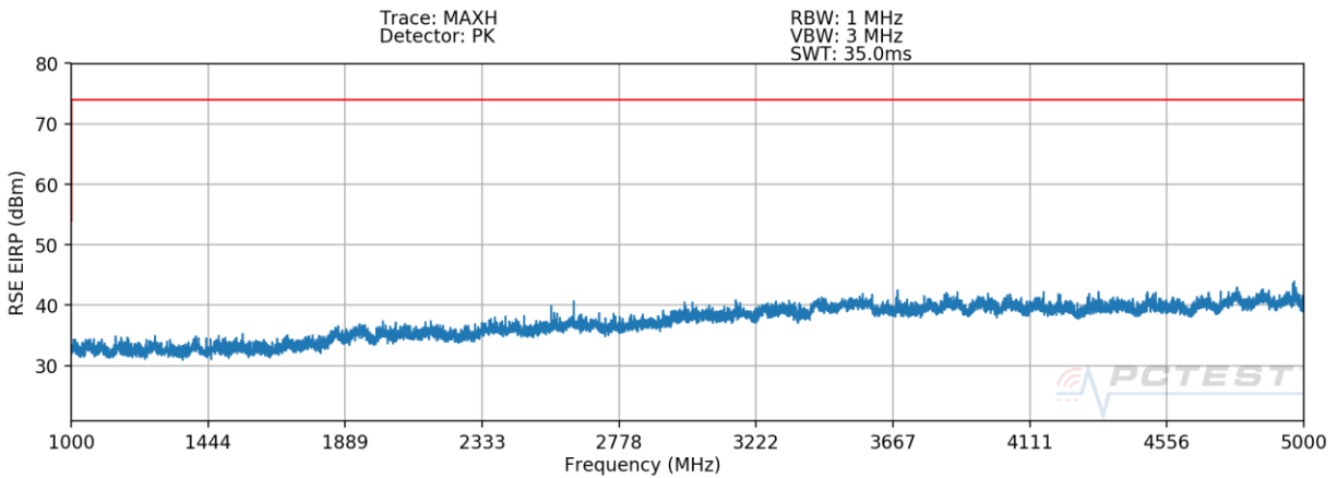
Plot 7-5. Radiated Spurious Plot above 1GHz – H – OPEN
