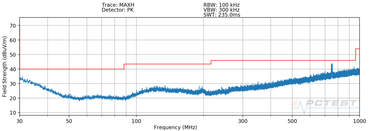
Plot 7-1. Radiated Spurious Plot below 1GHz – H – OPEN
