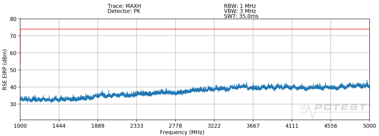
Plot 7-8. Radiated Spurious Plot above 1GHz – V – CLOSED
