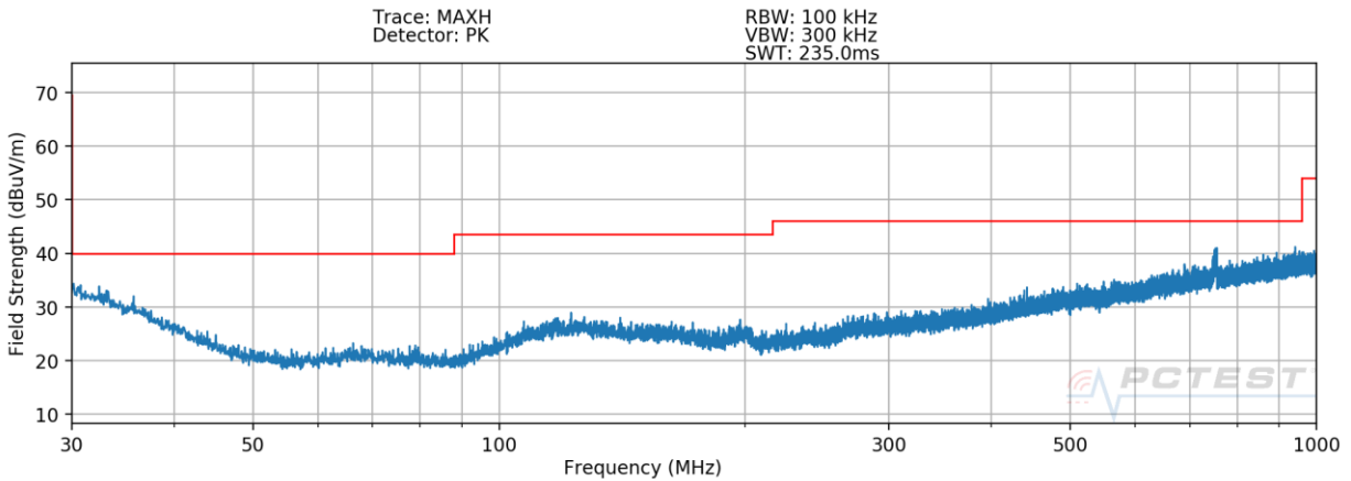
Plot 7-3. Radiated Spurious Plot below 1GHz – H – CLOSED
