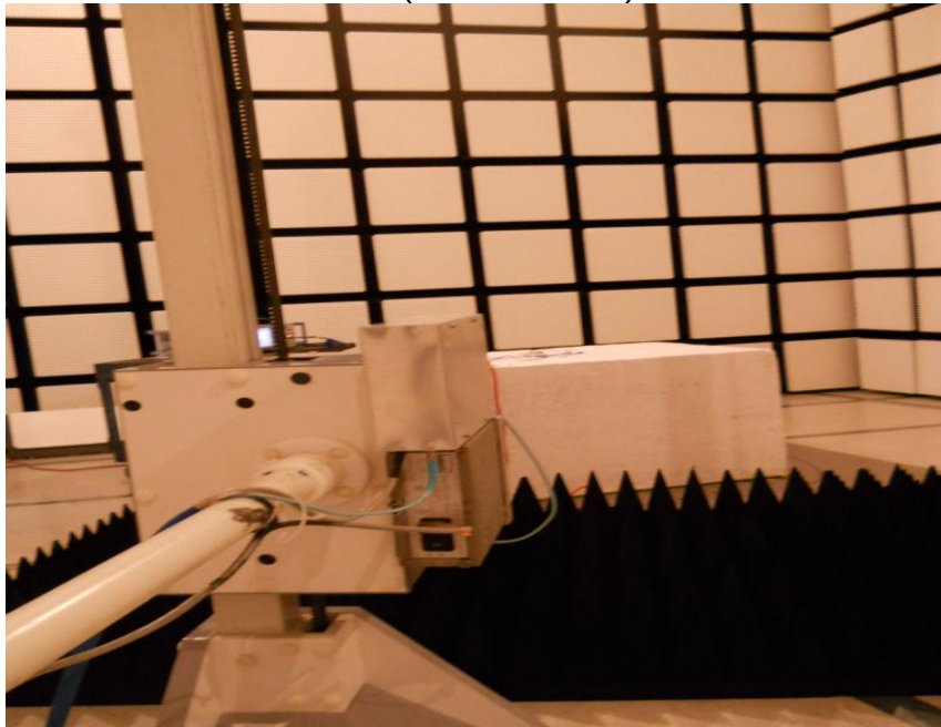
RADIATED BACK PHOTO (ABOVE 1 GHz)
