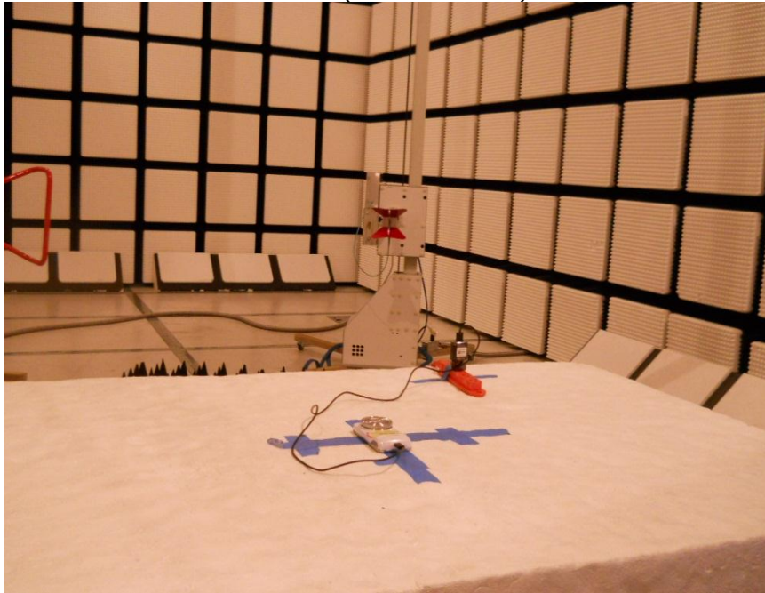
RADIATED FRONT PHOTO (ABOVE 1 GHz)
