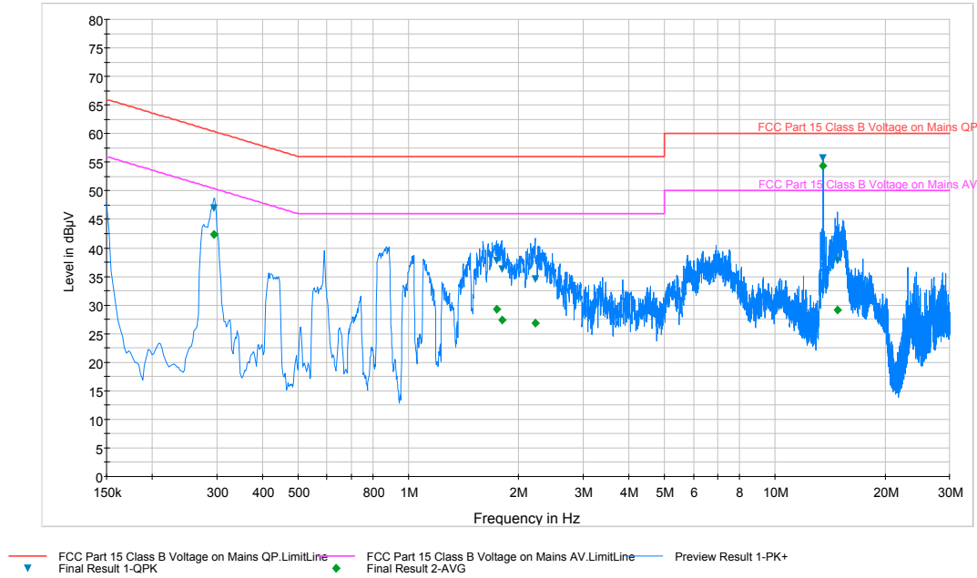
Plot 8-2. Line-Conducted Test Plot (N)
