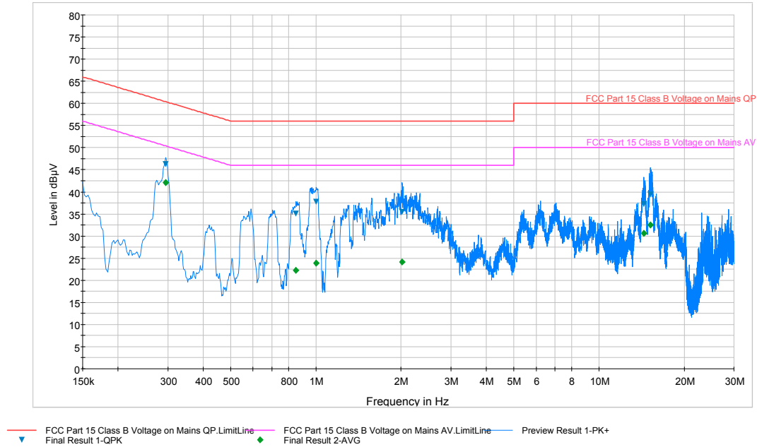
Plot 8-3. Line-Conducted Test Plot (L1)
