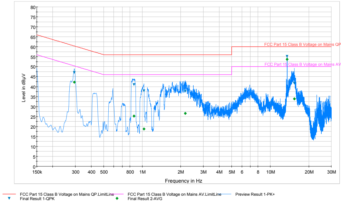
Plot 8-1. Line-Conducted Test Plot (L1)
