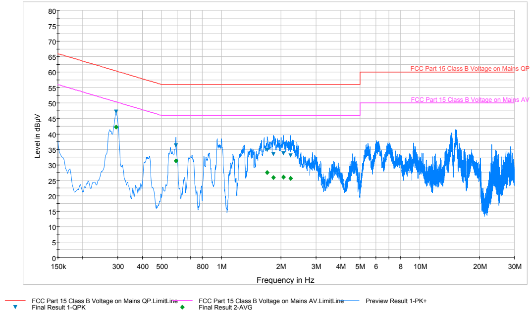
Plot 8-4. Line-Conducted Test Plot (N)
