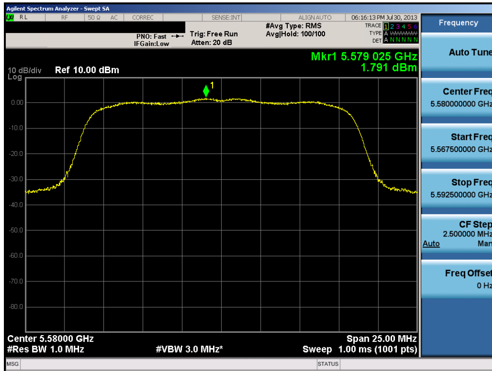
Plot 6-44. Peak Power Spectral Density Plot (802.11a (UNII Band 3) – Ch. 116)
