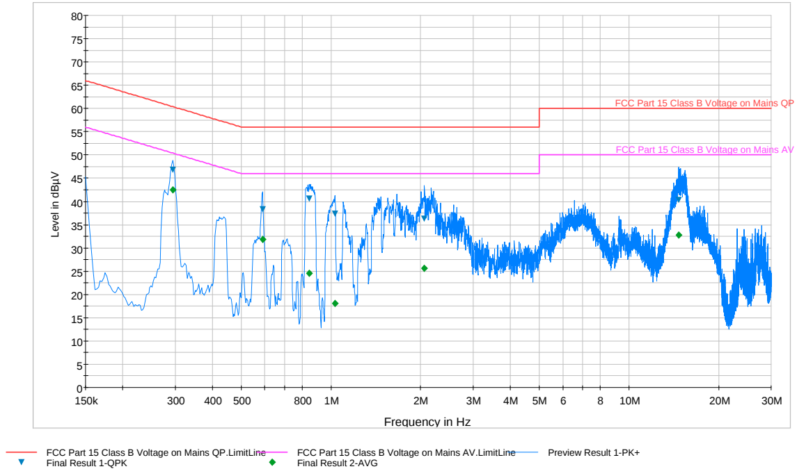
Plot 6-69. Line Conducted Plot with 802.11a UNII Band 1 (L1)
