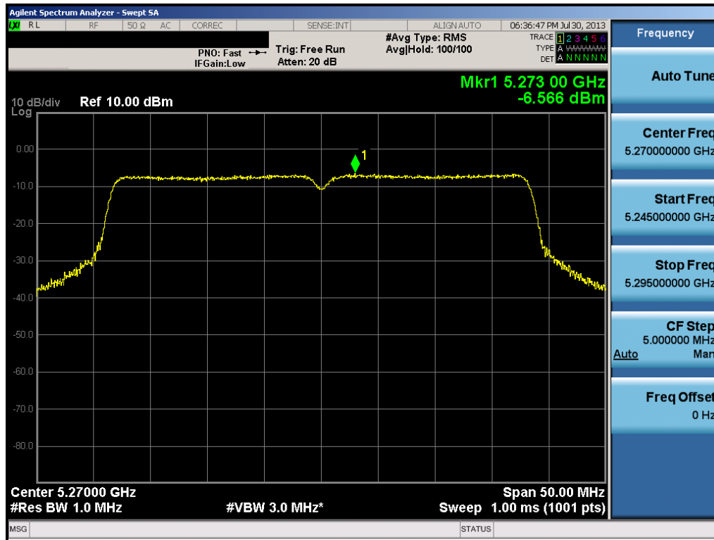
Plot 6-41. Peak Power Spectral Density Plot (40MHz BW 802.11n (UNII Band 2) – Ch. 54)
