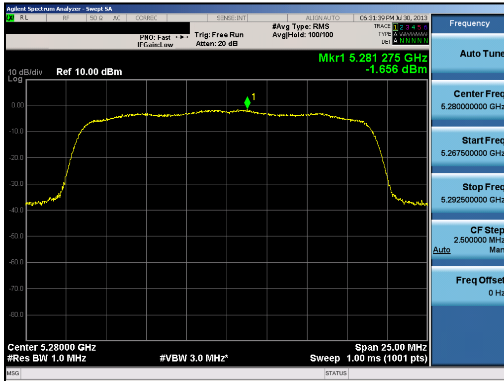
Plot 6-39. Peak Power Spectral Density Plot (20MHz BW 802.11n (UNII Band 2) – Ch. 56)
