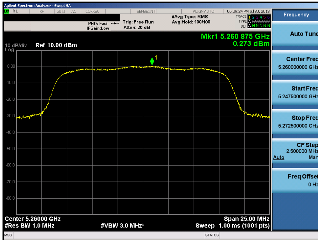
Plot 6-35. Peak Power Spectral Density Plot (802.11a (UNII Band 2) – Ch. 52)
