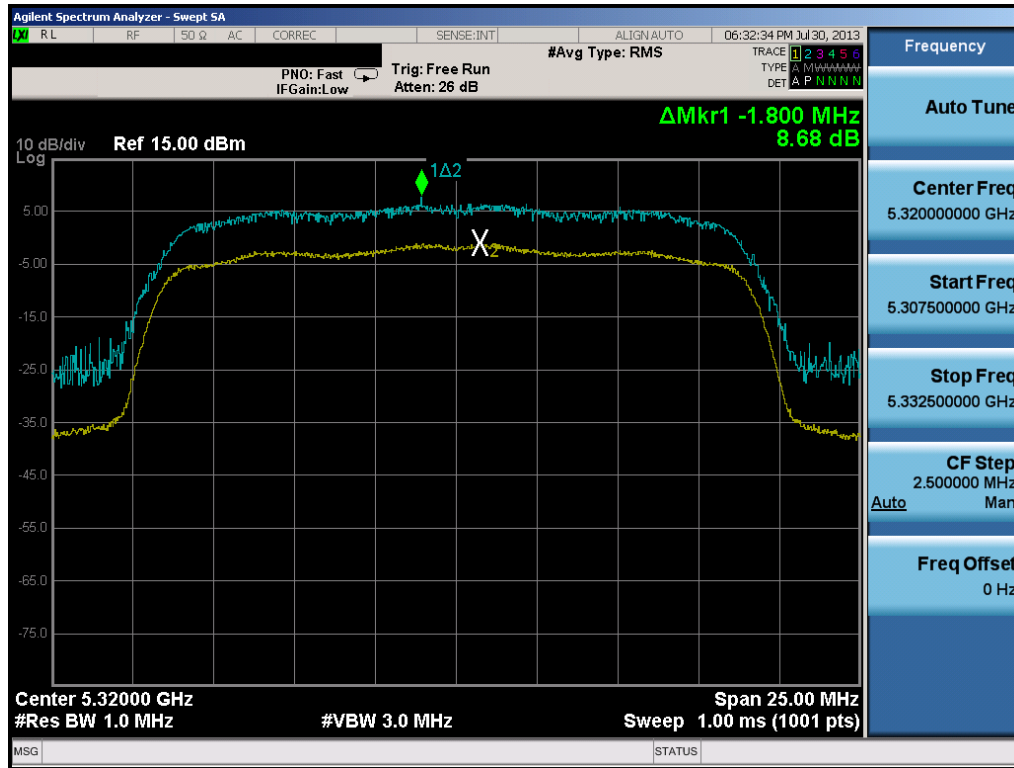
Plot 6-53. Peak Excursion Ratio Plot (20MHz BW 802.11n)
