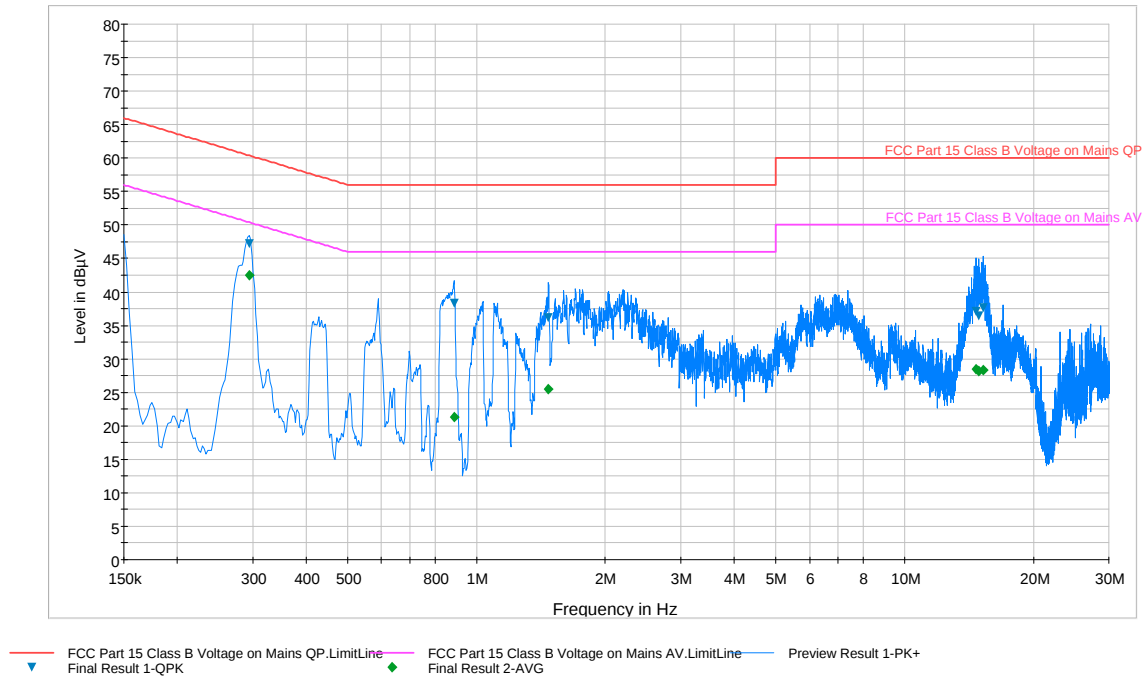
Plot 6-70. Line Conducted Plot with 802.11a UNII Band 1 (N)
