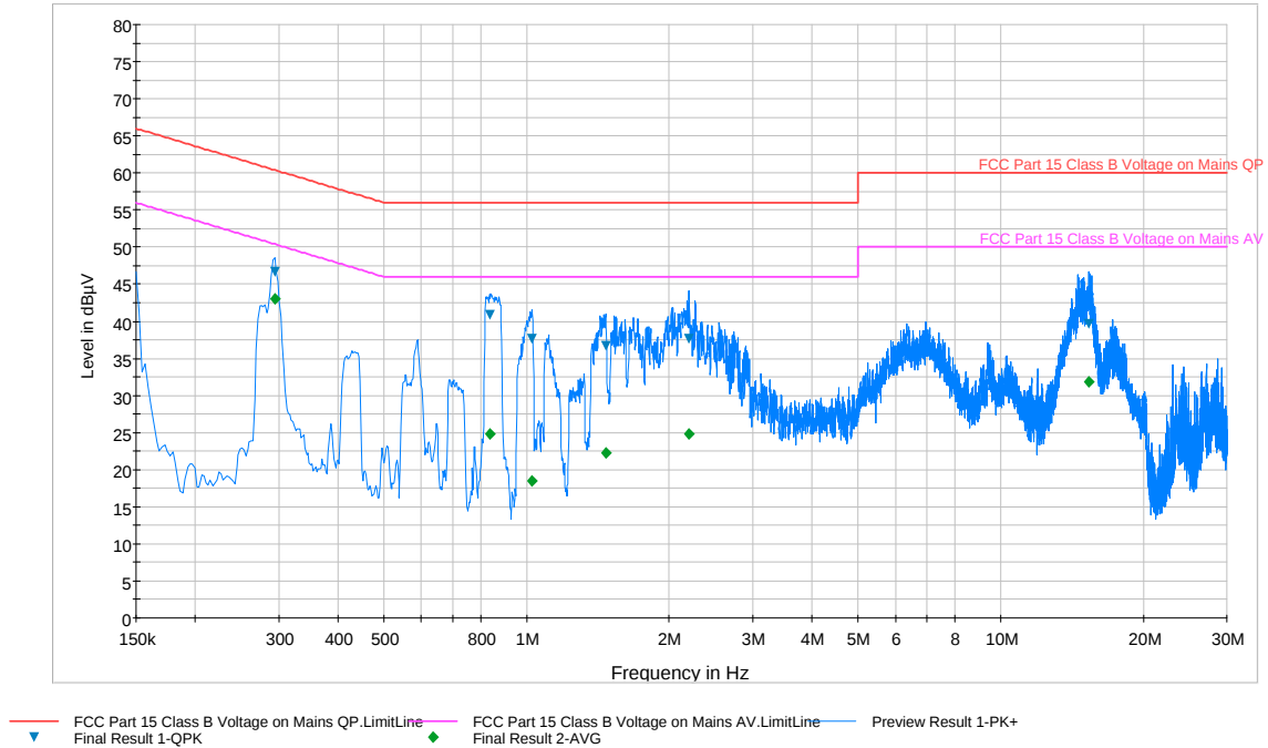
Plot 6-73. Line Conducted Plot with 802.11a UNII Band 3 (L1)
