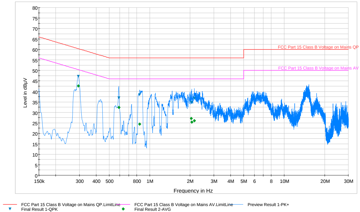
Plot 6-74. Line Conducted Plot with 802.11a UNII Band 3 (N)
