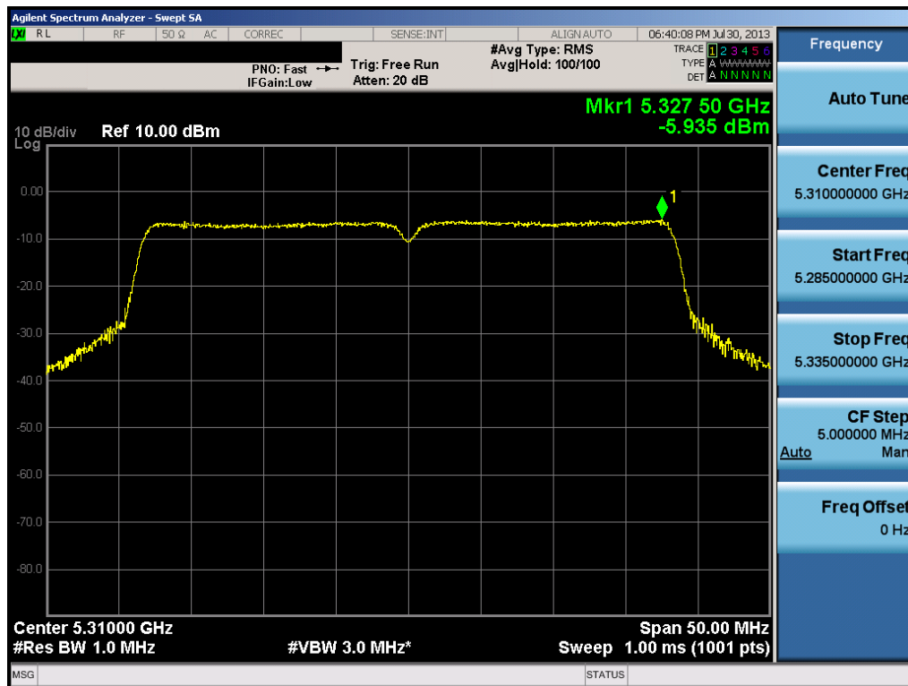
Plot 6-42. Peak Power Spectral Density Plot (40MHz BW 802.11n (UNII Band 2) – Ch. 62)
