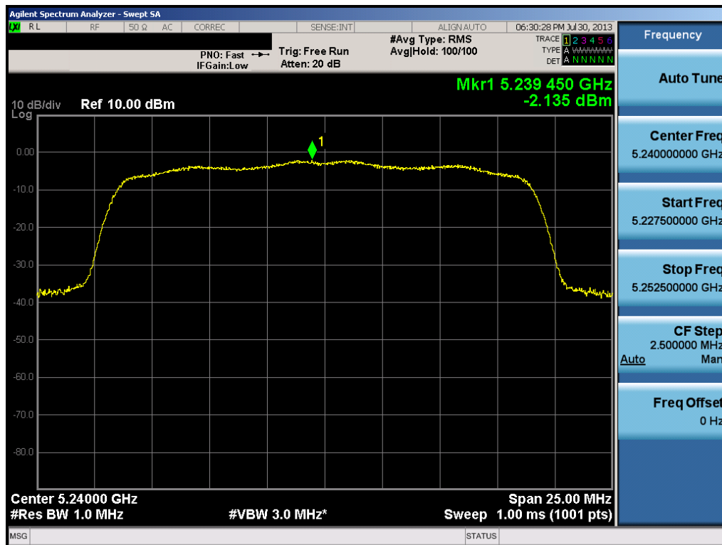
Plot 6-32. Peak Power Spectral Density Plot (20MHz BW 802.11n (UNII Band 1) – Ch. 48)
