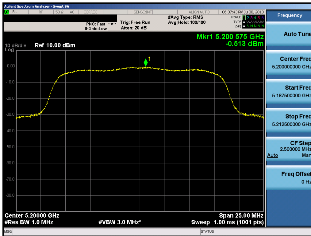
Plot 6-28. Peak Power Spectral Density Plot (802.11a (UNII Band 1) – Ch. 40)
