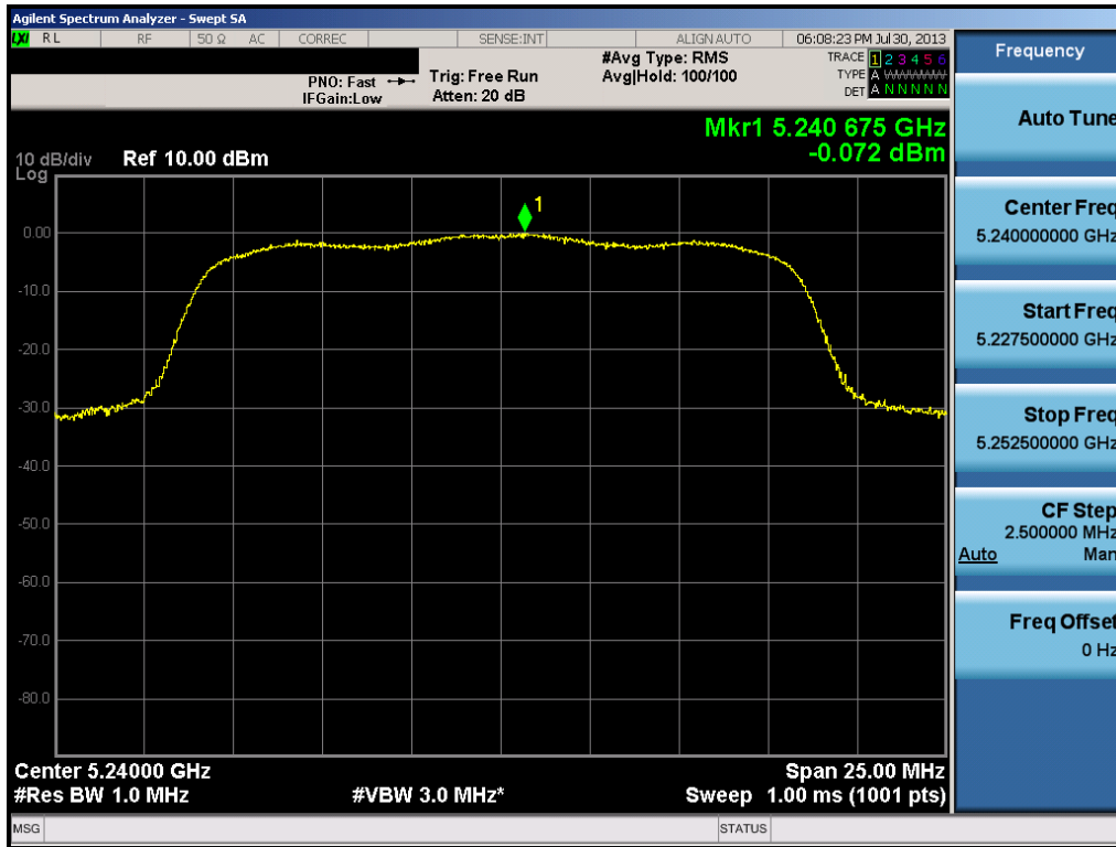
Plot 6-29. Peak Power Spectral Density Plot (802.11a (UNII Band 1) – Ch. 48)
