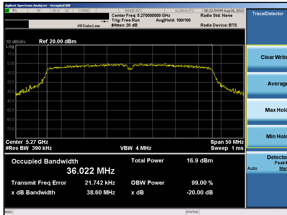
Plot 6-26. 20dB Bandwidth Plot (40MHz BW 802.11n (UNII Band 2) – Ch. 54)
