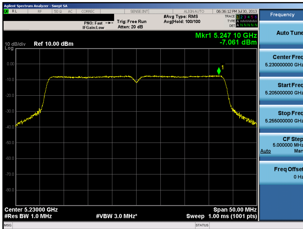
Plot 6-34. Peak Power Spectral Density Plot (40MHz BW 802.11n (UNII Band 1) – Ch. 46)
