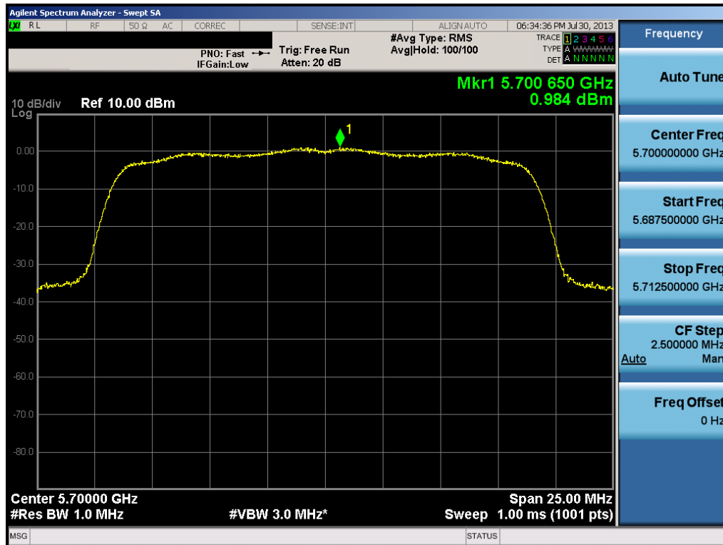
Plot 6-48. Peak Power Spectral Density Plot (20MHz BW 802.11n (UNII Band 3) – Ch. 140)
