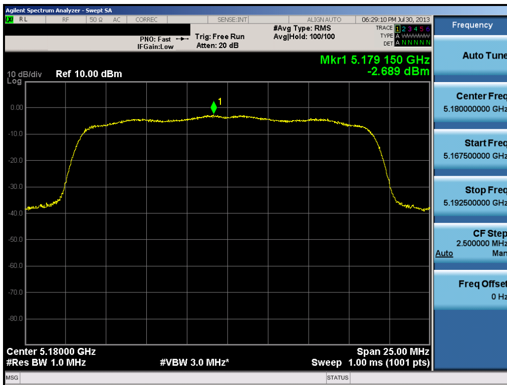
Plot 6-30. Peak Power Spectral Density Plot (20MHz BW 802.11n (UNII Band 1) – Ch. 36)
