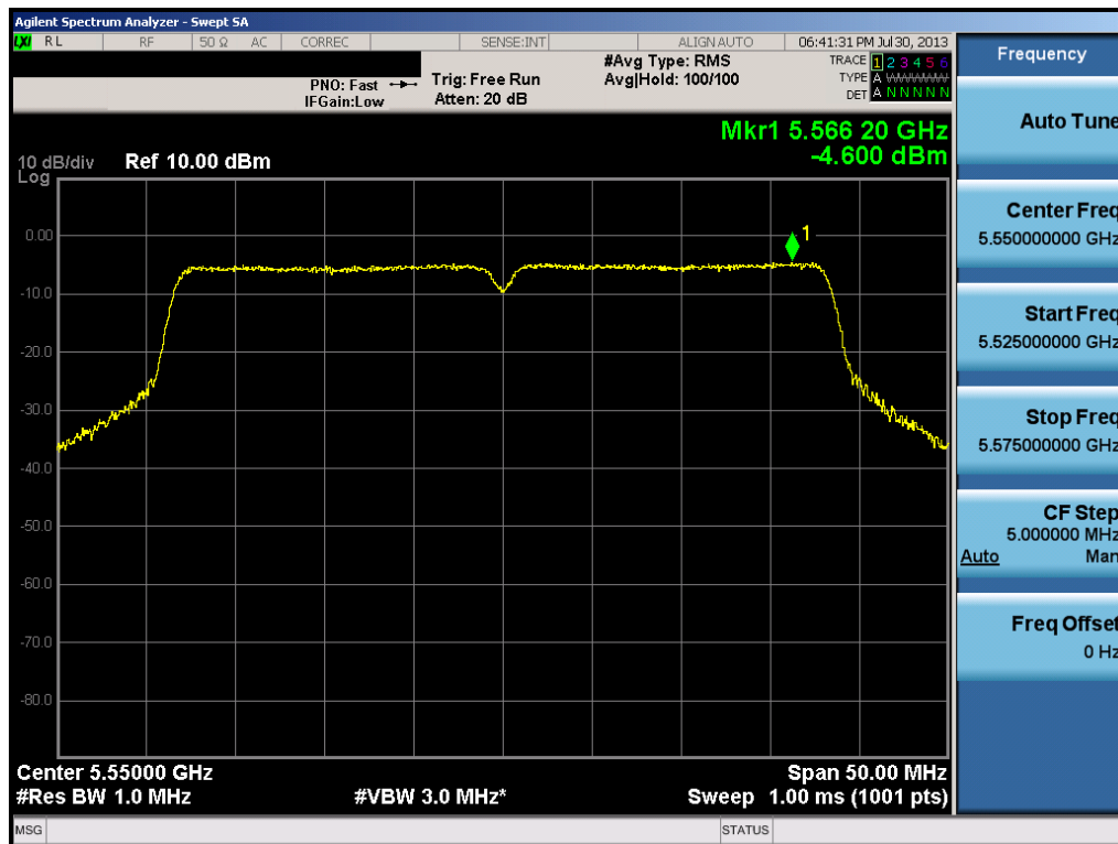
Plot 6-50. Peak Power Spectral Density Plot (40MHz BW 802.11n (UNII Band 3) – Ch. 110)
