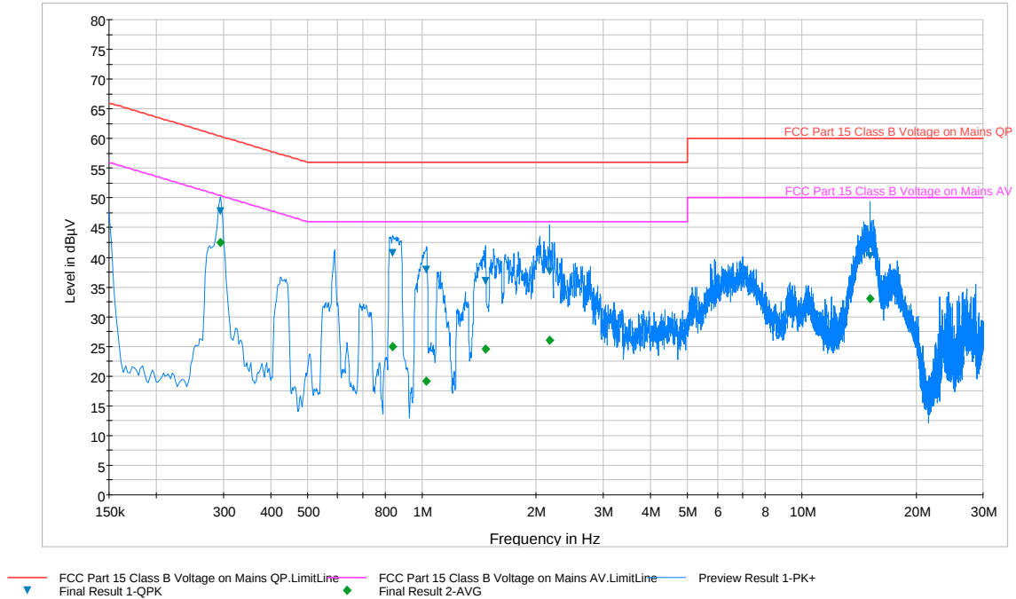
Plot 6-71. Line Conducted Plot with 802.11a UNII Band 2 (L1)
