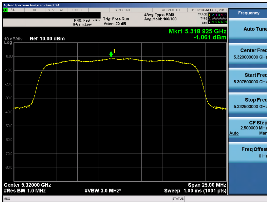
Plot 6-40. Peak Power Spectral Density Plot (20MHz BW 802.11n (UNII Band 2) – Ch. 64)
