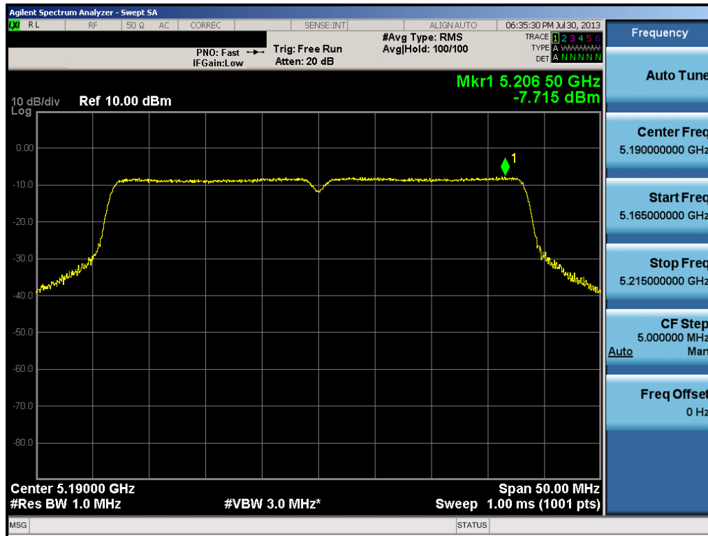
Plot 6-33. Peak Power Spectral Density Plot (40MHz BW 802.11n (UNII Band 1) – Ch. 38)
