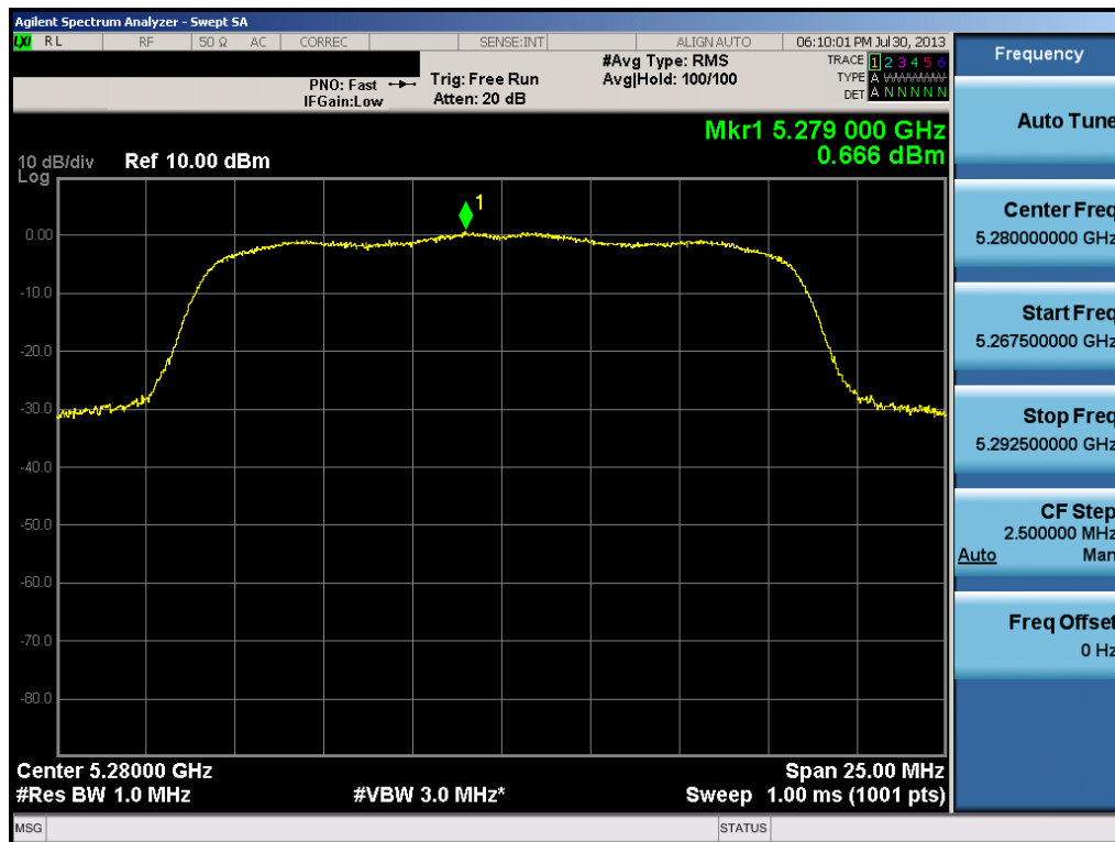
Plot 6-36. Peak Power Spectral Density Plot (802.11a (UNII Band 2) – Ch. 56)
