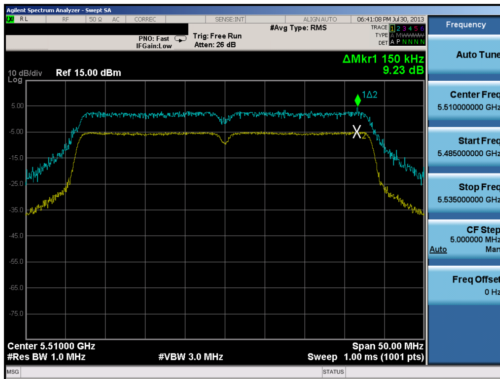
Plot 6-54. Peak Excursion Ratio Plot (40MHz BW 802.11n)
