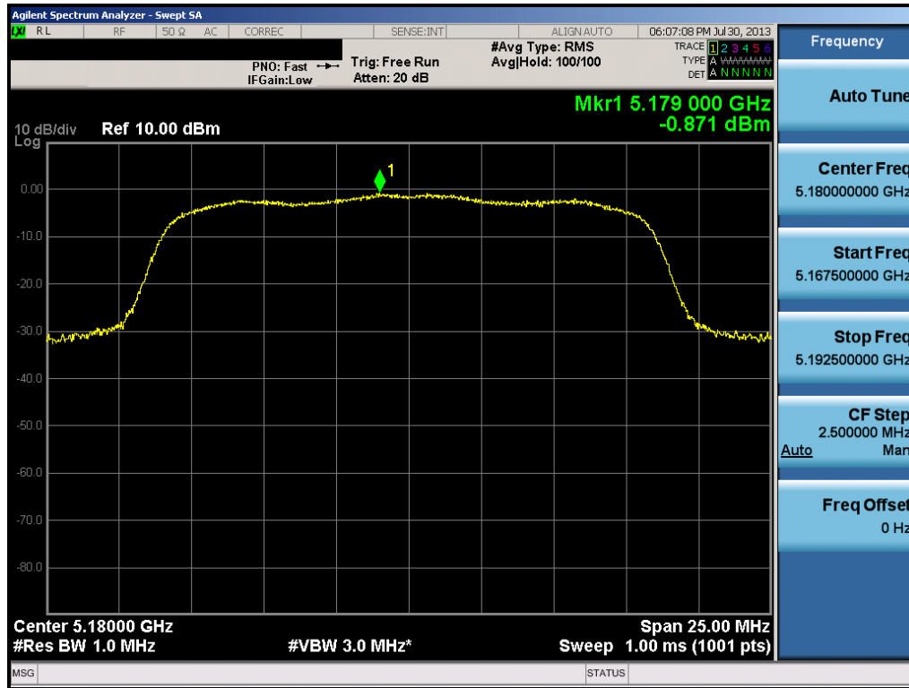
Plot 6-27. Peak Power Spectral Density Plot (802.11a (UNII Band 1) – Ch. 36)
