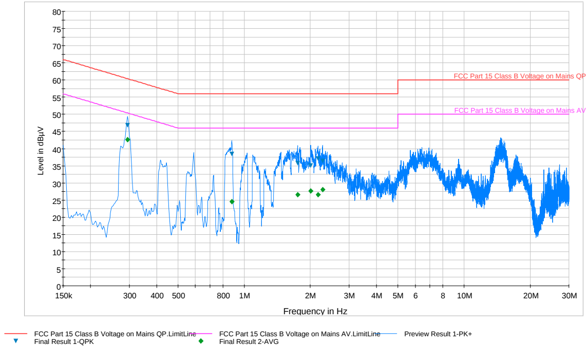
Plot 6-72. Line Conducted Plot with 802.11a UNII Band 2 (N)
