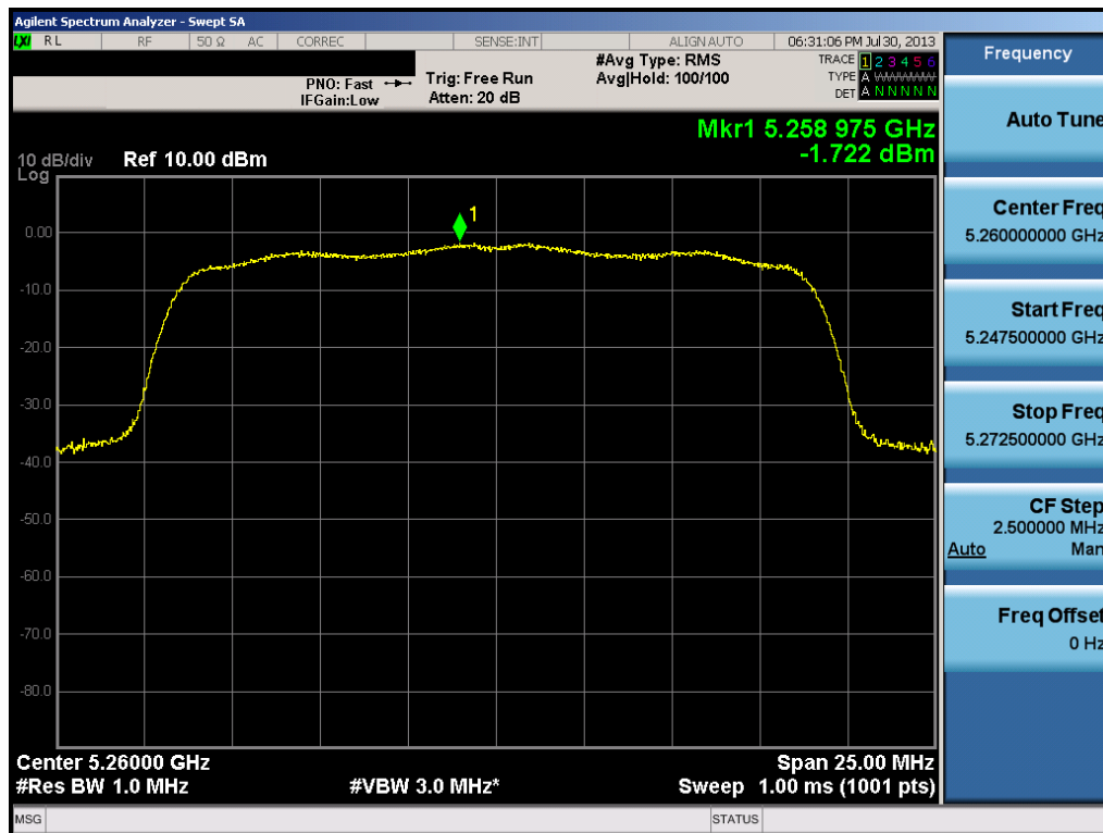
Plot 6-38. Peak Power Spectral Density Plot (20MHz BW 802.11n (UNII Band 2) – Ch. 52)
