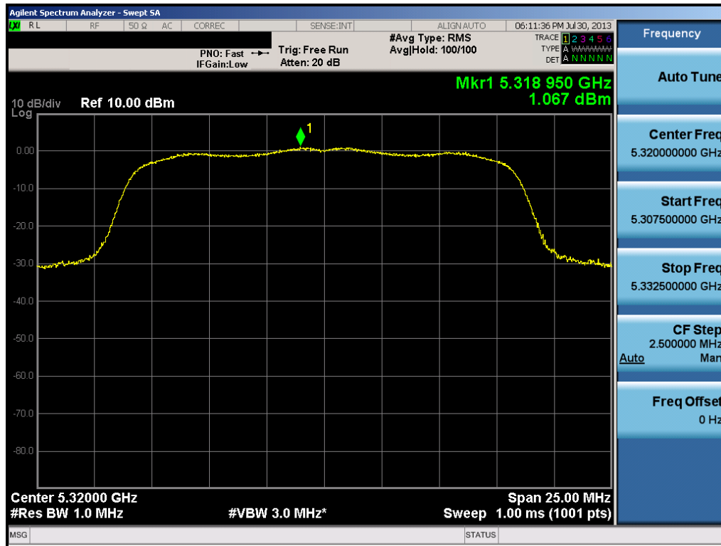
Plot 6-37. Peak Power Spectral Density Plot (802.11a (UNII Band 2) – Ch. 64)
