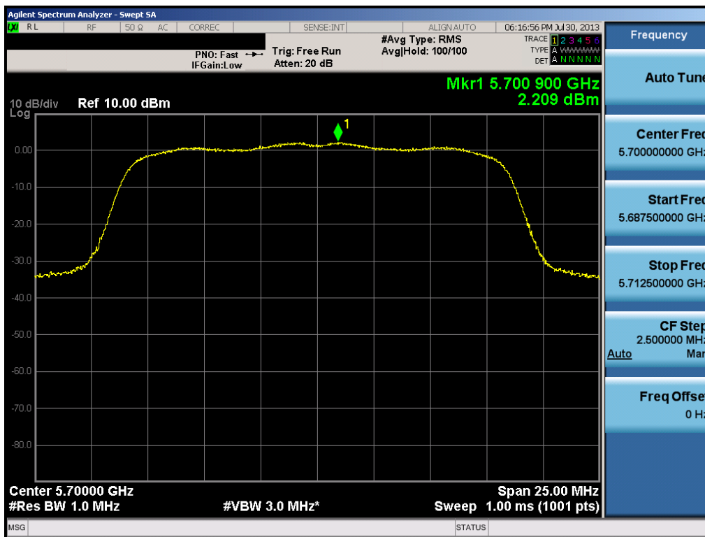
Plot 6-45. Peak Power Spectral Density Plot (802.11a (UNII Band 3) – Ch. 140)
