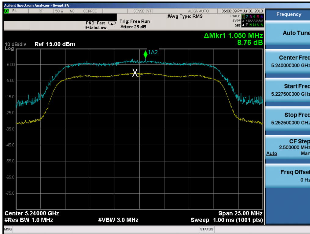
Plot 6-52. Peak Excursion Ratio Plot (802.11a)
