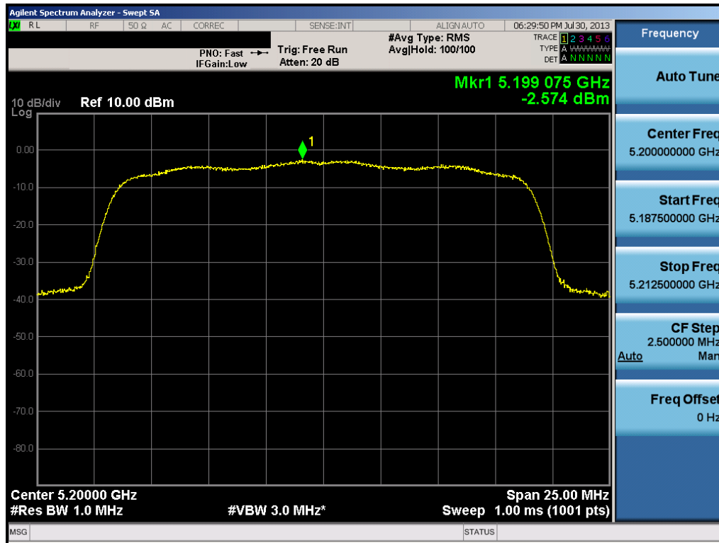
Plot 6-31. Peak Power Spectral Density Plot (20MHz BW 802.11n (UNII Band 1) – Ch. 40)
