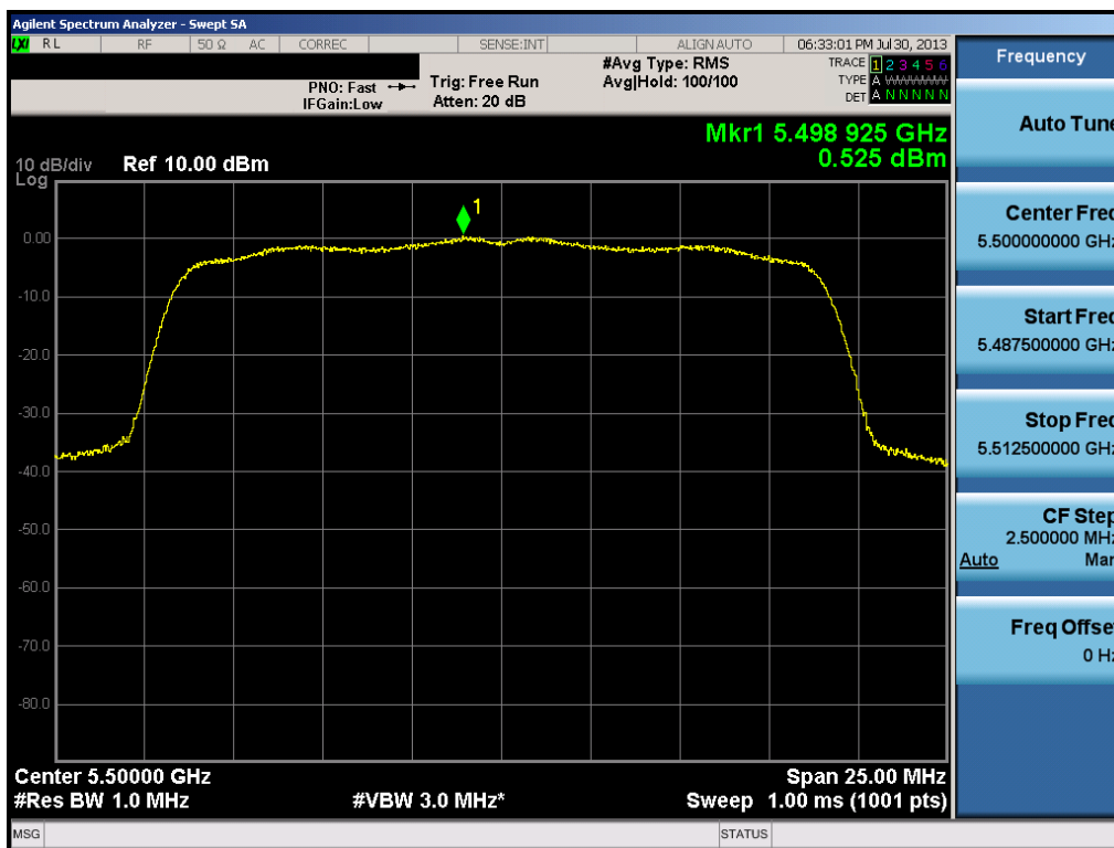
Plot 6-46. Peak Power Spectral Density Plot (20MHz BW 802.11n (UNII Band 3) – Ch. 100)
