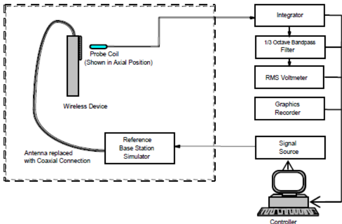
Figure 5-14 Audio Magnetic Field Test Setup
