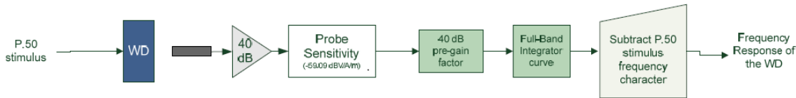
Figure 5-13 Frequency Response Block Diagram
