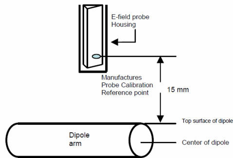
Figure 7-1 Separation Distance from Dipole to Field Probe
