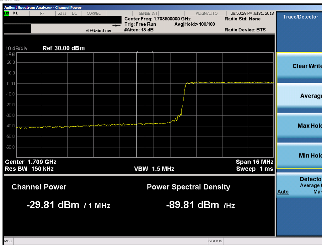
Plot 9-44. Lower Extended Band Edge Plot (20.0MHz QPSK – RB Size 100)
