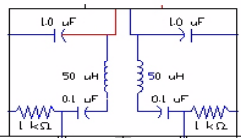
Figure 3-4. LISN Schematic Diagram
