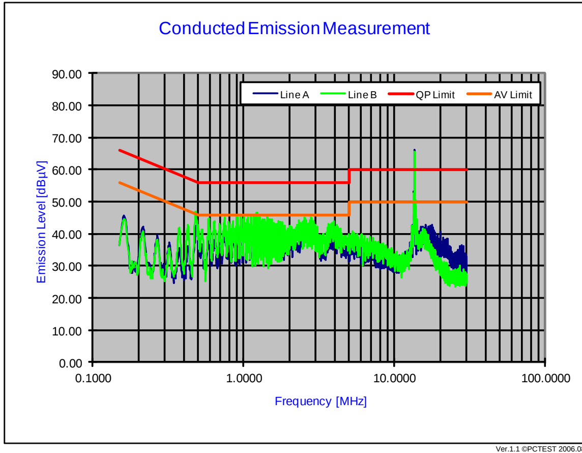
Plot 8-1. Line-Conducted Test Plot
