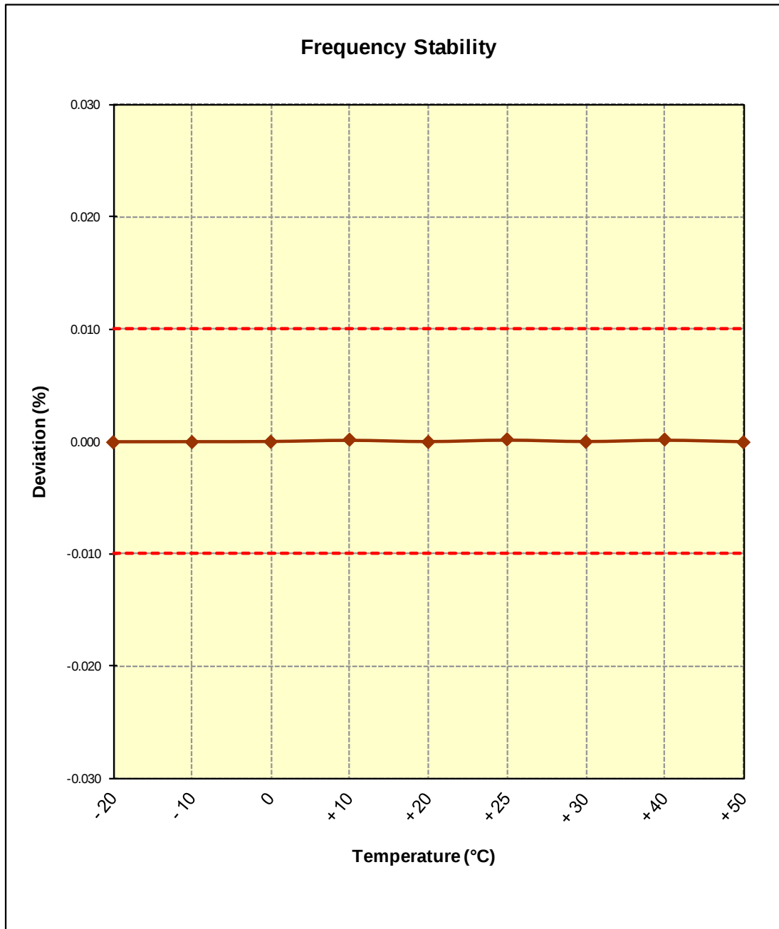
Figure 8-3. Frequency Stability Plot
