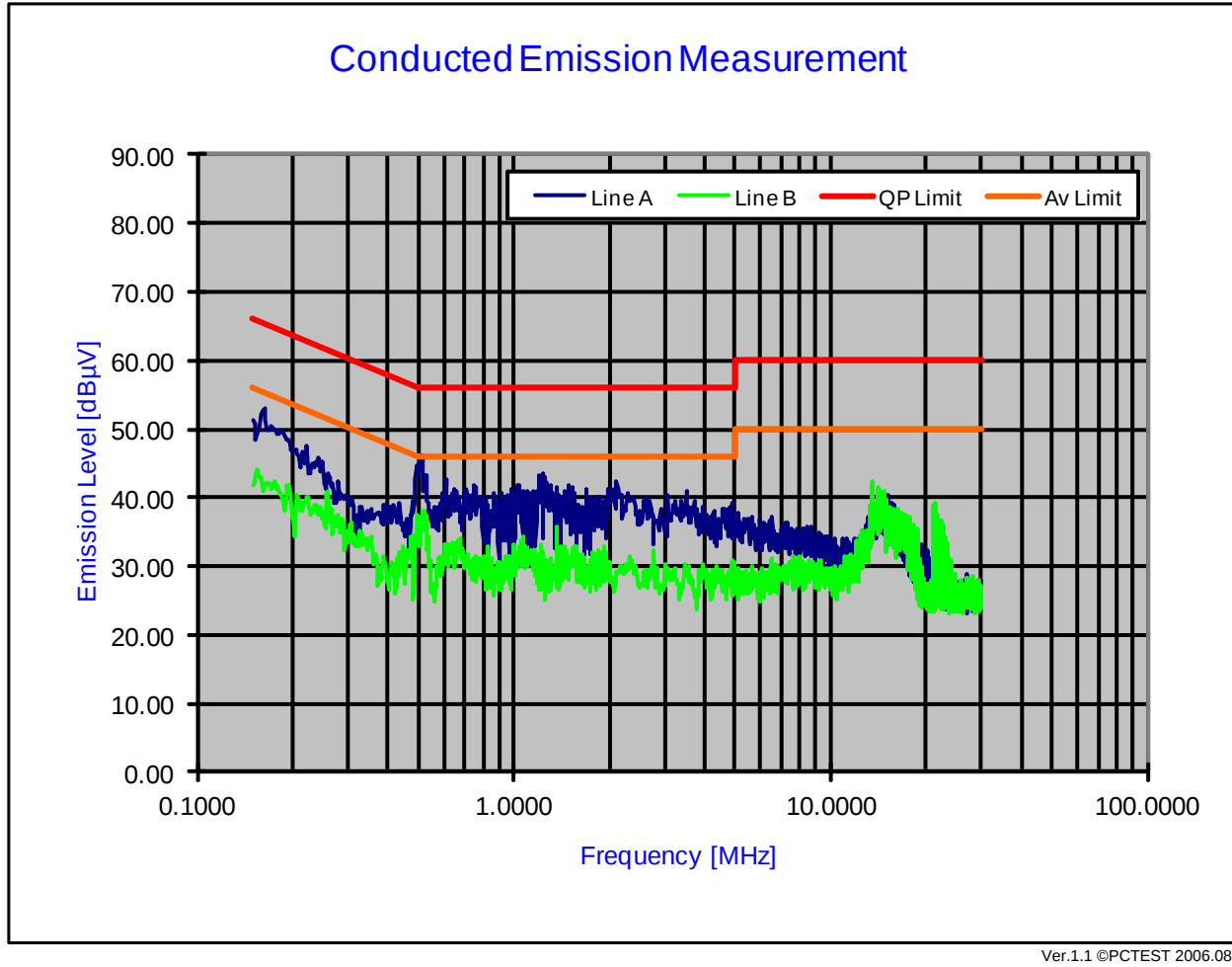
Plot 6-18. Line Conducted Plot with Bluetooth (LE)
