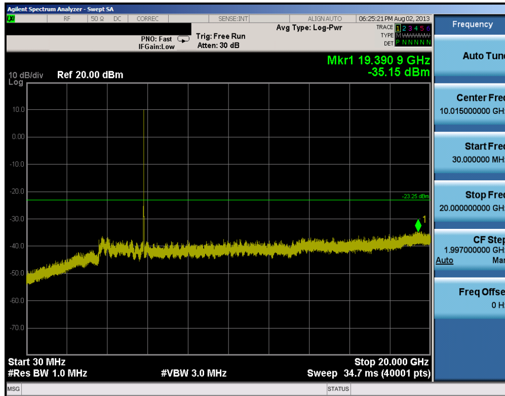
Plot 6-59. Conducted Spurious Plot (802.11a – Ch. 165)
