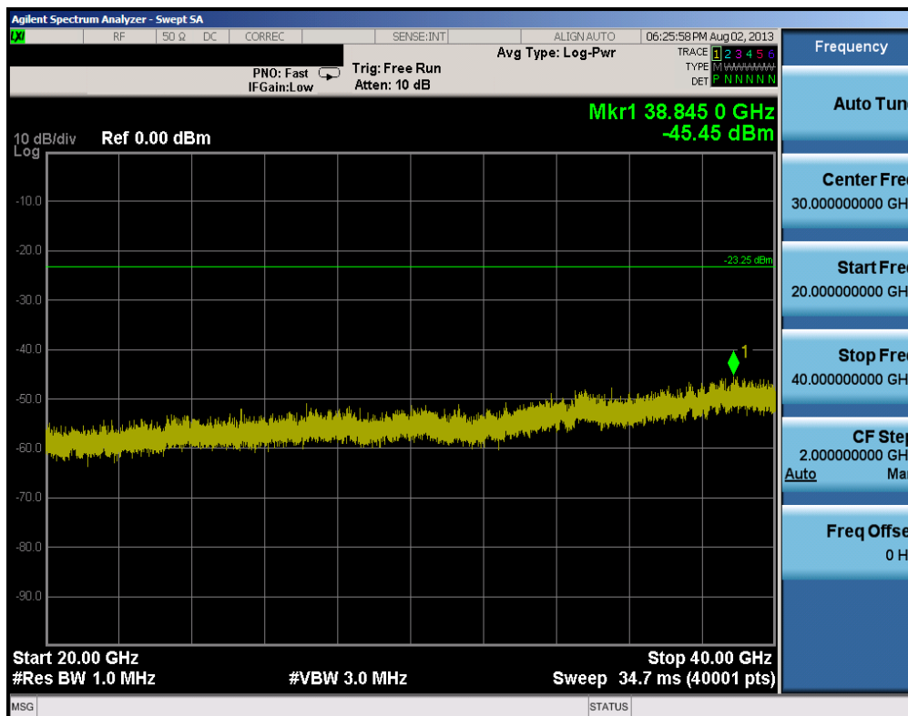
Plot 6-60. Conducted Spurious Plot (802.11a – Ch. 165)
