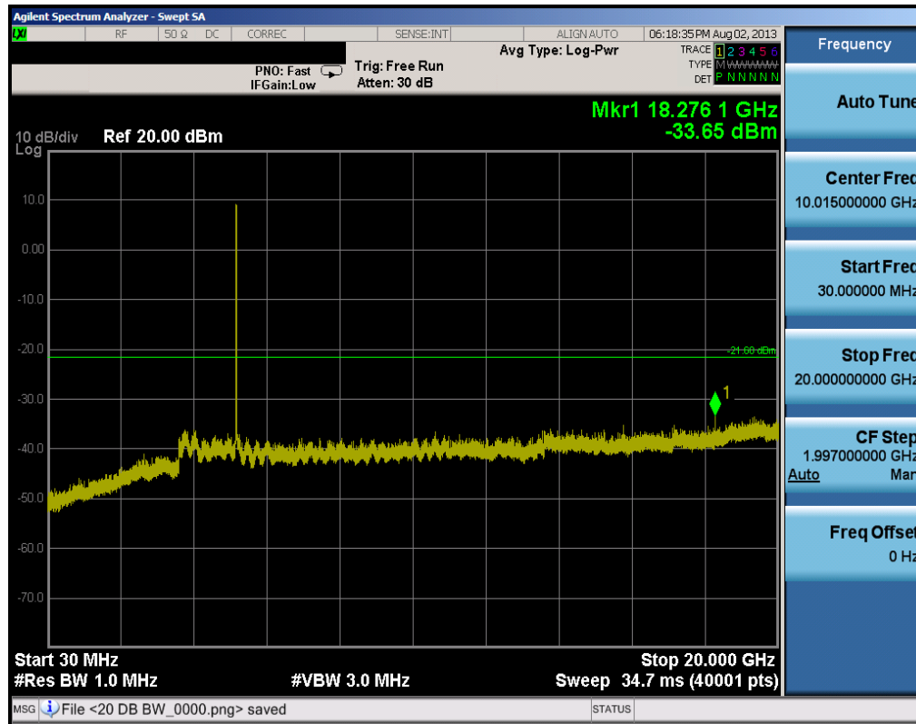
Plot 6-55. Conducted Spurious Plot (802.11a – Ch. 149)
