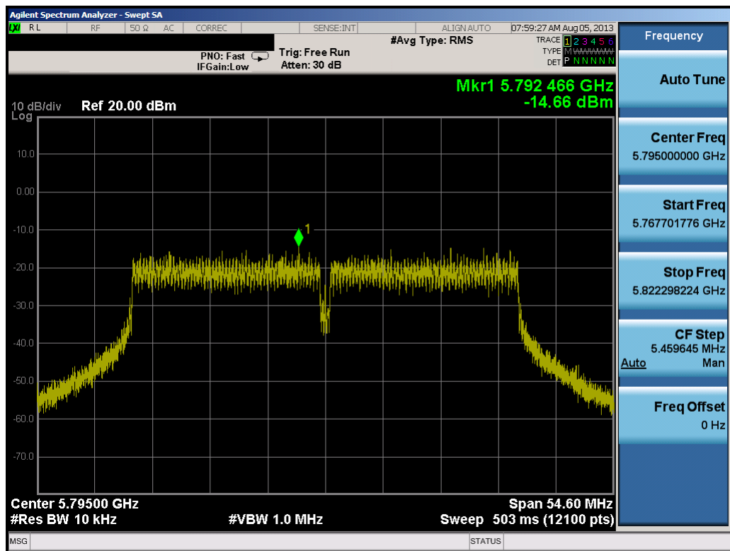
Plot 6-36. Power Spectral Density Plot (40MHz BW 802.11n (5.8GHz) – Ch. 159)
