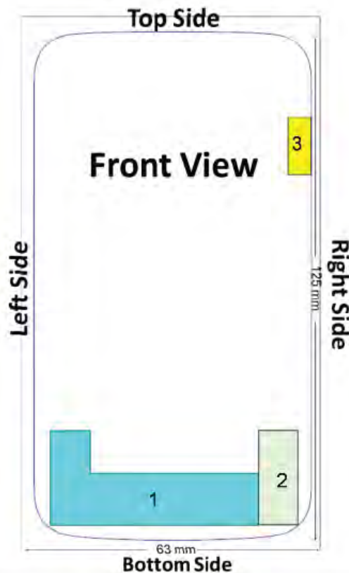
Figure 1-1 DUT Antenna Locations
