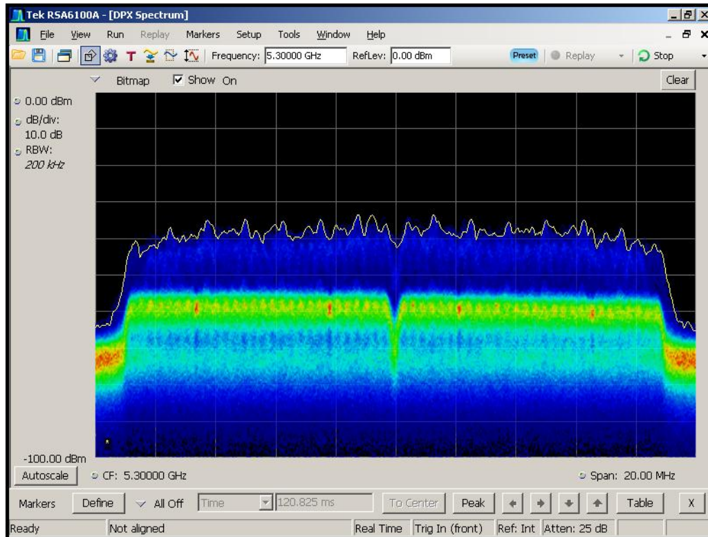
Figure 5-3. Real-Time Spectrum Display, WLAN Traffic (Streaming Video)
